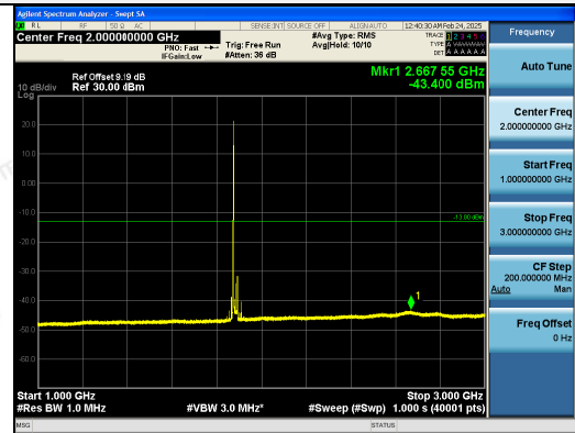
1GHz~3GHz
