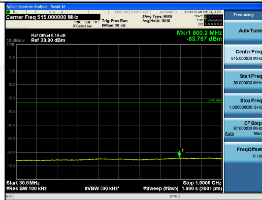
30MHz~1GHz
