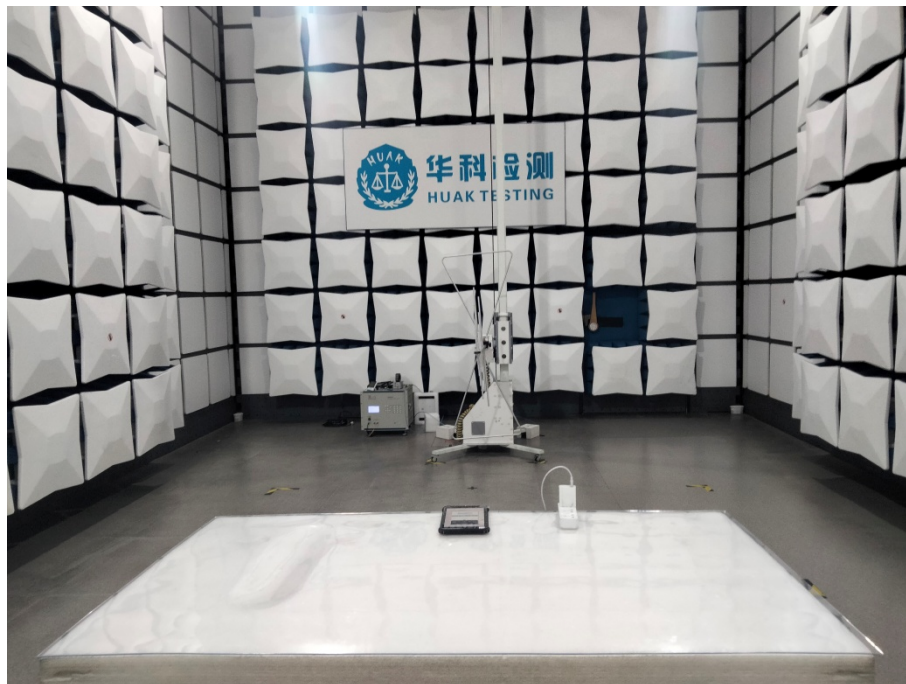
Test Model: K8 Active Radiated Emissions
