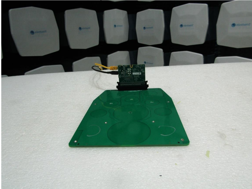
Radiated Spurious - Above 1 GHz
