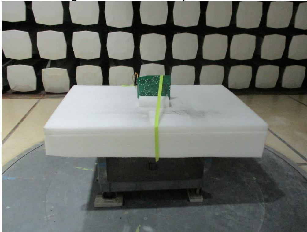
Field Strength and Radiated Spurious below 1 GHz
