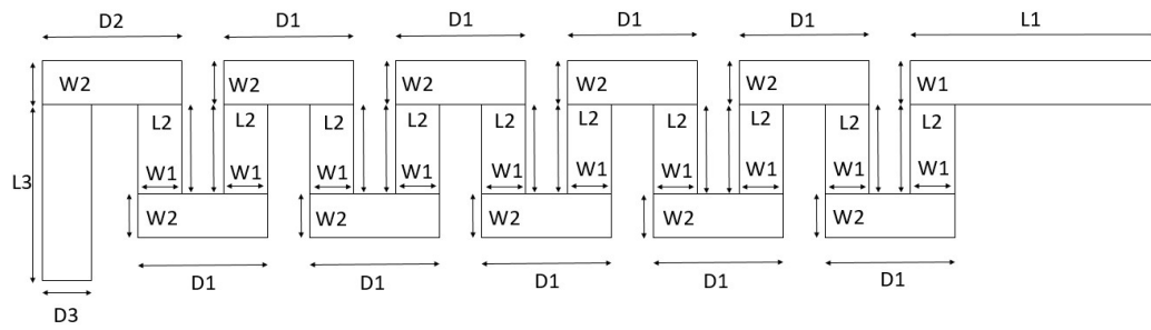
Antenna Dimensions
