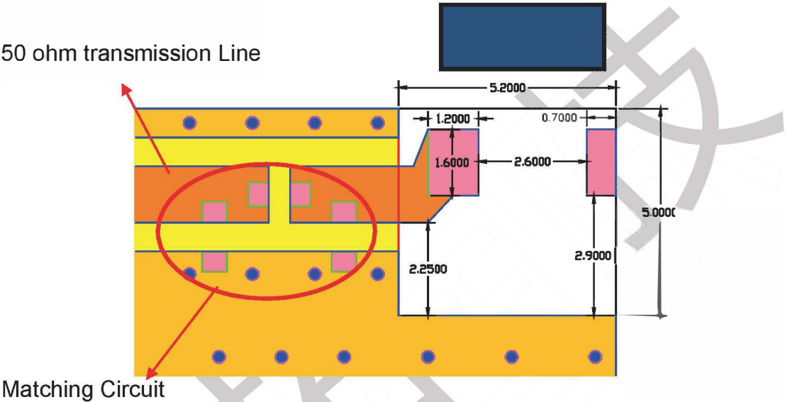
Layout Dimensions in Clearance area(Size=5.2*5.0mm)
