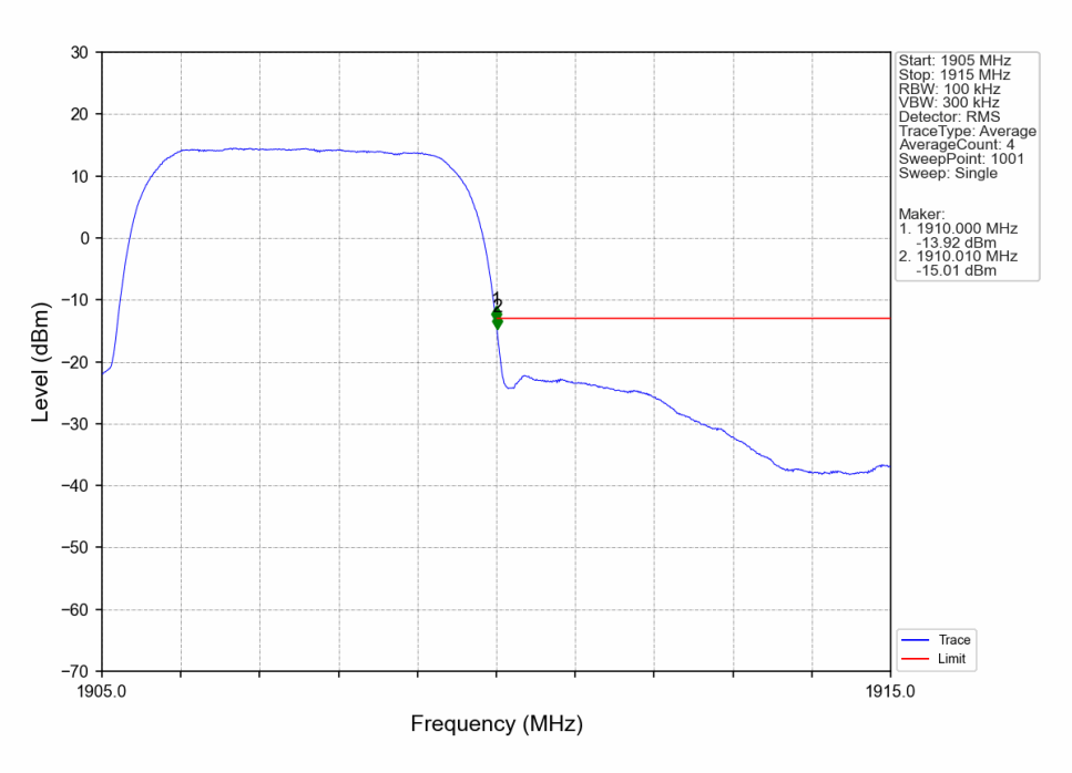
BandII_RMC_HCH_1907.6MHz_12.2kbps_RMC_NTNV
