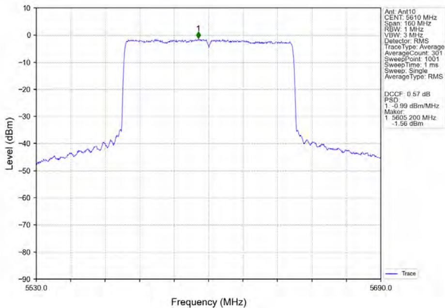
802.11ax(HEW80)_HCH_5610MHz_SU_/_Ant10_NTNV
