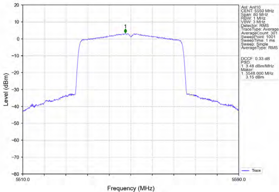
802.11ax(HEW40)_MCH_5550MHz_SU_/_Ant10_NTNV
