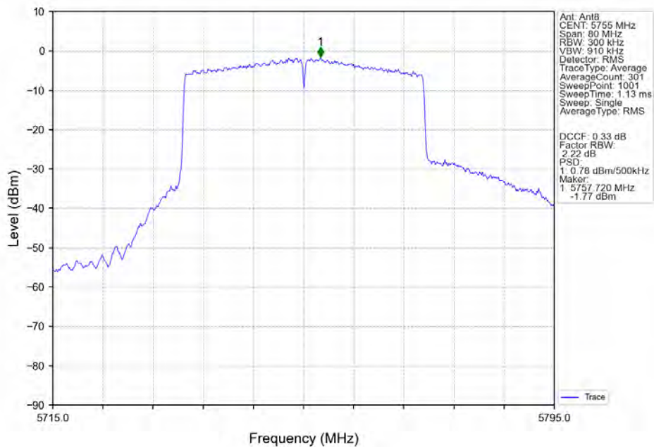
802.11ax(HEW40)_LCH_5755MHz_SU_/_Ant8_NTNV
