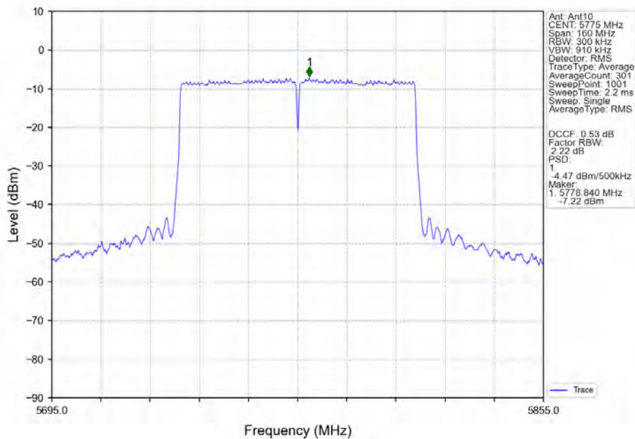
802.11ac(VHT80)_MCH_5775MHz_Ant10_NTNV
