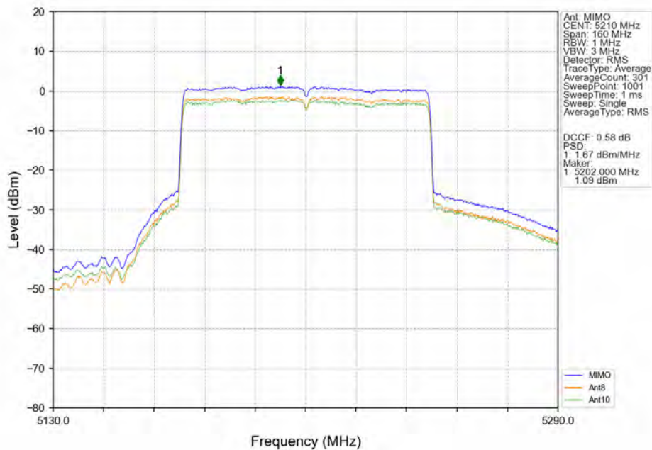
802.11ax(HEW80)_MCH_5210MHz_SU_/_MIMO_NTNV
