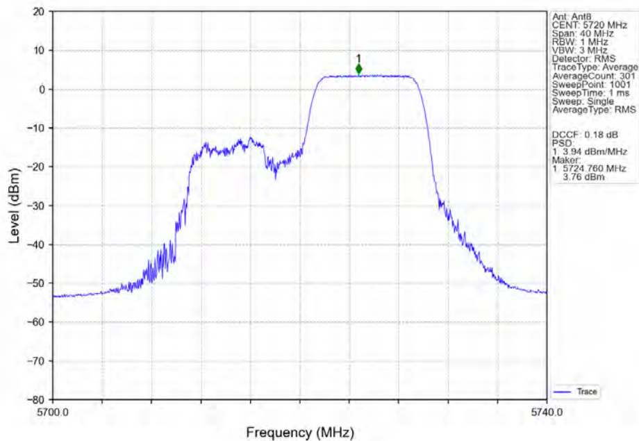
802.11ax(HEW20)_HCH_5720MHz_RU106_Right_Ant8_NTNV
