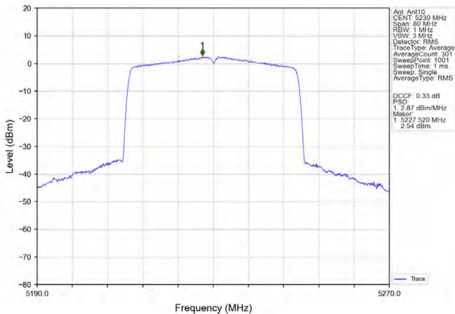
802.11ax(HEW40)_HCH_5230MHz_SU_/_Ant10_NTNV
