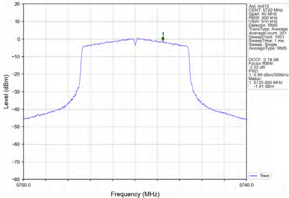
802.11ax(HEW20)_HCH_5720MHz_SU_/_MIMO_NTNV
