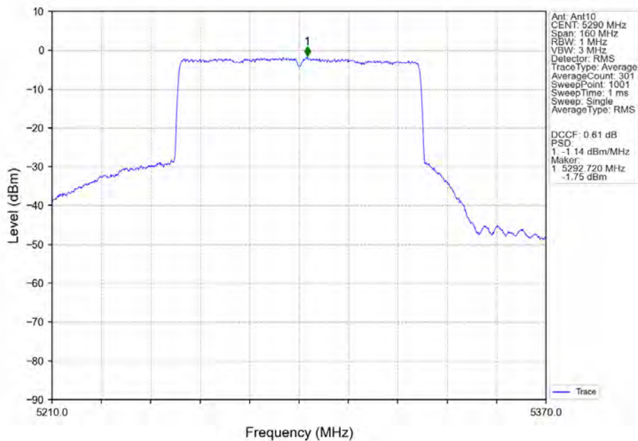
802.11ax(HEW80)_MCH_5290MHz_SU_/_Ant10_NTNV
