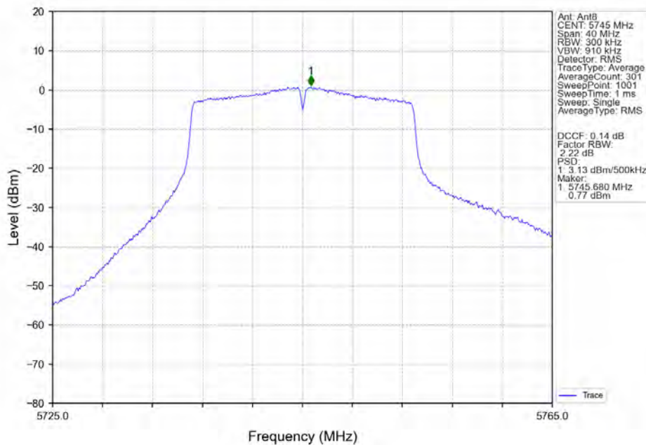
802.11ac(VHT20)_LCH_5745MHz_Ant8_NTNV
