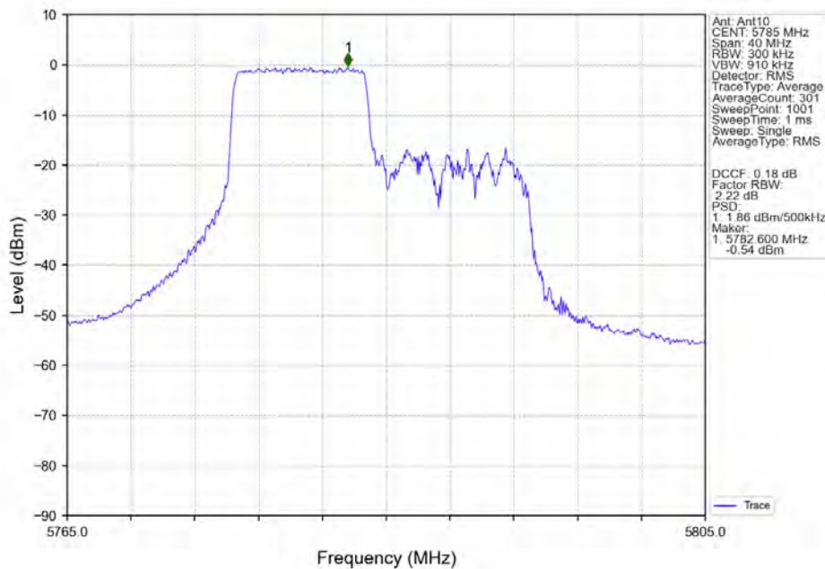
802.11ax(HEW20)_MCH_5785MHz_RU106_Left_Ant10_NTNV
