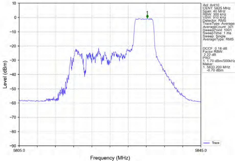
802.11ax(HEW20)_HCH_5825MHz_RU52_Right_MIMO_NTNV
