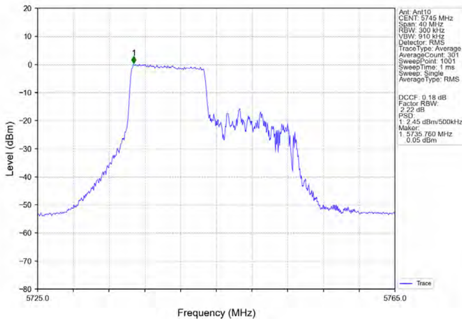
802.11ax(HEW20)_LCH_5745MHz_RU106_Left_Ant10_NTNV
