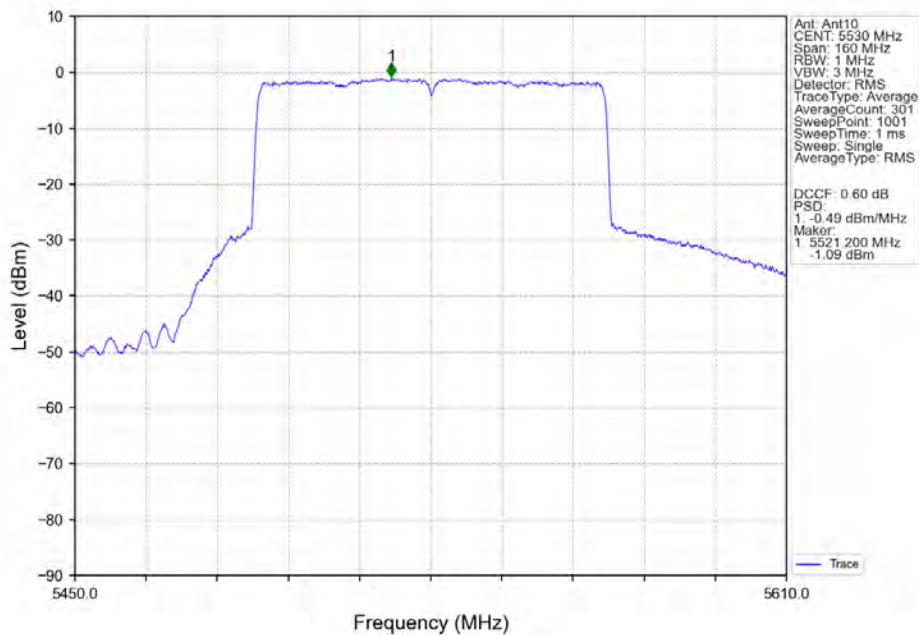
802.11ax(HEW80)_LCH_5530MHz_SU_/_Ant10_NTNV
