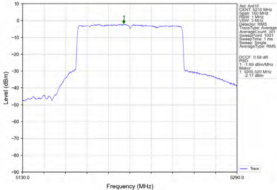
802.11ax(HEW80)_MCH_5210MHz_SU_/_MIMO_NTNV
