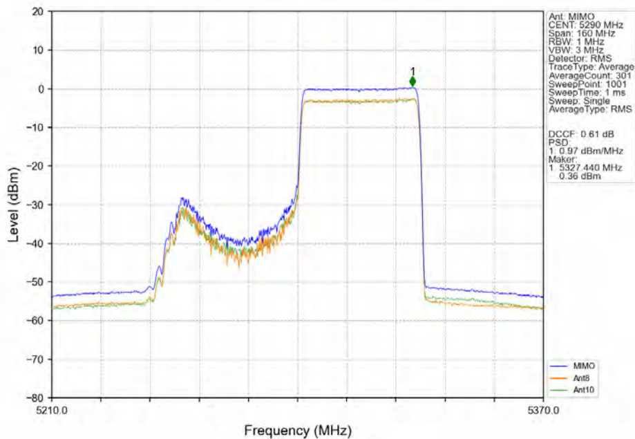
802.11ax(HEW80)_MCH_5290MHz_RU484_Right_MIMO_NTNV
