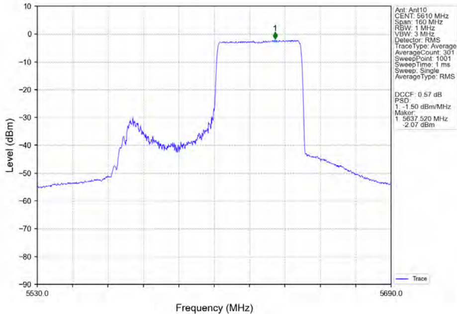
802.11ax(HEW80)_HCH_5610MHz_RU484_Right_MIMO_NTNV
