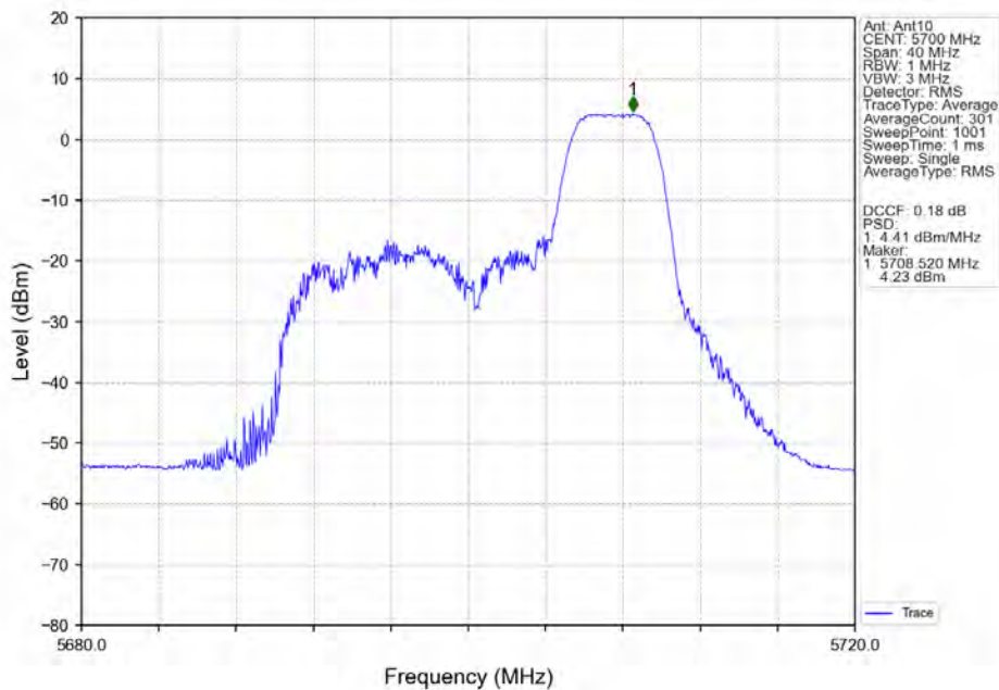
802.11ax(HEW20)_HCH_5700MHz_RU52_Right_Ant10_NTNV
