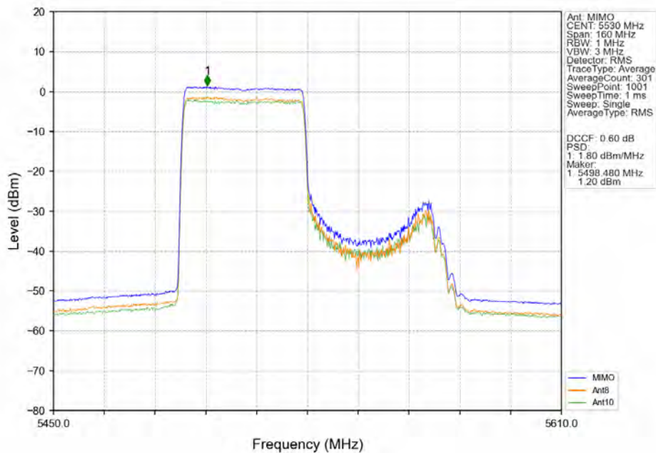
802.11ax(HEW80)_LCH_5530MHz_RU484_Left_MIMO_NTNV
