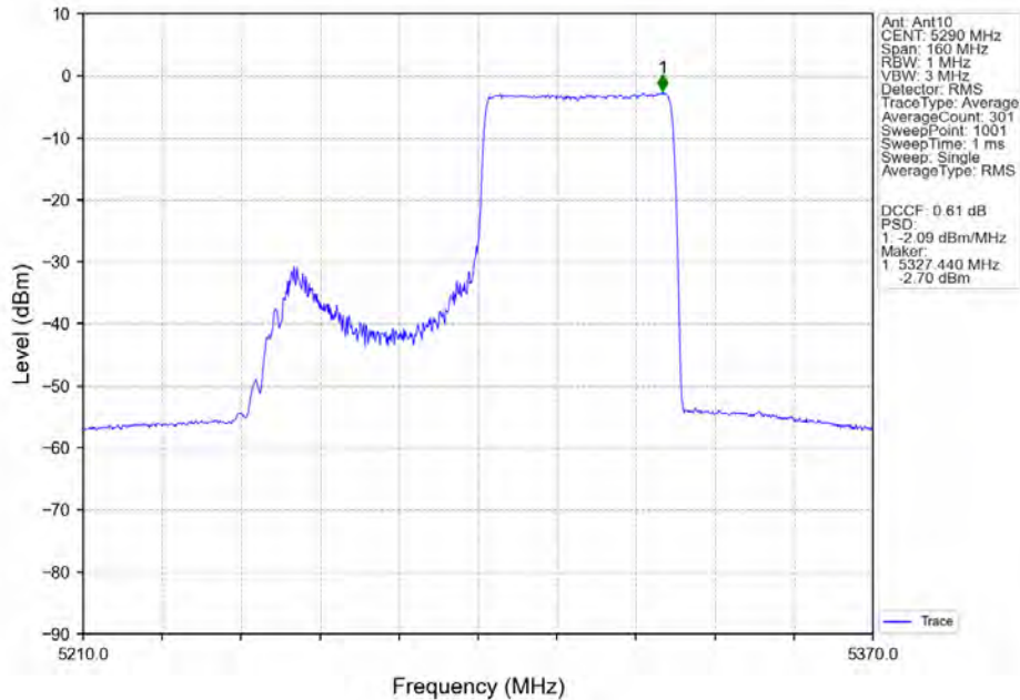
802.11ax(HEW80)_MCH_5290MHz_RU484_Right_MIMO_NTNV
