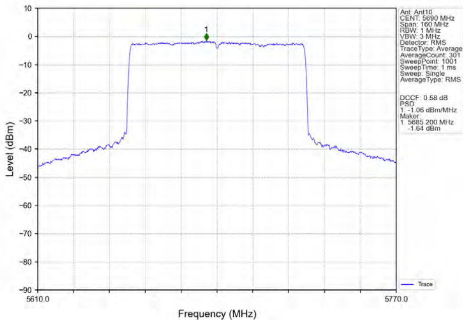
802.11ax(HEW80)_HCH_5690MHz_SU_/_Ant10_NTNV
