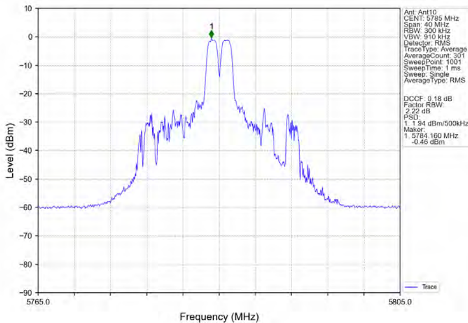
802.11ax(HEW20)_MCH_5785MHz_RU26_Mid_Ant10_NTNV
