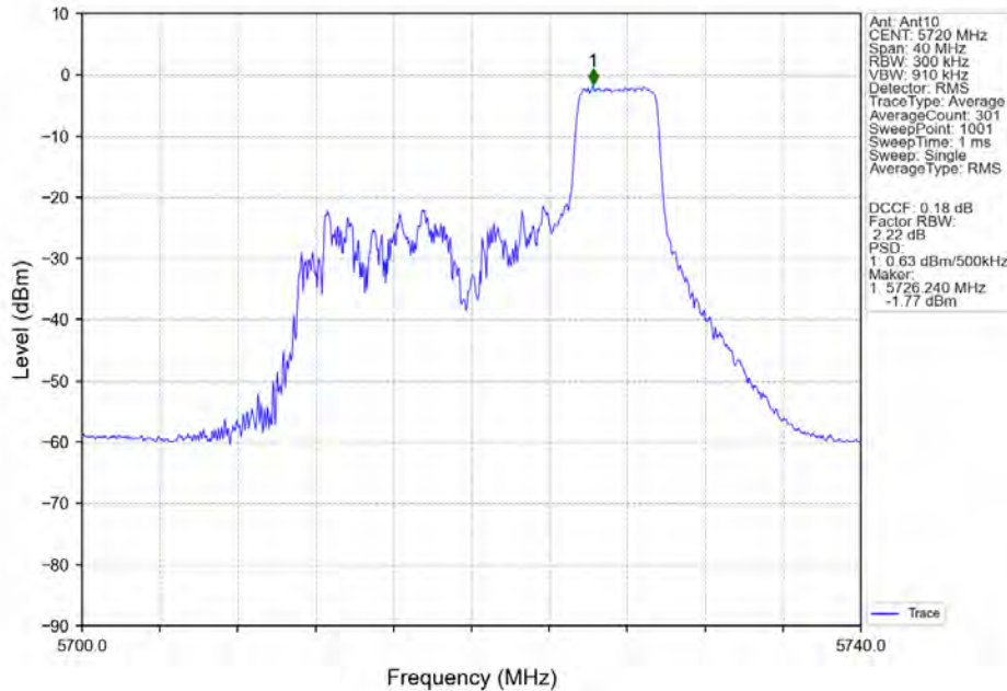
802.11ax(HEW20)_HCH_5720MHz_RU52_Right_MIMO_NTNV
