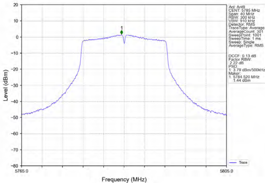
802.11a_MCH_5785MHz_Ant8_NTNV
