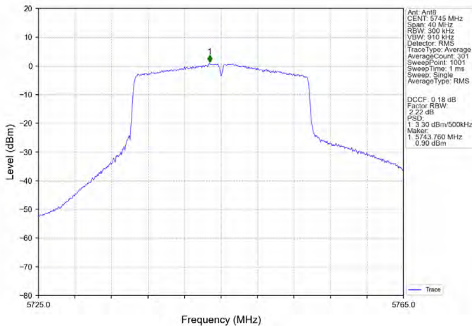
802.11ax(HEW20)_LCH_5745MHz_SU_/_Ant8_NTNV
