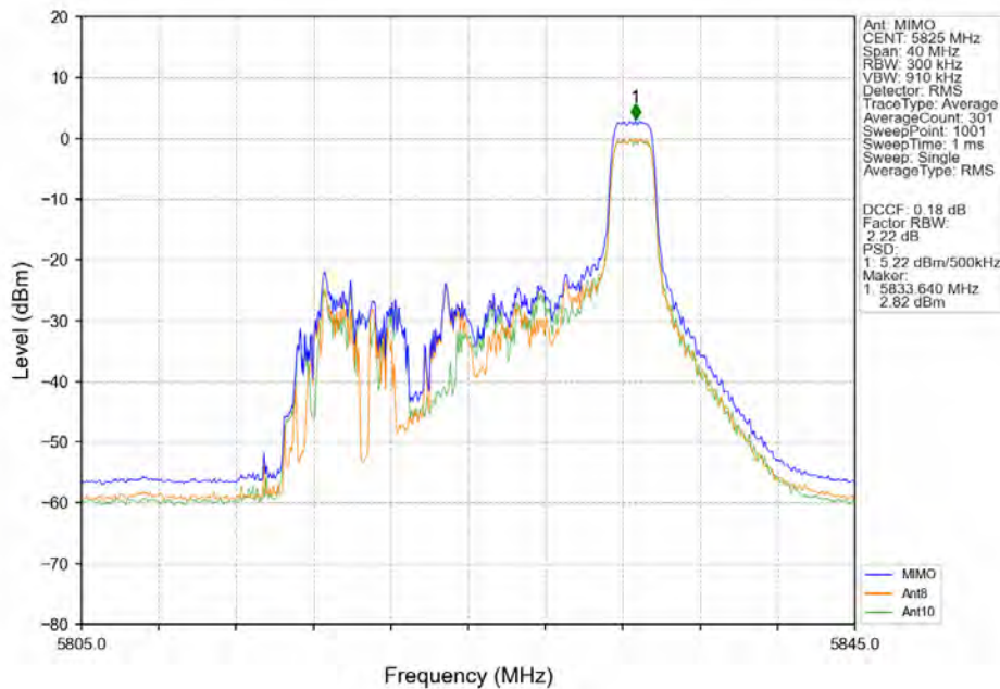
802.11ax(HEW20)_HCH_5825MHz_RU52_Right_Ant8_NTNV
