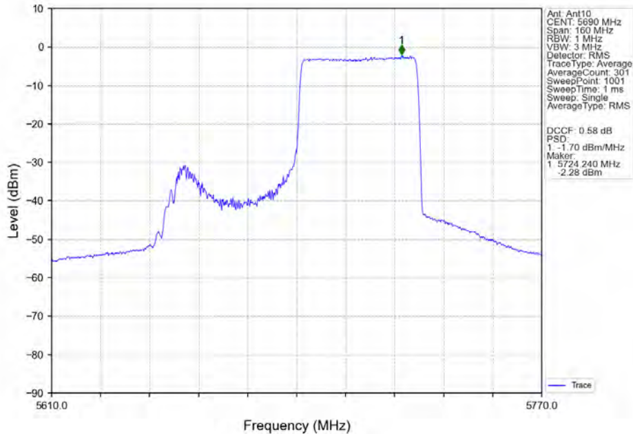
802.11ax(HEW80)_HCH_5690MHz_RU484_Right_MIMO_NTNV
