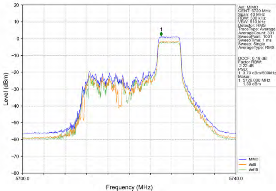
802.11ax(HEW20)_HCH_5720MHz_RU52_Right_MIMO_NTNV
