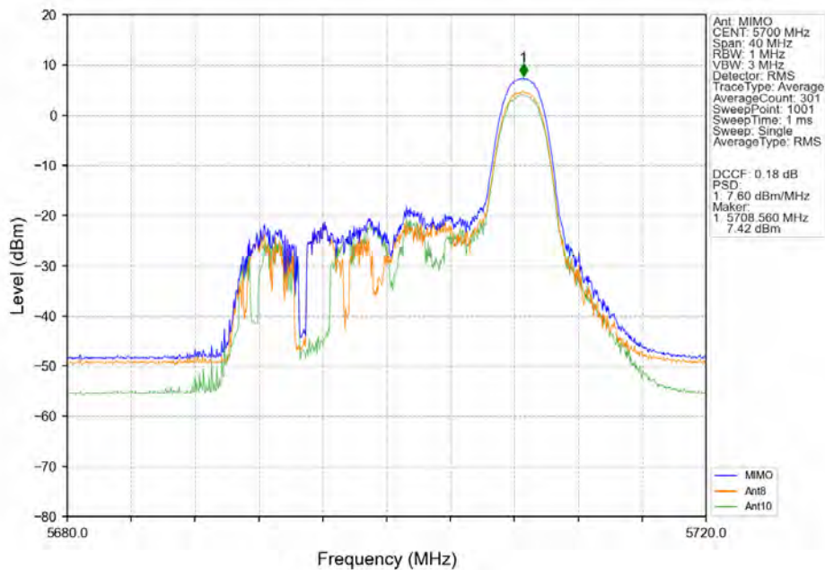
802.11ax(HEW20)_HCH_5700MHz_RU26_Right_MIMO_NTNV
