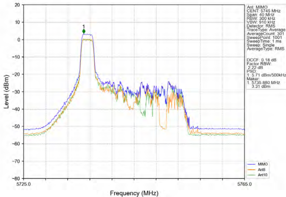
802.11ax(HEW20)_LCH_5745MHz_RU52_Left_Ant8_NTNV
