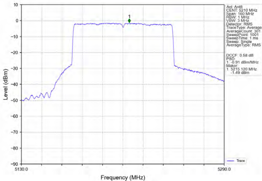
802.11ax(HEW80)_MCH_5210MHz_SU_/_Ant8_NTNV
