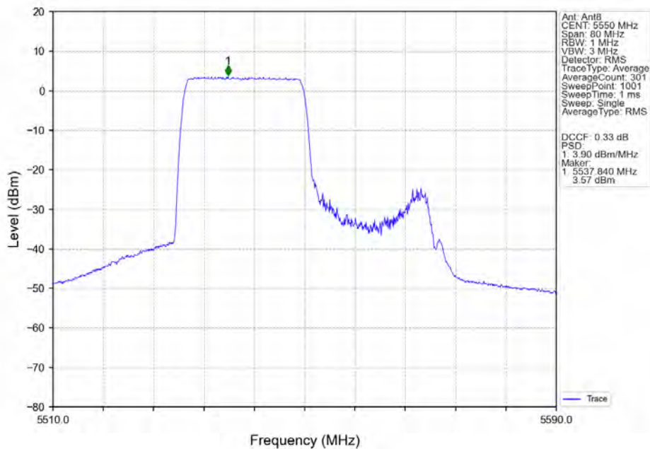
802.11ax(HEW40)_MCH_5550MHz_RU242_Left_Ant8_NTNV
