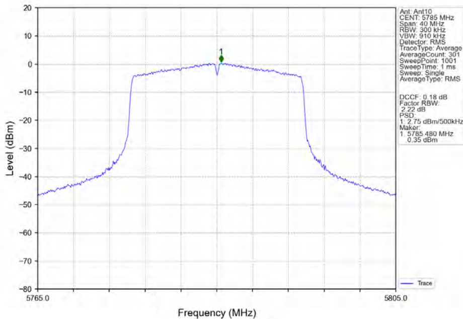
802.11ax(HEW20)_MCH_5785MHz_SU_ / _MIMO_NTNV
