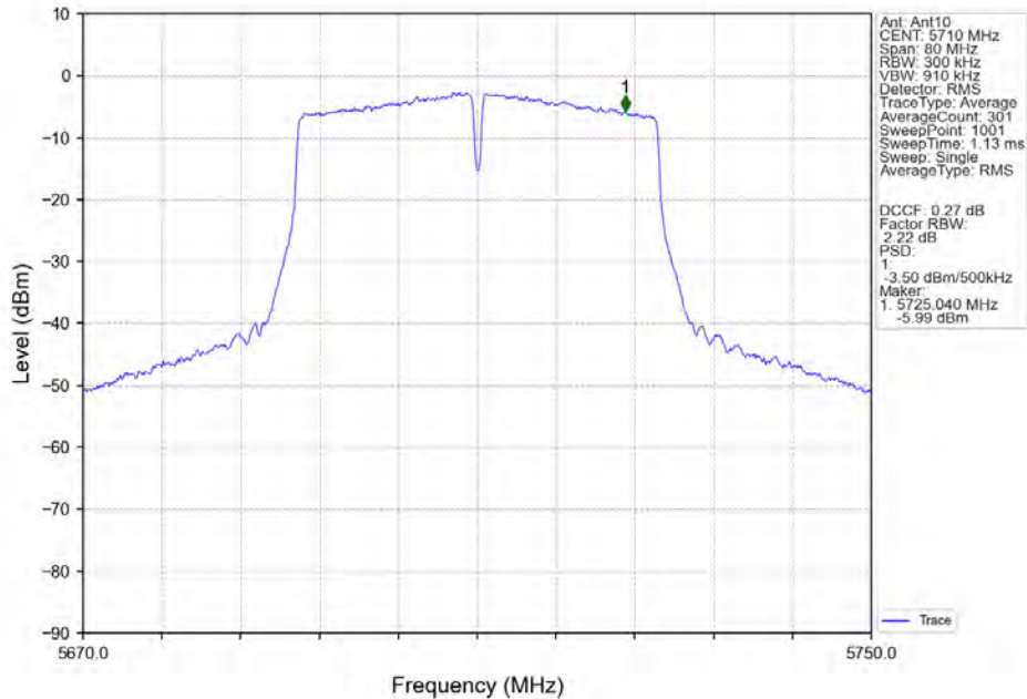
802.11ac(VHT40)_HCH_5710MHz_MIMO_NTNV
