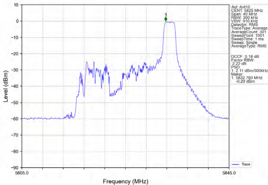
802.11ax(HEW20)_HCH_5825MHz_RU26_Right_Ant10_NTNV
