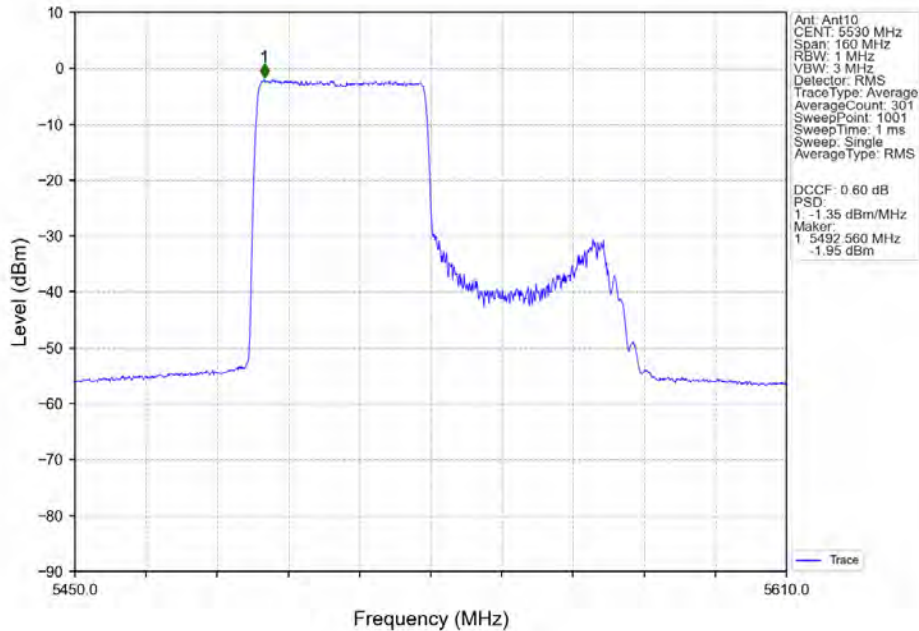
802.11ax(HEW80)_LCH_5530MHz_RU484_Left_MIMO_NTNV
