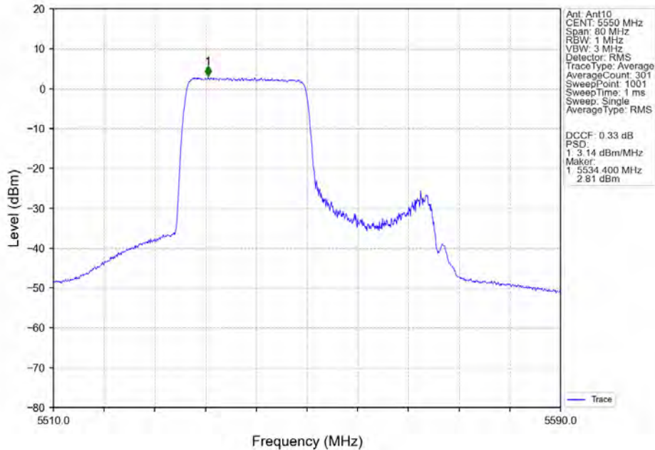
802.11ax(HEW40)_MCH_5550MHz_RU242_Left_MIMO_NTNV
