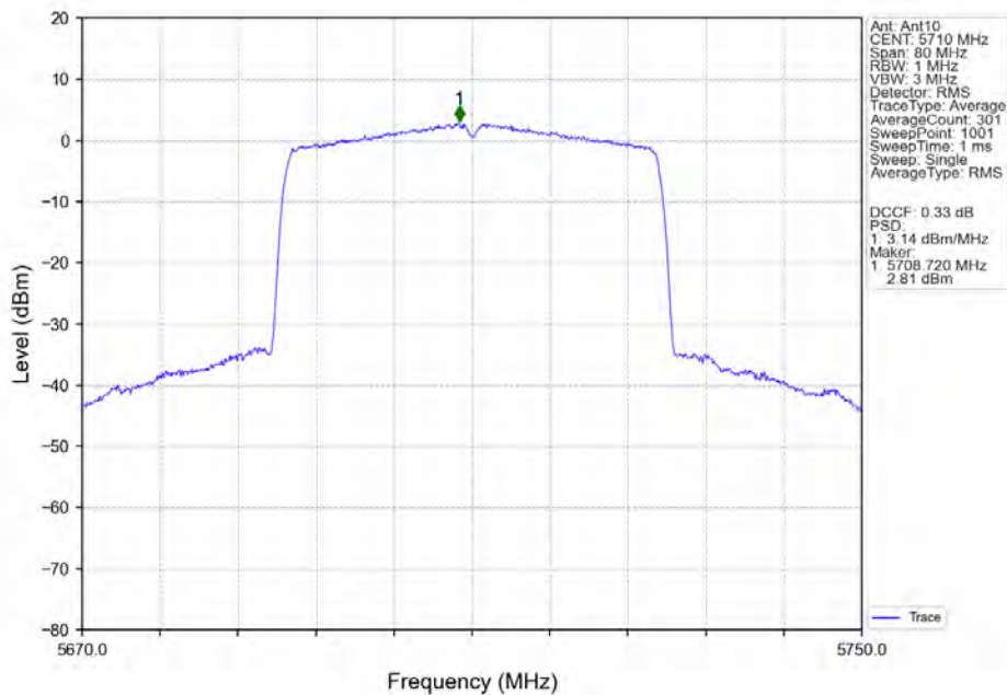
802.11ax(HEW40)_HCH_5710MHz_SU_/_Ant10_NTNV
