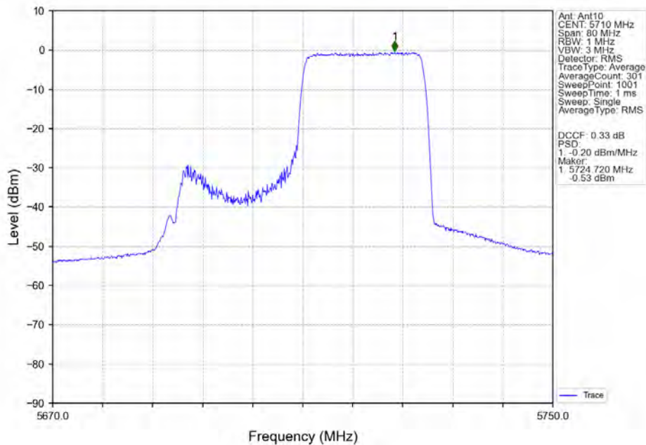
802.11ax(HEW40)_HCH_5710MHz_RU242_Right_MIMO_NTNV
