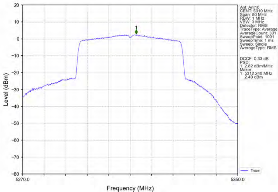
802.11ax(HEW40)_HCH_5310MHz_SU_/_Ant10_NTNV
