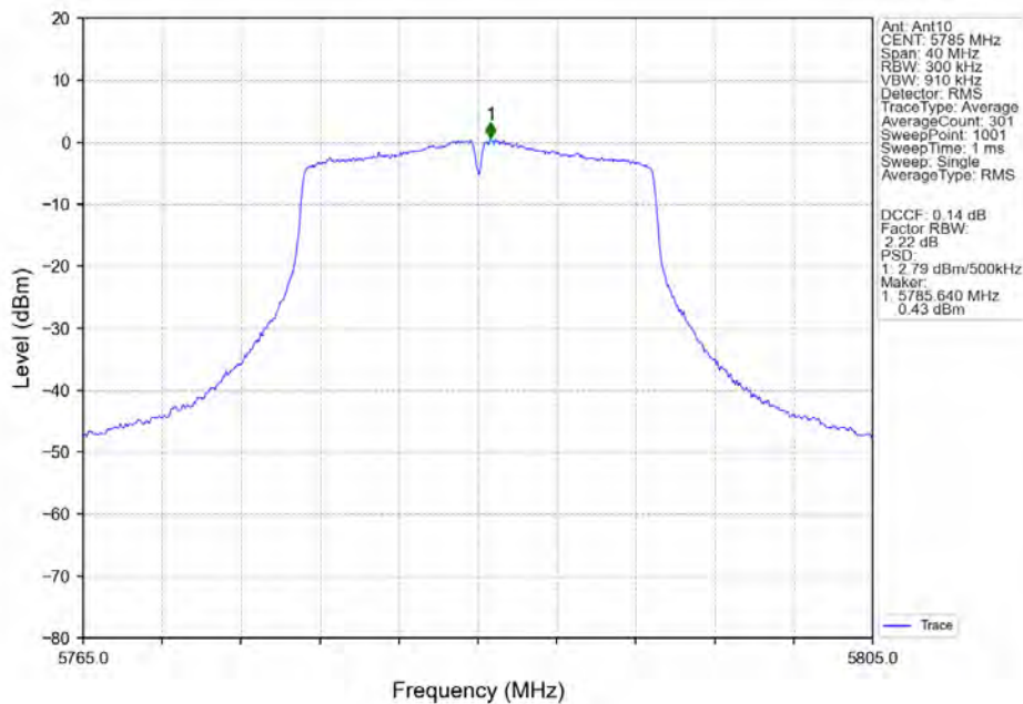
802.11ac(VHT20)_MCH_5785MHz_Ant10_NTNV
