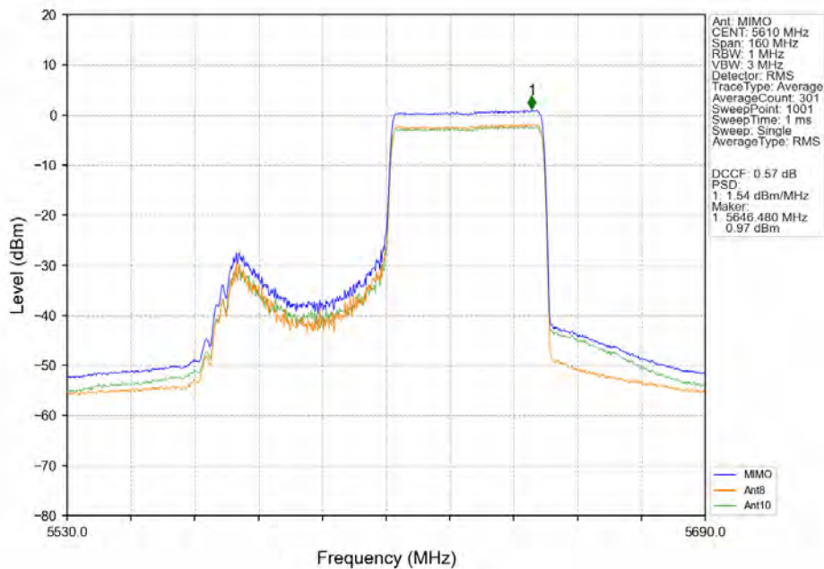
802.11ax(HEW80)_HCH_5610MHz_RU484_Right_MIMO_NTNV
