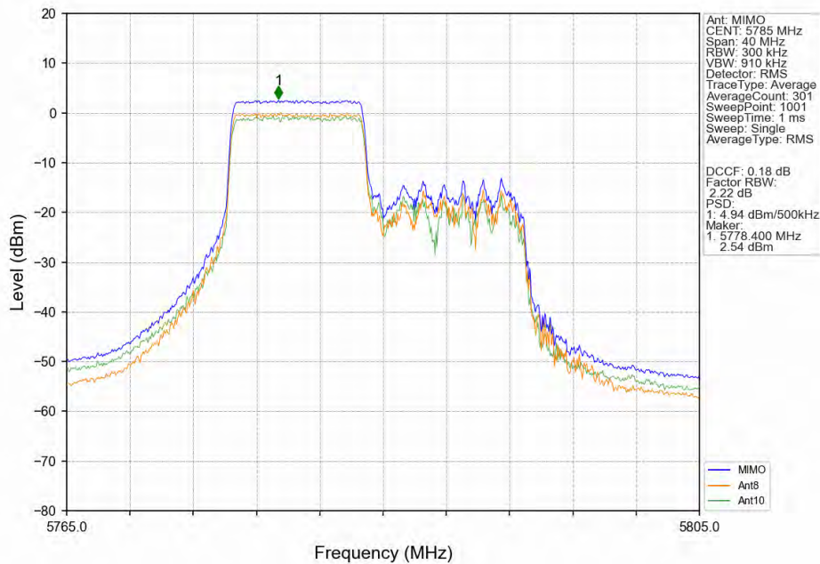
802.11ax(HEW20)_MCH_5785MHz_SU_/_Ant8_NTNV
