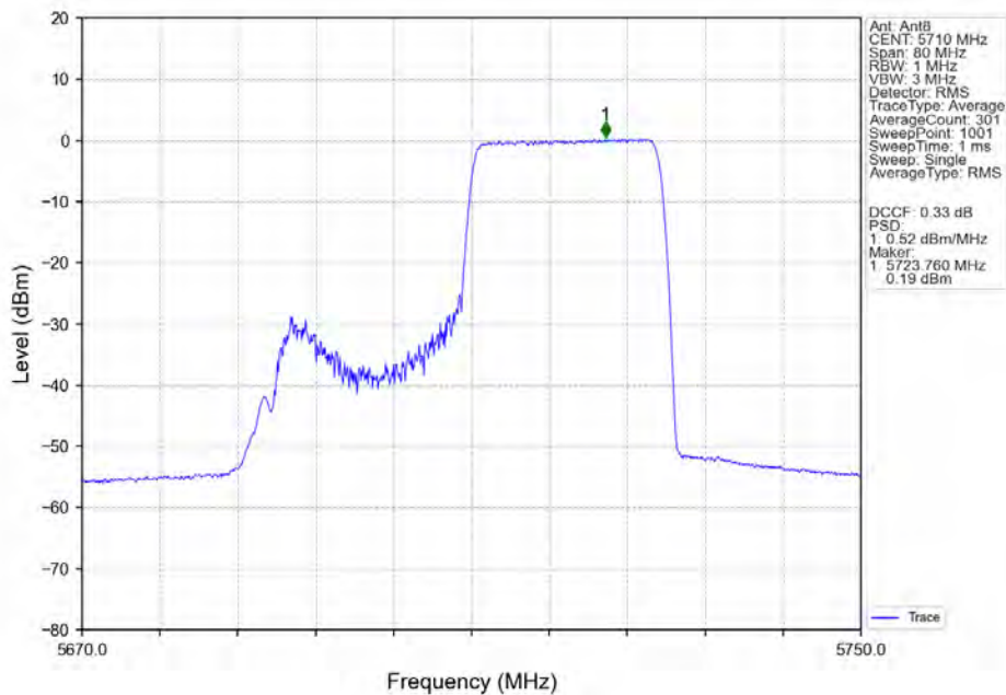
802.11ax(HEW40)_HCH_5710MHz_RU242_Right_Ant8_NTNV
