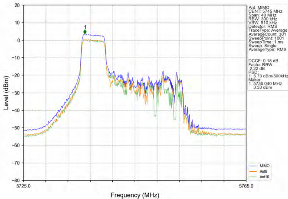
802.11ax(HEW20)_LCH_5745MHz_RU52_Left_MIMO_NTNV
