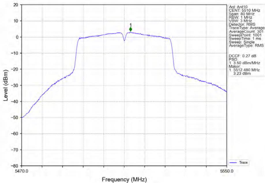
802.11ac(VHT40)_LCH_5510MHz_Ant10_NTNV
