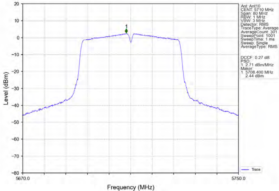
802.11ac(VHT40)_HCH_5710MHz_MIMO_NTNV
