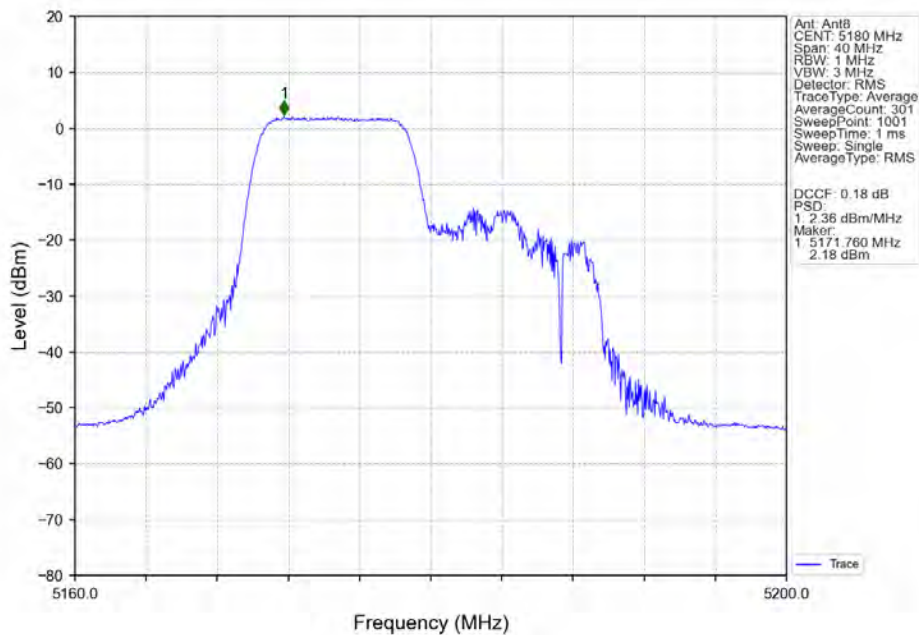
802.11ax(HEW20)_LCH_5180MHz_RU106_Left_Ant8_NTNV
