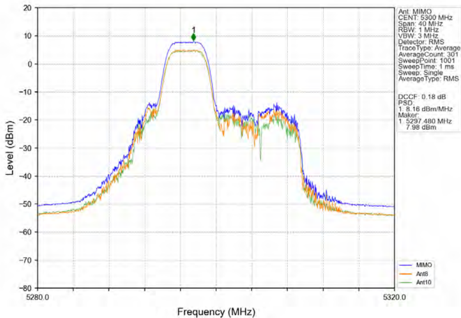
802.11ax(HEW20)_MCH_5300MHz_RU106_Left_Ant8_NTNV
