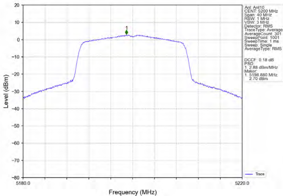
802.11ax(HEW20)_MCH_5200MHz_SU_/_Ant10_NTNV
