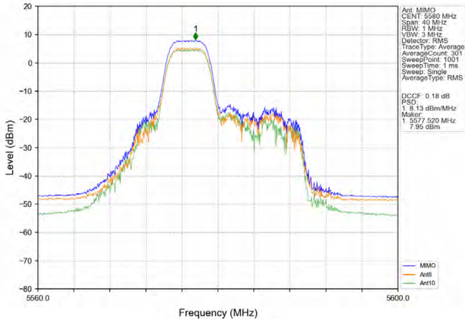
802.11ax(HEW20)_MCH_5580MHz_RU106_Left_Ant8_NTNV
