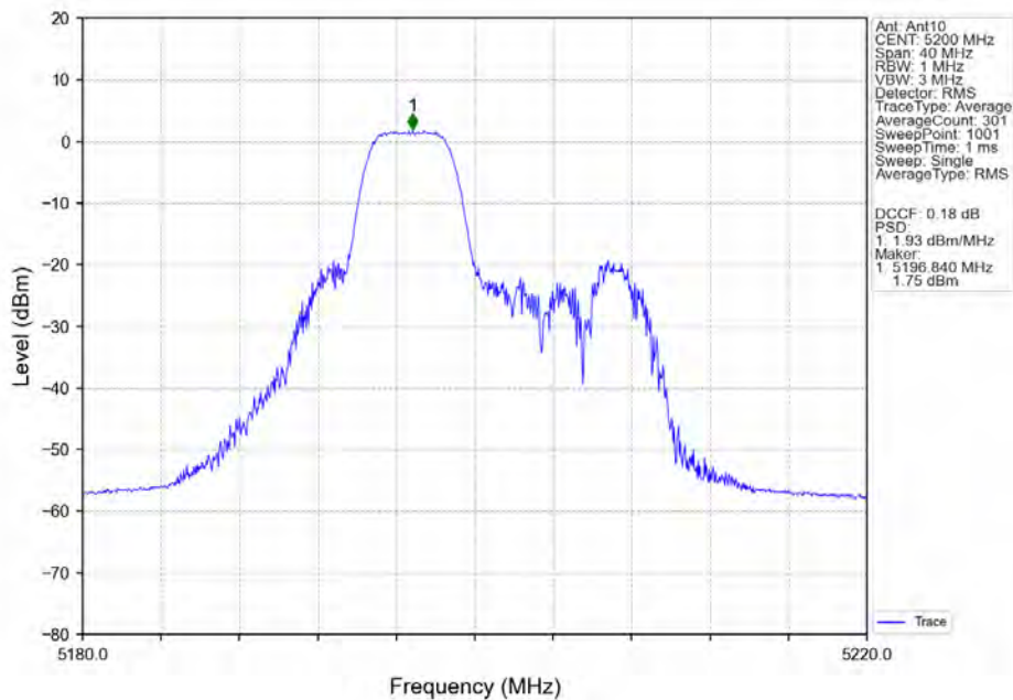
802.11ax(HEW20)_MCH_5200MHz_RU52_Mid_Ant10_NTNV
