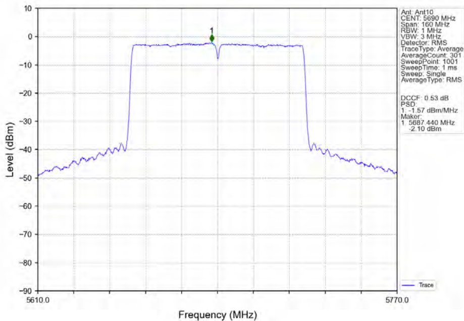
802.11ac(VHT80)_HCH_5690MHz_Ant10_NTNV
