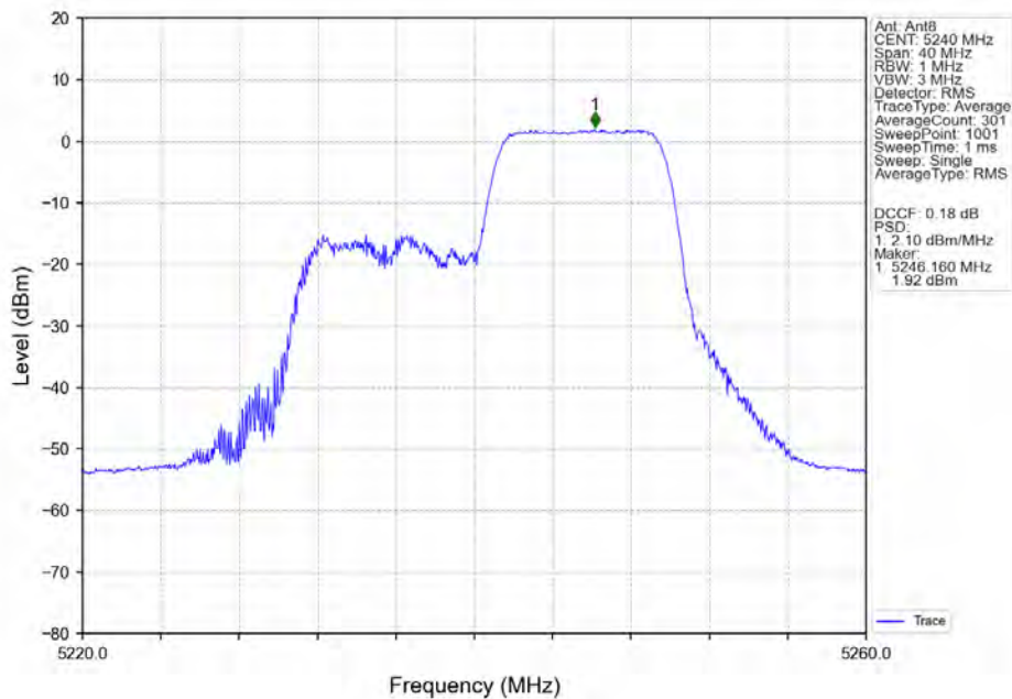
802.11ax(HEW20)_HCH_5240MHz_RU106_Right_Ant8_NTNV
