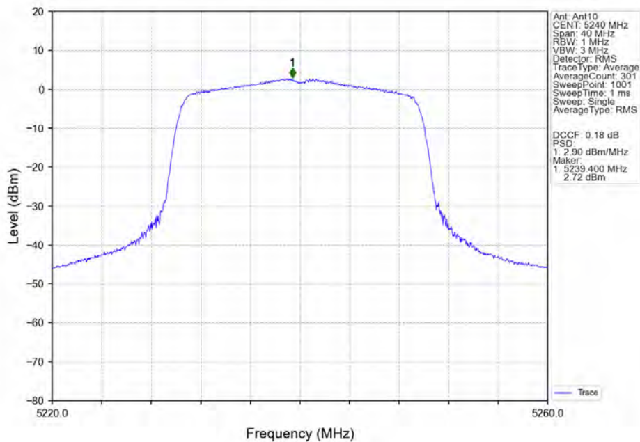
802.11ax(HEW20)_HCH_5240MHz_SU_/_Ant10_NTNV
