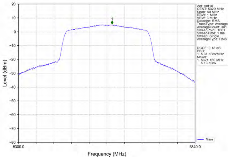
802.11ax(HEW20)_HCH_5320MHz_SU_ / _Ant10_NTNV
