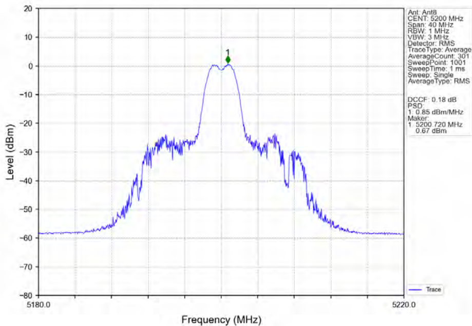
802.11ax(HEW20)_MCH_5200MHz_RU26_Mid_Ant8_NTNV
