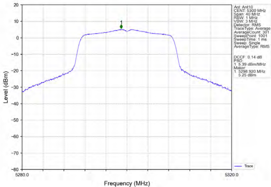
802.11ac(VHT20)_MCH_5300MHz_Ant10_NTNV
