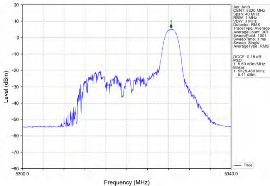
802.11ax(HEW20)_HCH_5320MHz_RU26_Right_Ant8_NTNV
