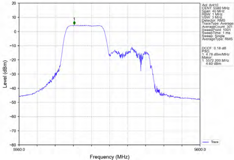
802.11ax(HEW20)_MCH_5580MHz_RU106_Left_MIMO_NTNV
