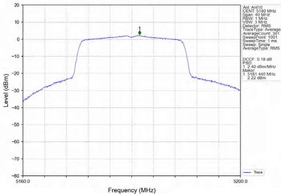
802.11ax(HEW20)_LCH_5180MHz_SU_/_Ant10_NTNV
