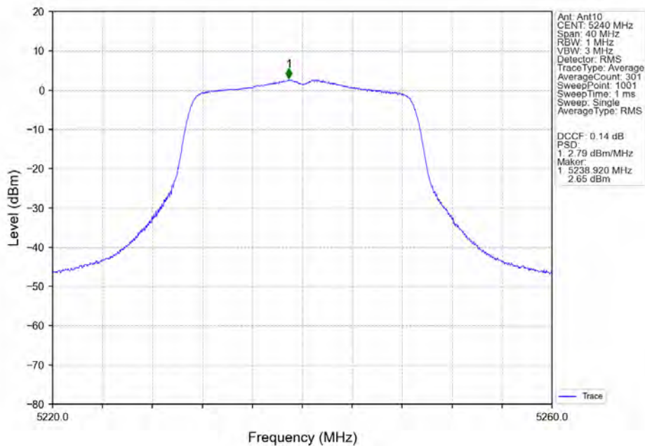
802.11ac(VHT20)_HCH_5240MHz_Ant10_NTNV
