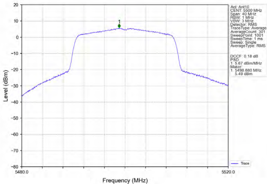
802.11ax(HEW20)_LCH_5500MHz_SU_/_Ant10_NTNV
