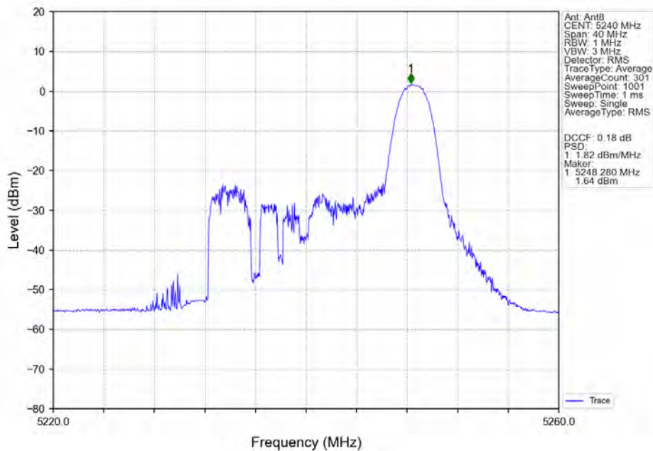
802.11ax(HEW20)_HCH_5240MHz_RU26_Right_Ant8_NTNV
