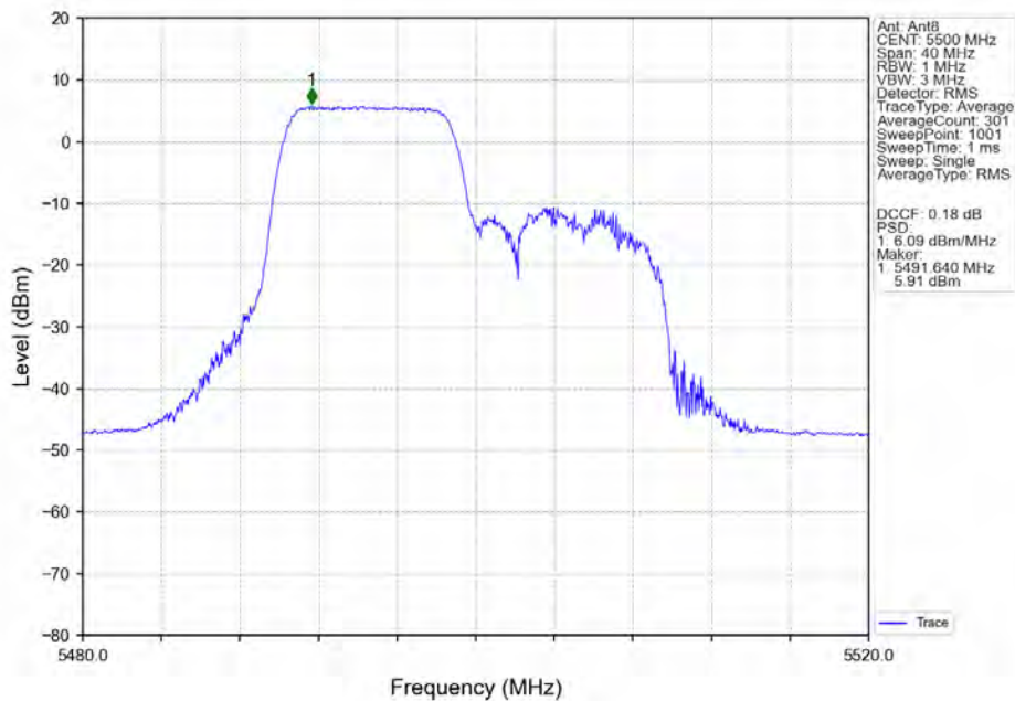
802.11ax(HEW20)_LCH_5500MHz_RU106_Left_Ant8_NTNV
