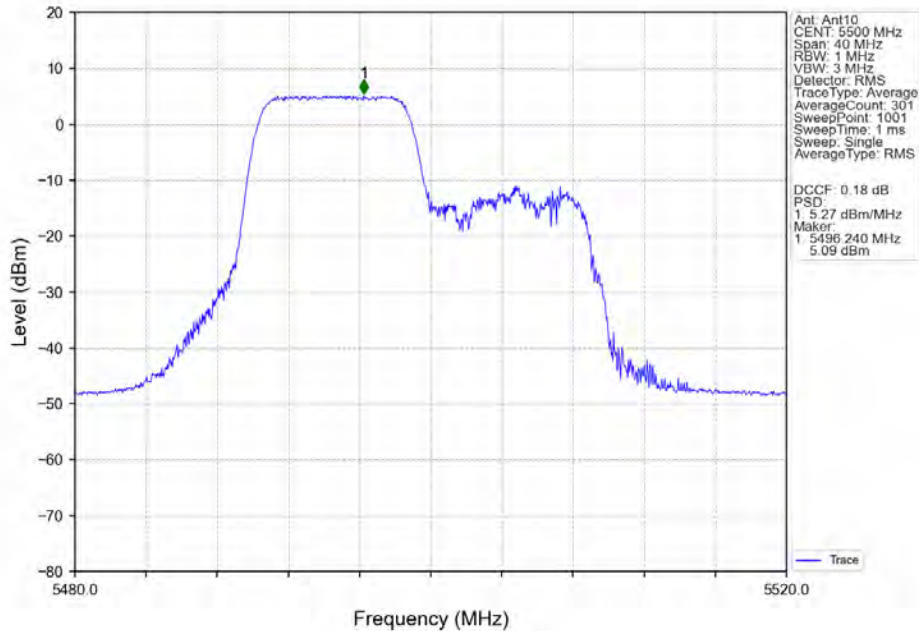
802.11ax(HEW20)_LCH_5500MHz_RU106_Left_MIMO_NTNV
