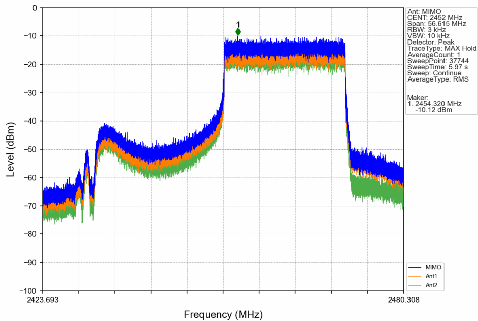
802.11ax(HEW40)_HCH_2452MHz_SU_/_Ant8 (MIMO)_NTNV
