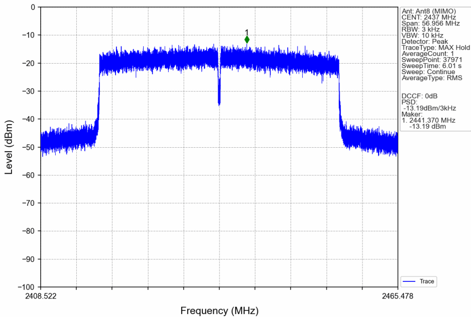
802.11ax(HEW40)_MCH_2437MHz_SU_/_Ant8 (MIMO)_NTNV
