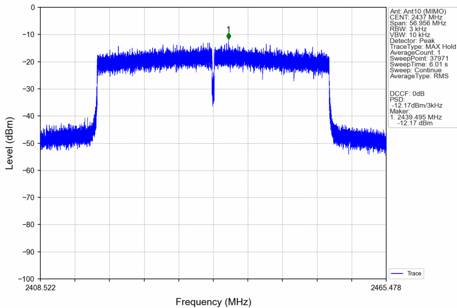
802.11ax(HEW40)_MCH_2437MHz_SU_/_MIMO_NTNV
