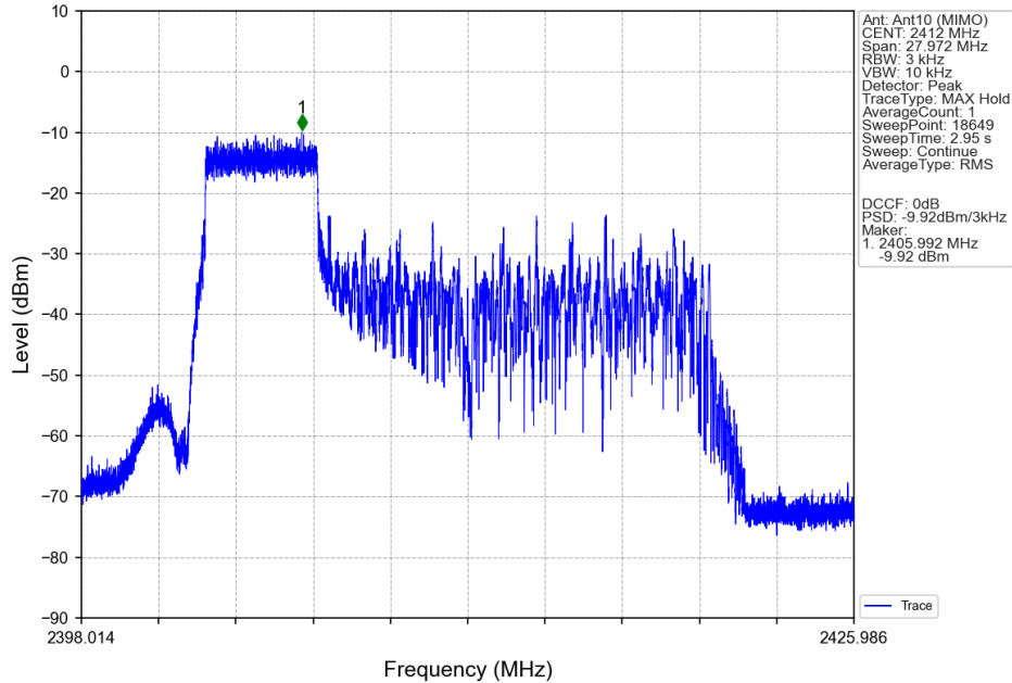
802.11ax(HEW20)_LCH_2412MHz_RU52_Left_MIMO_NTNV
