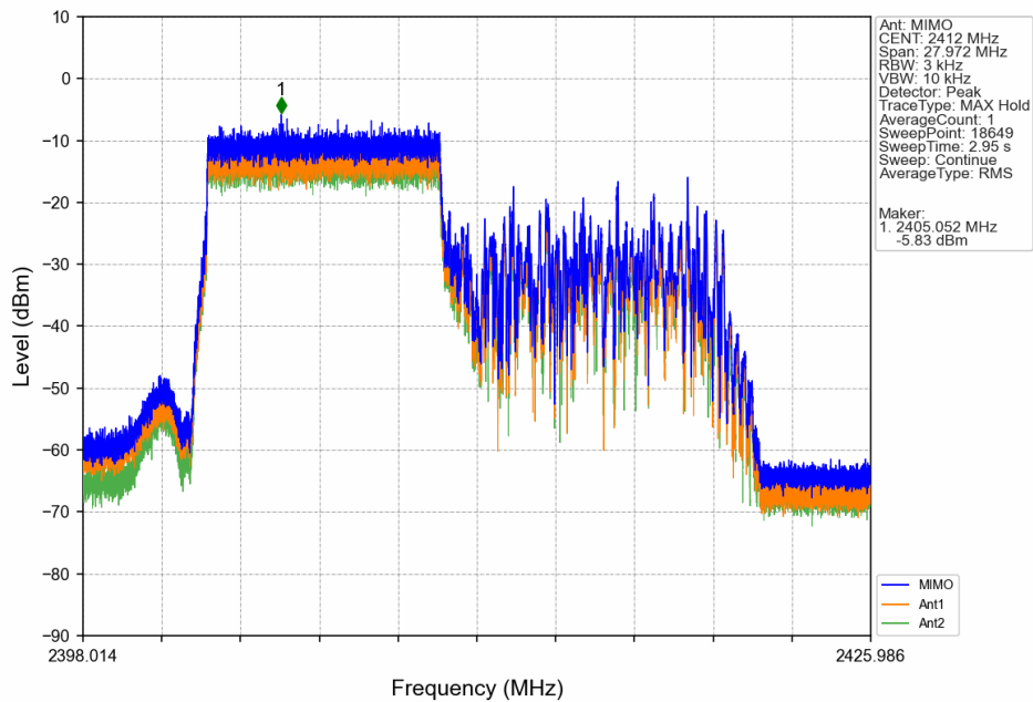
802.11ax(HEW20)_LCH_2412MHz_SU_/_Ant8 (MIMO)_NTNV
