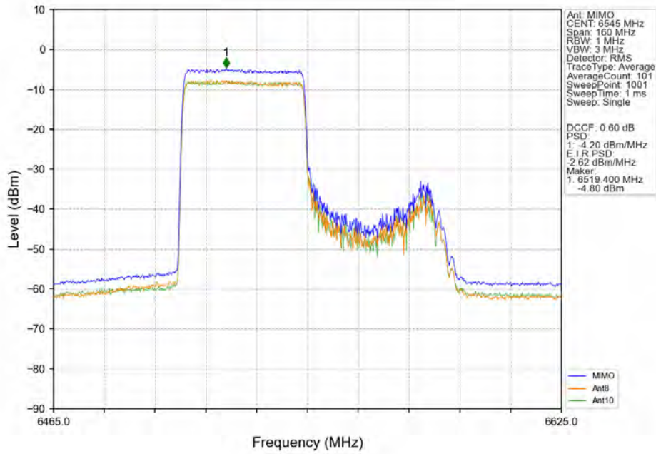
802.11ax(HEW80)_HCH_6545MHz_RU484_Right_Ant8_NTNV
