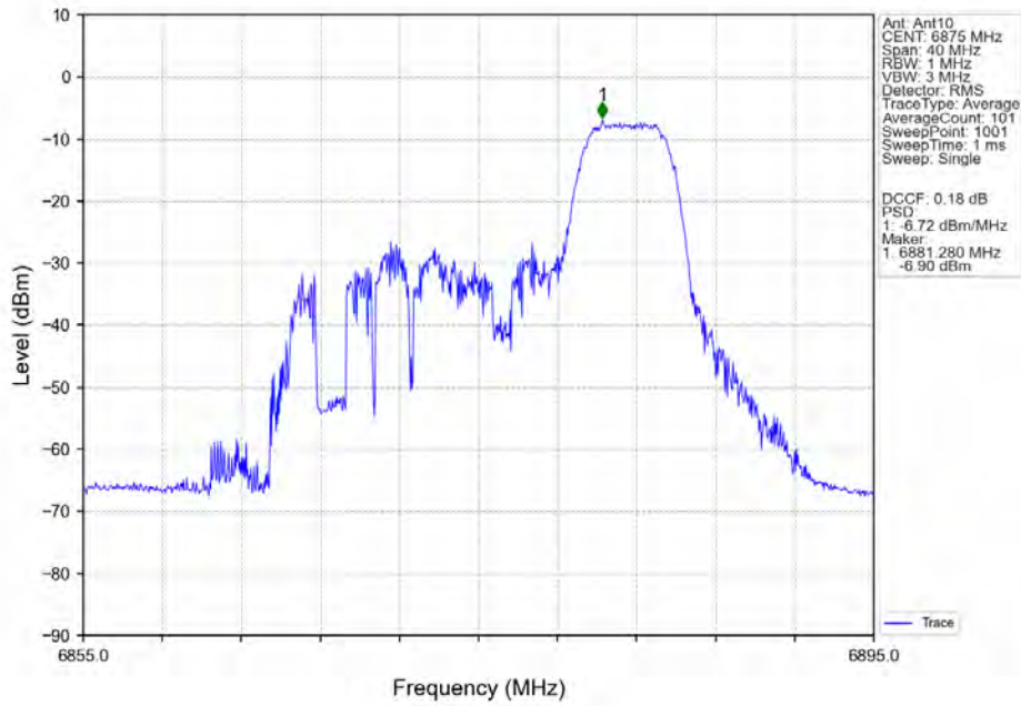
802.11ax(HEW20)_HCH_6875MHz_RU52_Right_MIMO_NTNV
