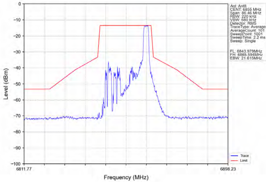
802.11ax(HEW20)_HCH_6855MHz_RU52_Right_Ant8_NTNV
