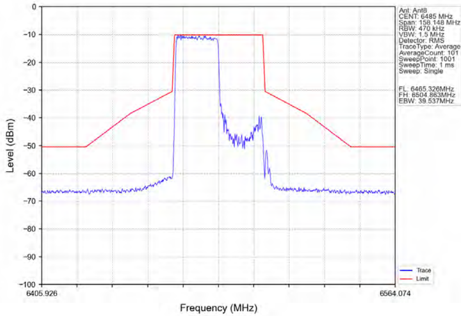
802.11ax(HEW40)_MCH_6485MHz_SU / Ant8_NTNV
