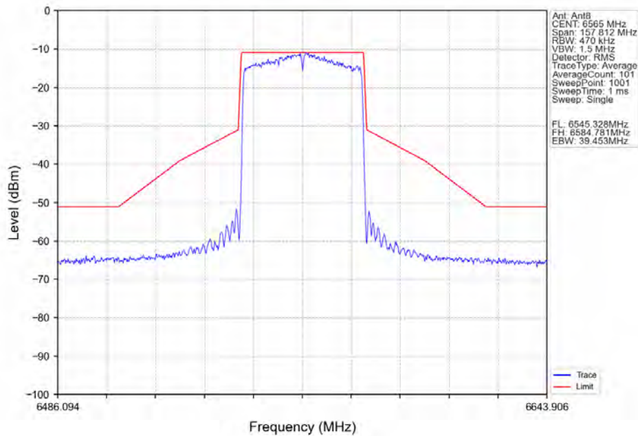
802.11ax(HEW40)_LCH_6565MHz_SU / Ant8_NTNV
