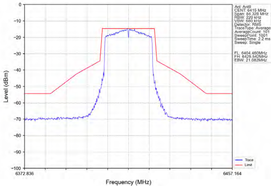
802.11ax(HEW20)_HCH_6415MHz_SU / Ant8_NTNV
