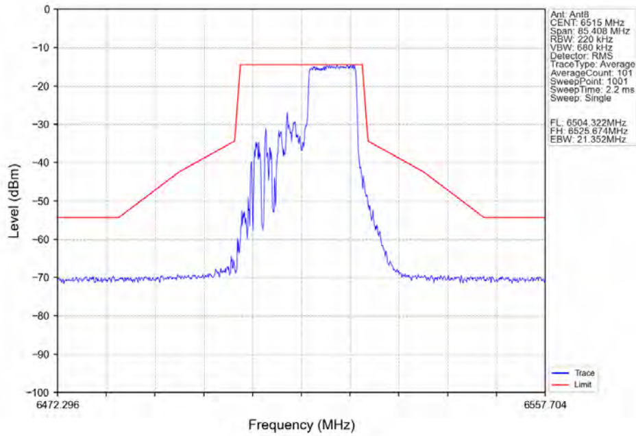
802.11ax(HEW20)_HCH_6515MHz_SU / Ant8_NTNV
