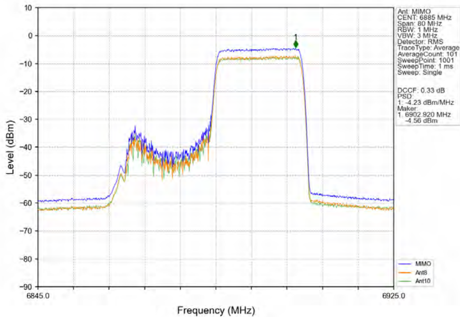
802.11ax(HEW40)_HCH_6885MHz_RU242_Right_MIMO_NTNV
