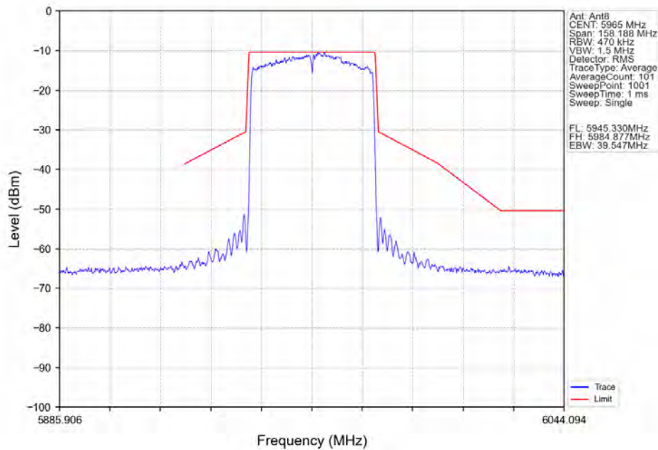
802.11ax(HEW40)_LCH_5965MHz_SU / Ant8_NTNV
