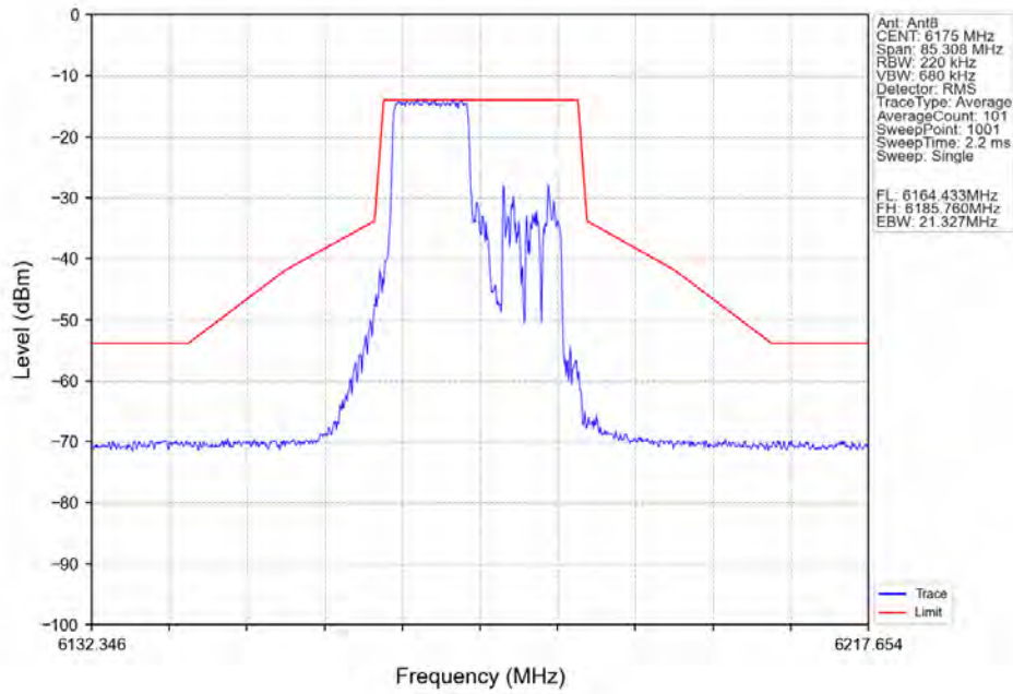
802.11ax(HEW20)_MCH_6175MHz_SU / Ant8_NTNV
