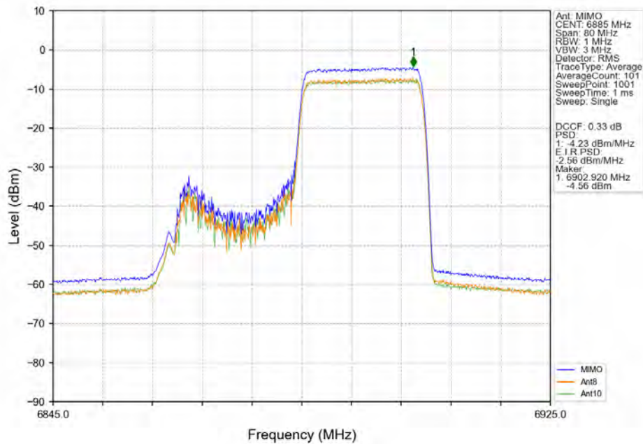
802.11ax(HEW40)_HCH_6885MHz_RU242_Right MIMO NTN
