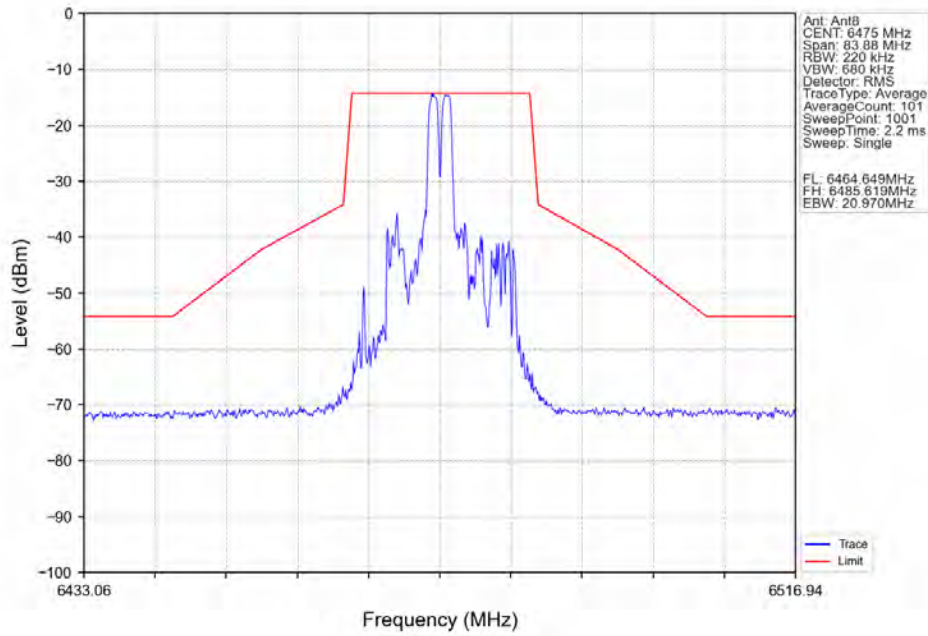
802.11ax(HEW20)_MCH_6475MHz_RU52_Mid_Ant8_NTNV
