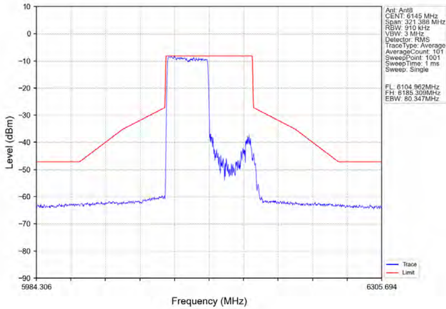
802.11ax(HEW80)_MCH_6145MHz_SU / Ant8_NTNV
