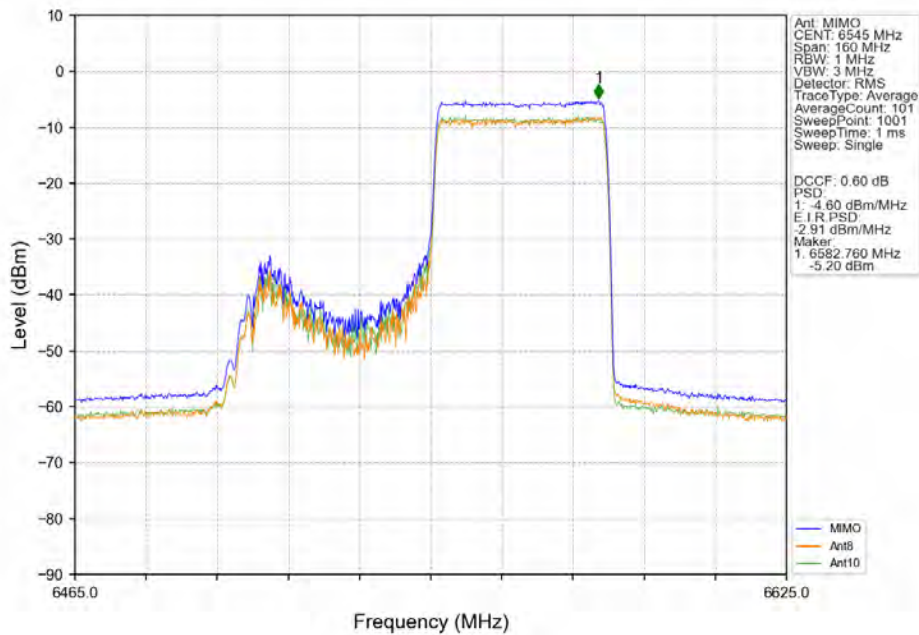
802.11ax(HEW80)_HCH_6545MHz_RU484_Right_MIMO_NTNV
