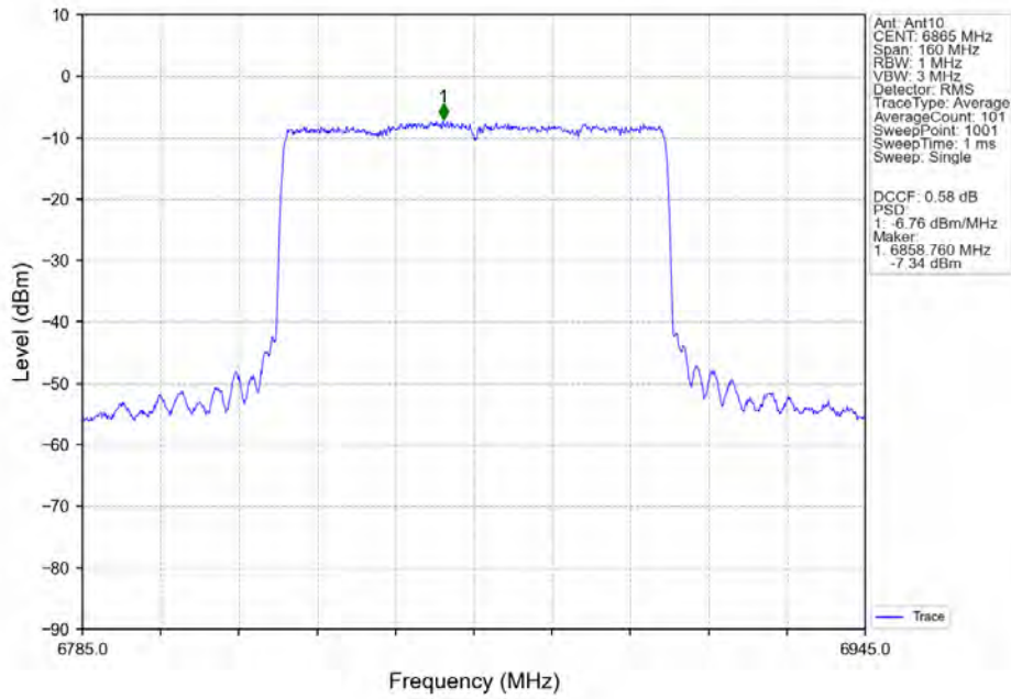
802.11ax(HEW80)_HCH_6865MHz_SU_/_MIMO_NTNV
