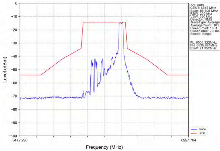
802.11ax(HEW20)_HCH_6515MHz_RU52_Right_Ant8_NTNV
