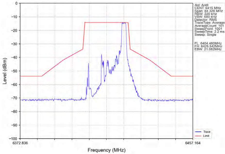
802.11ax(HEW20)_HCH_6415MHz_RU52_Right_Ant8_NTNV
