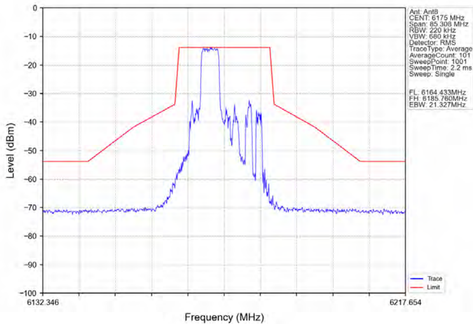
802.11ax(HEW20)_MCH_6175MHz_RU52_Mid_Ant8_NTNV
