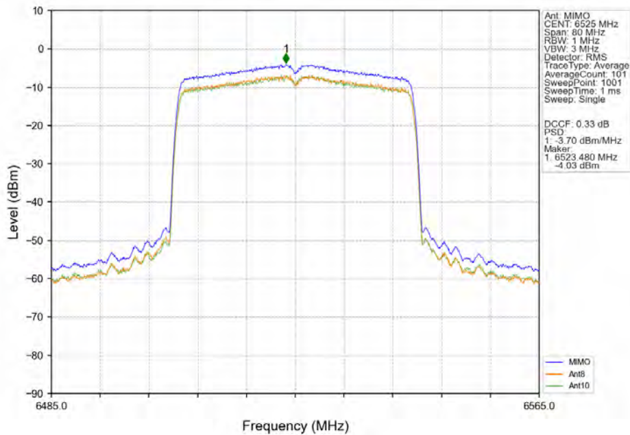
802.11ax(HEW40)_HCH_6525MHz_SU_/_MIMO_NTNV
