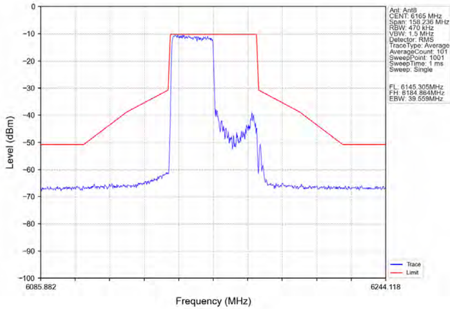
802.11ax(HEW40)_MCH_6165MHz_SU / Ant8_NTNV
