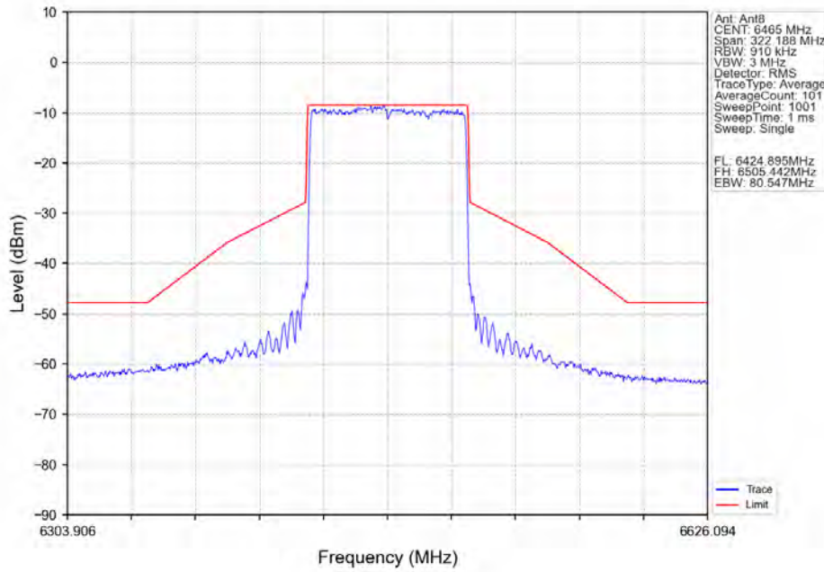
802.11ax(HEW80)_LCH_6465MHz_SU_/_Ant8_NTNV
