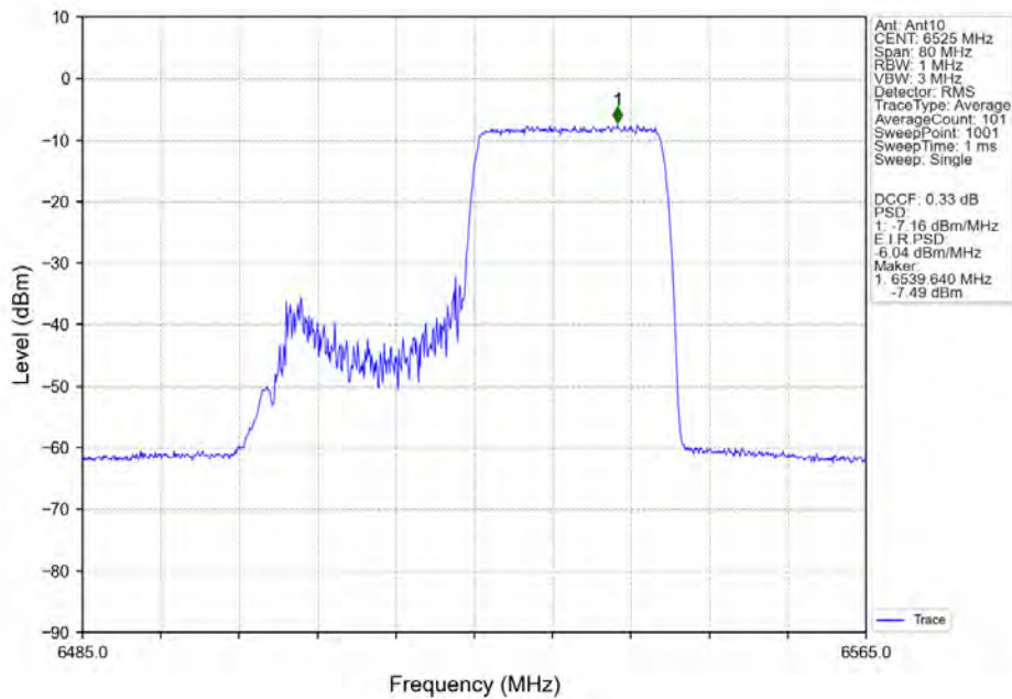
802.11ax(HEW40)_HCH_6525MHz_RU242_Right_Ant10_NTNV
