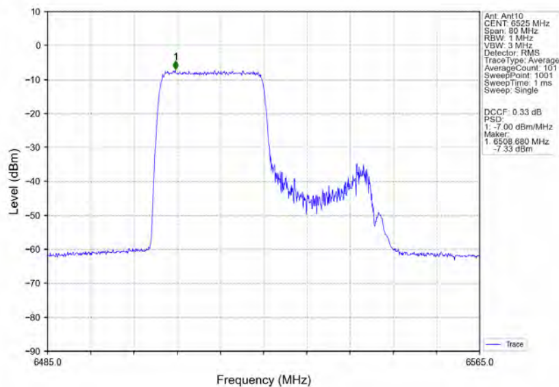
802.11ax(HEW40) HCH 6525MHz RU242 Left Ant10 NTN
