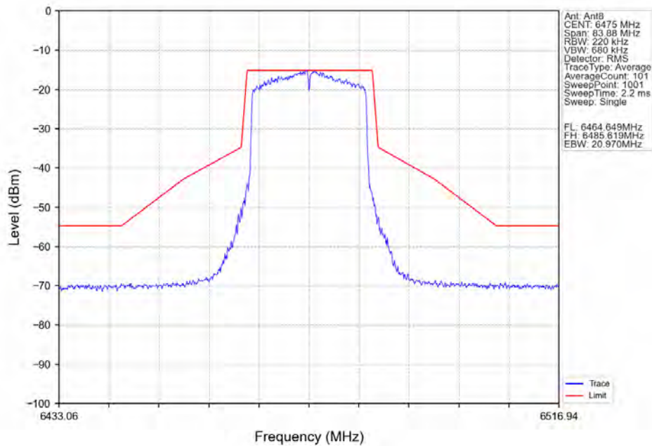
802.11ax(HEW20)_MCH_6475MHz_SU / Ant8_NTNV
