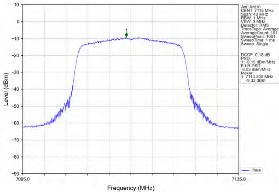
802.11ax(HEW20)_HCH_7115MHz_SU / _Ant10_NTNV
