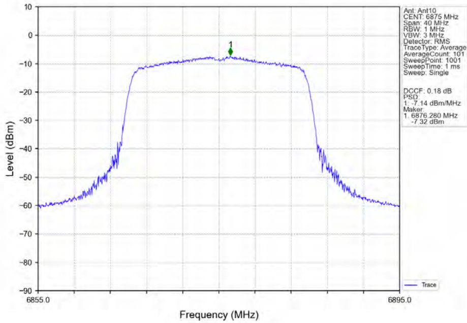
802.11ax(HEW20)_HCH_6875MHz_SU_/_MIMO_NTNV
