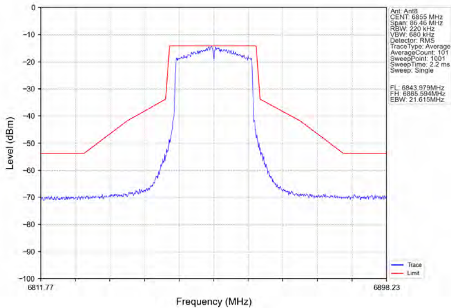
802.11ax(HEW20)_HCH_6855MHz_SU / Ant8_NTNV
