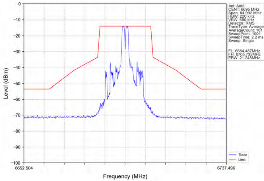
802.11ax(HEW20)_MCH_6695MHz_RU52_Mid_Ant8_NTNV
