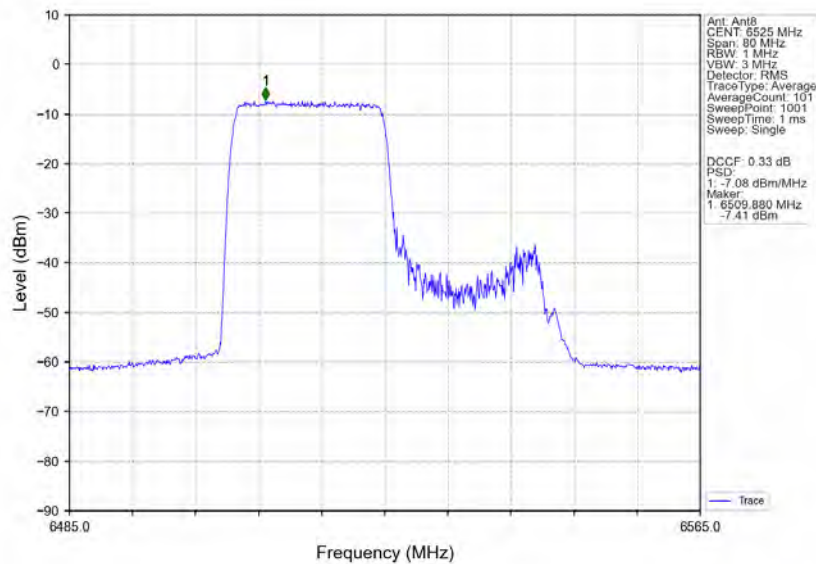
802.11ax(HEW40) HCH 6525MHz RU242 Left Ant8 NTN
