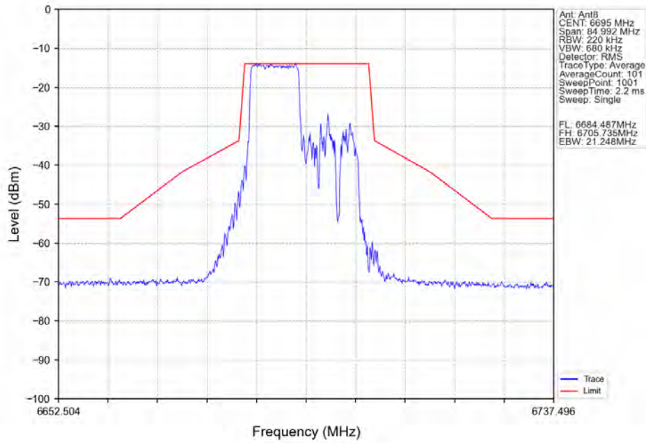
802.11ax(HEW20)_MCH_6695MHz_SU / Ant8_NTNV
