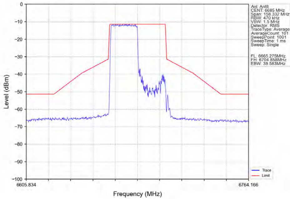
802.11ax(HEW40)_MCH_6685MHz_SU / Ant8_NTNV
