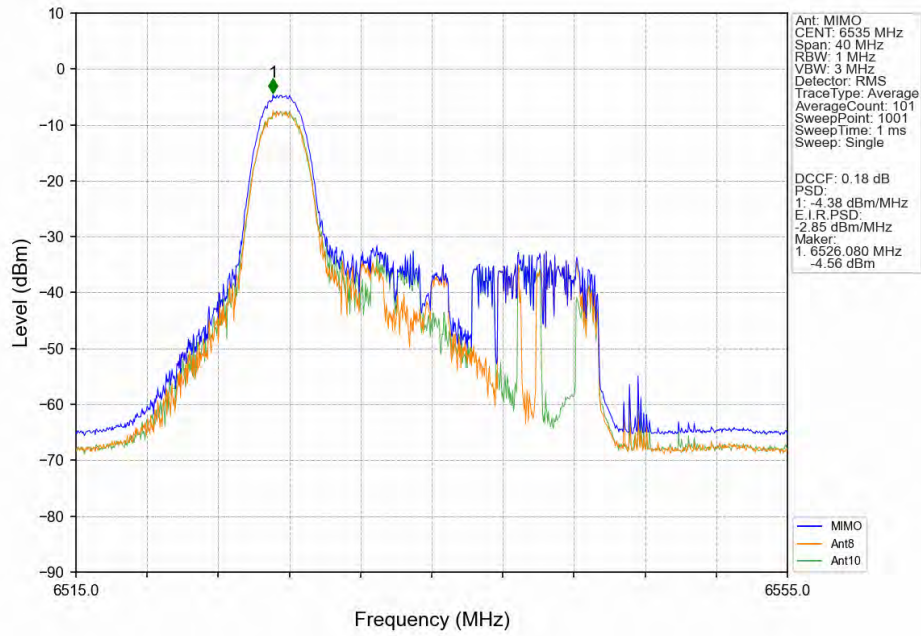
802.11ax(HEW20)_LCH_6535MHz_RU52_Left_Ant8_NTNV
