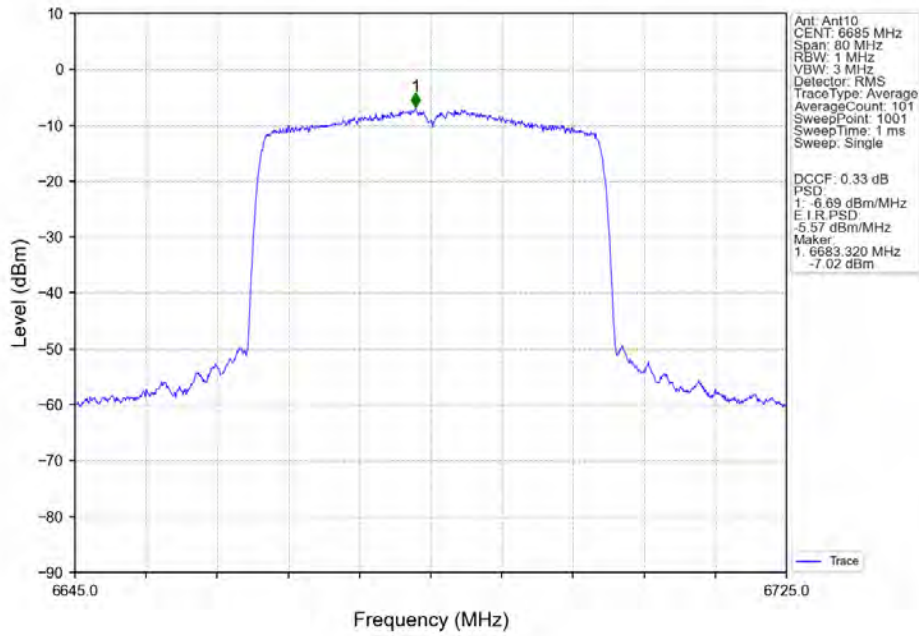
802.11ax(HEW40)_MCH_6685MHz_SU_/_MIMO NTN
