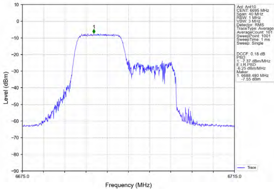
802.11ax(HEW20)_MCH_6695MHz_RU106_Left_Ant10_NTNV
