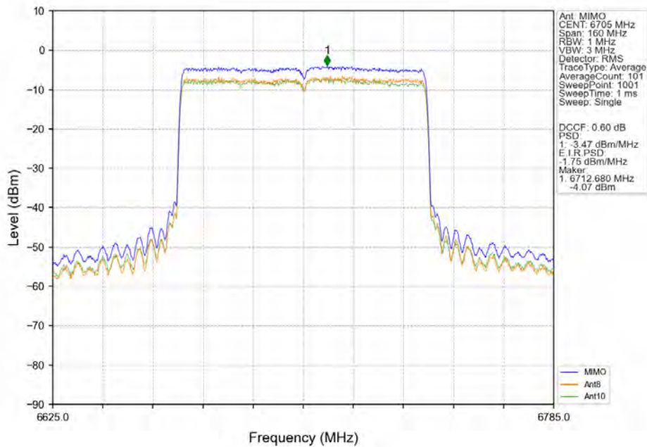
802.11ax(HEW80)_MCH_6705MHz_SU_/_MIMO NTN
