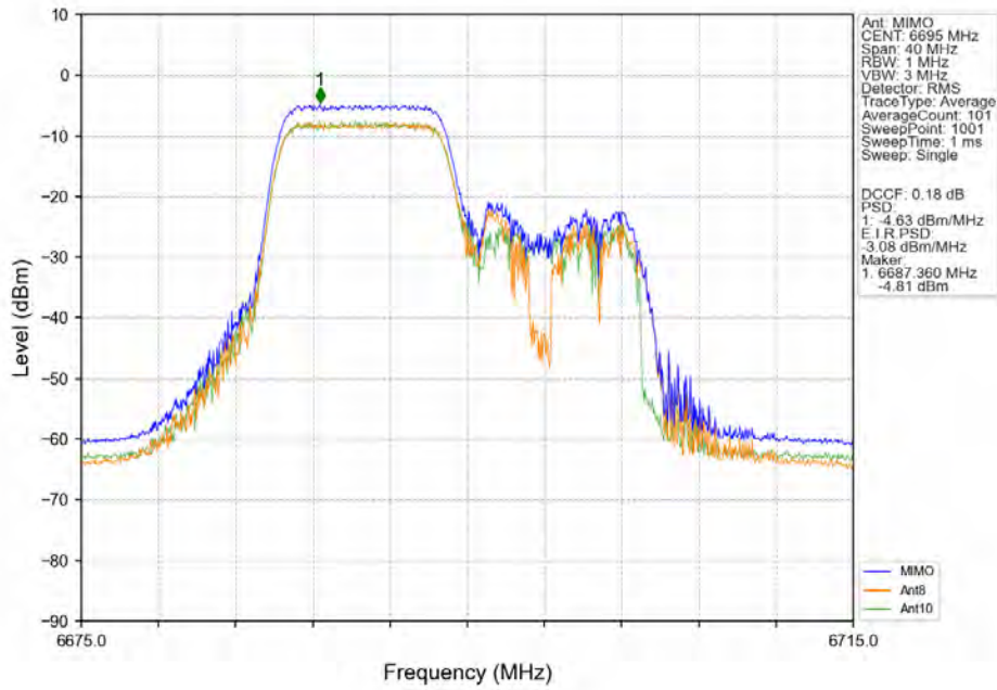
802.11ax(HEW20)_MCH_6695MHz_SU / Ant8 NTN
