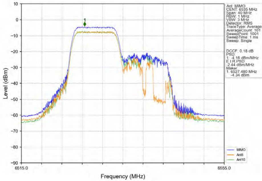
802.11ax(HEW20)_LCH_6535MHz_SU / Ant8 NTN
