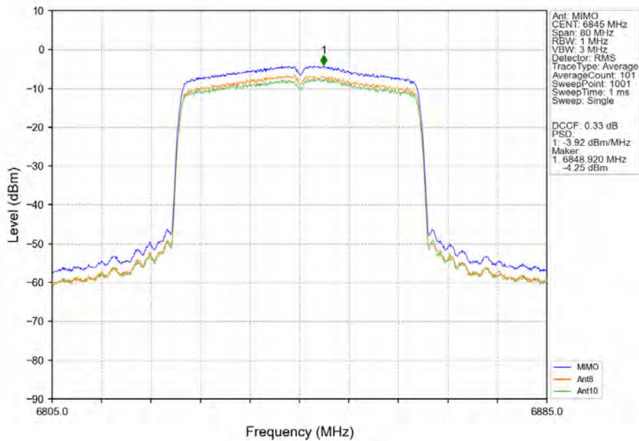
802.11ax(HEW40)_HCH_6845MHz_SU_/_MIMO_NTNV
