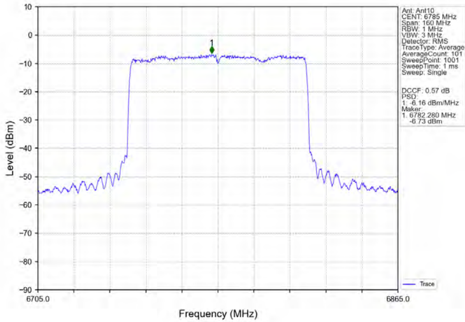
802.11ax(HEW80)_HCH_6785MHz_SU_/_MIMO_NTNV
