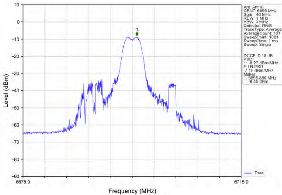
802.11ax(HEW20)_MCH_6695MHz_RU26_Mid_Ant10_NTNV
