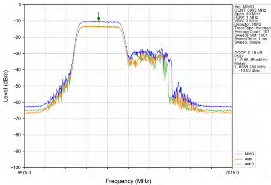
802.11ax(HEW20)_MCH_6995MHz_RU106_Left_MIMO_NTNV
