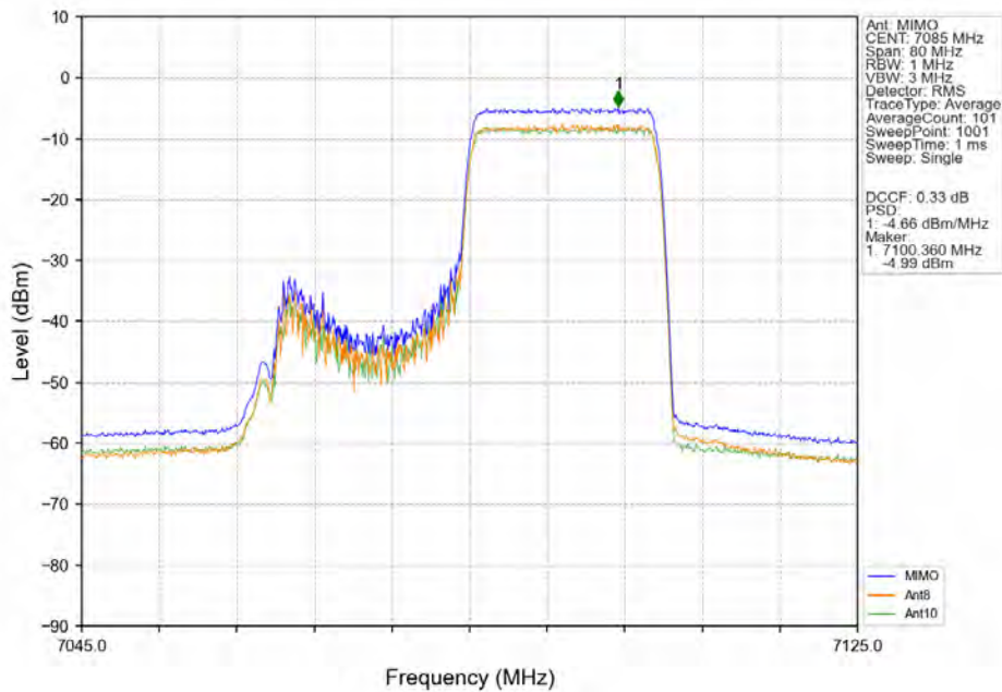
802.11ax(HEW40)_HCH_7085MHz_RU242_Right_MIMO_NTNV
