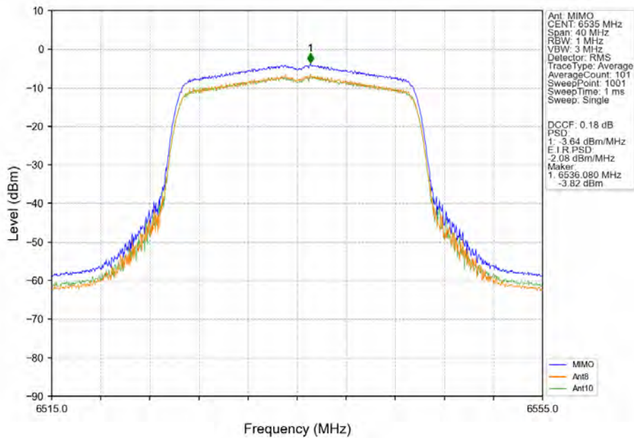
802.11ax(HEW20)_LCH_6535MHz_SU_/_MIMO_NTNV
