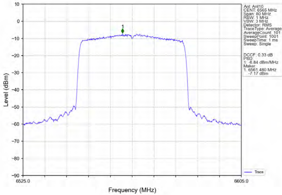
802.11ax(HEW40)_LCH_6565MHz_SU_/_MIMO NTN
