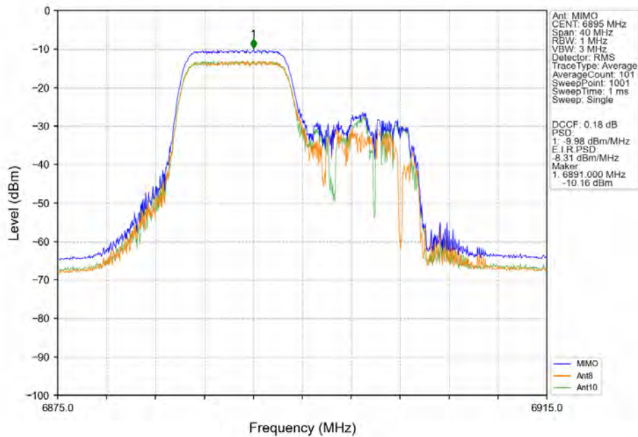
802.11ax(HEW20)_LCH_6895MHz_RU106_Left MIMO NTN
