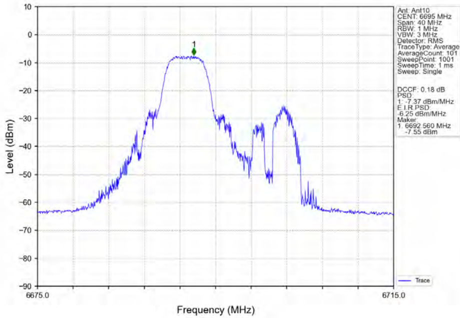
802.11ax(HEW20)_MCH_6695MHz_RU52_Mid MIMO NTN
