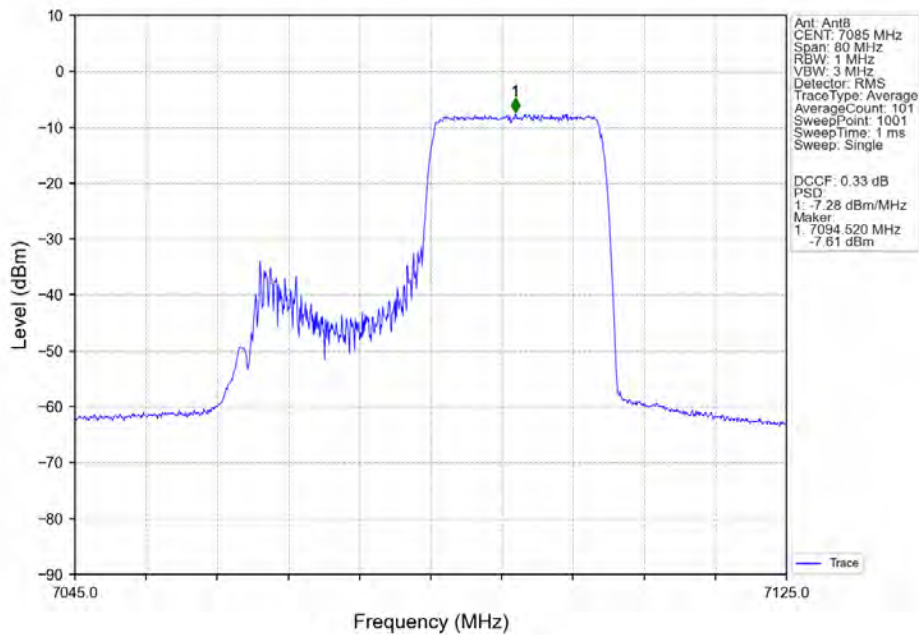
802.11ax(HEW40) HCH 7085MHz RU242 Right Ant8 NTN
