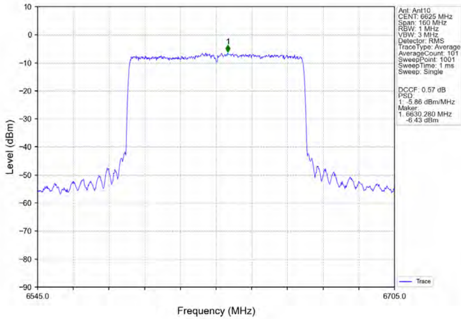
802.11ax(HEW80)_LCH_6625MHz_SU_/_MIMO NTN
