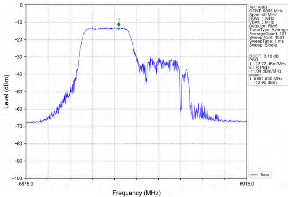
802.11ax(HEW20)_LCH_6895MHz_RU106_Left_Ant8_NTNV
