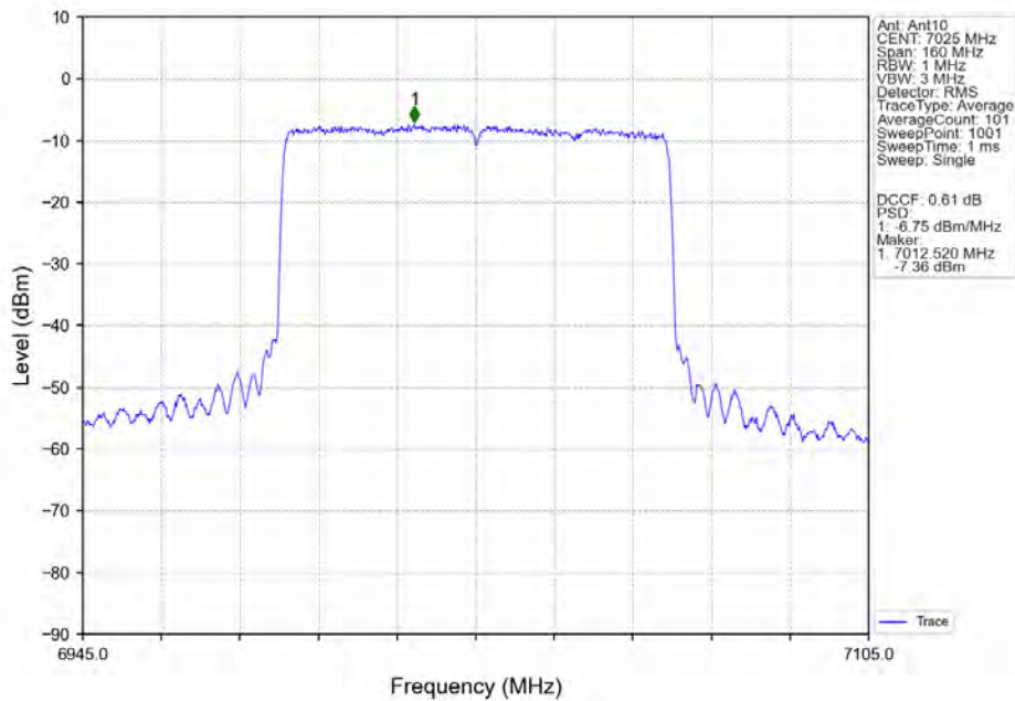
802.11ax(HEW80)_HCH_7025MHz_SU / Ant10_NTNV
