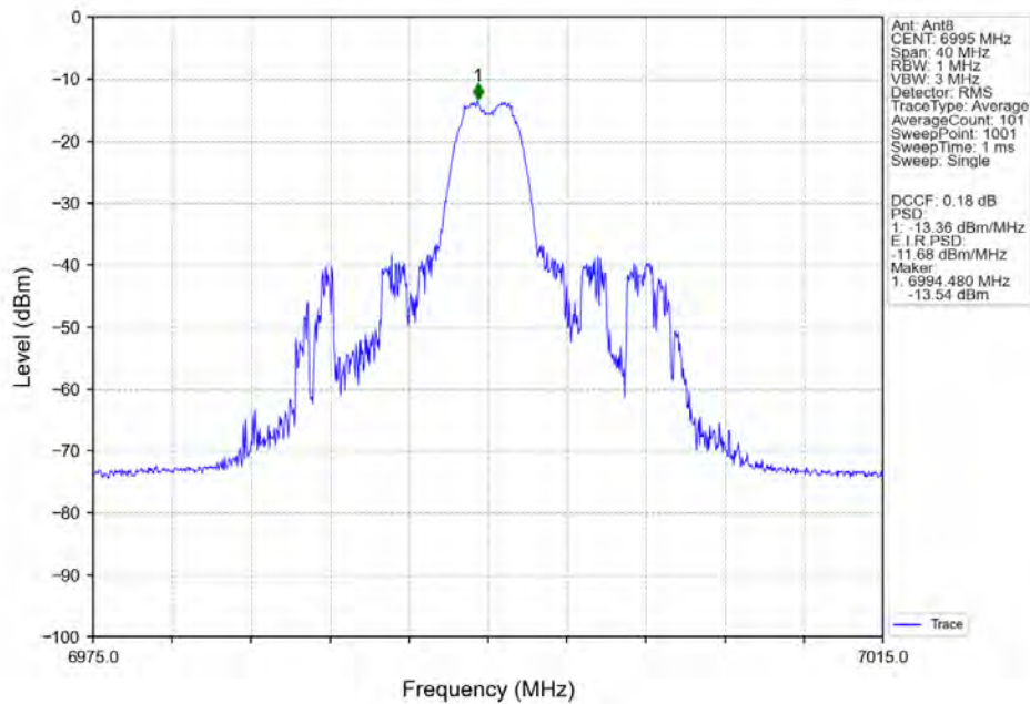
802.11ax(HEW20) MCH 6995MHz RU26 Mid Ant8 NTN
