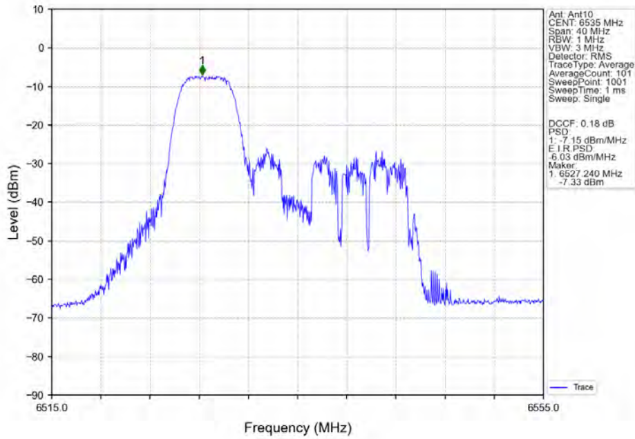
802.11ax(HEW20)_LCH_6535MHz_RU52_Left_MIMO_NTNV
