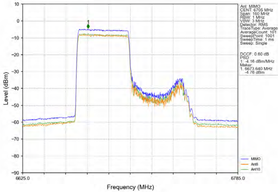
802.11ax(HEW80)_MCH_6705MHz_SU / Ant8 NTN
