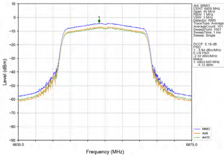
802.11ax(HEW20)_HCH_6855MHz_SU_/_MIMO_NTNV
