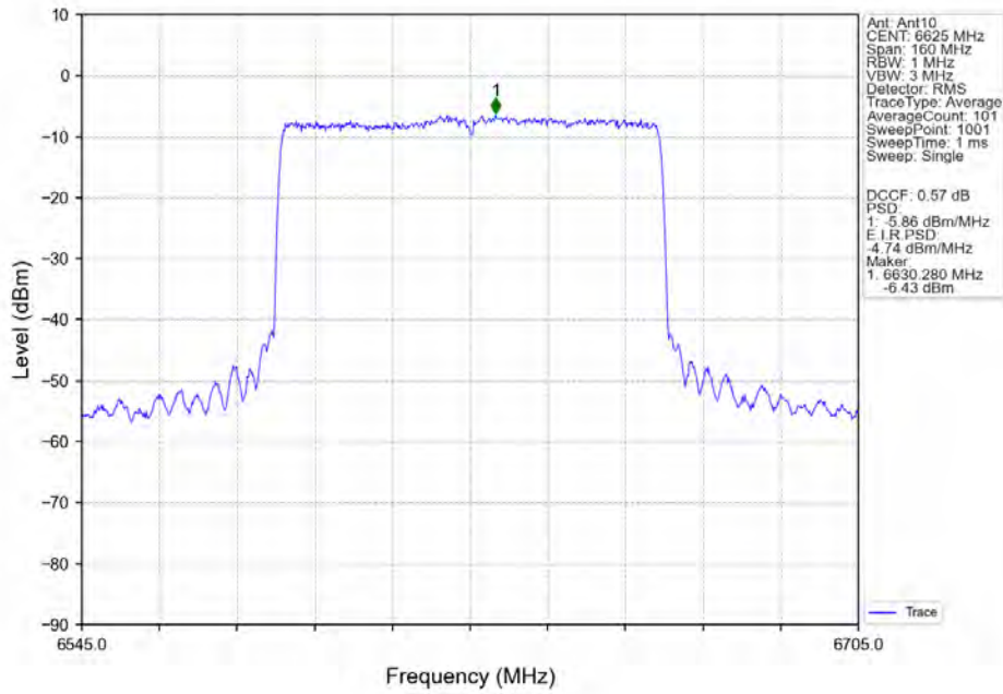
802.11ax(HEW80)_LCH_6625MHz_SU_/_MIMO_NTNV
