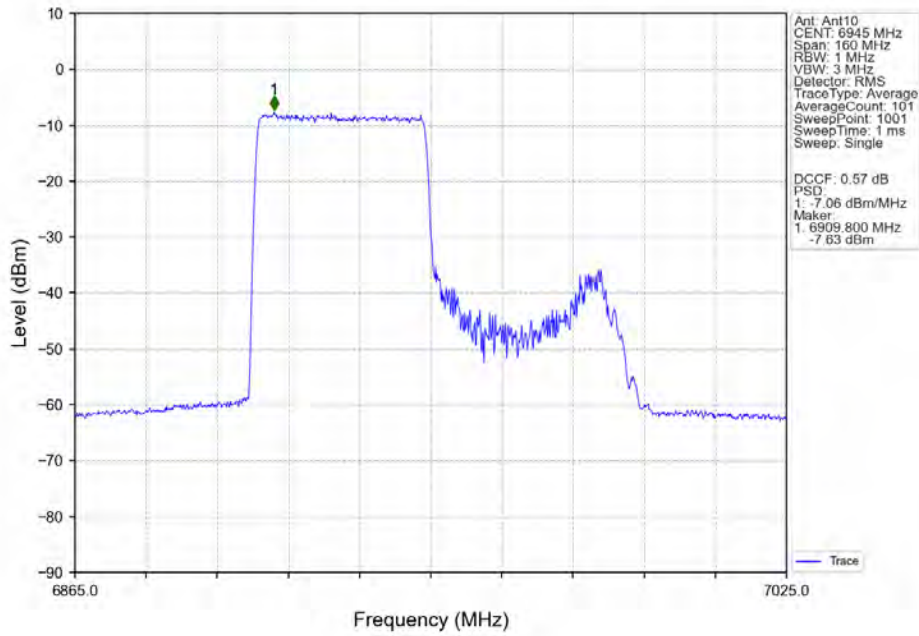
802.11ax(HEW80)_LCH_6945MHz_RU484_Left MIMO NTN
