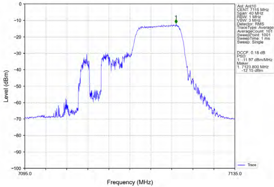
802.11ax(HEW20) HCH 7115MHz RU106 Right MIMO NTN
