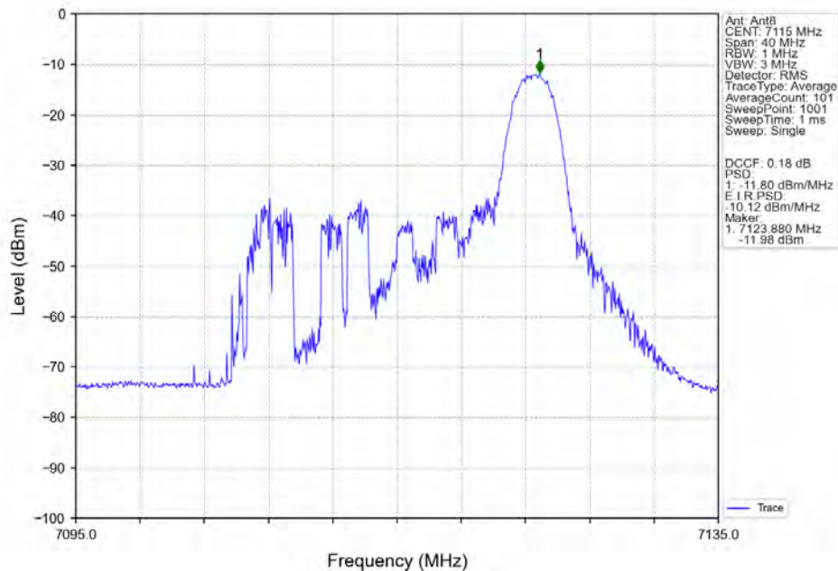
802.11ax(HEW20) HCH 7115MHz RU26 Right Ant8 NTN
