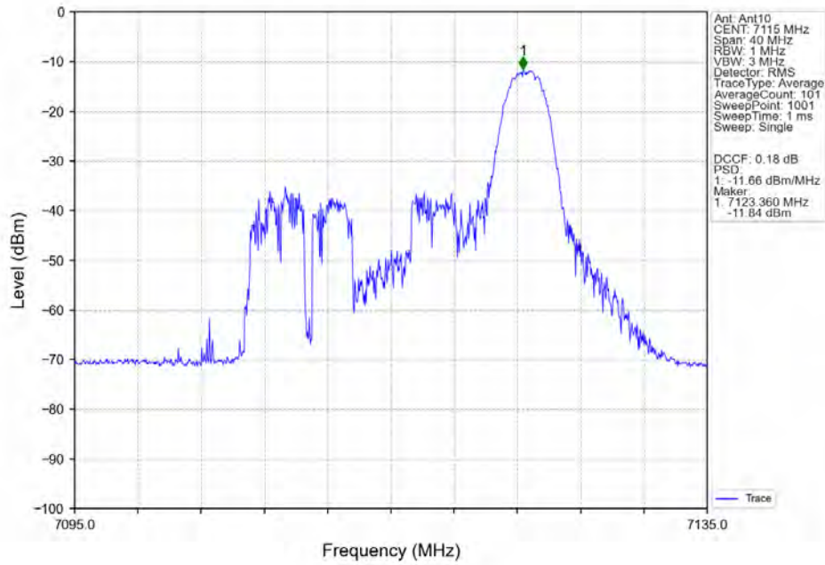
802.11ax(HEW20)_HCH_7115MHz_RU26_Right MIMO NTN
