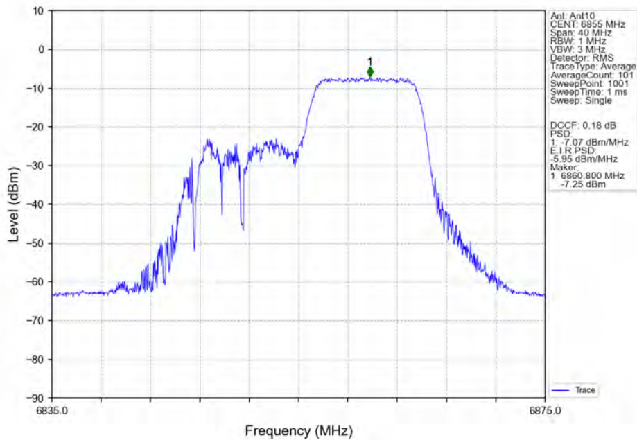
802.11ax(HEW20) HCH 6855MHz RU106 Right Ant10 NTN
