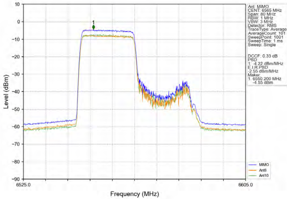
802.11ax(HEW40)_LCH_6565MHz_SU / Ant8 NTN
