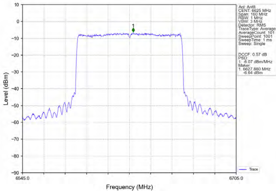
802.11ax(HEW80)_LCH_6625MHz_SU / Ant8 NTN
