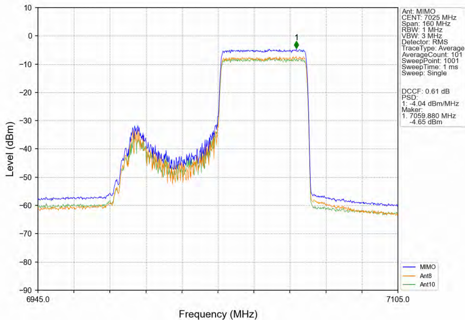
802.11ax(HEW80) HCH 7025MHz RU484 Right MIMO NTN
