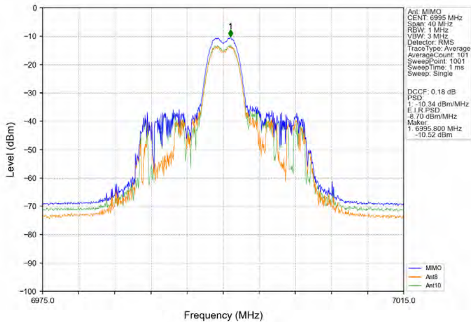
802.11ax(HEW20)_MCH_6995MHz_RU26_Mid MIMO NTN
