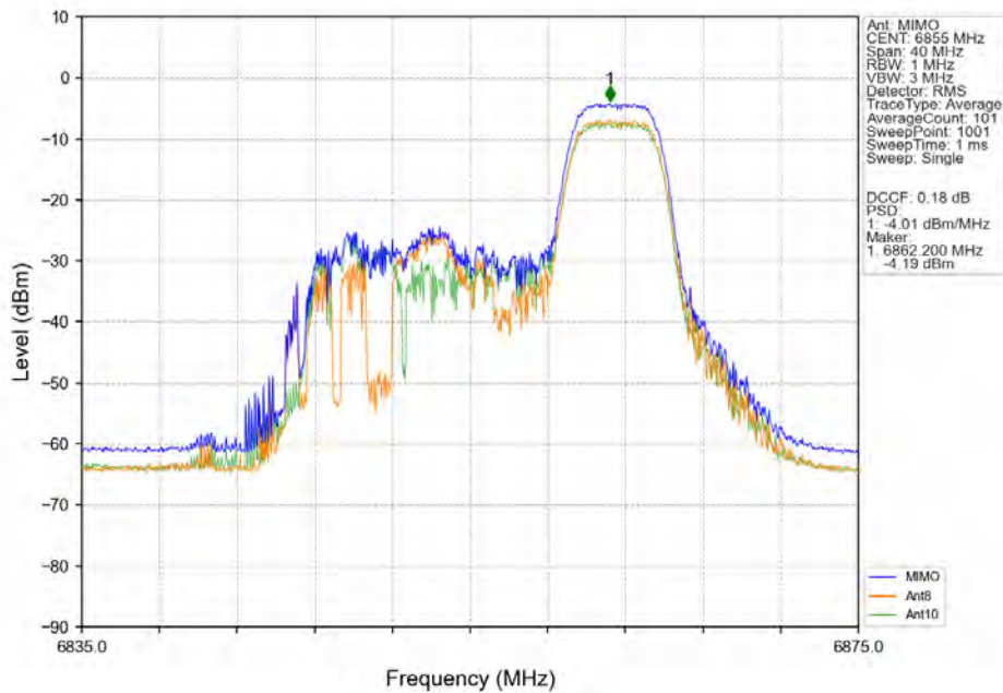
802.11ax(HEW20)_HCH_6855MHz_RU52_Right_MIMO_NTNV
