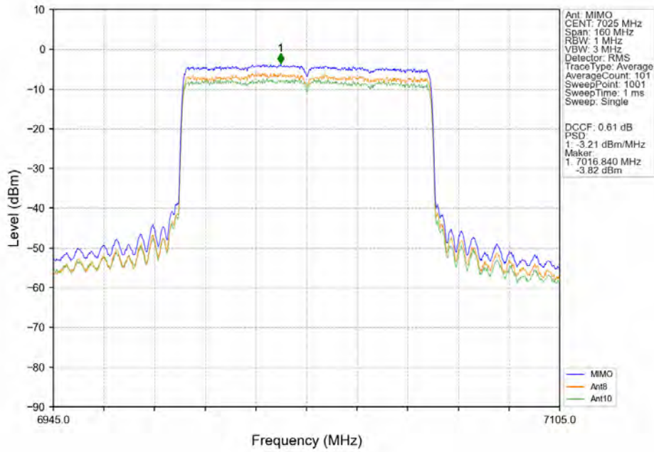
802.11ax(HEW80)_HCH_7025MHz_SU_/_MIMO_NTNV
