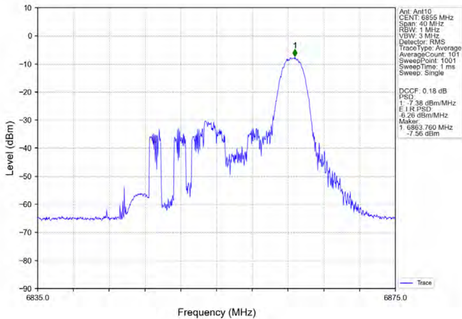
802.11ax(HEW20)_HCH_6855MHz_RU26_Right_Ant10_NTNV
