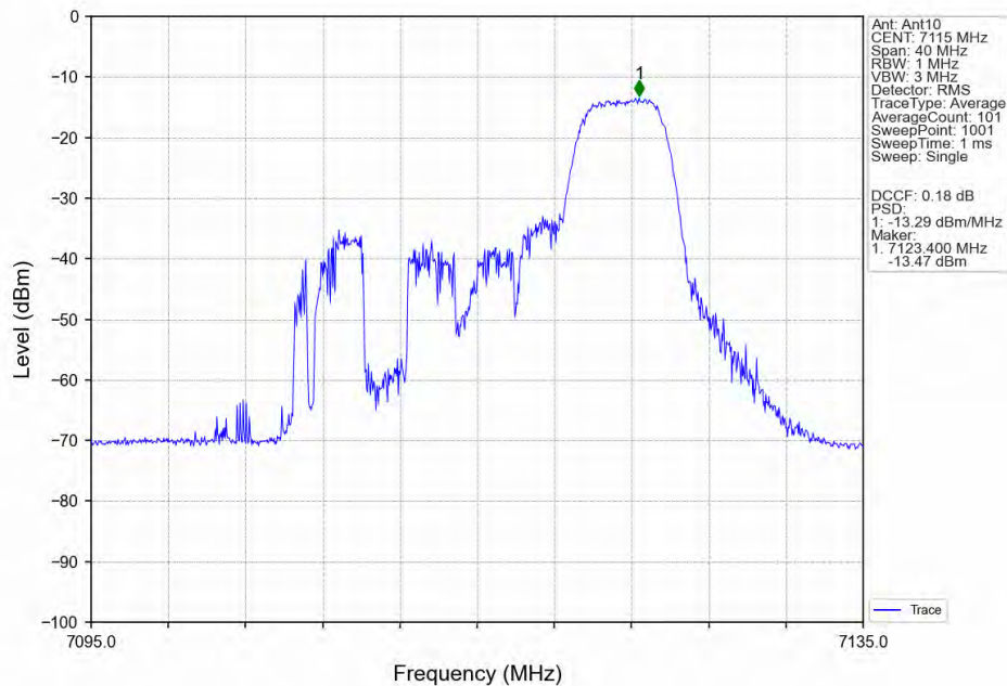
802.11ax(HEW20)_HCH_7115MHz_RU52_Right_Ant10_NTNV
