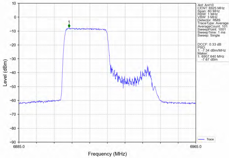
802.11ax(HEW40)_LCH_6925MHz_RU242_Left MIMO NTNV
