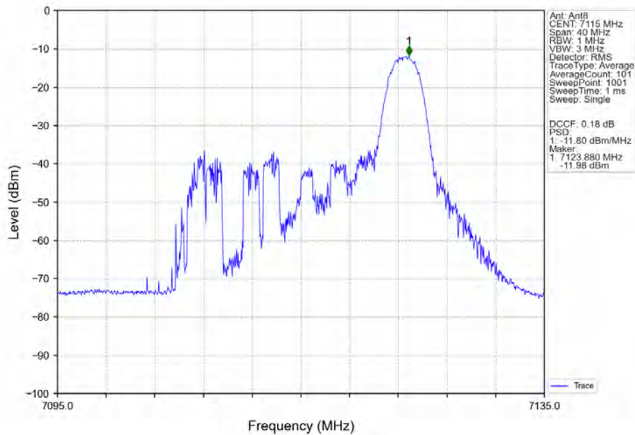
802.11ax(HEW20) HCH 7115MHz RU26 Right Ant8 NTN
