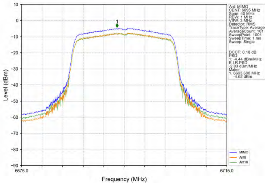
802.11ax(HEW20)_MCH_6695MHz_SU_/_MIMO_NTNV
