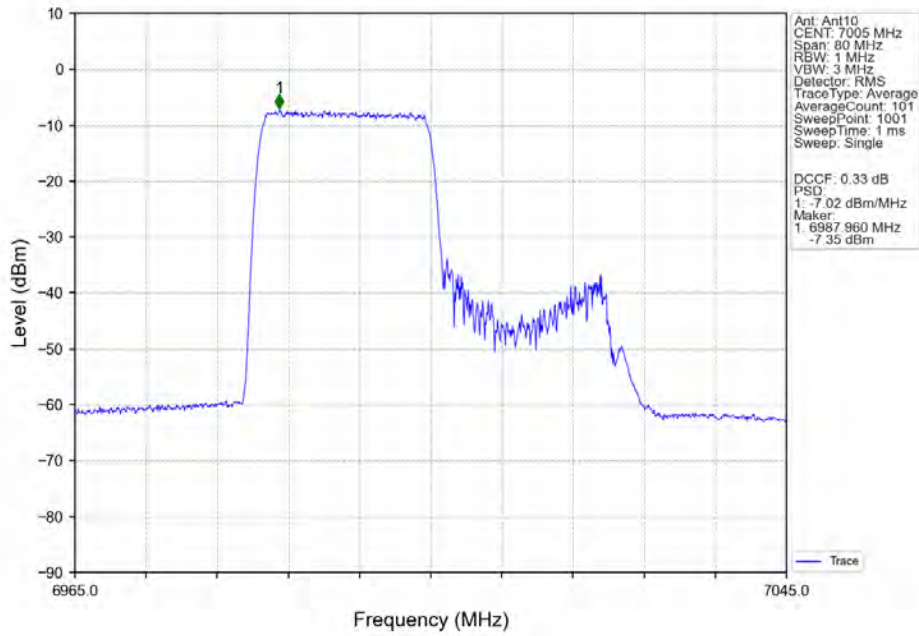
802.11ax(HEW40)_MCH_7005MHz_RU242_Left_MIMO_NTNV
