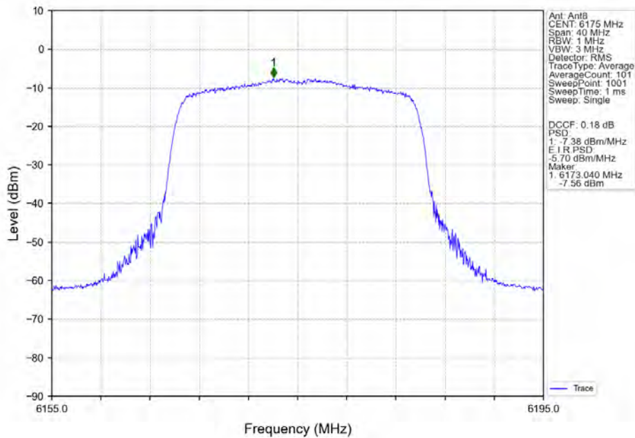
802.11ax(HEW20)_MCH_6175MHz_SU / Ant8 NTN
