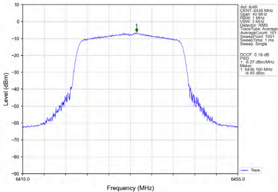
802.11ax(HEW20)_LCH_6435MHz_SU / Ant8 NTN
