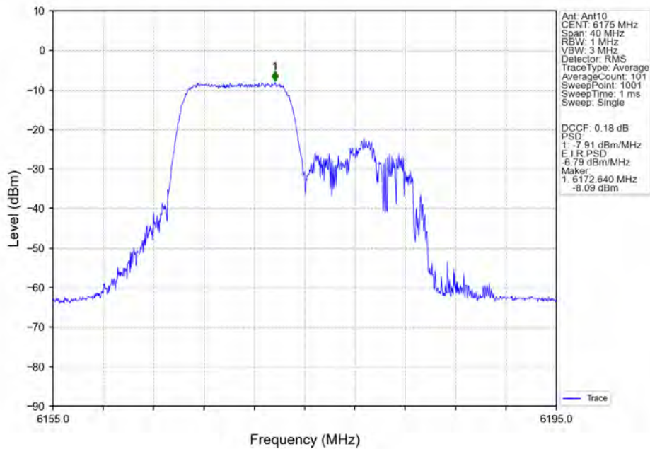
802.11ax(HEW20)_MCH_6175MHz_RU106_Left_Ant10_NTNV
