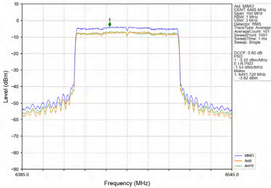
802.11ax(HEW80)_LCH_6465MHz_SU_/_MIMO_NTNV
