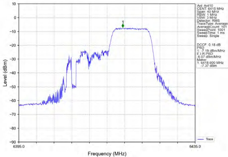
802.11ax(HEW20) HCH 6415MHz RU106 Right Ant10 NTN
