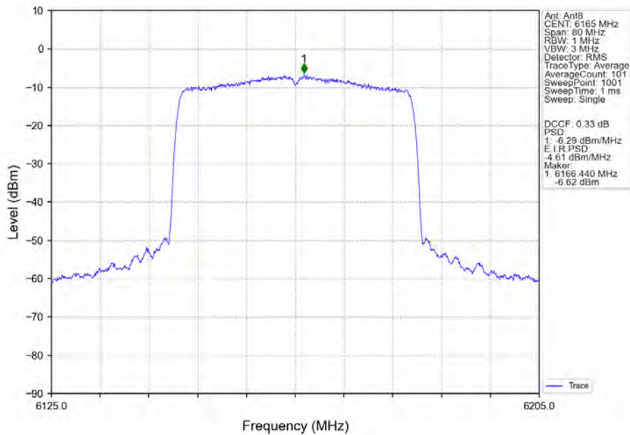
802.11ax(HEW40)_MCH_6165MHz_SU / Ant8 NTN
