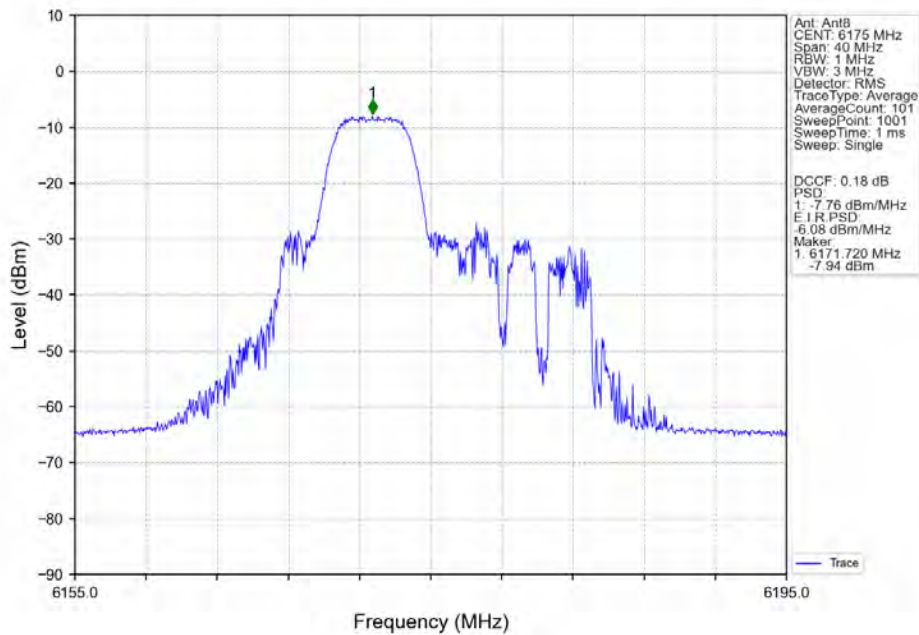
802.11ax(HEW20) MCH 6175MHz RU52 Mid Ant8 NTN
