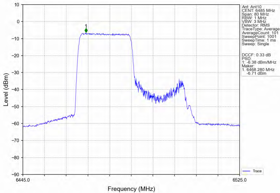
802.11ax(HEW40)_MCH_6485MHz_RU242_Left_Ant10_NTNV
