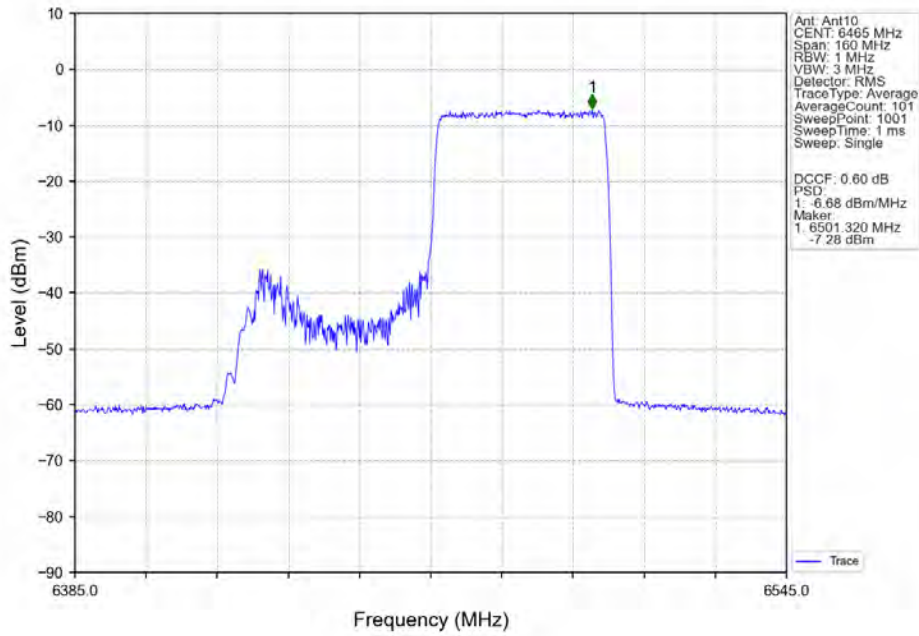
802.11ax(HEW80)_LCH_6465MHz_RU484_Right MIMO NTN
