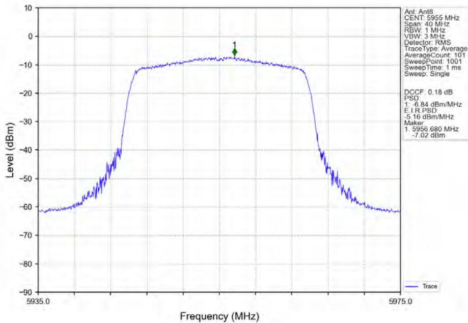
802.11ax(HEW20)_LCH_5955MHz_SU / Ant8 NTN
