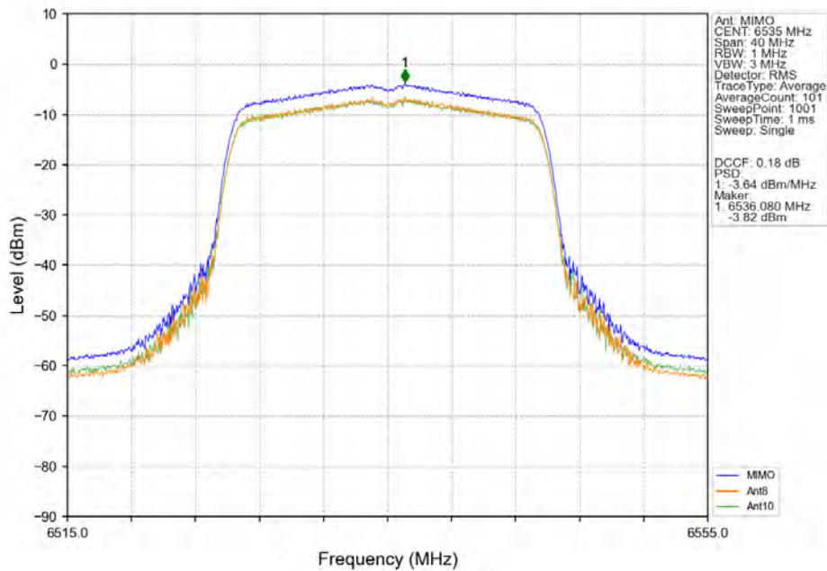
802.11ax(HEW20)_LCH_6535MHz_SU_/_MIMO NTN
