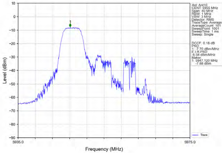
802.11ax(HEW20)_LCH_5955MHz_RU52_Left_MIMO_NTNV
