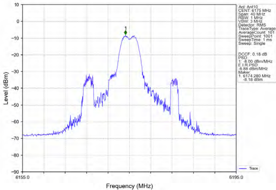
802.11ax(HEW20)_MCH_6175MHz_RU26_Mid_Ant10_NTNV
