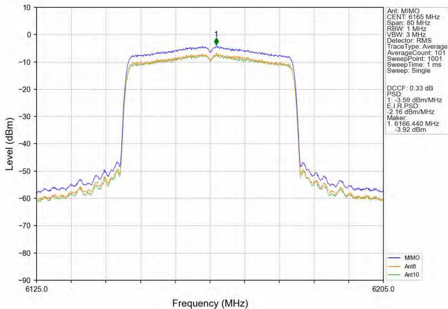
802.11ax(HEW40)_MCH_6165MHz_SU_/_MIMO NTN
