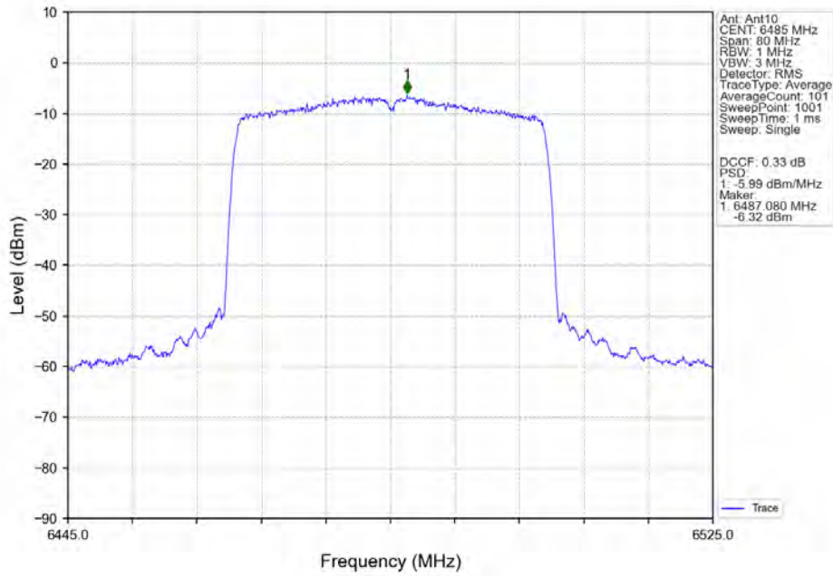
802.11ax(HEW40)_MCH_6485MHz_SU / MIMO NTN
