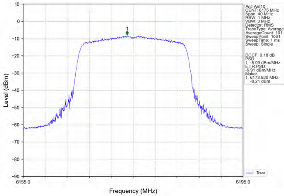
802.11ax(HEW20)_MCH_6175MHz_SU_/_MIMO_NTNV
