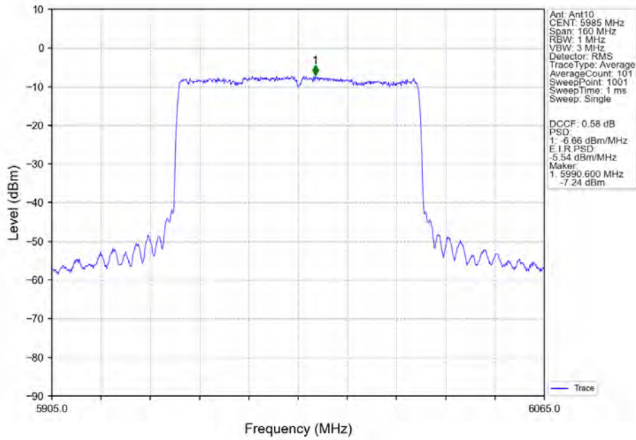
802.11ax(HEW80)_LCH_5985MHz_SU_/_MIMO NTN
