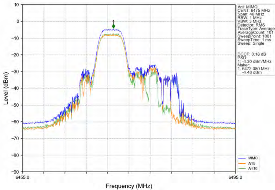
802.11ax(HEW20)_MCH_6475MHz_RU52_Mid MIMO NTN
