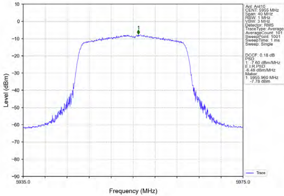
802.11ax(HEW20)_LCH_5955MHz_SU_/_MIMO_NTNV
