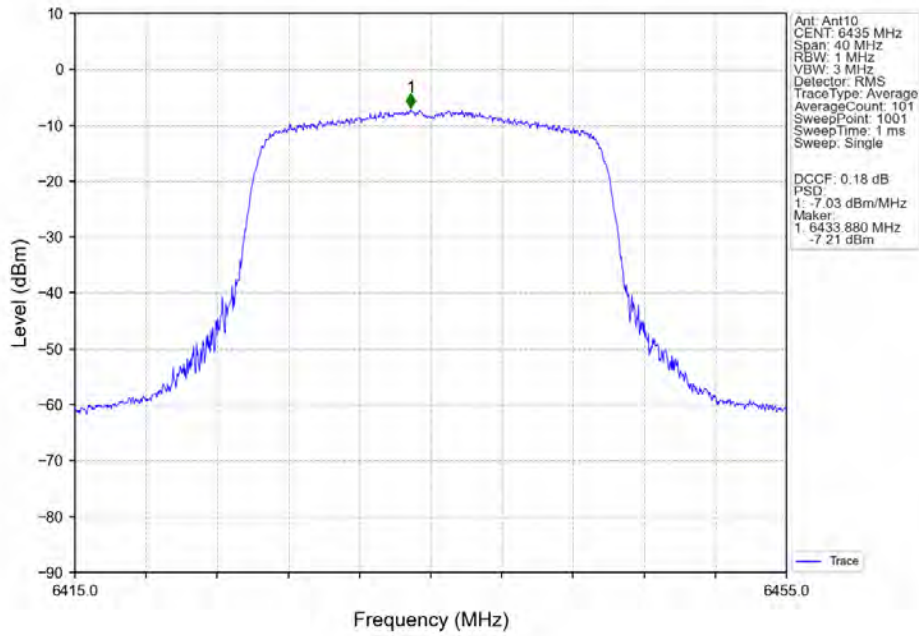
802.11ax(HEW20)_LCH_6435MHz_SU_/_MIMO NTN
