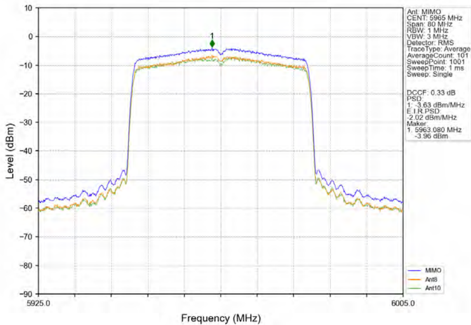
802.11ax(HEW40)_LCH_5965MHz_SU_/_MIMO NTN
