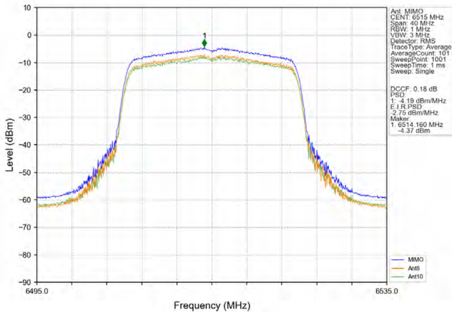
802.11ax(HEW20)_HCH_6515MHz_SU_/_MIMO_NTNV
