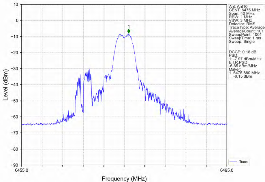
802.11ax(HEW20)_MCH_6475MHz_RU26_Mid_Ant10_NTNV
