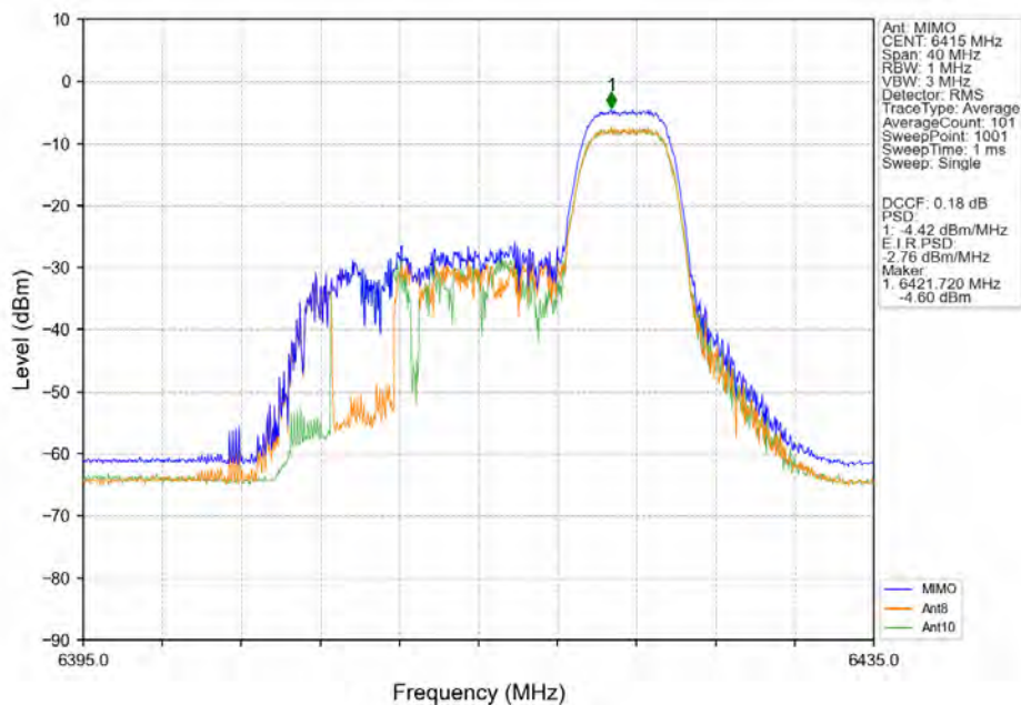
802.11ax(HEW20)_HCH_6415MHz_RU52_Right_MIMO_NTNV
