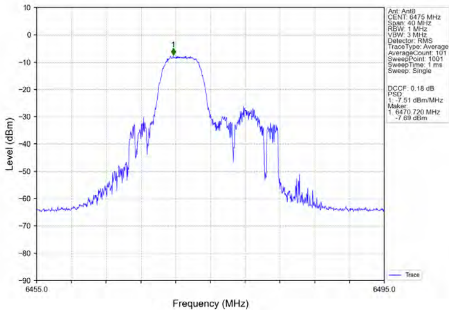
802.11ax(HEW20) MCH 6475MHz RU52 Mid Ant8 NTN
