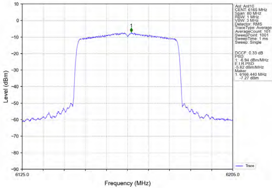
802.11ax(HEW40)_MCH_6165MHz_SU_/_MIMO NTN
