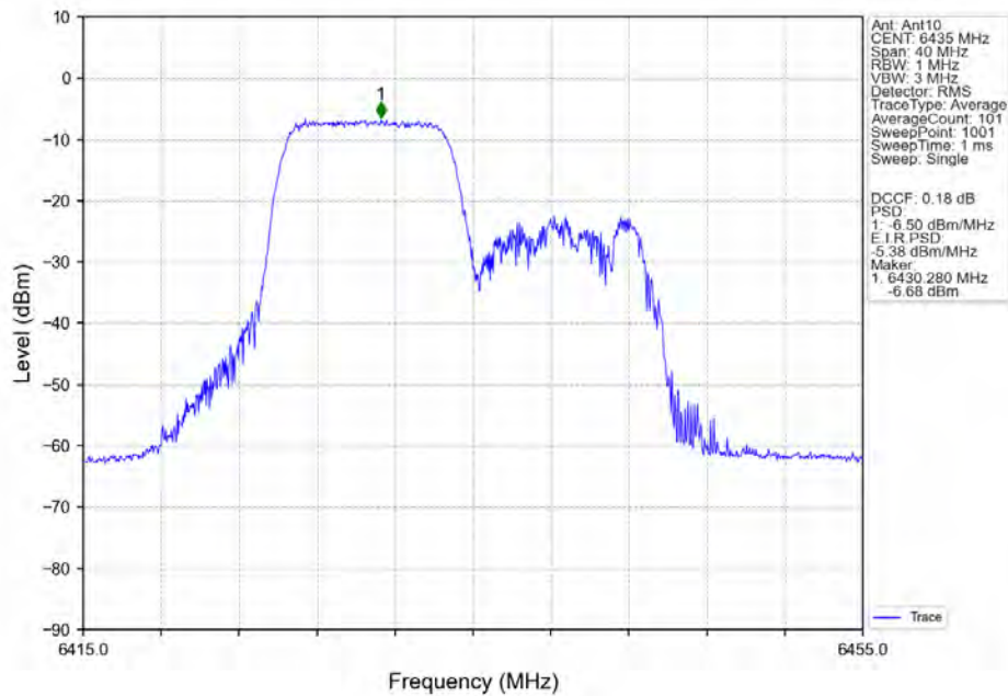
802.11ax(HEW20)_LCH_6435MHz_RU106_Left_Ant10_NTNV
