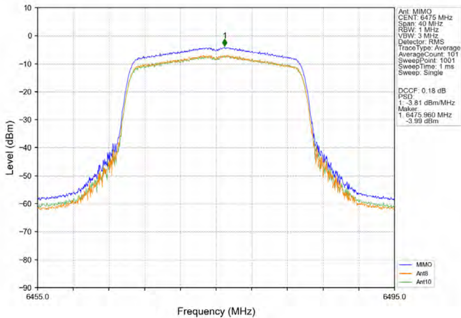
802.11ax(HEW20)_MCH_6475MHz_SU_/_MIMO_NTNV
