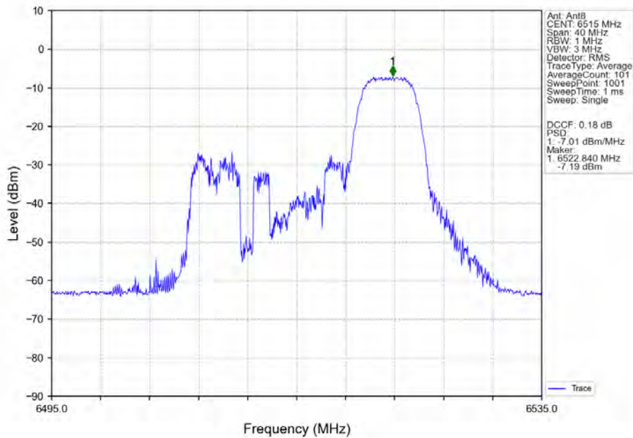
802.11ax(HEW20)_HCH_6515MHz_RU52_Right_Ant8_NTNV
