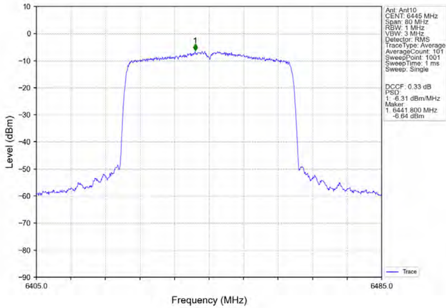
802.11ax(HEW40)_LCH_6445MHz_SU_/_MIMO NTN
