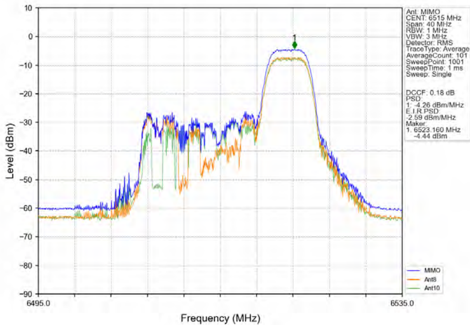
802.11ax(HEW20)_HCH_6515MHz_RU52_Right MIMO NTN
