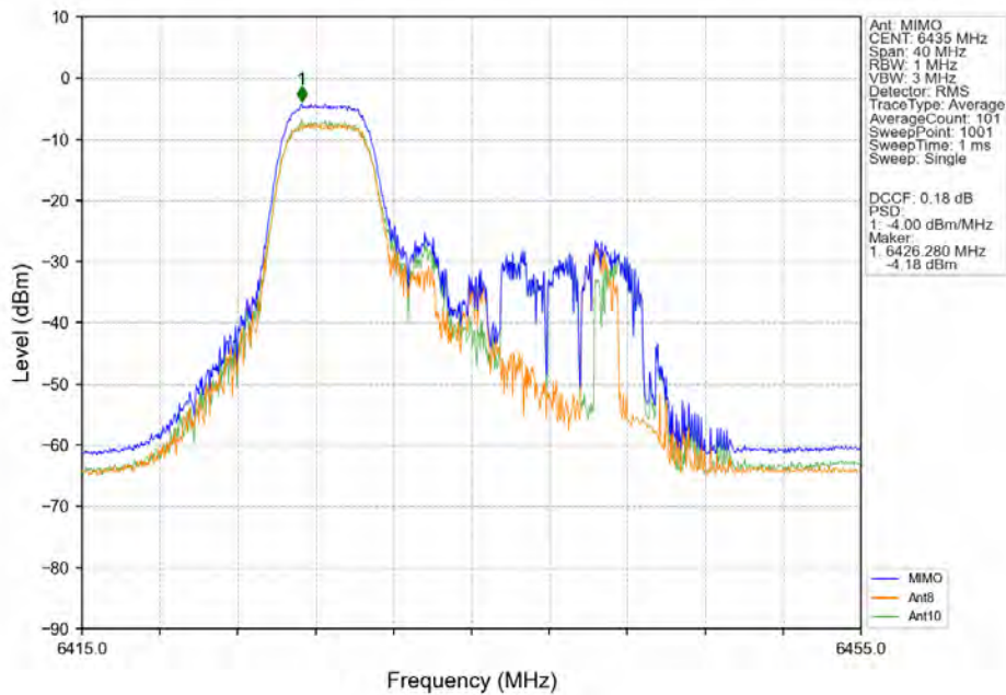
802.11ax(HEW20)_LCH_6435MHz_RU52_Left_MIMO_NTNV
