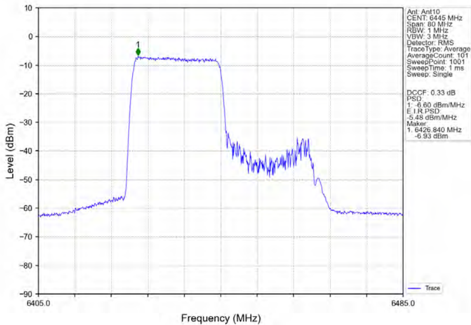
802.11ax(HEW40)_LCH_6445MHz_RU242_Left_Ant10_NTNV
