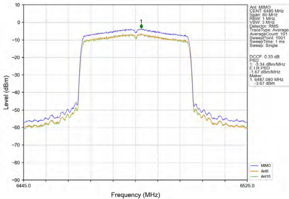
802.11ax(HEW40)_MCH_6485MHz_SU_/_MIMO_NTNV
