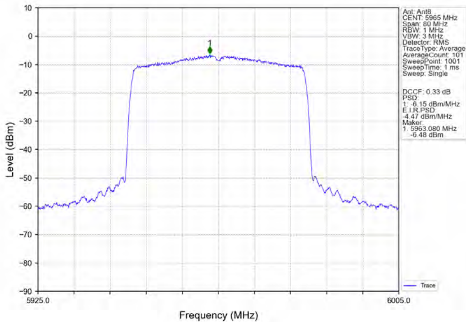
802.11ax(HEW40)_LCH_5965MHz_SU / Ant8 NTN
