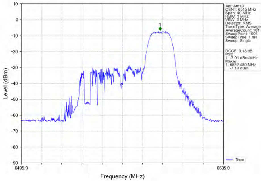
802.11ax(HEW20)_HCH_6515MHz_RU52_Right_MIMO_NTNV
