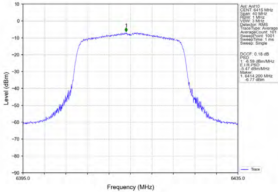
802.11ax(HEW20)_HCH_6415MHz_SU_/_MIMO_NTNV
