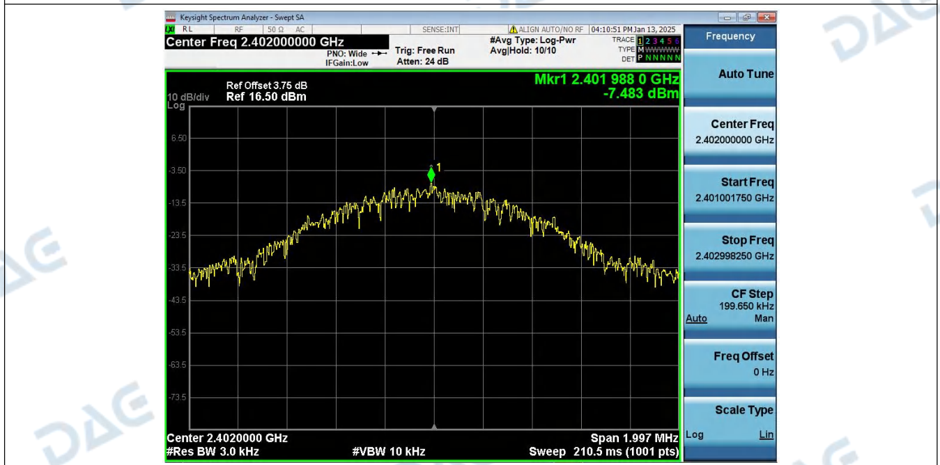
Power_Spectral_Density_NVNT_ANT1_1Mbps_2402
