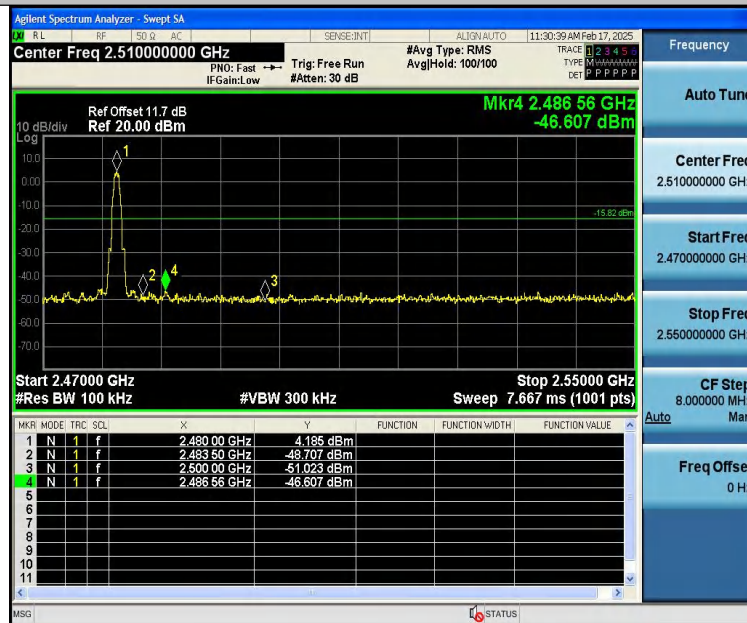
BLE_1M-Ant0-2480-PASS
