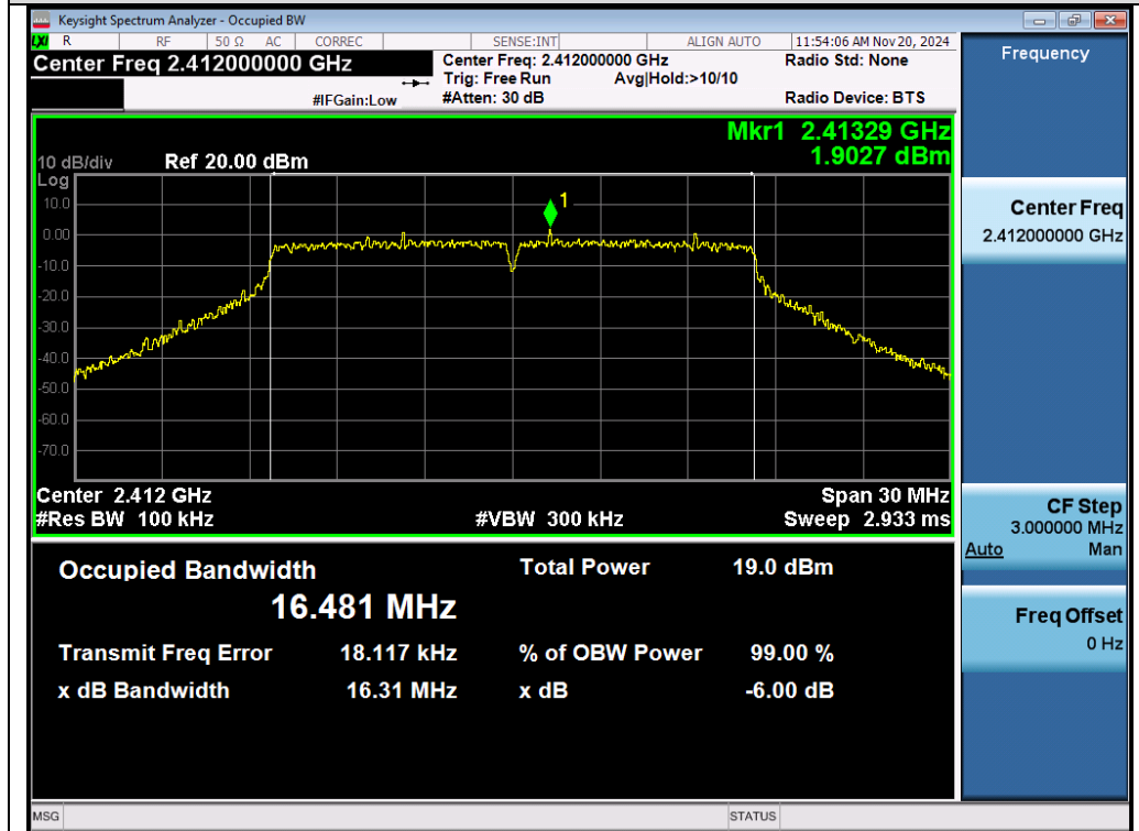
Test_Graph_802.11g_ANT1_2412_6Mbps_DTSSBW
