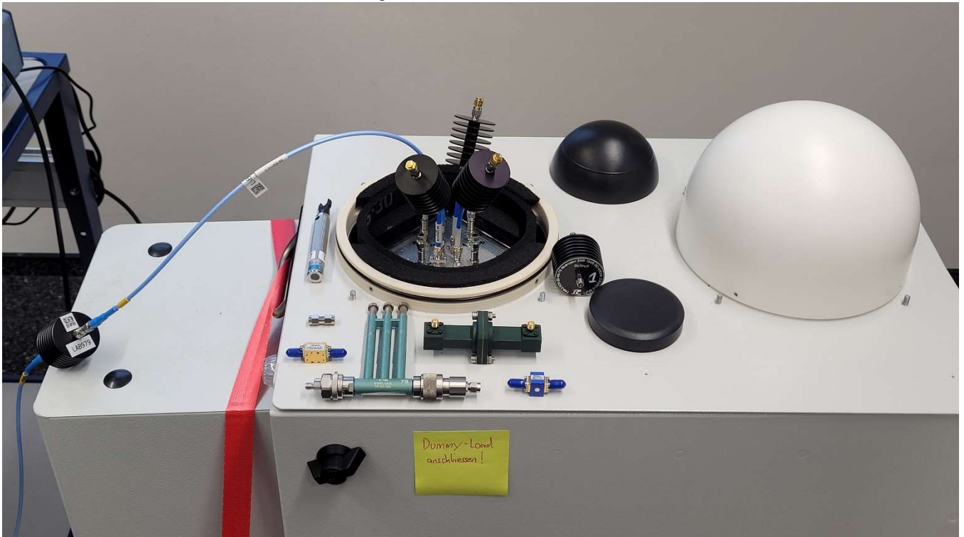
Photo No. 31: conducted RF tests, wanted signal
