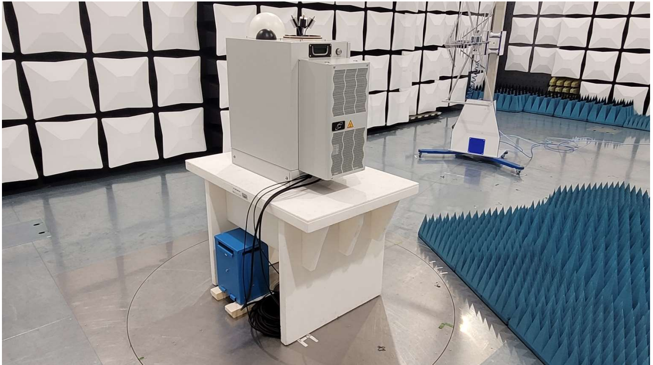
Photo No. 25: radiated spurious
