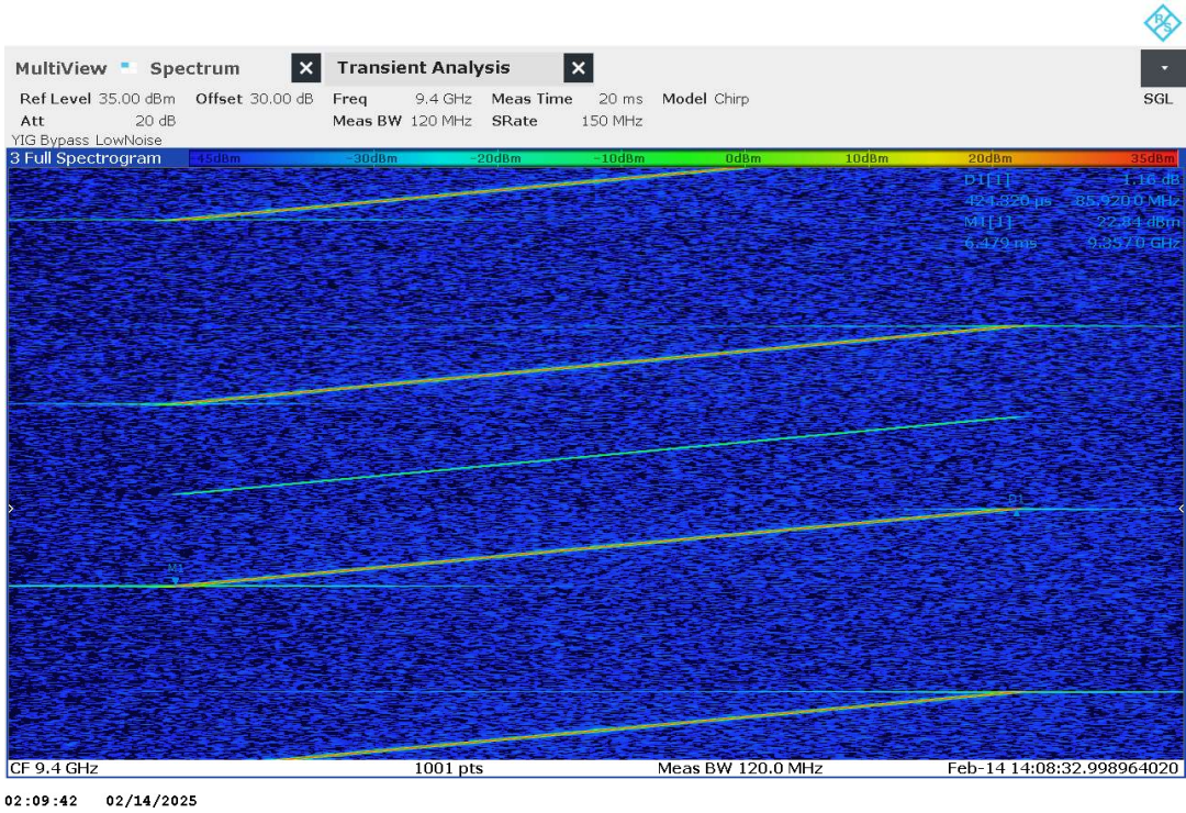
Plot no. 123: Timing CH4, 83 MHz
