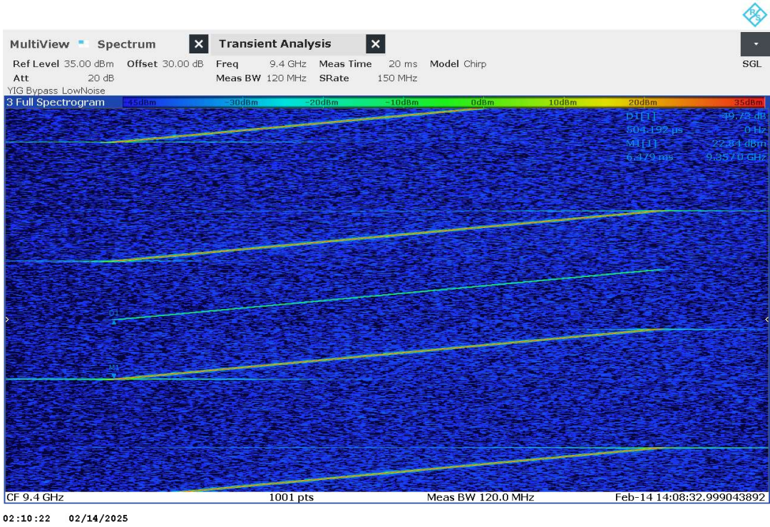
Plot no. 124: Timing CH4, 83 MHz
