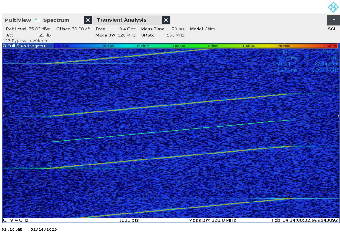
Plot no. 125: Timing CH4, 83 MHz
