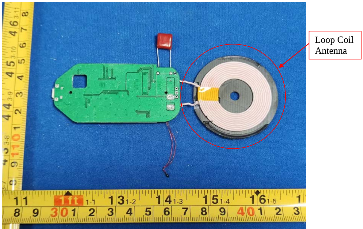
FIGURE 9 FAST WIRELESS CHARGER (HD01) MAINBOARD BACK
