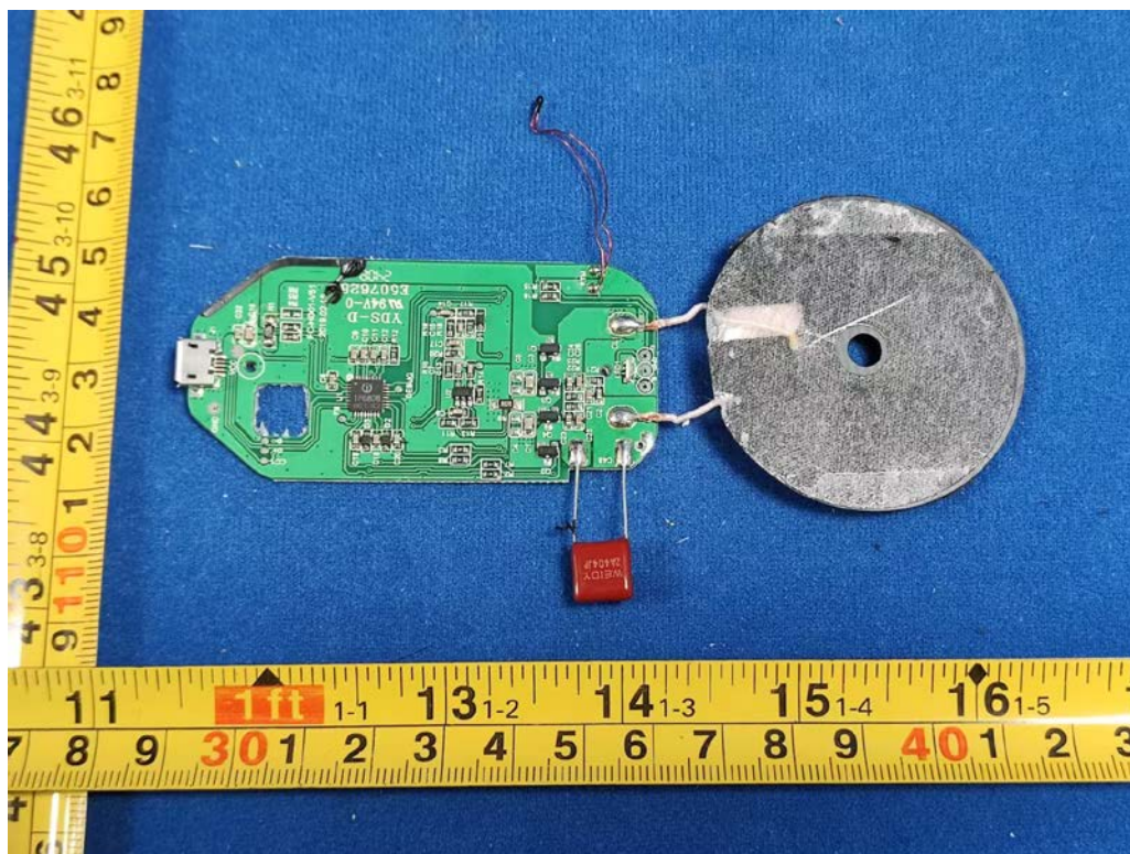
FIGURE 8 FAST WIRELESS CHARGER (HD01) MAINBOARD FRONT
