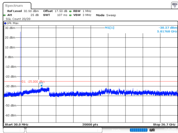
5MHz_High_QPSK_1@0(30MHz~26.7GHz)
