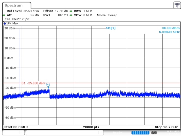
5MHz_Middle_QPSK_1@0(30MHz~26.7GHz)
