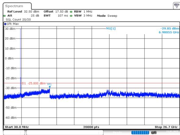
10MHz_Middle_QPSK_1@0(30MHz~26.7GHz)
