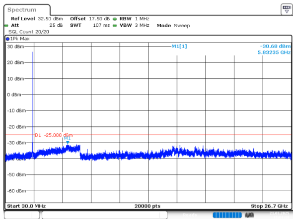
10MHz_High_QPSK_1@0(30MHz~26.7GHz)
