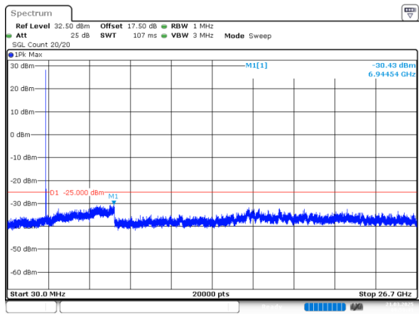
10MHz_Low_QPSK_1@0(30MHz~26.7GHz)
