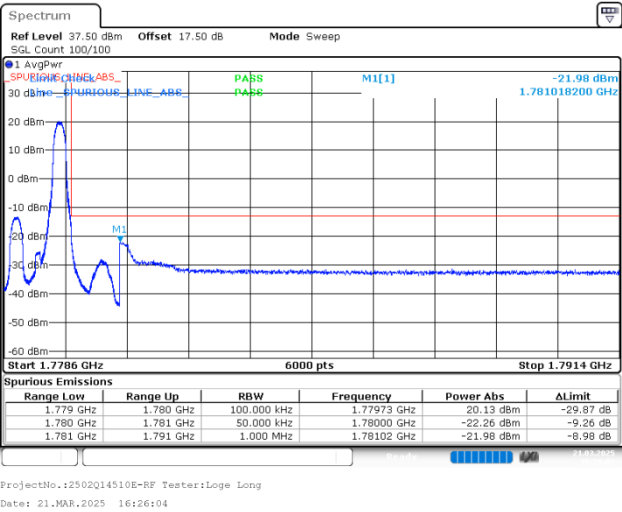
1.4MHz_High_16QAM_1@5
