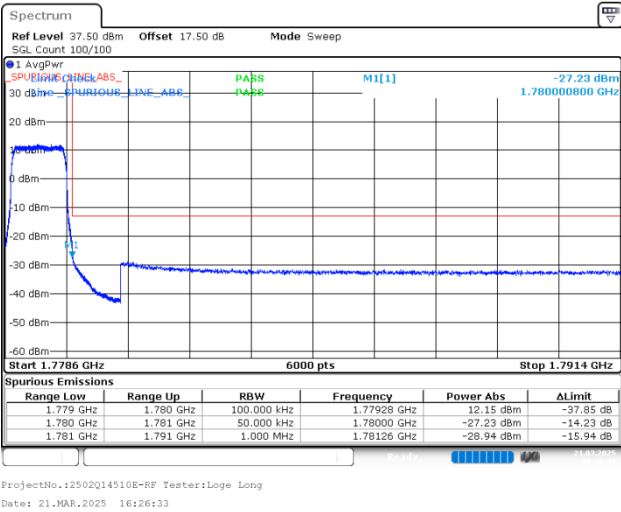
1.4MHz_High_16QAM_6@0
