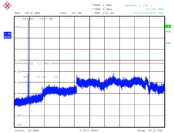
15MHz_Middle_QPSK_1@0(30MHz~18.8GHz)
