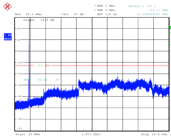
20MHz_High_QPSK_1@0(30MHz~18.8GHz)
