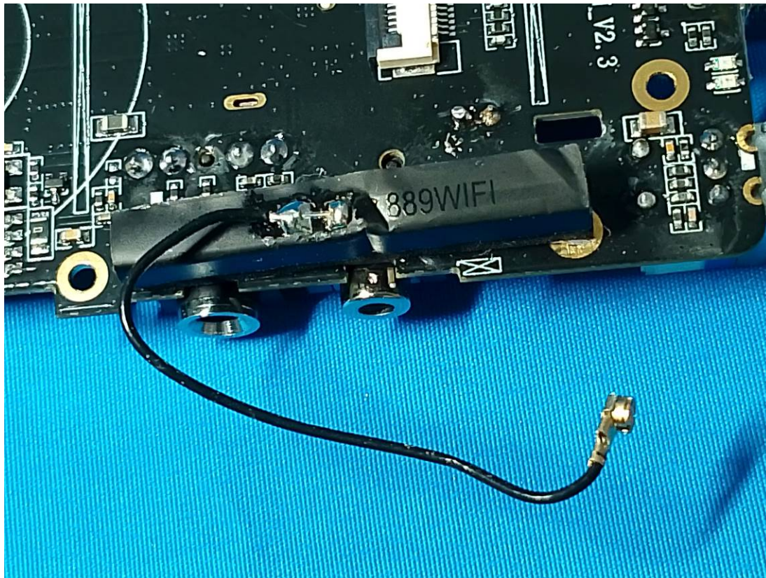
Bluetooth&Wifi Antenna(no use)
