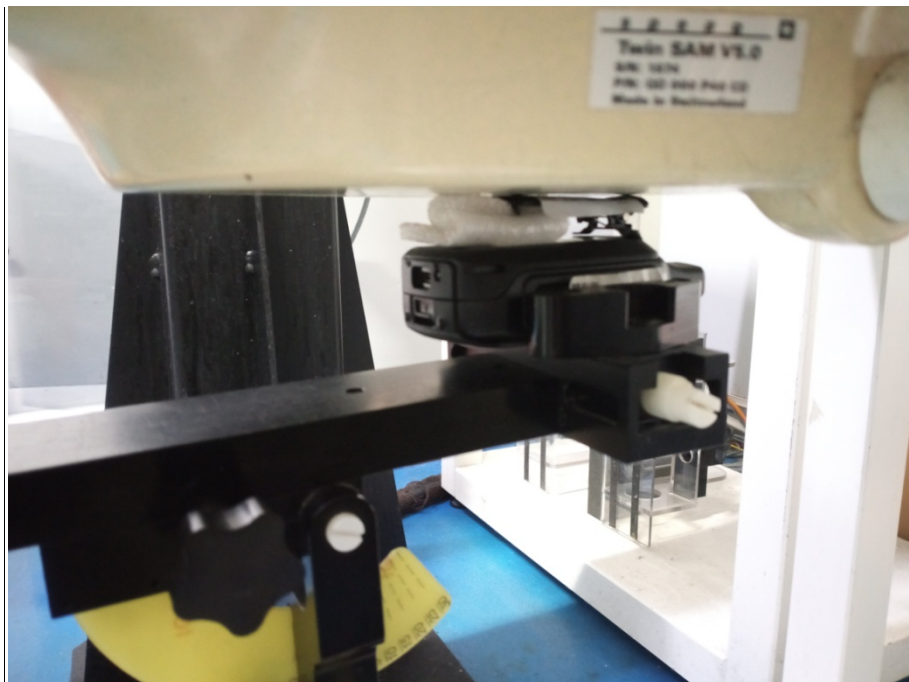
Body Back With Belt Clip Setup Photo(0mm)
