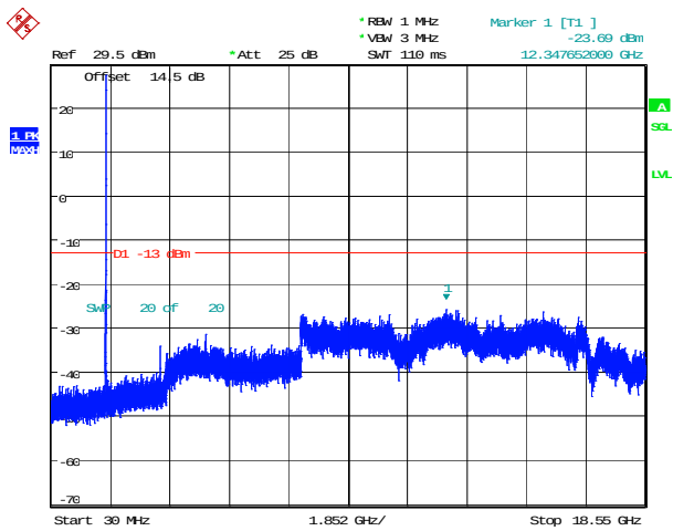
5MHz_Low_QPSK_1@0(30MHz~18.55GHz)
