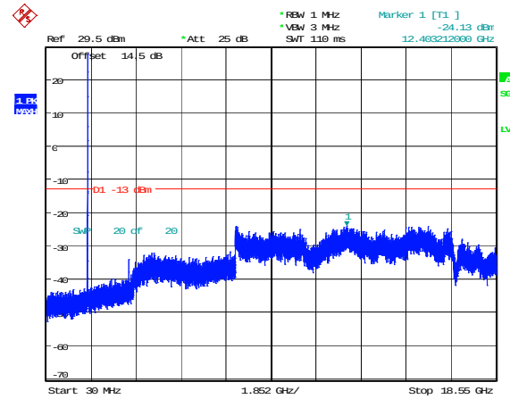
3MHz_Low_QPSK_1@0(30MHz~18.55GHz)
