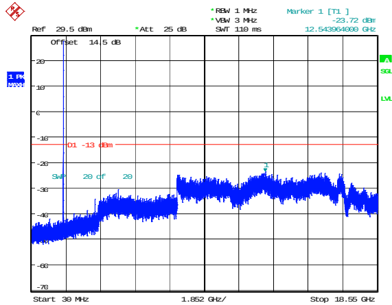
1.4MHz_Low_QPSK_1@0(30MHz~18.55GHz)
