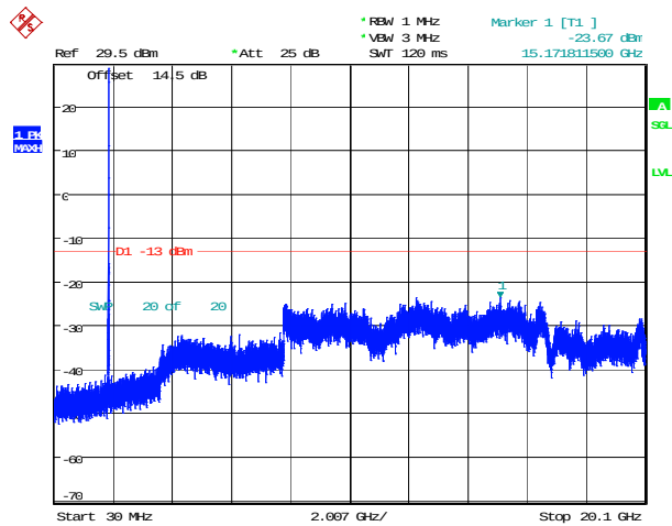
10MHz_Low_QPSK_1@0(30MHz~20.1GHz)
