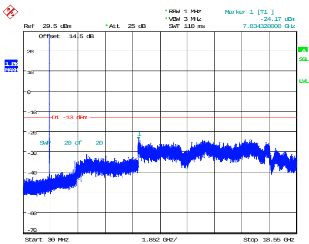
5MHz_High_QPSK_1@0(30MHz~18.55GHz)
