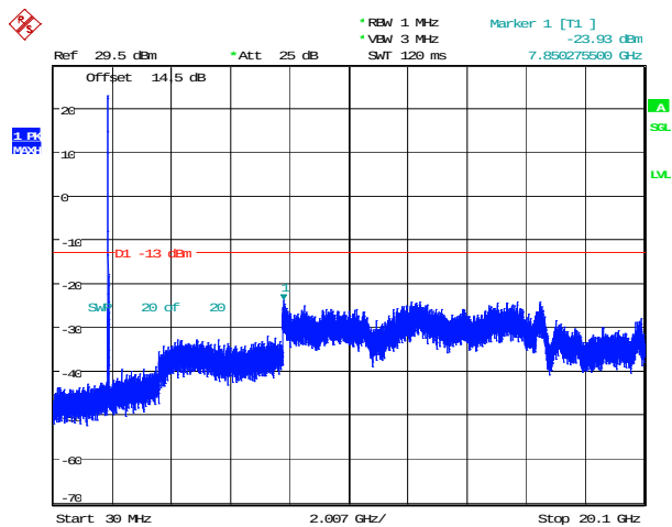
10MHz_Middle_QPSK_1@0(30MHz~20.1GHz)
