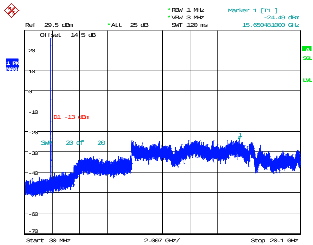
5MHz_High_QPSK_1@0(30MHz~20.1GHz)
