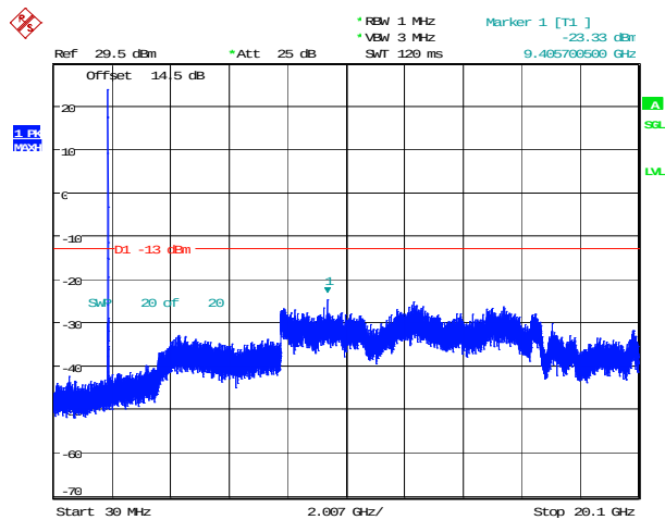
5MHz_Middle_QPSK_1@0(30MHz~20.1GHz)
