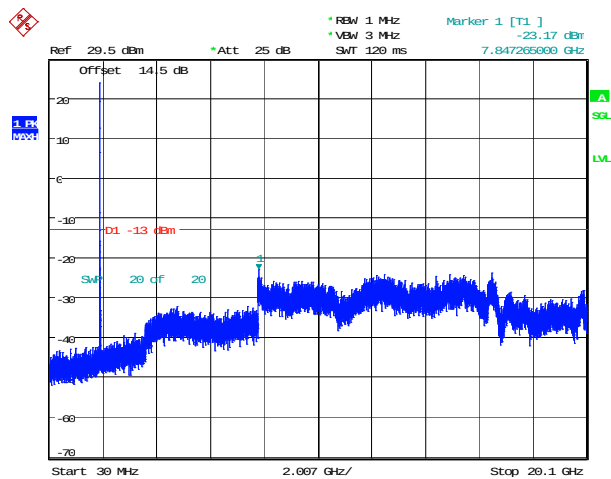
10MHz_High_QPSK_1@0(30MHz~20.1GHz)
