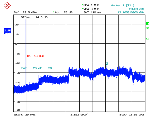
3MHz_High_QPSK_1@0(30MHz~18.55GHz)
