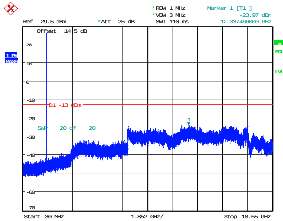
1.4MHz_High_QPSK_1@0(30MHz~18.55GHz)
