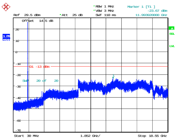
10MHz_Middle_QPSK_1@0(30MHz~18.55GHz)
