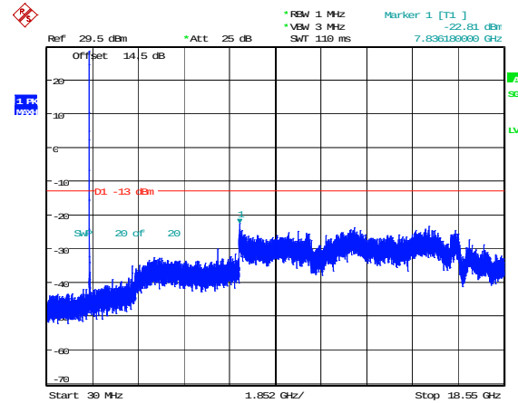
1.4MHz_Middle_QPSK_1@0(30MHz~18.55GHz)
