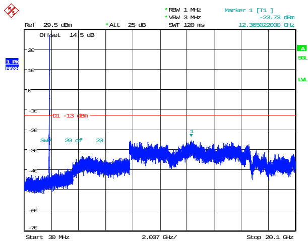
5MHz_Low_QPSK_1@0(30MHz~20.1GHz)
