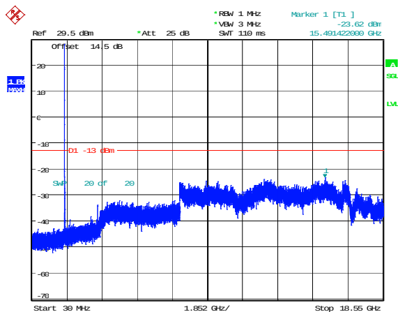
3MHz_Middle_QPSK_1@0(30MHz~18.55GHz)
