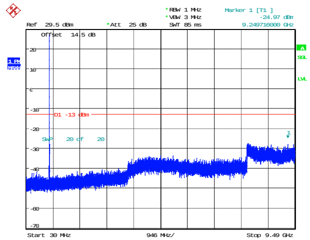
5MHz_Middle_QPSK_1@0(30MHz~9.49GHz)
