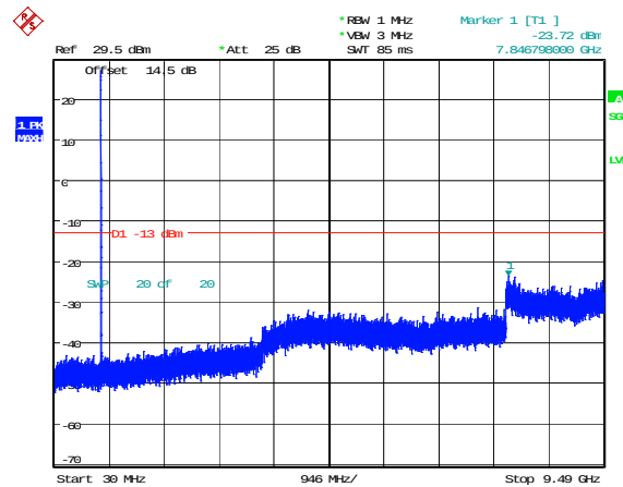
3MHz_Low_QPSK_1@0(30MHz~9.49GHz)
