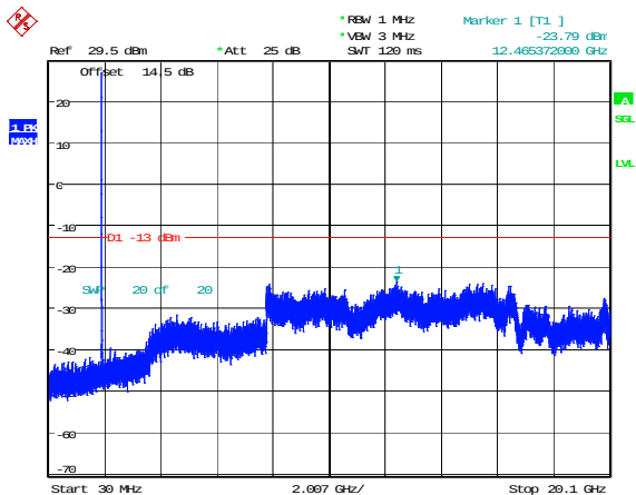
3MHz_High_QPSK_1@0(30MHz~20.1GHz)
