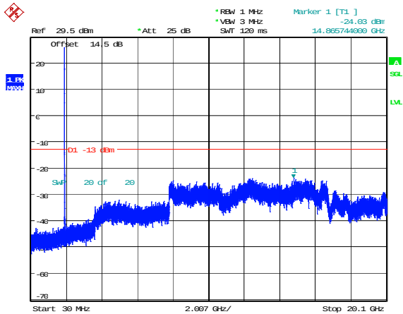
1.4MHz_High_QPSK_1@0(30MHz~20.1GHz)
