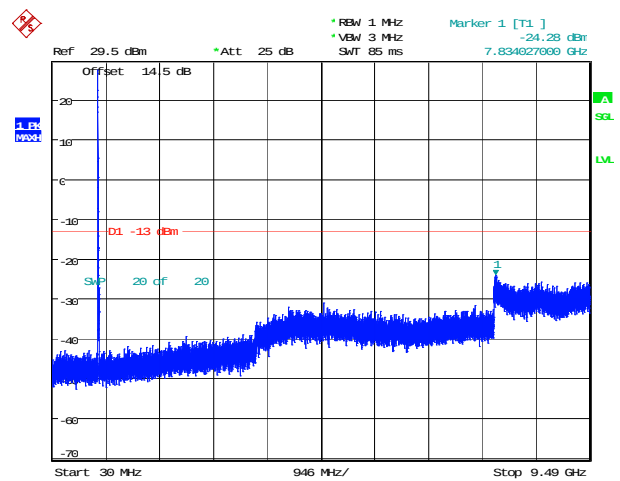
10MHz_Low_QPSK_1@0(30MHz~9.49GHz)
