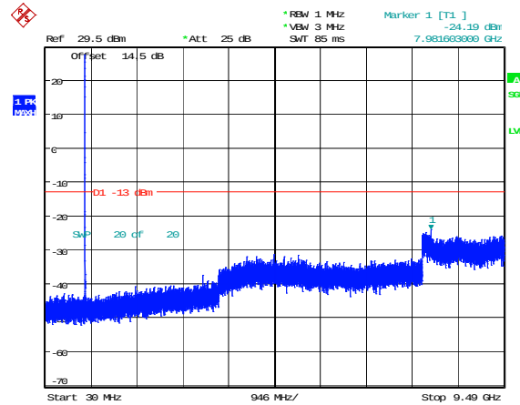
1.4MHz_Middle_QPSK_1@0(30MHz~9.49GHz)
