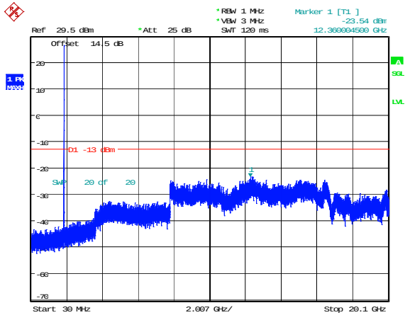
1.4MHz_Low_QPSK_1@0(30MHz~20.1GHz)
