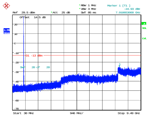
10MHz_High_QPSK_1@0(30MHz~9.49GHz)
