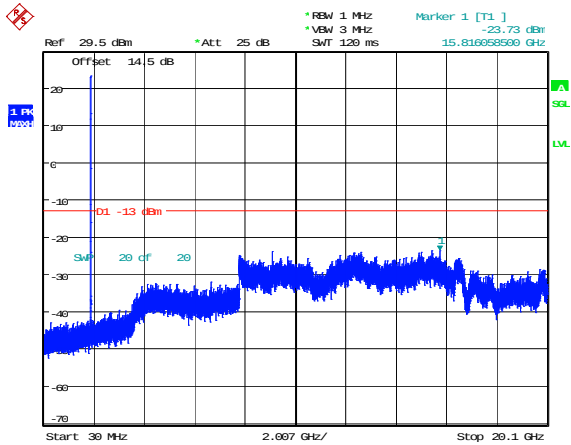
1.4MHz_Middle_QPSK_1@0(30MHz~20.1GHz)
