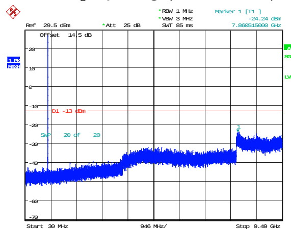
3MHz_High_QPSK_1@0(30MHz~9.49GHz)
