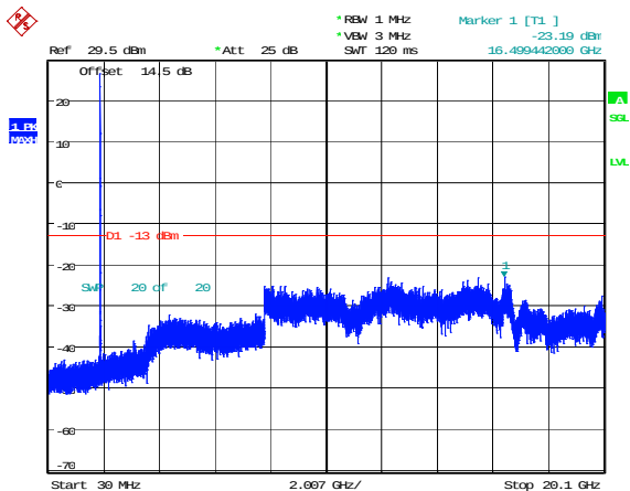
3MHz_Middle_QPSK_1@0(30MHz~20.1GHz)
