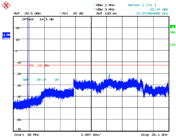
3MHz_Low_QPSK_1@0(30MHz~20.1GHz)
