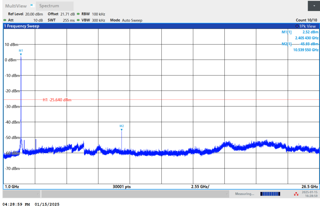
11N20SISO-Ant1-2412-1000~26500-PASS
