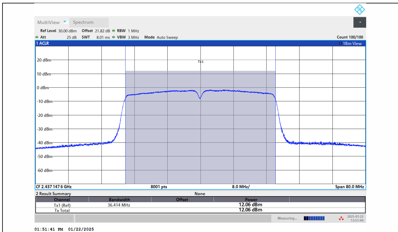
11N40SISO-Ant1-2437-PASS
