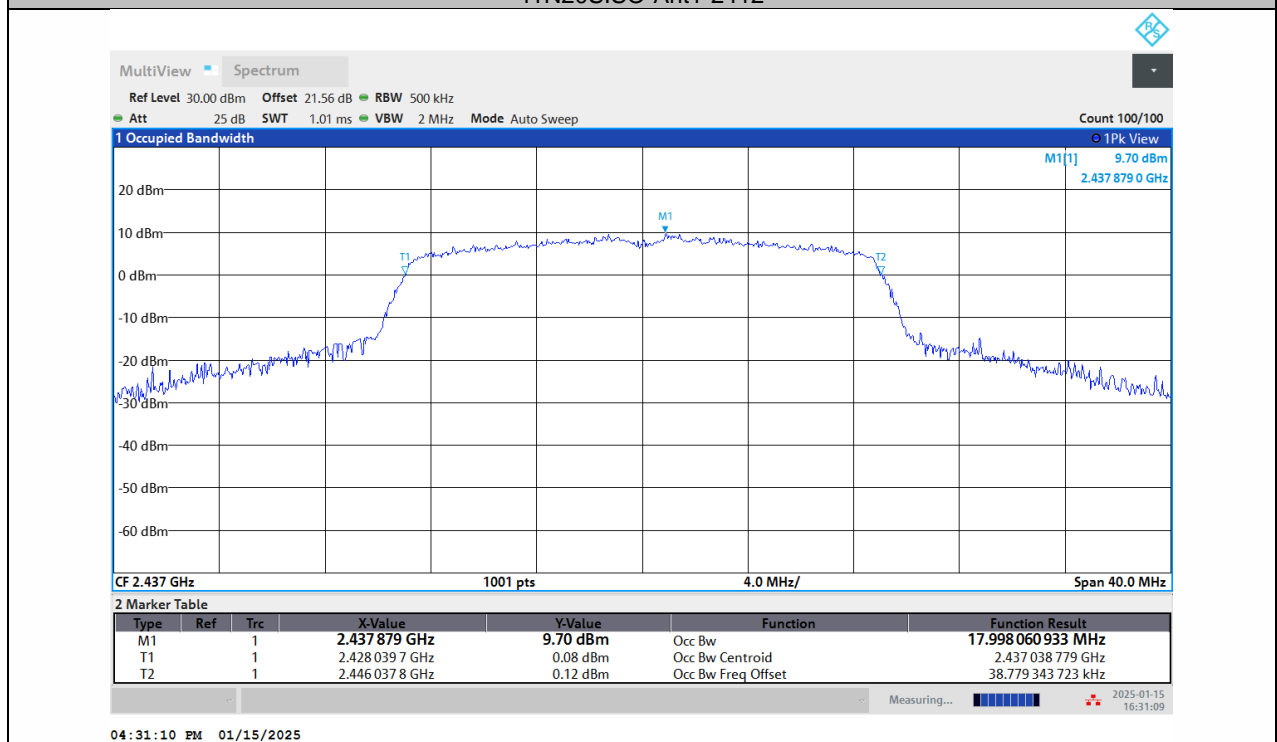
11N20SISO-Ant1-2437
