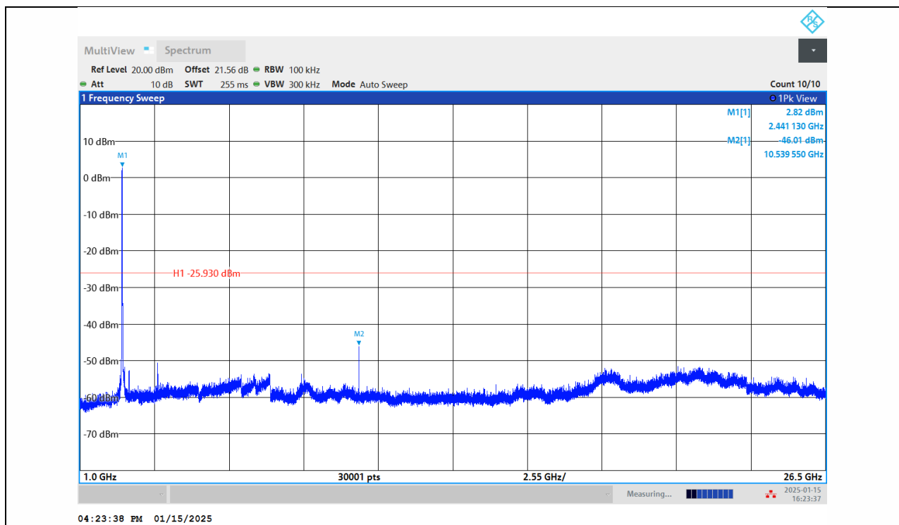
11G-Ant1-2437-1000~26500-PASS
