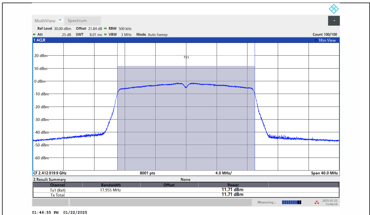
11N20SISO-Ant1-2412-PASS
