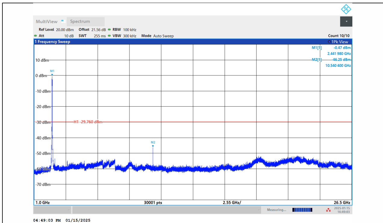
11N40SISO-Ant1-2437-1000~26500-PASS
