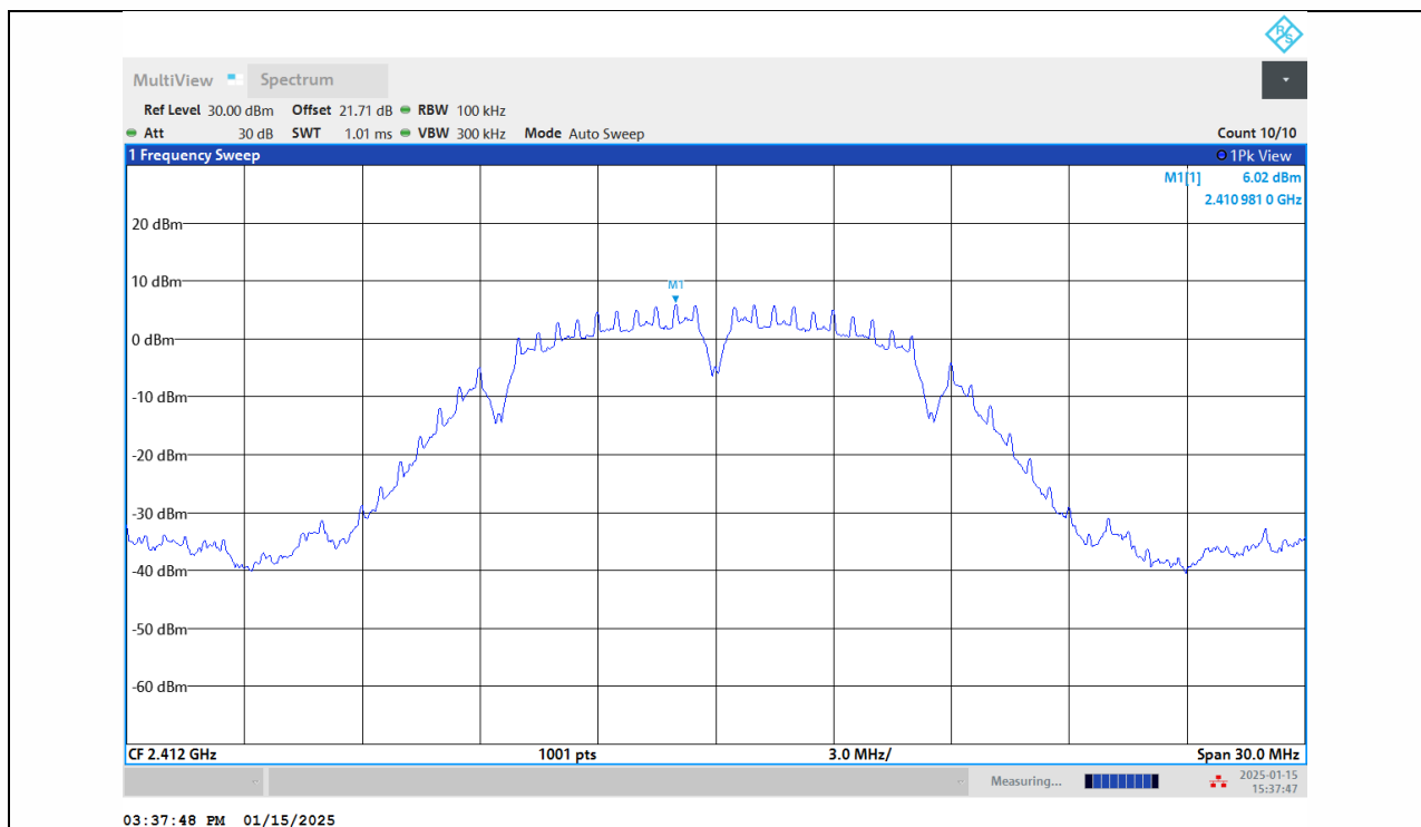
11B-Ant1-2412-0~Reference-PASS
