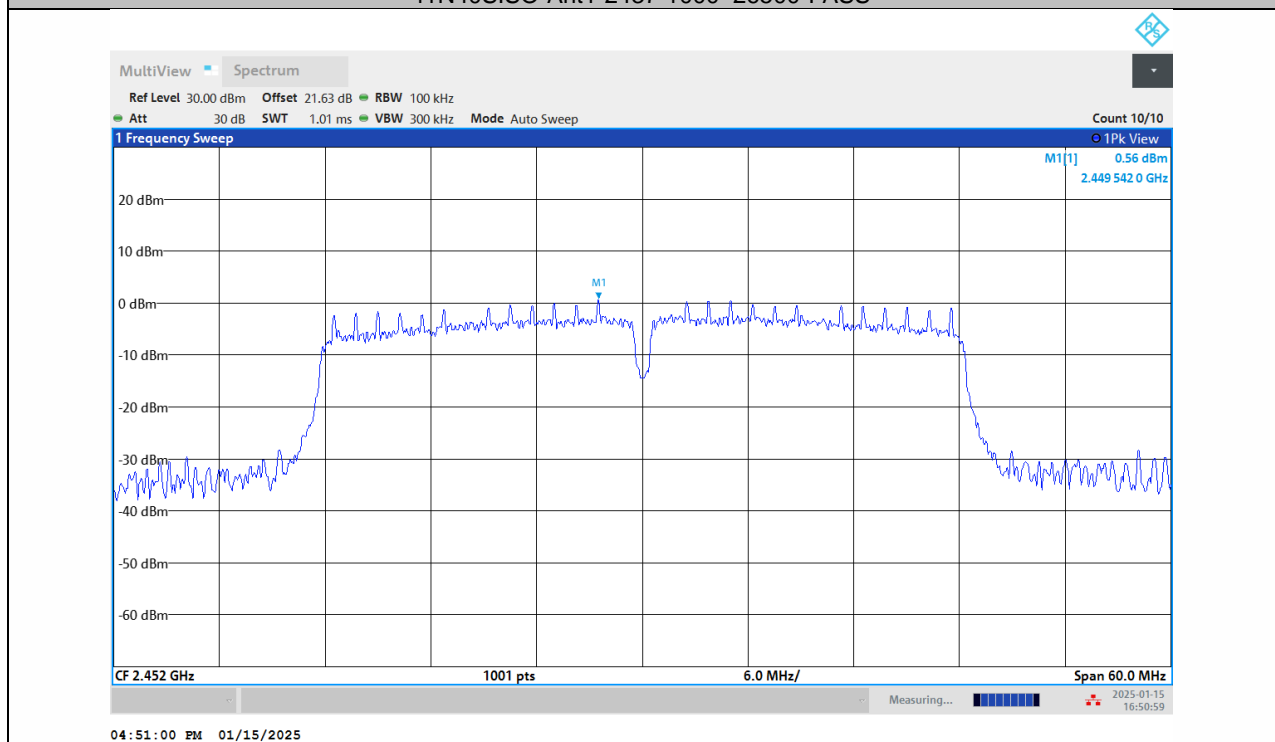
11N40SISO-Ant1-2452-0~Reference-PASS
