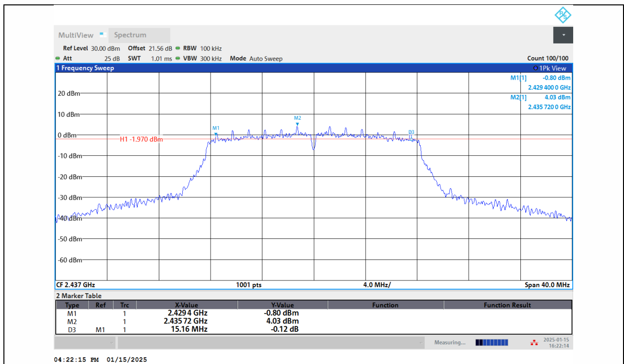
11G-Ant1-2437-PASS
