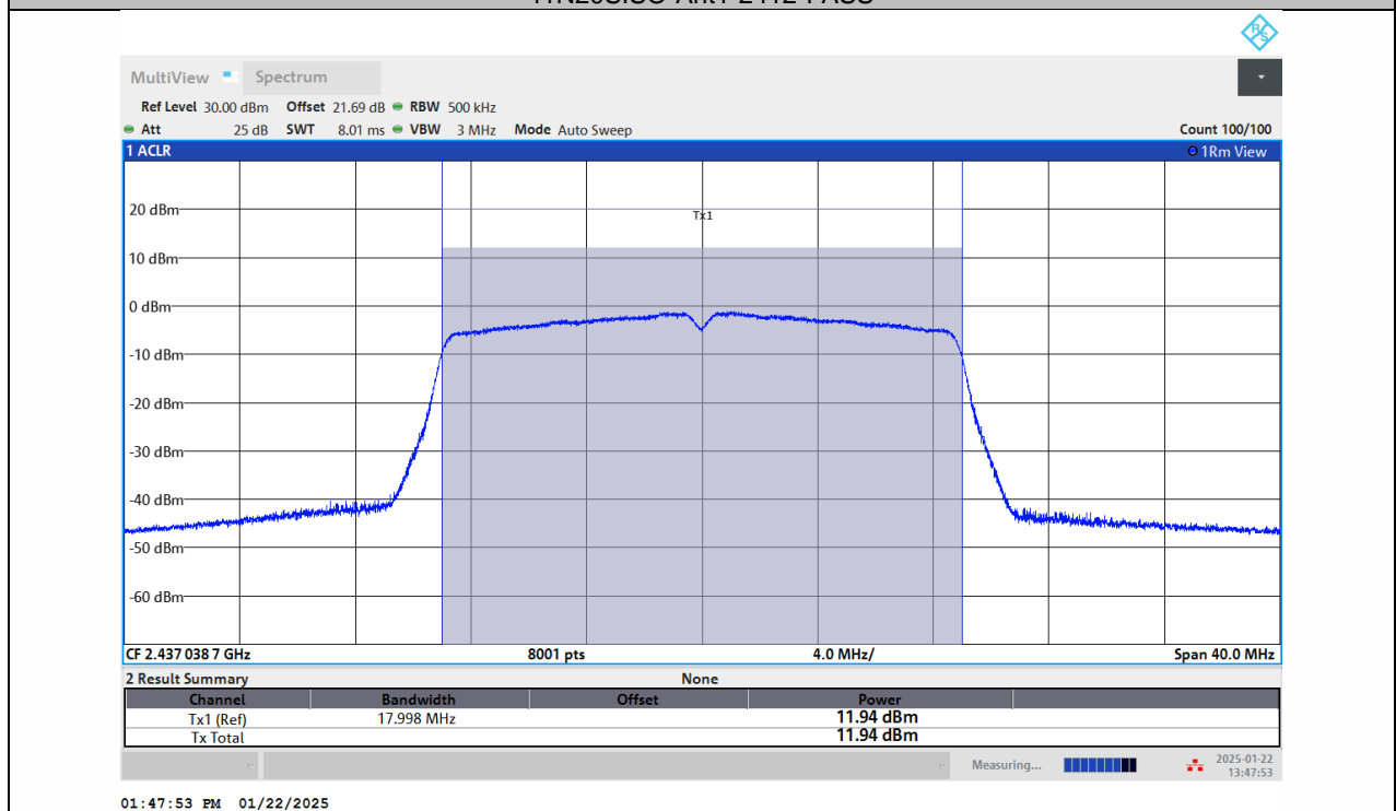
11N20SISO-Ant1-2437-PASS
