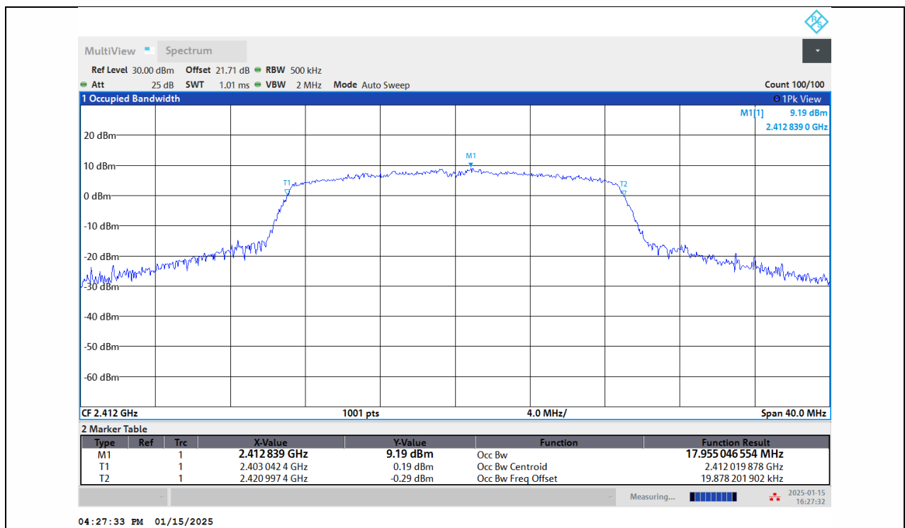
11N20SISO-Ant1-2412
