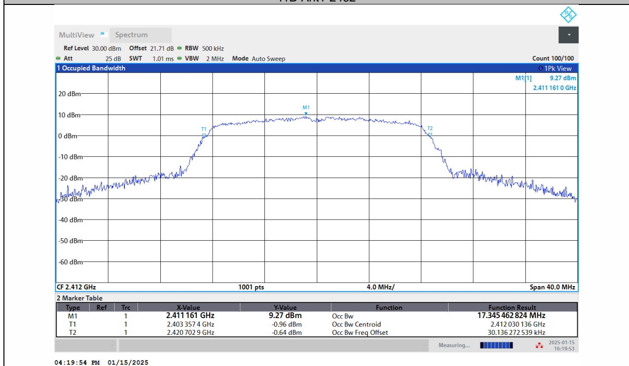
11G-Ant1-2412
