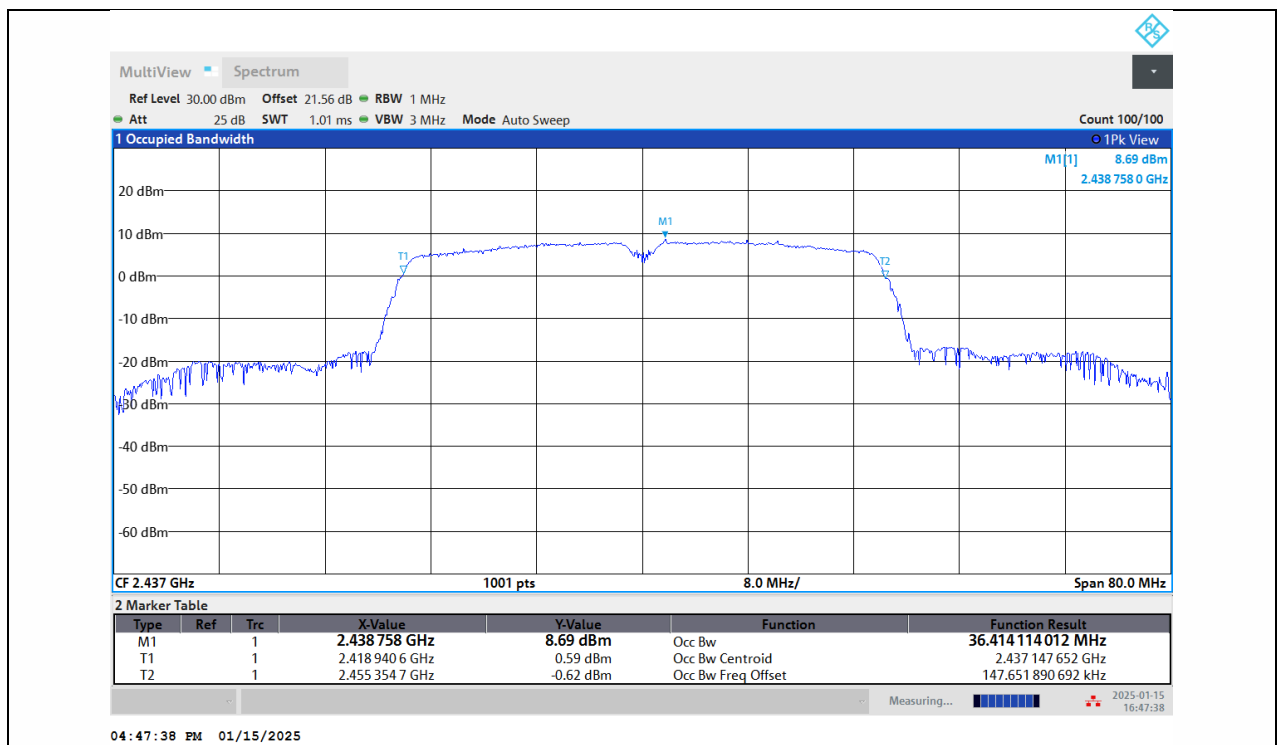
11N40SISO-Ant1-2437
