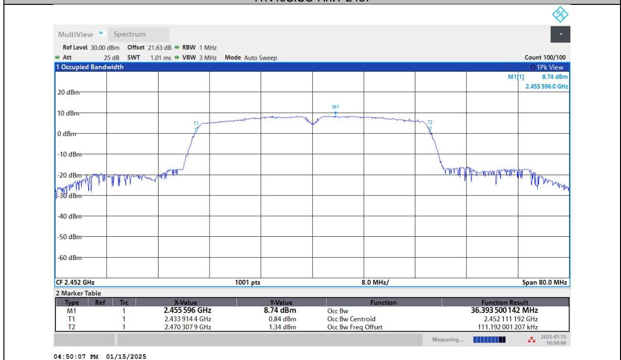
11N40SISO-Ant1-2452
