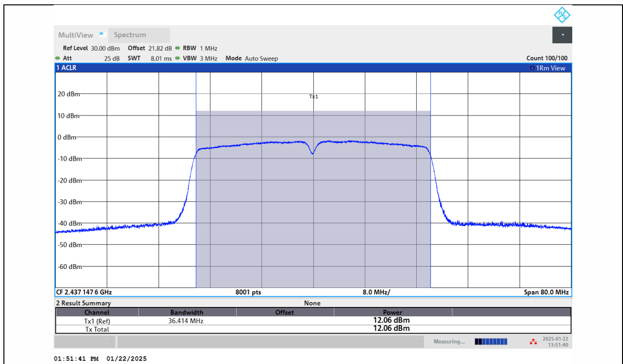
11N40SISO-Ant1-2437-PASS
