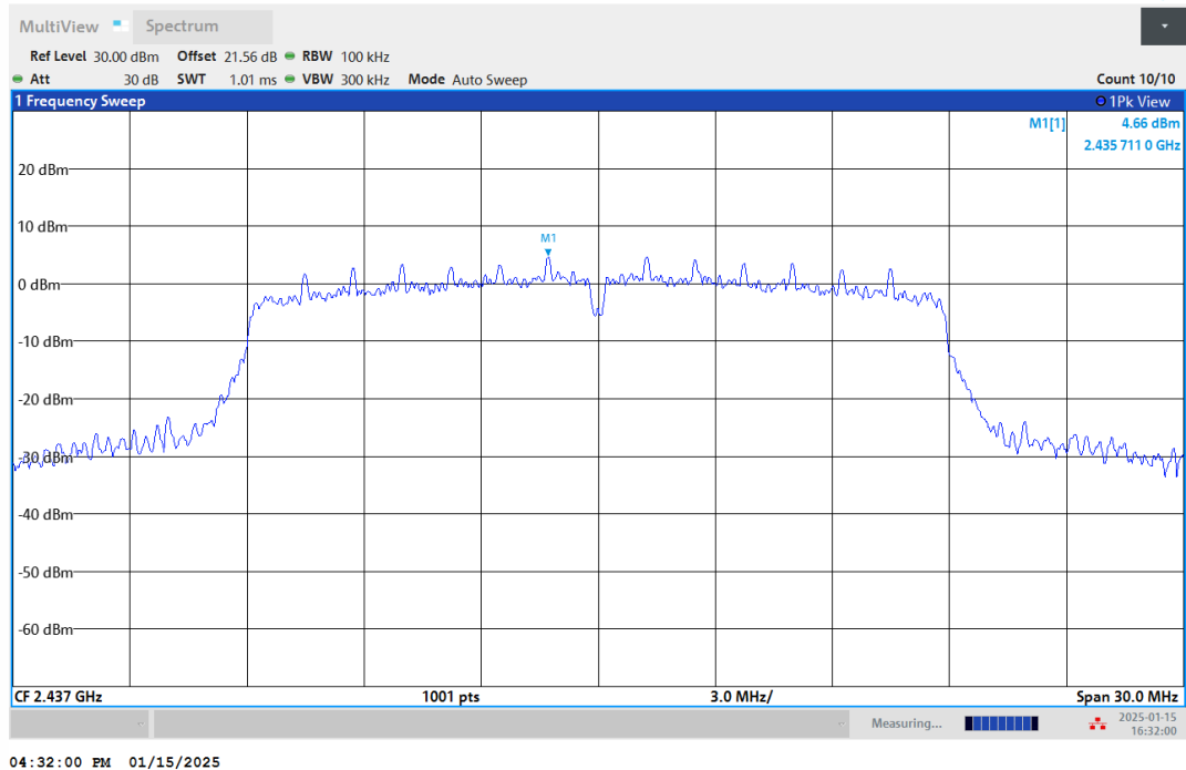
11N20SISO-Ant1-2437-0~Reference-PASS
