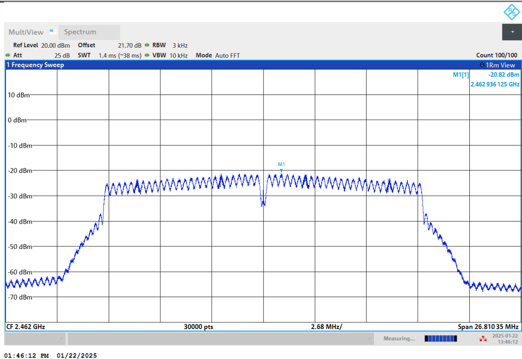
11G-Ant1-2462-PASS
