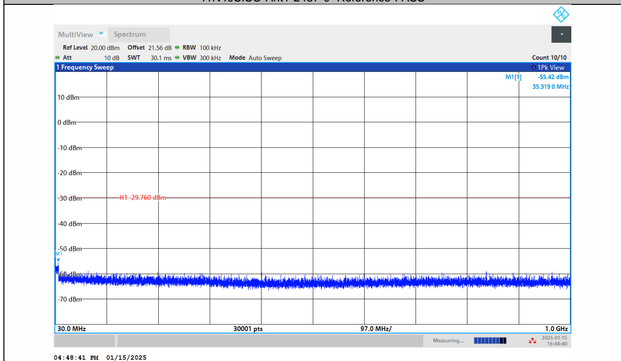
11N40SISO-Ant1-2437-30~1000-PASS
