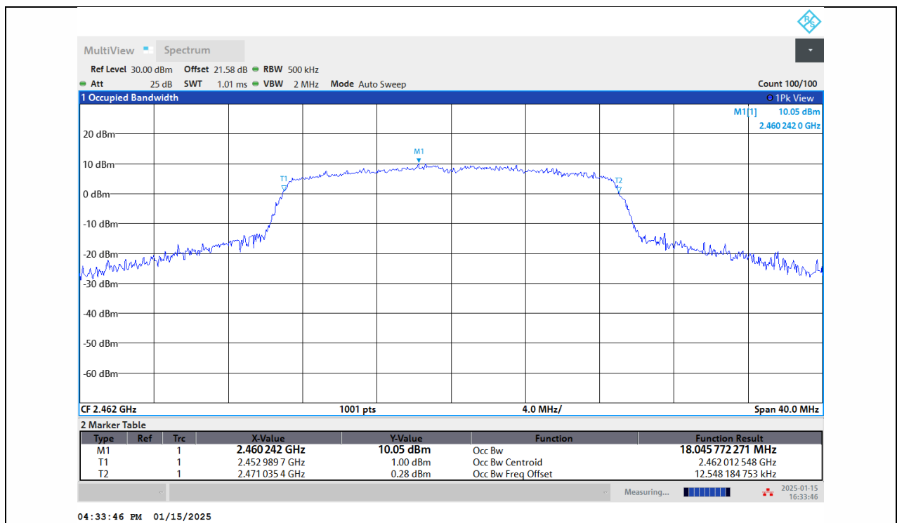
11N20SISO-Ant1-2462
