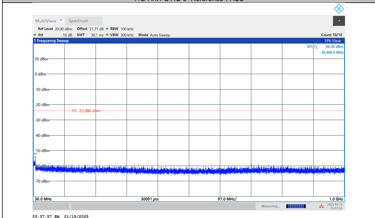
11B-Ant1-2412-30~1000-PASS
