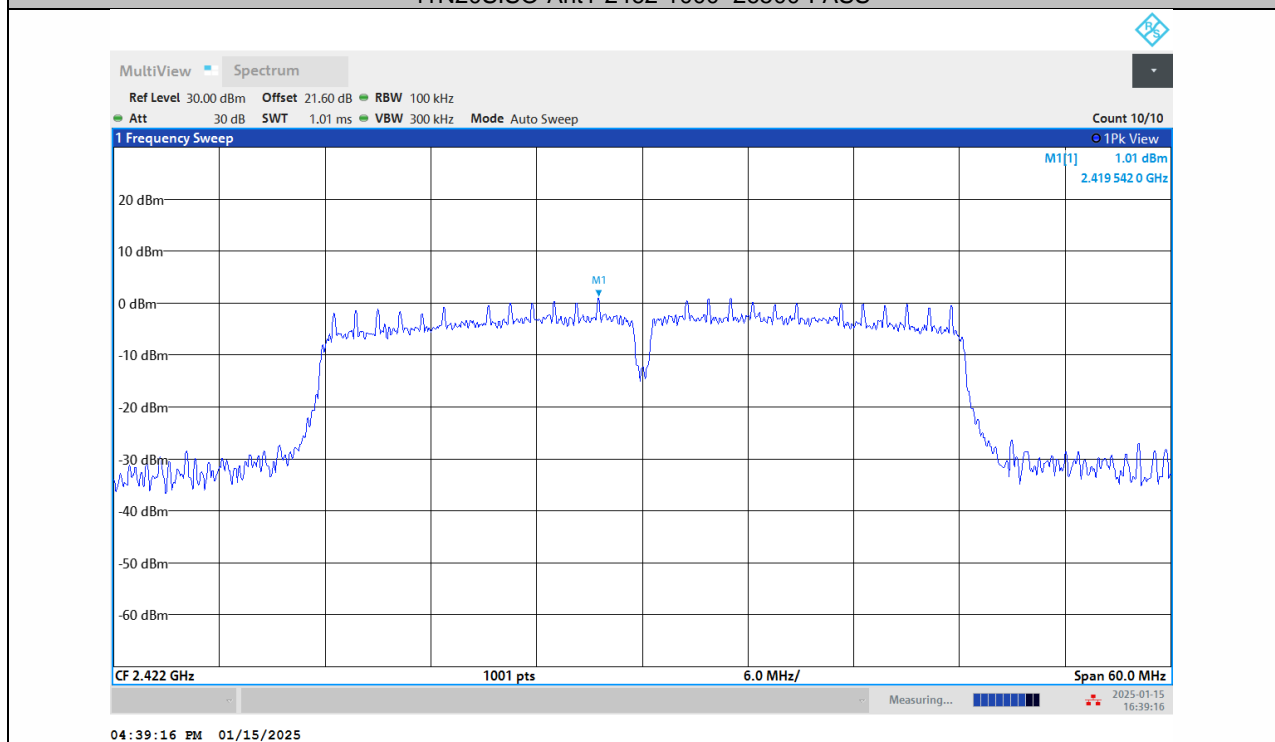
11N40SISO-Ant1-2422-0~Reference-PASS
