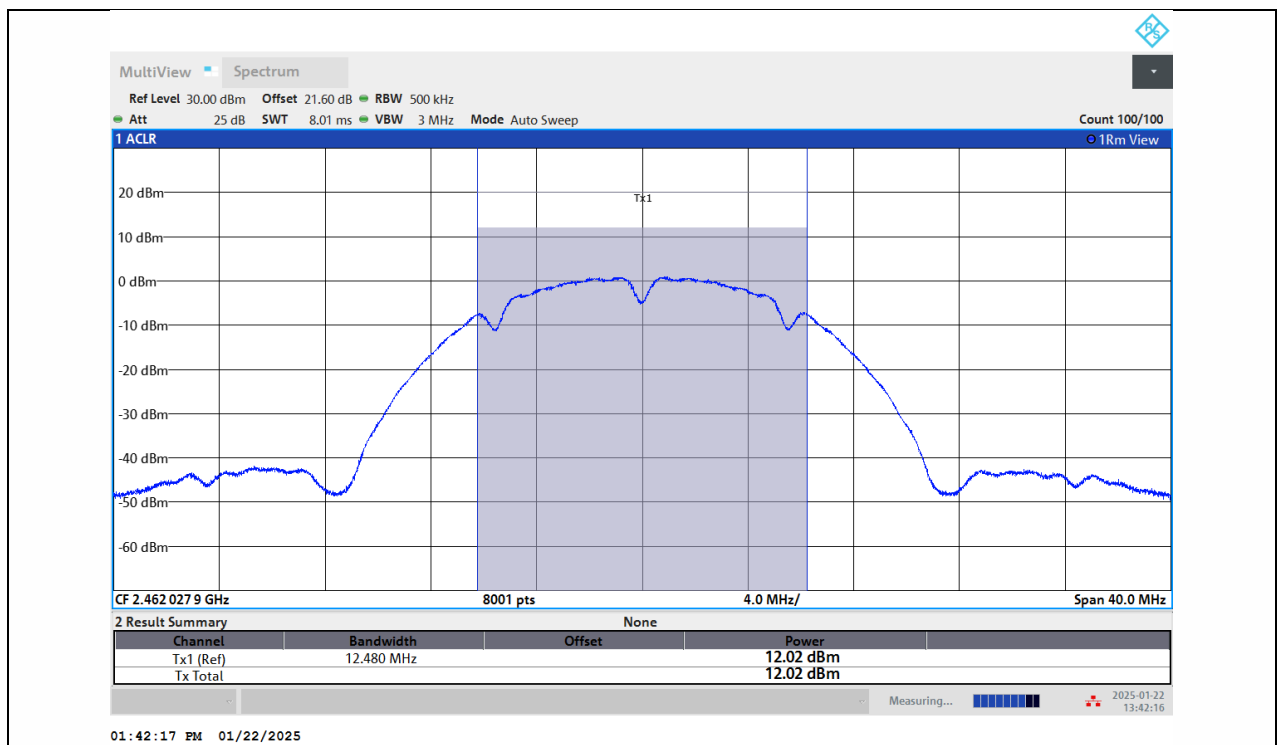
11B-Ant1-2462-PASS
