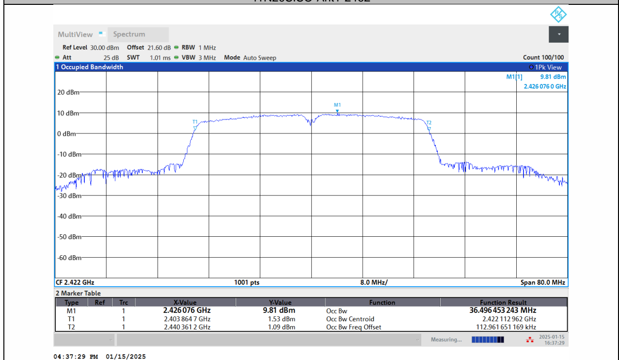
11N40SISO-Ant1-2422
