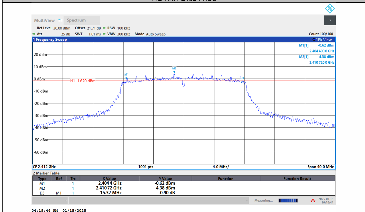
11G-Ant1-2412-PASS
