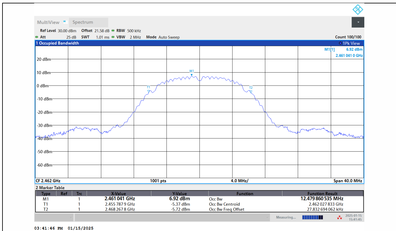
11B-Ant1-2462
