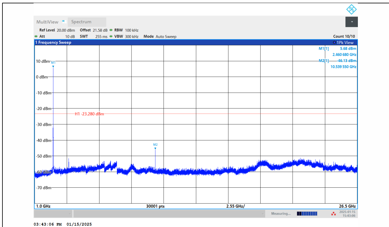
11B-Ant1-2462-1000~26500-PASS
