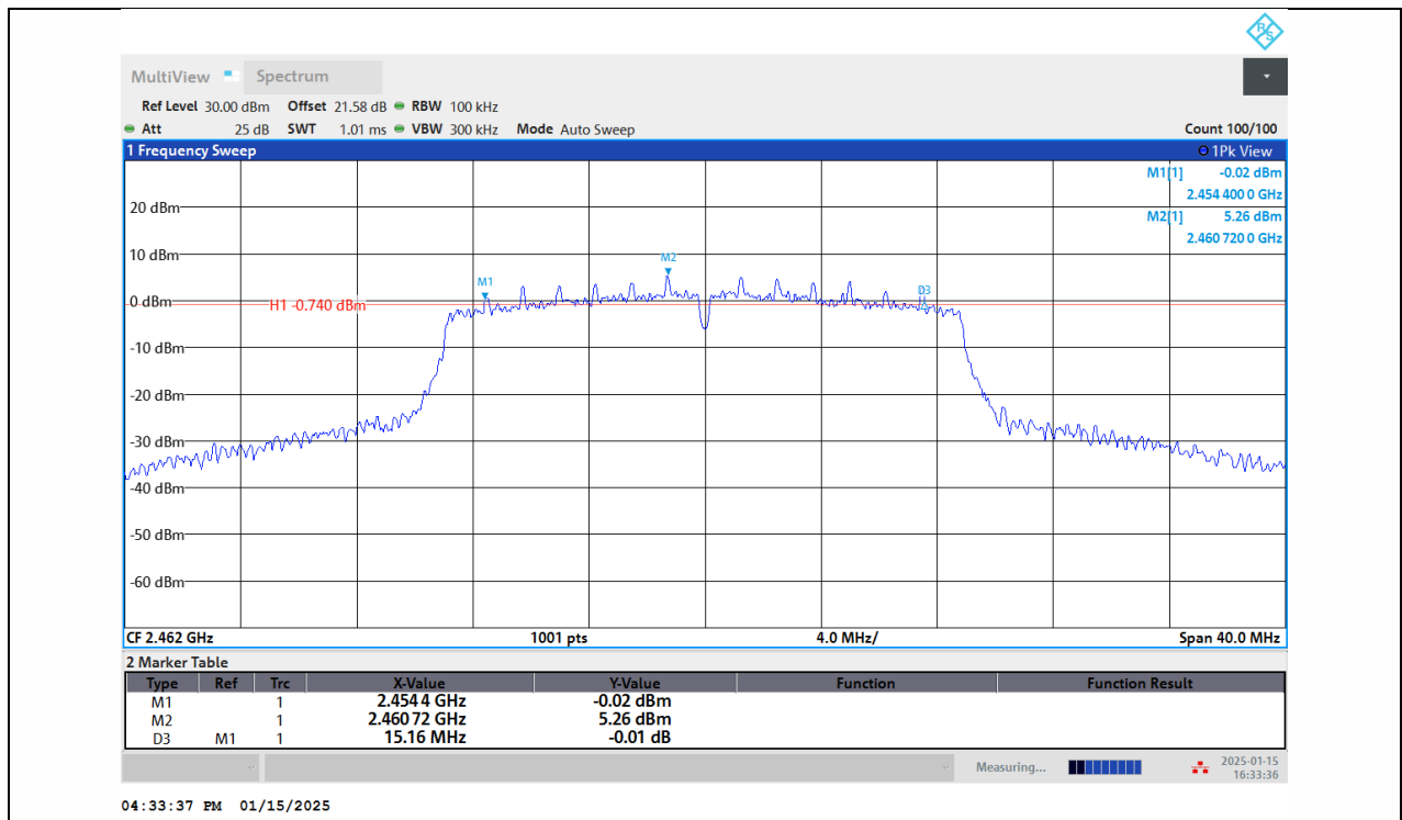
11N20SISO-Ant1-2462-PASS
