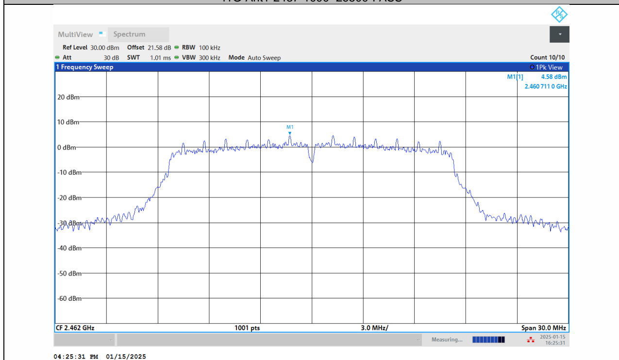
11G-Ant1-2462-0~Reference-PASS
