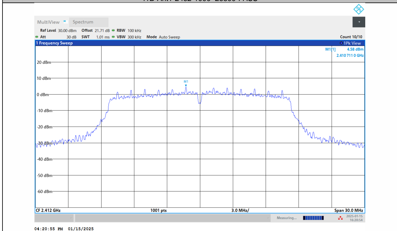
11G-Ant1-2412-0~Reference-PASS
