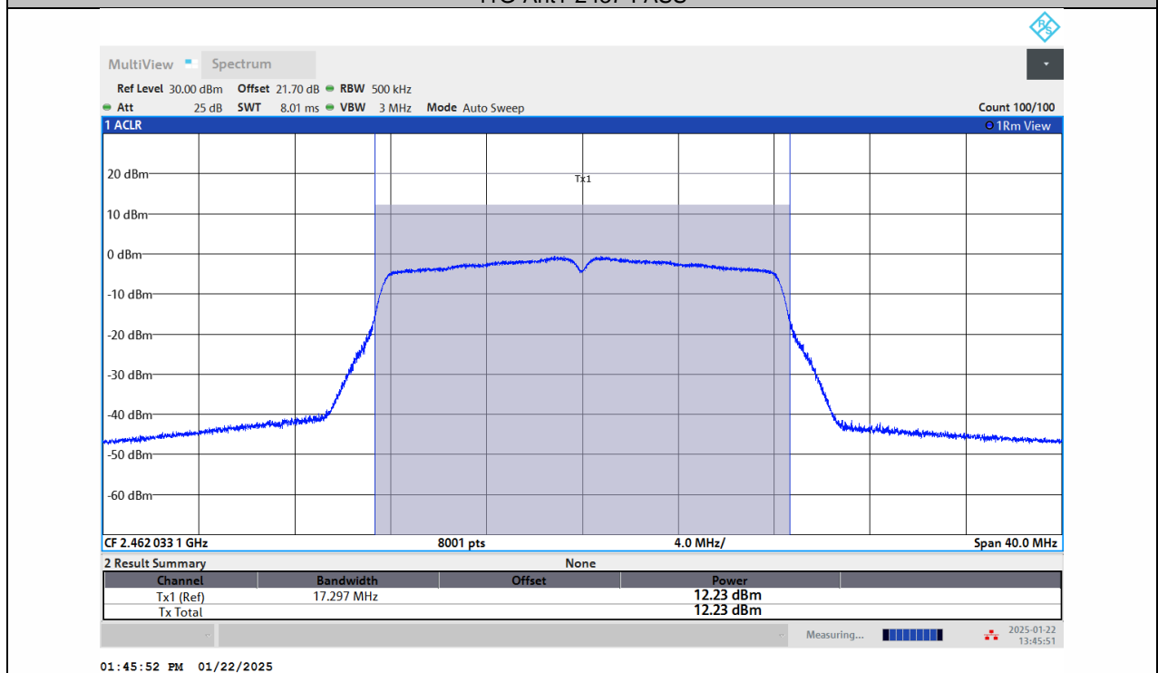
11G-Ant1-2462-PASS
