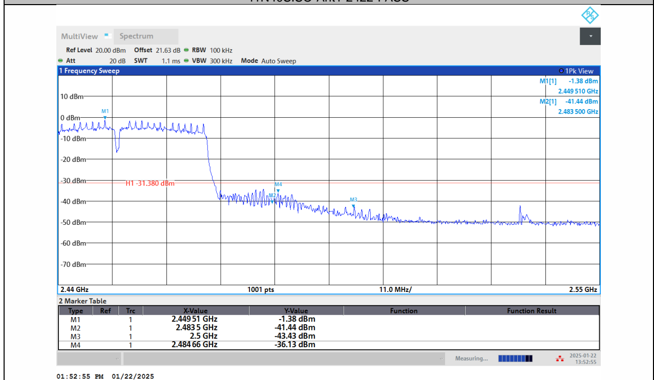
11N40SISO-Ant1-2452-PASS
