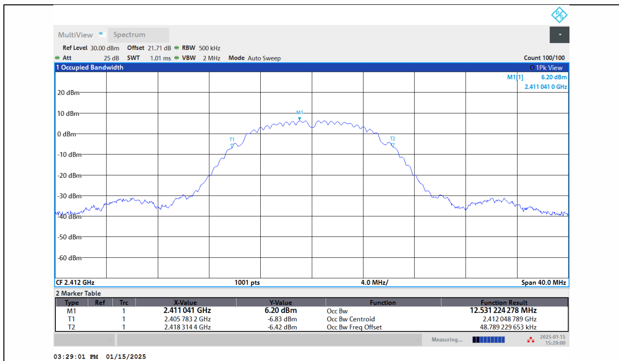
11B-Ant1-2412
