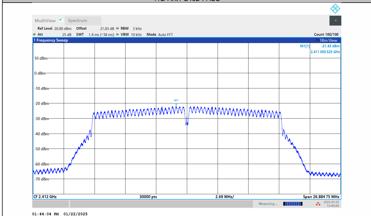
11G-Ant1-2412-PASS
