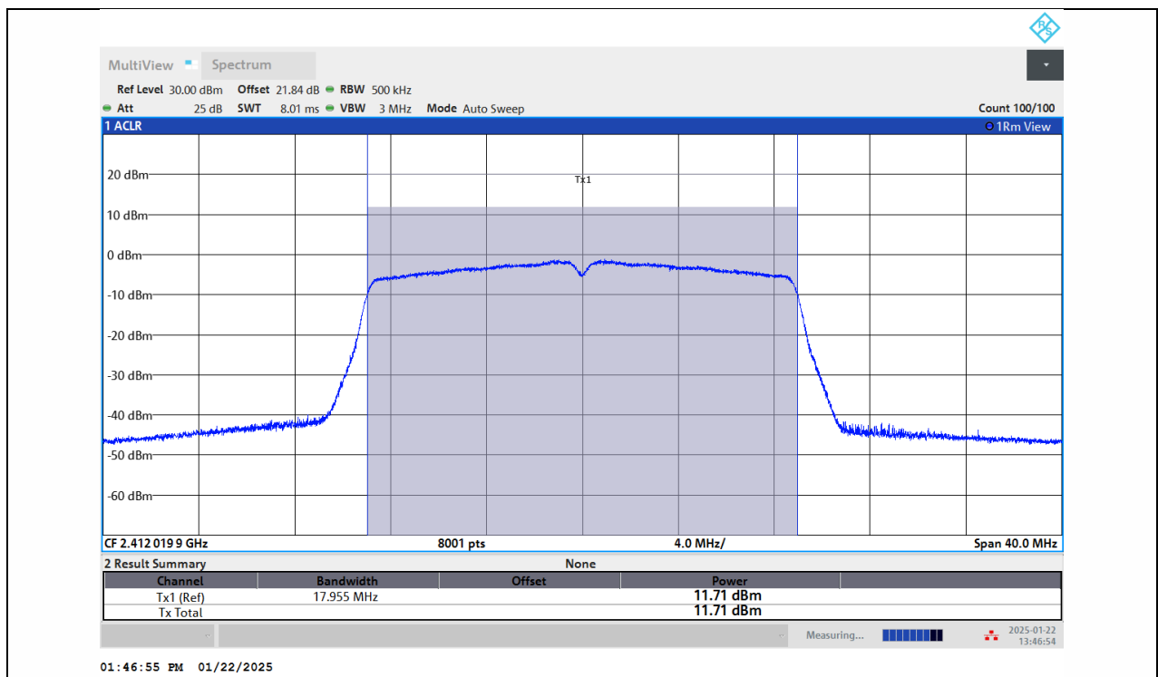
11N20SISO-Ant1-2412-PASS
