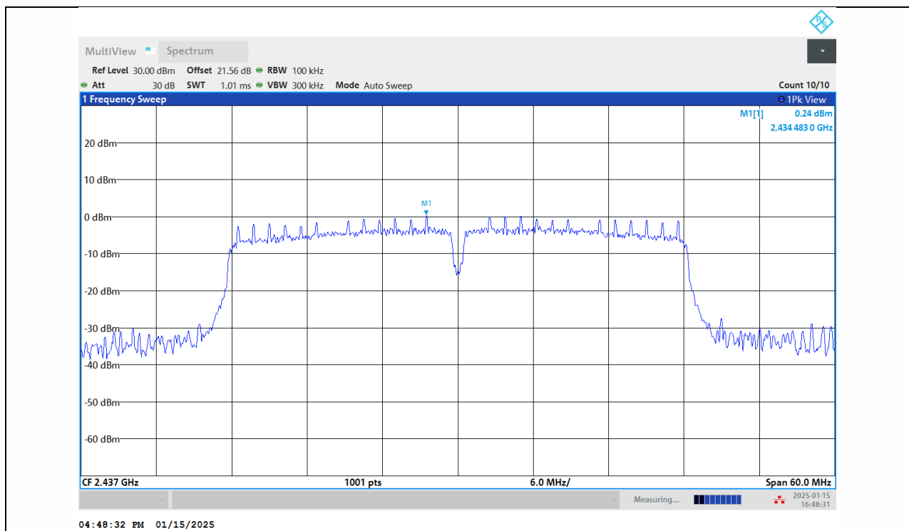
11N40SISO-Ant1-2437-0~Reference-PASS
