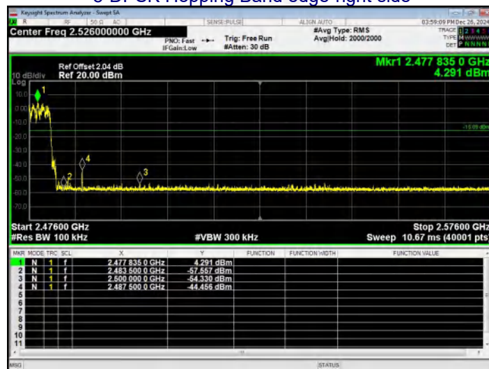
8-DPSK Hopping Band edge-right side
