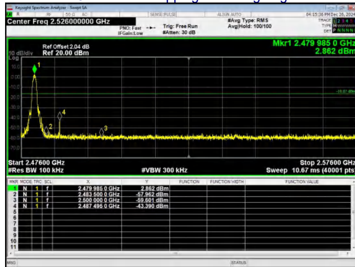
8-DPSK No-hopping Band edge-right side
