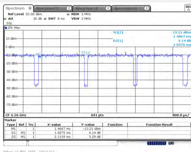
11a-5260 MHz
