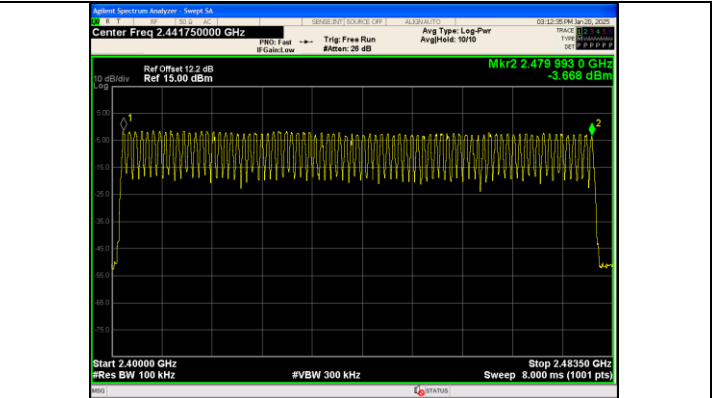
Hopping Plot 8DPSK
