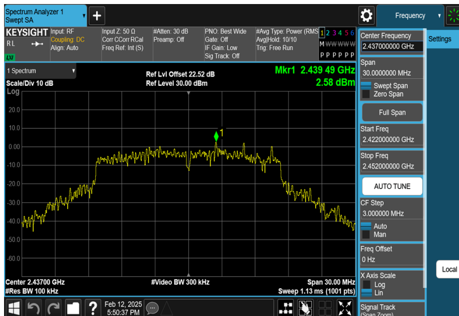
11G-Ant1-2437-0~Reference-PASS
