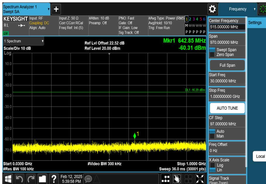
11B-Ant1-2437-30~1000-PASS
