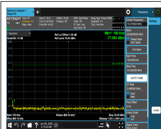
Band71_10MHz_QPSK_133422_1RB#0_0.15~30_0.15~30
