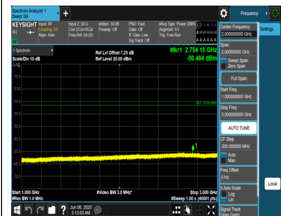
Band71_10MHz_QPSK_133422_1RB#0_1000~3_000_1000~3000
