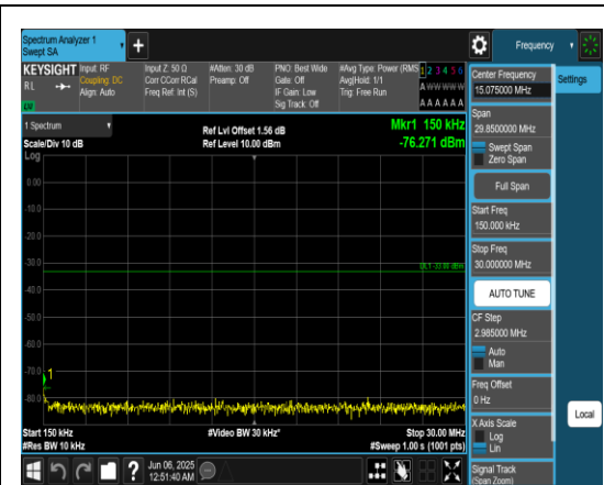
Band66_20MHz_QPSK_132572_1RB#0_0.15~30_0.15~30
