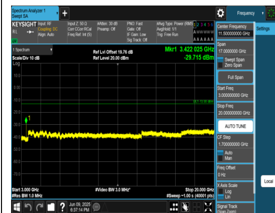
Band4_20MHz_QPSK_20050_1RB#0_3000~20000_00_3000~20000
