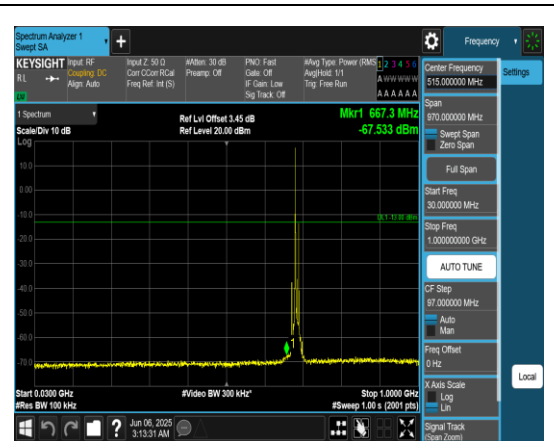
Band71_10MHz_QPSK_133422_1RB#0_30~100_0_30~1000
