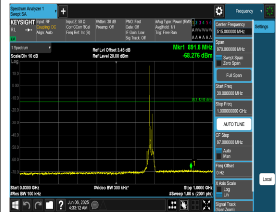
Band71_15MHz_QPSK_133397_1RB#0_30~1000_30~1000
