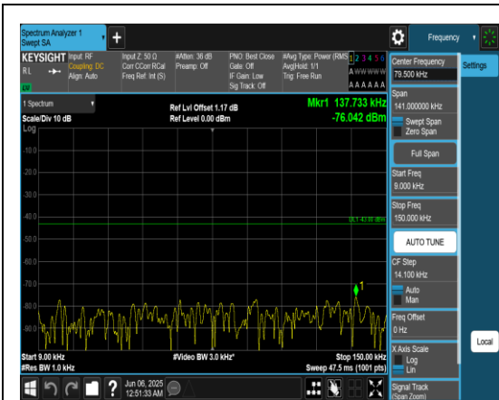
Band66_20MHz_QPSK_132572_1RB#0_0.009~0.15_0.009~0.15
