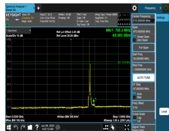
Band71_10MHz_QPSK_133172_1RB#0_30~100_30~1000
