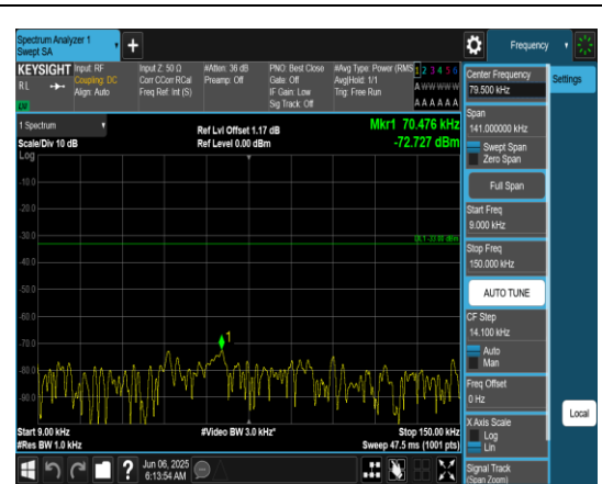
Band71_20MHz_QPSK_133322_1RB#0_0.009~0.15_0.009~0.15
