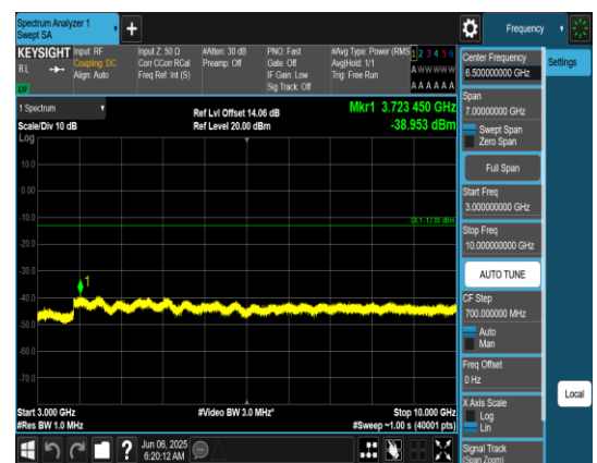
Band71_20MHz_QPSK_133372_1RB#0_3000~1_0000_3000~10000
