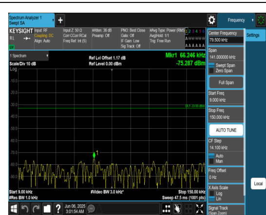
Band71_10MHz_QPSK_133172_1RB#0_0.009~0.15_0.009~0.15
