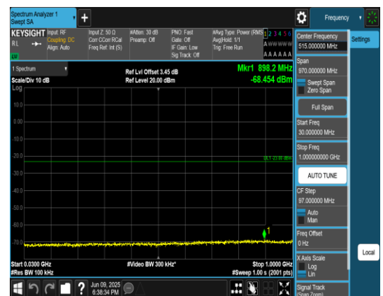
Band4_20MHz_QPSK_20175_1RB#0_30~1000_30~1000
