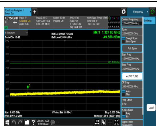
Band71_15MHz_QPSK_133197_1RB#0_1000~3 000_1000~3000
