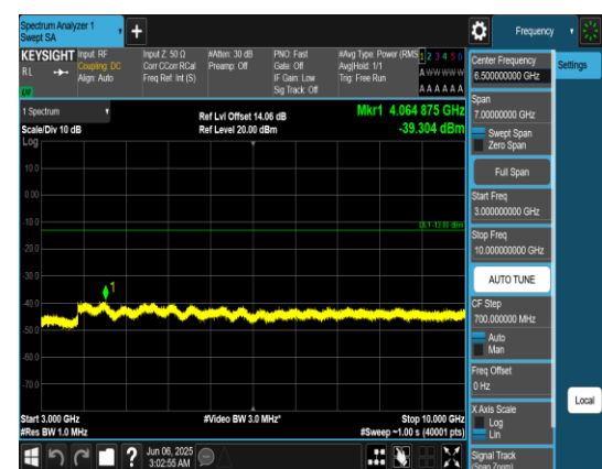
Band71_10MHz_QPSK_133172_1RB#0_3000~10000_3000~10000
