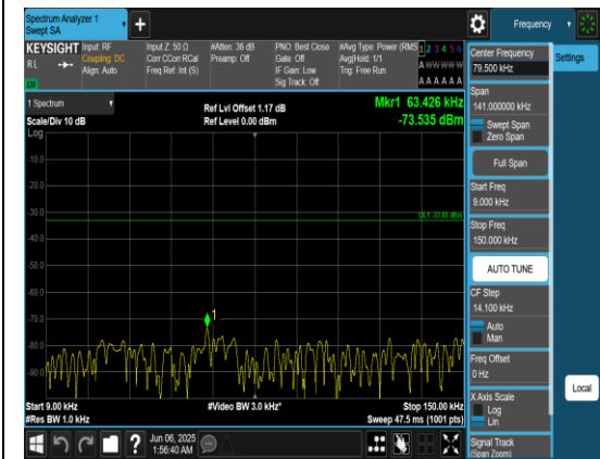
Band71_5MHz_QPSK_133447_1RB#0_0.009~0.15_15_0.009~0.15
