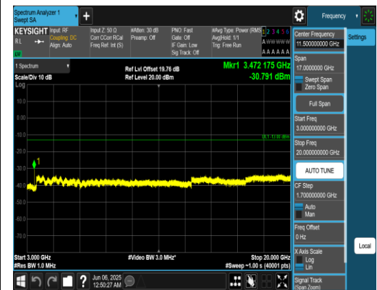
Band66_20MHz_QPSK_132322_1RB#0_3000~20000_0000_3000~20000
