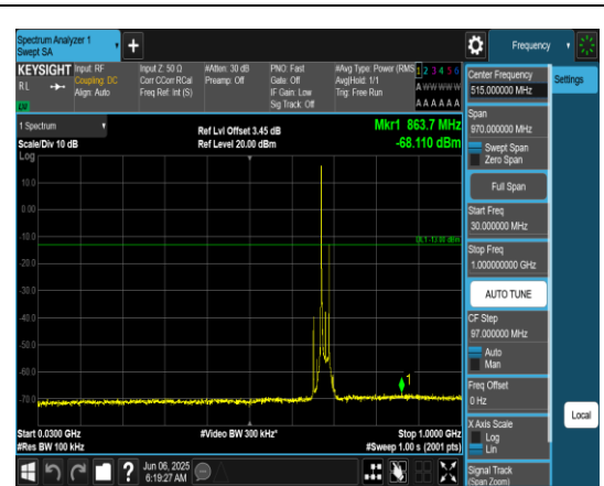
Band71_20MHz_QPSK_133372_1RB#0_30~100_0_30~1000
