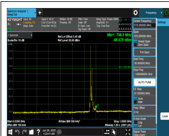
Band71_15MHz_QPSK_133197_1RB#0_30~100 0_30~1000
