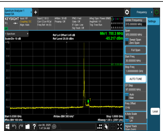
Band71_5MHz_QPSK_133147_1RB#0_30~1000_30~1000
