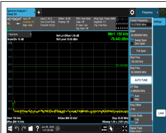
Band71_5MHz_QPSK_133147_1RB#0_0.15~30_0.15~30
