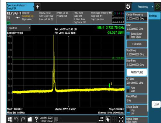
Band66_20MHz_QPSK_132322_1RB#0_1000~3000_000_1000~3000
