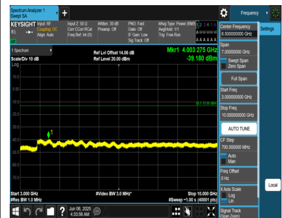
Band71_15MHz_QPSK_133397_1RB#0_3000~10000_3000~10000
