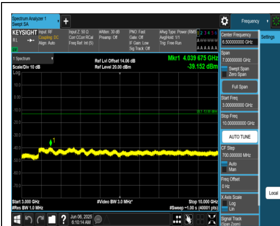
Band71_20MHz_QPSK_133222_1RB#0_3000~10000_3000~10000
