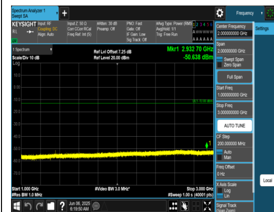
Band71_20MHz_QPSK_133372_1RB#0_1000~3_000_1000~3000
