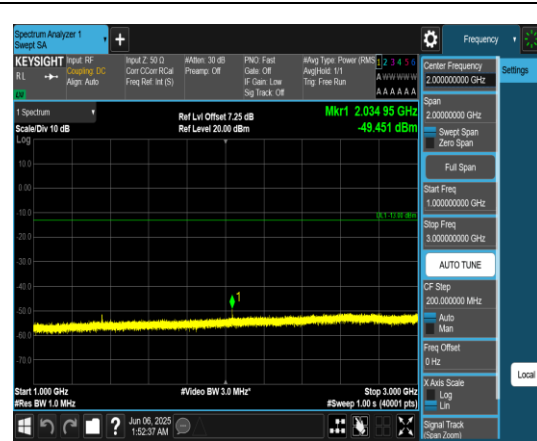
Band71_5MHz_QPSK_133297_1RB#0_1000~30_00_1000~3000
