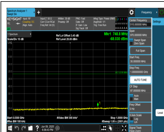
Band4_20MHz_QPSK_20050_1RB#0_30~1000_30~1000
