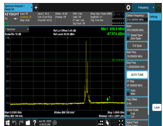
Band71_15MHz_QPSK_133297_1RB#0_30~100 0_30~1000
