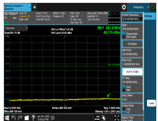
Band4_20MHz_QPSK_20300_1RB#0_30~1000_30~1000
