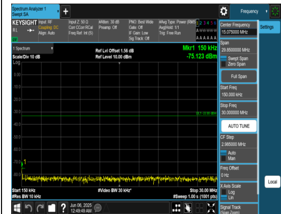
Band66_20MHz_QPSK_132322_1RB#0_0.15~30_0.15~30
