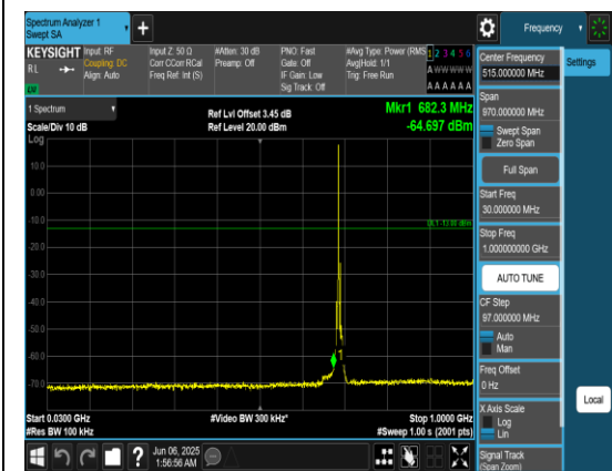
Band71_5MHz_QPSK_133447_1RB#0_30~1000_30~1000
