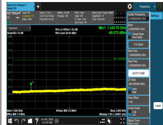
Band71_5MHz_QPSK_133147_1RB#0_1000~3000_1000~3000
