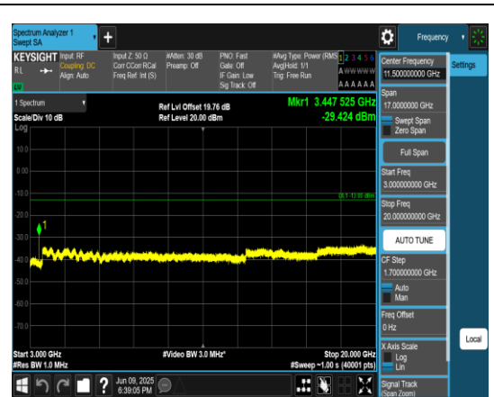
Band4_20MHz_QPSK_20175_1RB#0_3000~20000_00_3000~20000
