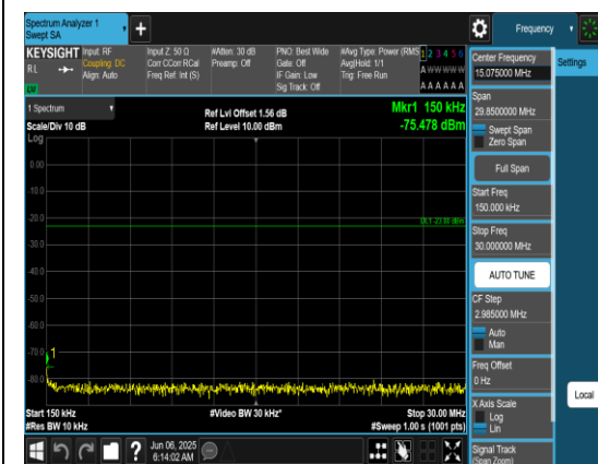
Band71_20MHz_QPSK_133322_1RB#0_0.15~30_0.15~30
