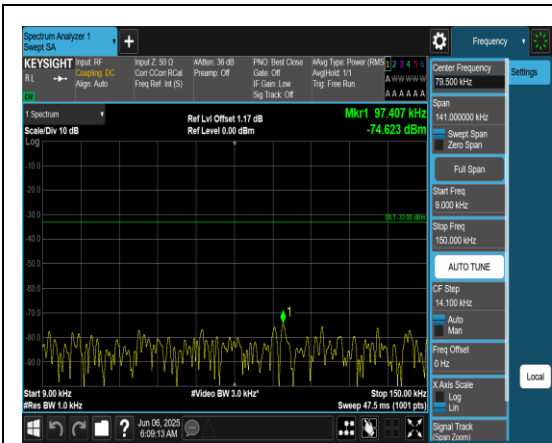
Band71_20MHz_QPSK_133222_1RB#0_0.009~0.15_0.009~0.15
