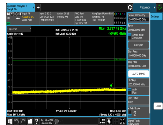
Band71_15MHz_QPSK_133397_1RB#0_1000~3000_1000~3000
