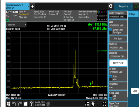
Band71_20MHz_QPSK_133222_1RB#0_30~100_30~1000
