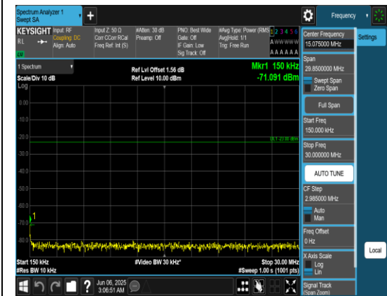
Band71_10MHz_QPSK_133297_1RB#0_0.15~30_0.15~30
