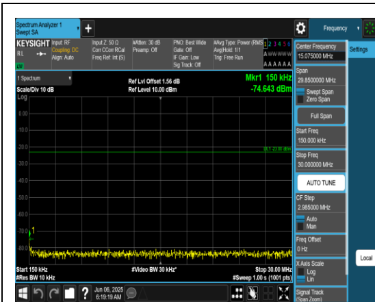
Band71_20MHz_QPSK_133372_1RB#0_0.15~30_0.15~30
