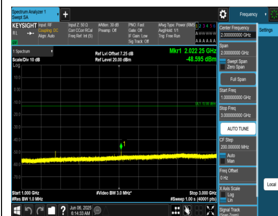
Band71_20MHz_QPSK_133322_1RB#0_1000~3000_1000~3000
