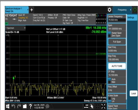
Band71_15MHz_QPSK_133397_1RB#0_0.009~0.15_0.009~0.15
