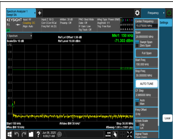
Band71_20MHz_QPSK_133222_1RB#0_0.15~30_0.15~30
