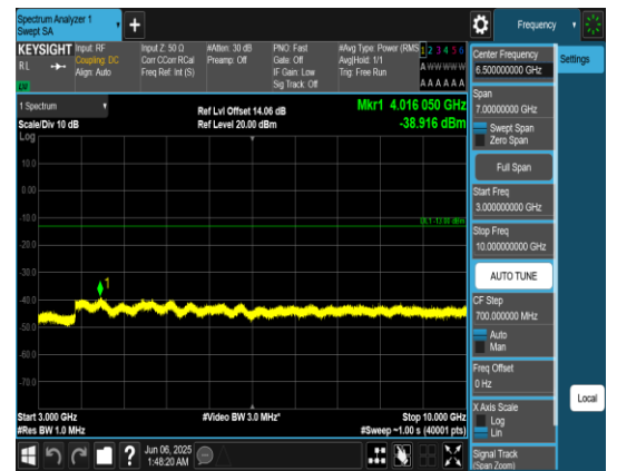
Band71_5MHz_QPSK_133147_1RB#0_3000~10000_3000~10000
