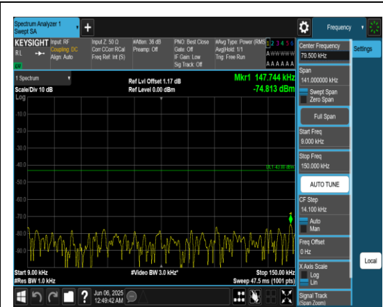
Band66_20MHz_QPSK_132322_1RB#0_0.009~0.15_0.009~0.15
