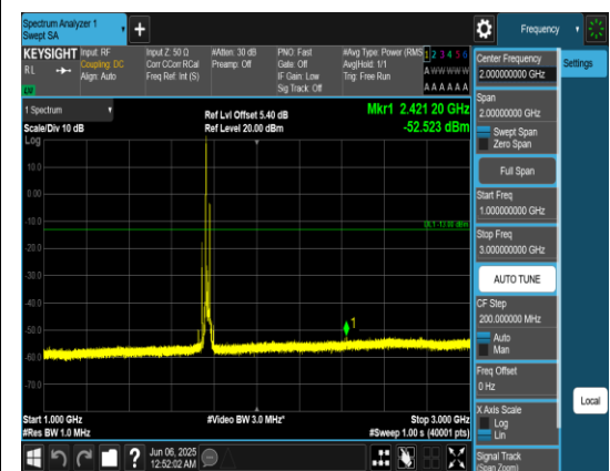
Band66_20MHz_QPSK_132572_1RB#0_1000~3000_1000~3000
