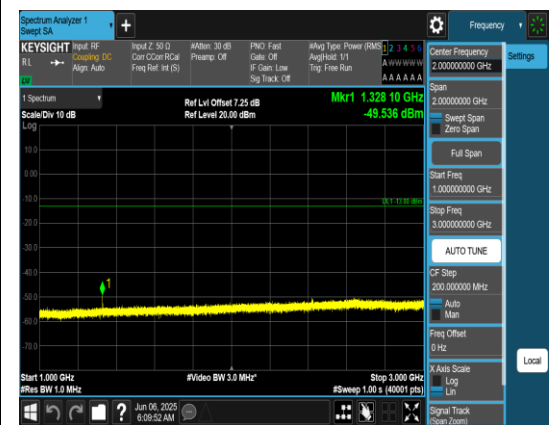
Band71_20MHz_QPSK_133222_1RB#0_1000~3000_1000~3000
