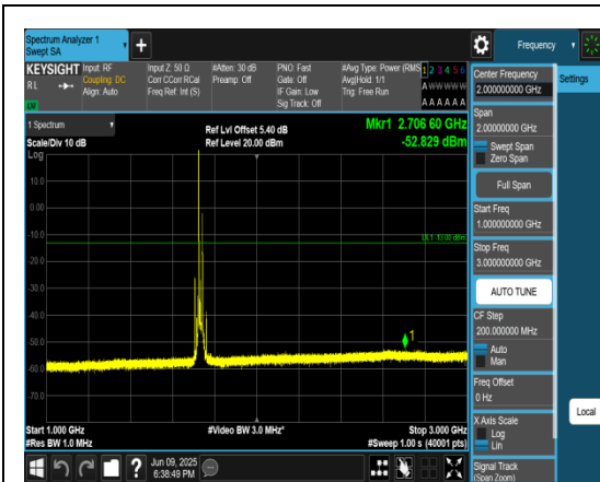
Band4_20MHz_QPSK_20175_1RB#0_1000~3000_1000~3000
