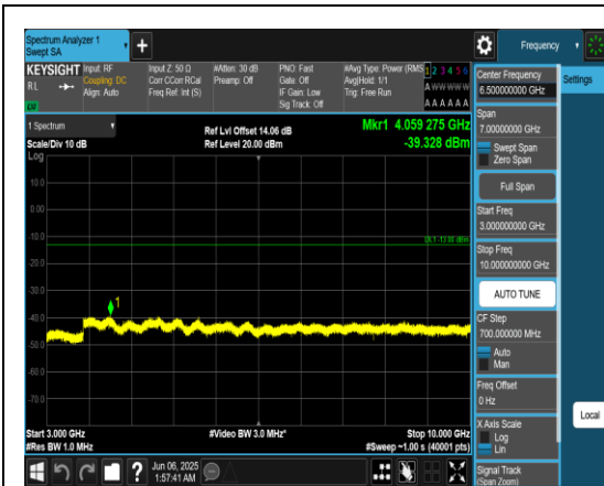
Band71_5MHz_QPSK_133447_1RB#0_3000~10000_3000~10000
