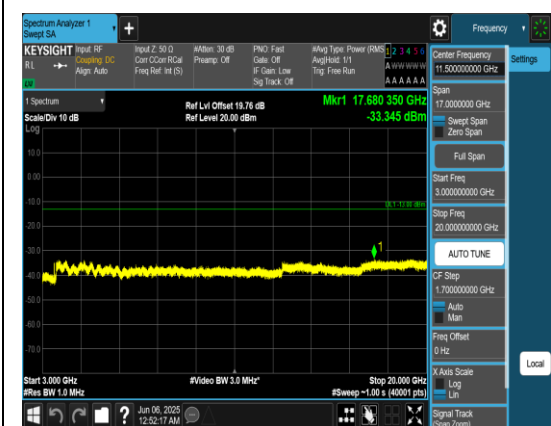
Band66_20MHz_QPSK_132572_1RB#0_3000~20000_0000_3000~20000
