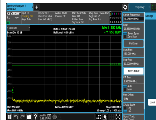
Band4_20MHz_QPSK_20175_1RB#0_0.15~30_0.15~30
