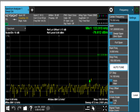
Band71_10MHz_QPSK_133297_1RB#0_0.009~0.15_0.009~0.15
