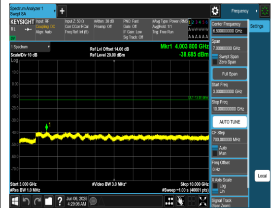
Band71_15MHz_QPSK_133297_1RB#0_3000~10000_3000~10000
