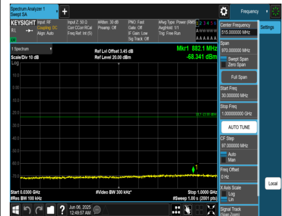
Band66_20MHz_QPSK_132322_1RB#0_30~100_30~1000
