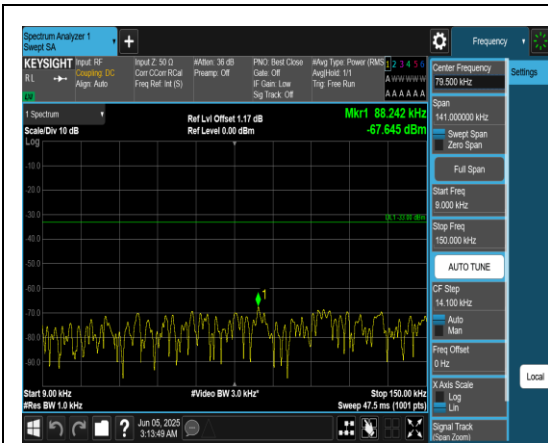
Band13_10MHz_QPSK_23230_1RB#0_0.009~0.15_0.009~0.15
