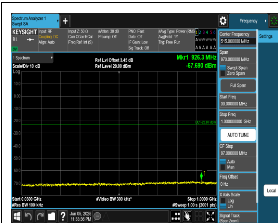
Band66_15MHz_QPSK_132322_1RB#0_30~100 0_30~1000
