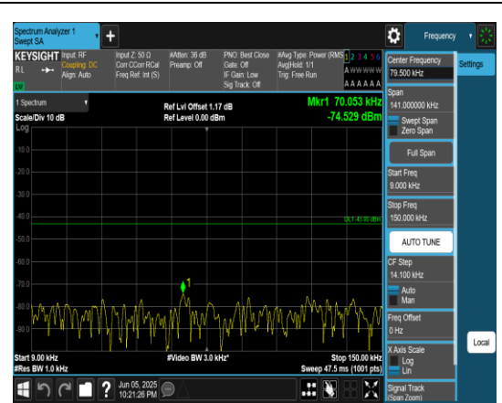
Band66_10MHz_QPSK_132322_1RB#0_0.009~0.15_0.009~0.15
