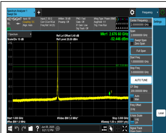
Band66_5MHz_QPSK_132647_1RB#0_1000~3000_1000~3000
