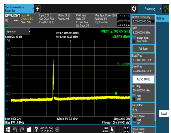
Band66_10MHz_QPSK_132022_1RB#0_1000~3000_000_1000~3000
