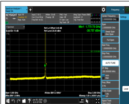
Band66_1.4MHz_QPSK_132665_1RB#0_1000~3000_1000~3000
