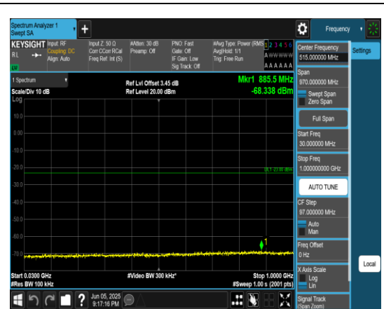
Band66_5MHz_QPSK_131997_1RB#0_30~1000_30~1000
