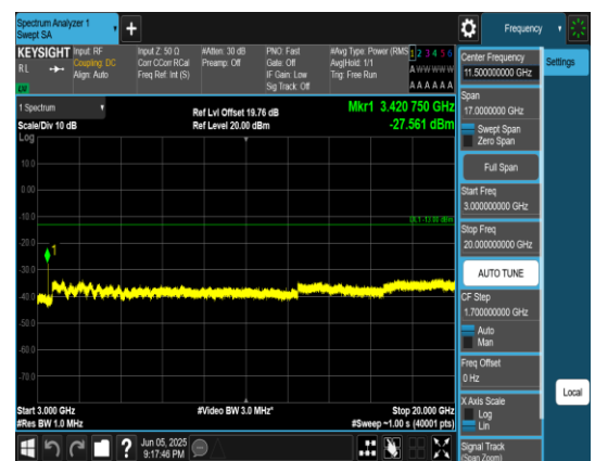
Band66_5MHz_QPSK_131997_1RB#0_3000~20000_3000~20000
