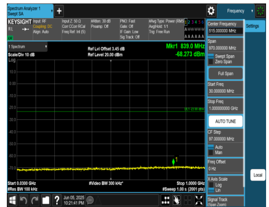
Band66_10MHz_QPSK_132322_1RB#0_30~100_30~1000
