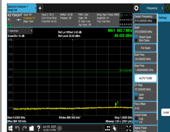
Band66_10MHz_QPSK_132622_1RB#0_30~100_0_30~1000
