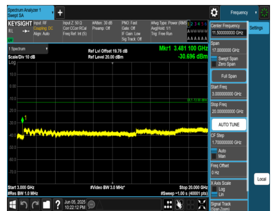
Band66_10MHz_QPSK_132322_1RB#0_3000~20000_3000~20000
