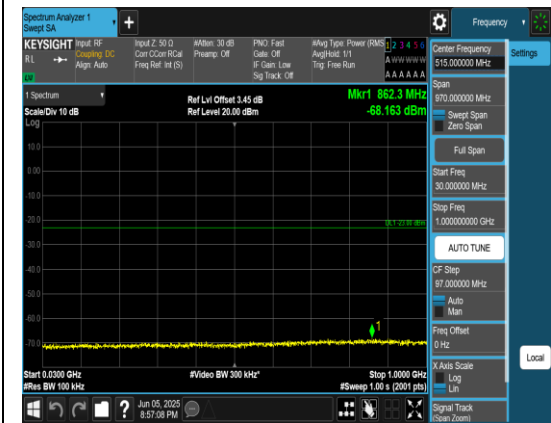
Band66_3MHz_QPSK_132657_1RB#0_30~1000_30~1000
