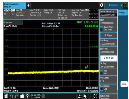
Band13_10MHz_QPSK_23230_1RB#0_1000~30_00_1000~3000
