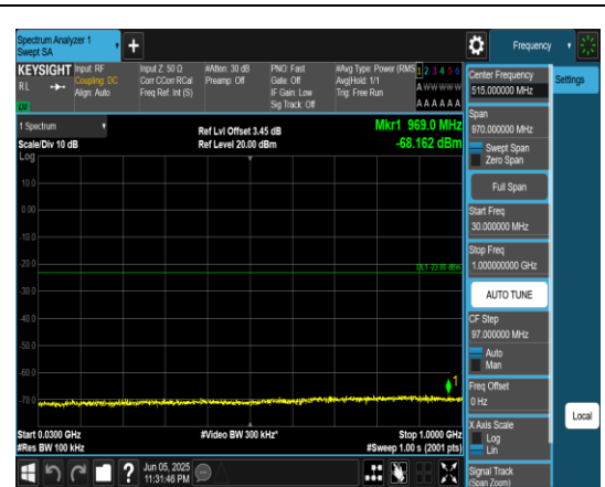
Band66_15MHz_QPSK_132047_1RB#0_30~100 0_30~1000
