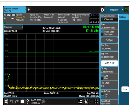
Band13_10MHz_QPSK_23230_1RB#0_0.15~30_0.15~30
