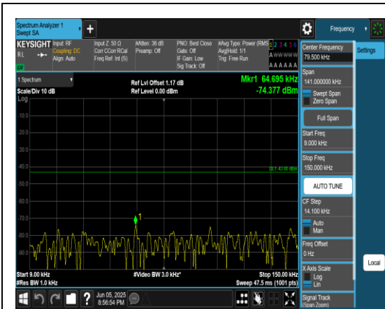
Band66_3MHz_QPSK_132657_1RB#0_0.009~0.15_0.009~0.15
