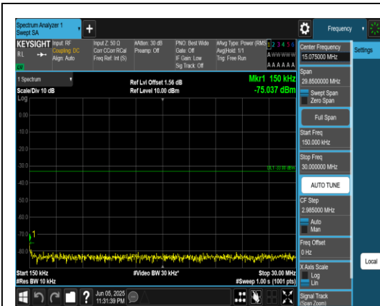
Band66_15MHz_QPSK_132047_1RB#0_0.15~30 _0.15~30
