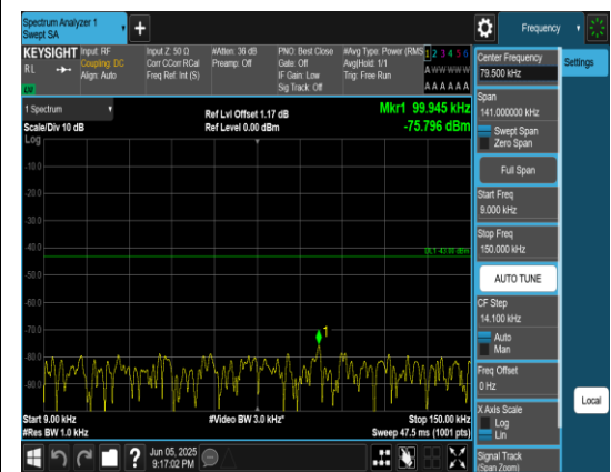
Band66_5MHz_QPSK_131997_1RB#0_0.009~0.15_0.009~0.15
