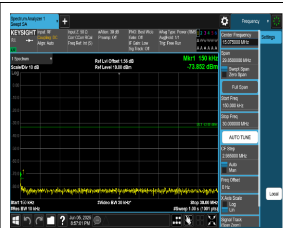
Band66_3MHz_QPSK_132657_1RB#0_0.15~30_0.15~30
