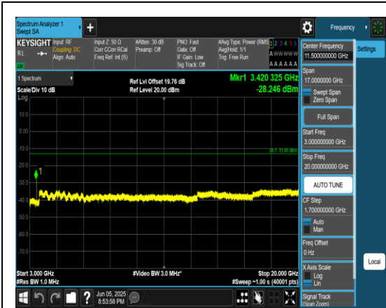
Band66_3MHz_QPSK_131987_1RB#0_3000~20000_3000~20000
