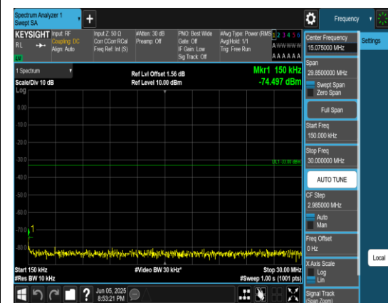
Band66_3MHz_QPSK_131987_1RB#0_0.15~30_0.15~30
