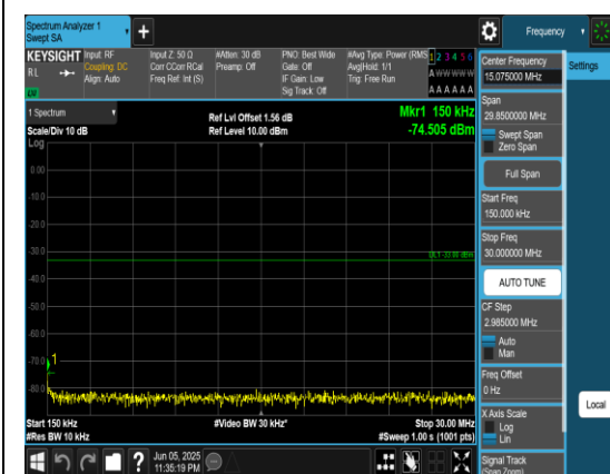
Band66_15MHz_QPSK_132597_1RB#0_0.15~30 _0.15~30
