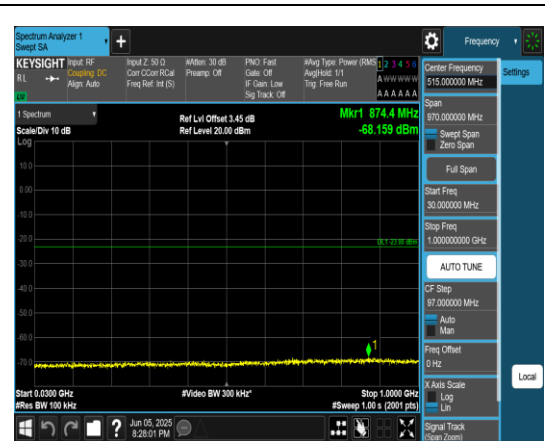
Band66_1.4MHz_QPSK_131979_1RB#0_30~100 0_30~1000
