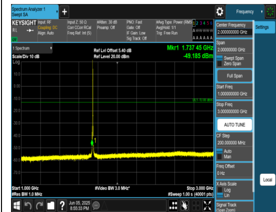
Band66_3MHz_QPSK_132322_1RB#0_1000~3000_00_1000~3000
