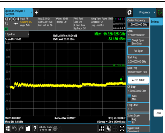
Band66_5MHz_QPSK_132647_1RB#0_3000~20000_000_3000~20000
