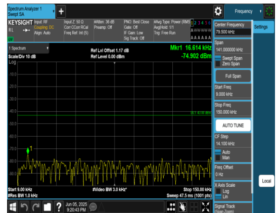
Band66_5MHz_QPSK_132647_1RB#0_0.009~0.15_0.009~0.15
