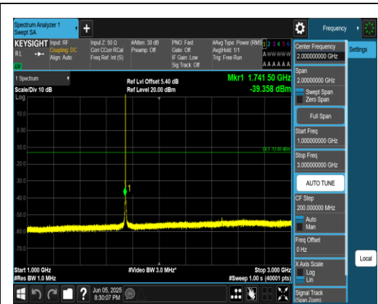
Band66_1.4MHz_QPSK_132322_1RB#0_1000~3 000_1000~3000
