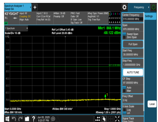
Band66_5MHz_QPSK_132647_1RB#0_30~1000_30~1000
