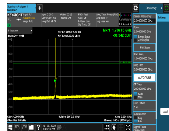
Band66_1.4MHz_QPSK_131979_1RB#0_1000~3 000_1000~3000
