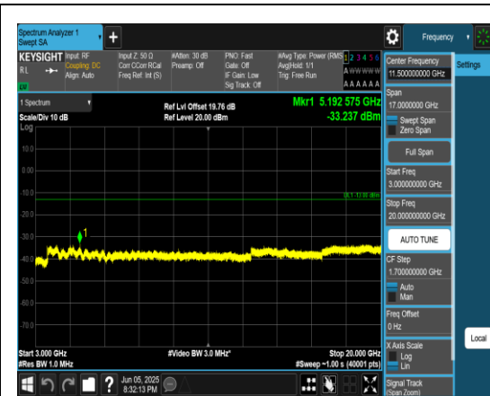
Band66_1.4MHz_QPSK_132665_1RB#0_3000~20000_0000_3000~20000
