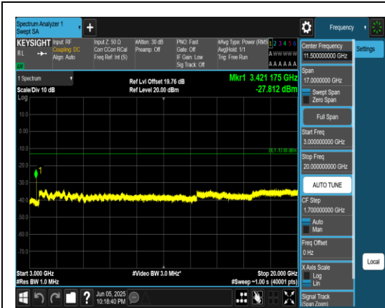
Band66_10MHz_QPSK_132022_1RB#0_3000~20000_3000~20000
