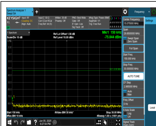
Band66_1.4MHz_QPSK_131979_1RB#0_0.15~3 0_0.15~30
