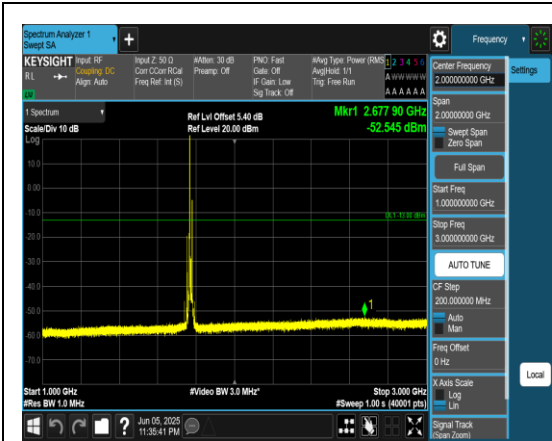
Band66_15MHz_QPSK_132597_1RB#0_1000~3000_1000~3000
