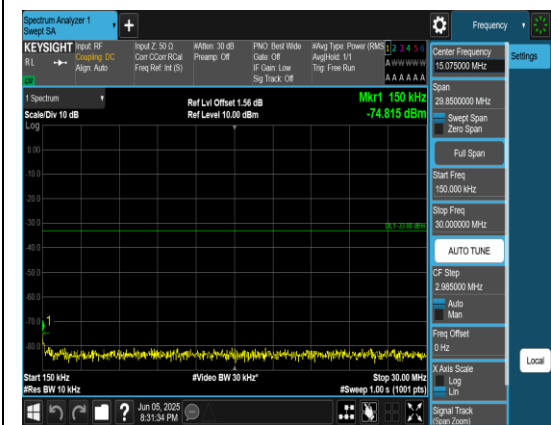
Band66_1.4MHz_QPSK_132665_1RB#0_0.15~3 0_0.15~30
