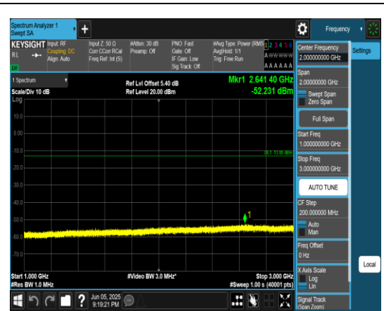
Band66_5MHz_QPSK_132322_1RB#0_1000~3000_00_1000~3000
