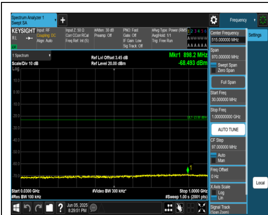
Band66_1.4MHz_QPSK_132322_1RB#0_30~100 0_30~1000
