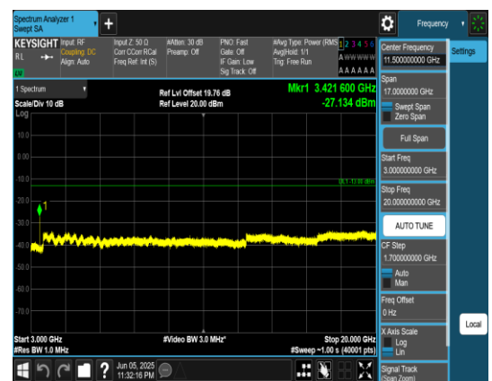
Band66_15MHz_QPSK_132047_1RB#0_3000~2 0000_3000~20000
