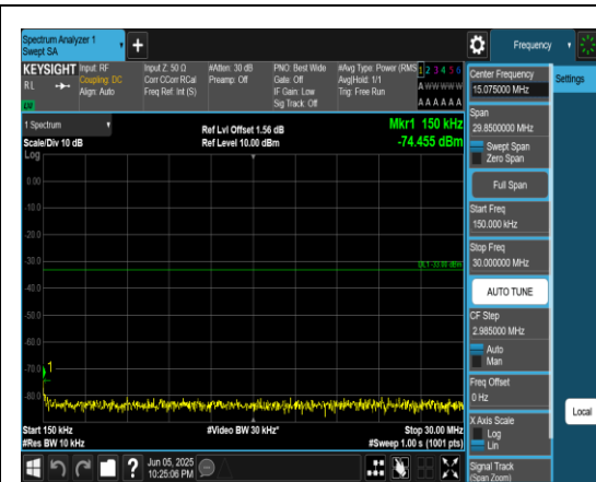
Band66_10MHz_QPSK_132622_1RB#0_0.15~30_0.15~30
