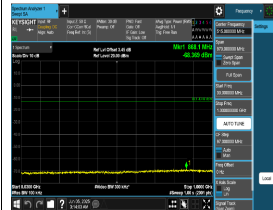
Band13_10MHz_QPSK_23230_1RB#0_30~1000_30~1000
