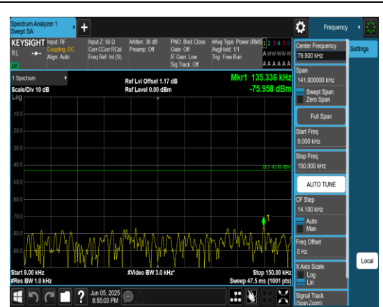
Band66_3MHz_QPSK_132322_1RB#0_0.009~0.15_0.009~0.15
