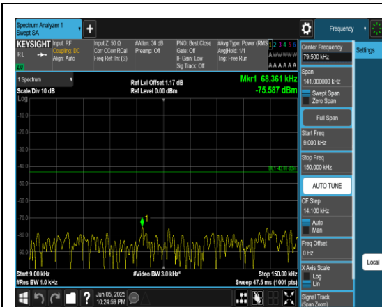
Band66_10MHz_QPSK_132622_1RB#0_0.009~0.15_0.009~0.15
