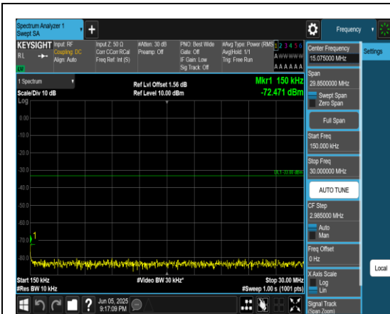
Band66_5MHz_QPSK_131997_1RB#0_0.15~30_0.15~30
