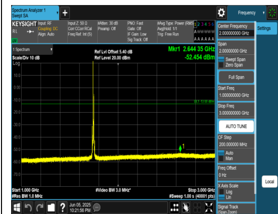
Band66_10MHz_QPSK_132322_1RB#0_1000~3000_1000~3000
