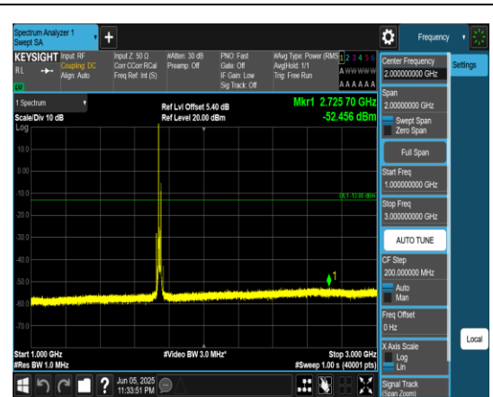
Band66_15MHz_QPSK_132322_1RB#0_1000~3 000_1000~3000
