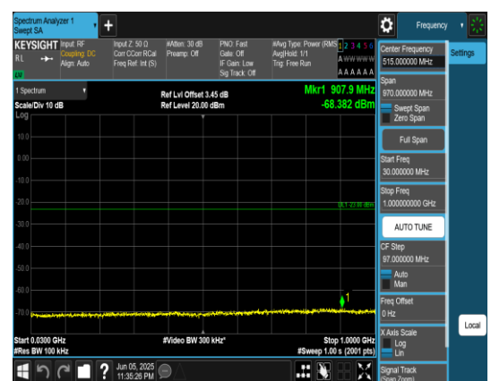
Band66_15MHz_QPSK_132597_1RB#0_30~100 0_30~1000
