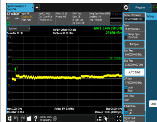
Band66_15MHz_QPSK_132322_1RB#0_3000~2 0000_3000~20000
