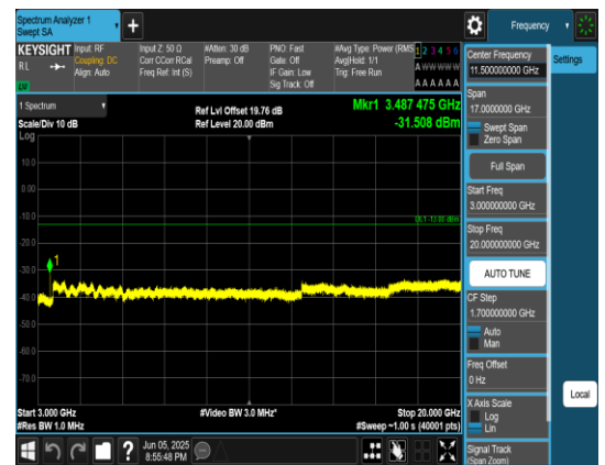
Band66_3MHz_QPSK_132322_1RB#0_3000~20000_00_3000~20000
