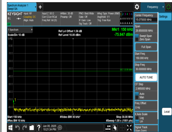
Band66_10MHz_QPSK_132322_1RB#0_0.15~30_0.15~30
