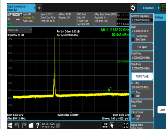
Band66_15MHz_QPSK_132047_1RB#0_1000~3 000_1000~3000
