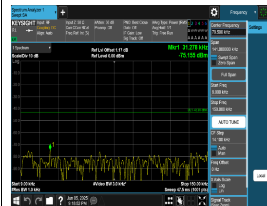
Band66_5MHz_QPSK_132322_1RB#0_0.009~0.15_0.009~0.15
