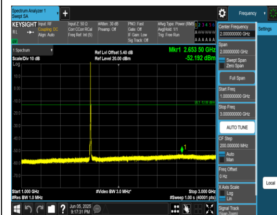
Band66_5MHz_QPSK_131997_1RB#0_1000~3000_1000~3000
