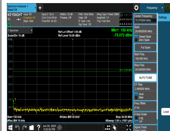
Band66_5MHz_QPSK_132647_1RB#0_0.15~30_0.15~30
