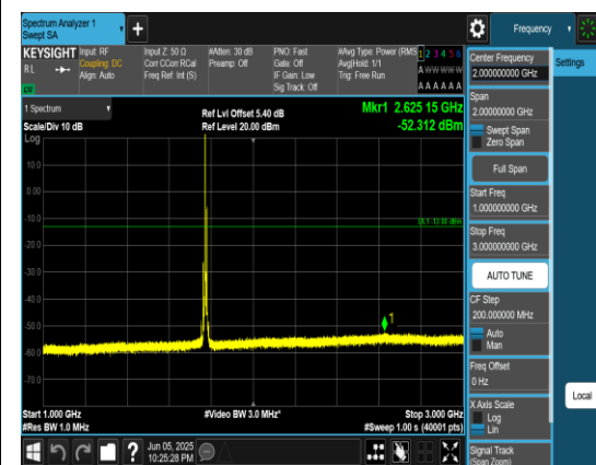
Band66_10MHz_QPSK_132622_1RB#0_1000~3000_000_1000~3000
