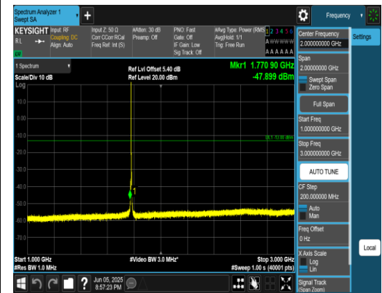
Band66_3MHz_QPSK_132657_1RB#0_1000~3000_00_1000~3000
