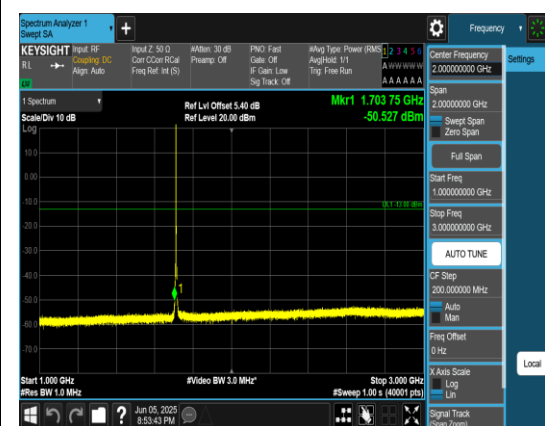
Band66_3MHz_QPSK_131987_1RB#0_1000~3000_00_1000~3000
