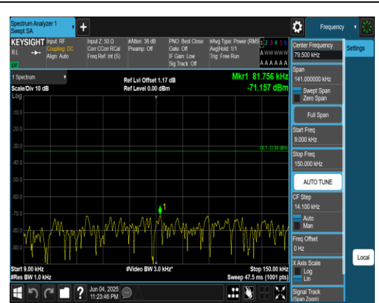
Band12_1.4MHz_QPSK_23173_1RB#0_0.009~0.15_0.009~0.15
