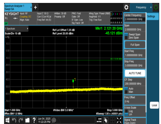
Band12_1.4MHz_QPSK_23095_1RB#0_1000~3000_1000~3000
