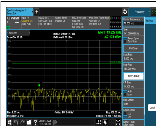
Band12_3MHz_QPSK_23025_1RB#0_0.009~0.15_0.009~0.15
