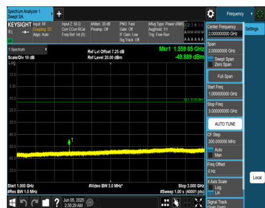
Band13_5MHz_QPSK_23230_1RB#0_1000~3000_1000~3000
