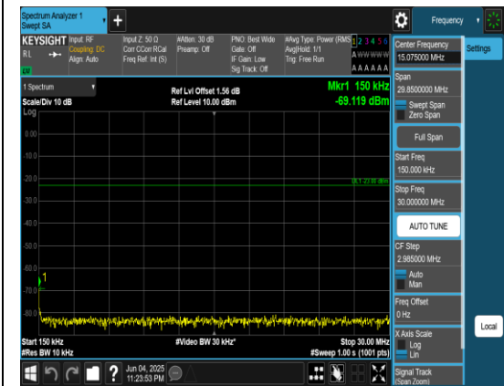
Band12_1.4MHz_QPSK_23173_1RB#0_0.15~30_0.15~30
