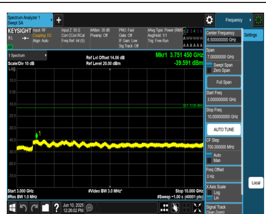
Band5_10MHz_QPSK_20600_1RB#0_3000~10000_3000~10000
