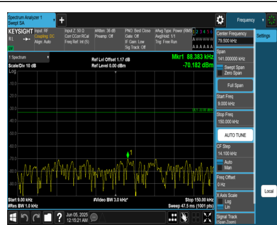
Band12_5MHz_QPSK_23155_1RB#0_0.009~0.1 5_0.009~0.15
