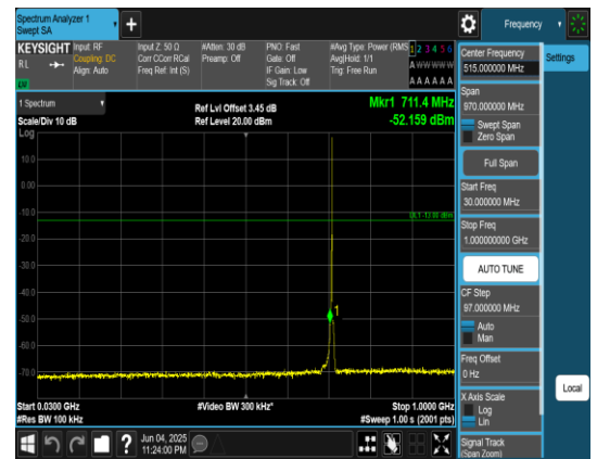
Band12_1.4MHz_QPSK_23173_1RB#0_30~1000_30~1000
