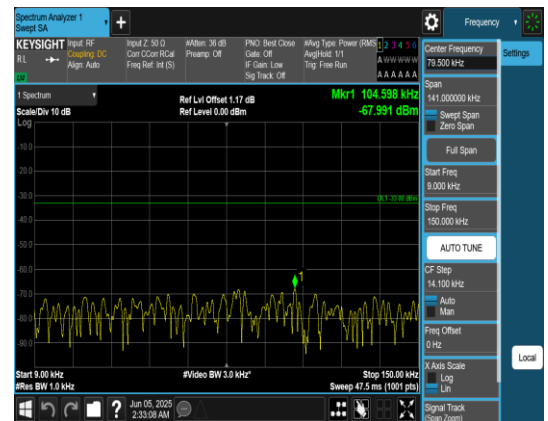
Band13_5MHz_QPSK_23205_1RB#0_0.009~0.15_5_0.009~0.15
