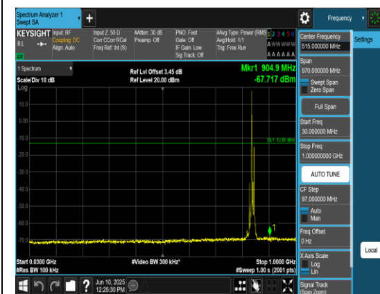
Band5_10MHz_QPSK_20600_1RB#0_30~1000_30~1000
