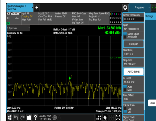
Band12_5MHz_QPSK_23095_1RB#0_0.009~0.15_0.009~0.15
