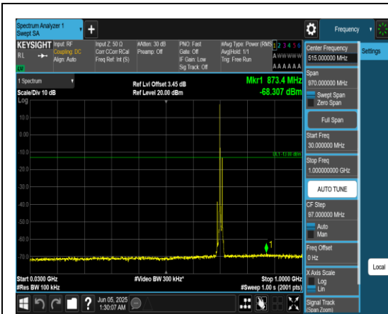
Band12_10MHz_QPSK_23130_1RB#0_30~1000_30~1000
