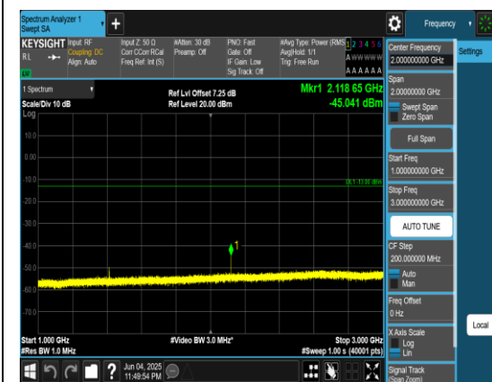
Band12_3MHz_QPSK_23095_1RB#0_1000~300_0_1000~3000
