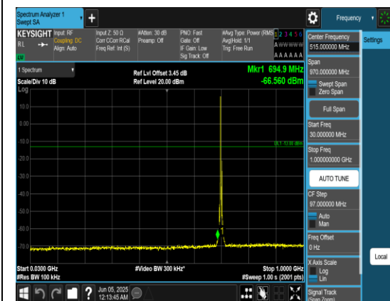
Band12_5MHz_QPSK_23095_1RB#0_30~1000_30~1000
