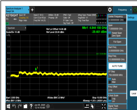
Band12_5MHz_QPSK_23095_1RB#0_3000~100 00_3000~10000
