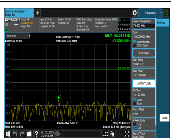
Band13_5MHz_QPSK_23255_1RB#0_0.009~0.1 5_0.009~0.15
