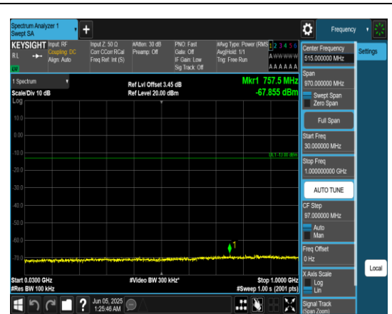
Band12_10MHz_QPSK_23095_1RB#0_30~1000_30~1000
