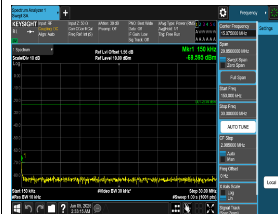
Band13_5MHz_QPSK_23205_1RB#0_0.15~30_0.15~30
