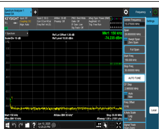
Band5_10MHz_QPSK_20600_1RB#0_0.15~30_0.15~30
