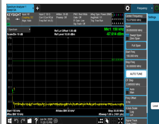
Band12_1.4MHz_QPSK_23017_1RB#0_0.15~30_0.15~30
