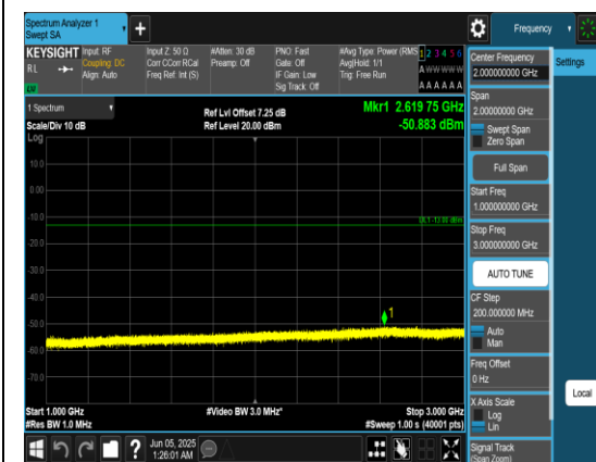
Band12_10MHz_QPSK_23095_1RB#0_1000~30_00_1000~3000
