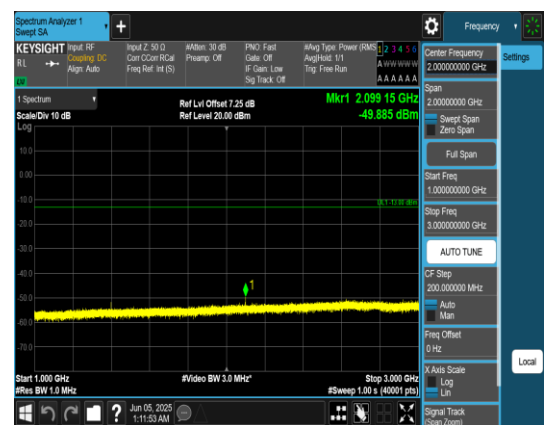
Band12_10MHz_QPSK_23060_1RB#0_1000-3000_00_1000-3000
