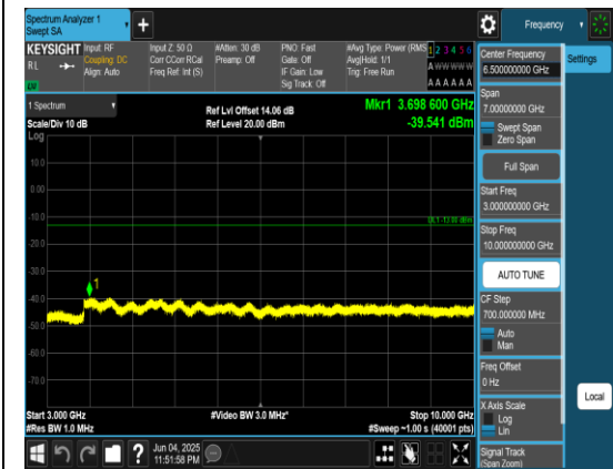
Band12_3MHz_QPSK_23165_1RB#0_3000~10000_00_3000~10000
