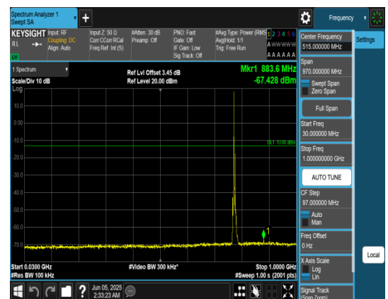
Band13_5MHz_QPSK_23205_1RB#0_30~1000_30~1000
