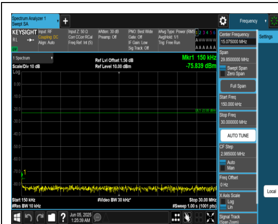
Band12_10MHz_QPSK_23095_1RB#0_0.15~30_0.15~30
