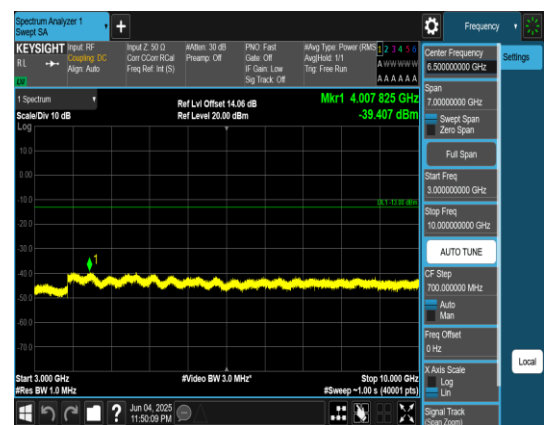
Band12_3MHz_QPSK_23095_1RB#0_3000~100_00_3000~10000
