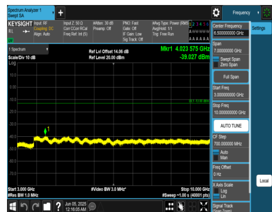
Band12_5MHz_QPSK_23155_1RB#0_3000~100 00_3000~10000
