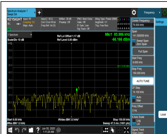
Band12_10MHz_QPSK_23060_1RB#0_0.009-0.15_0.009-0.15
