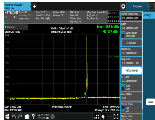
Band12_5MHz_QPSK_23155_1RB#0_30~1000_ 30~1000
