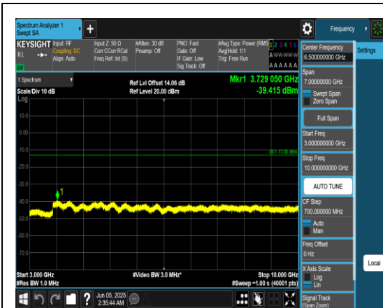
Band13_5MHz_QPSK_23230_1RB#0_3000~100 00_3000~10000
