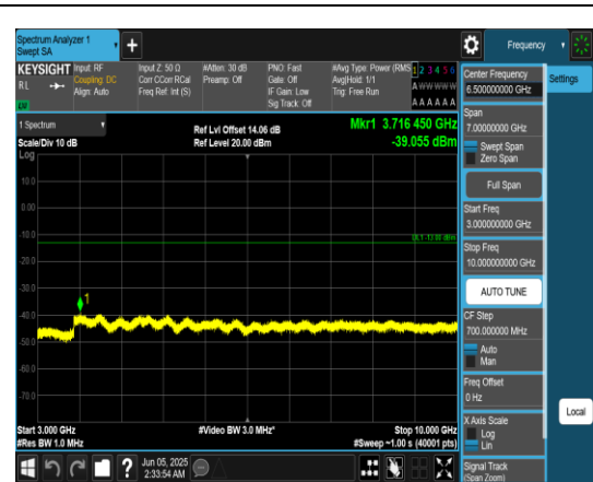
Band13_5MHz_QPSK_23205_1RB#0_3000~10000_3000~10000
