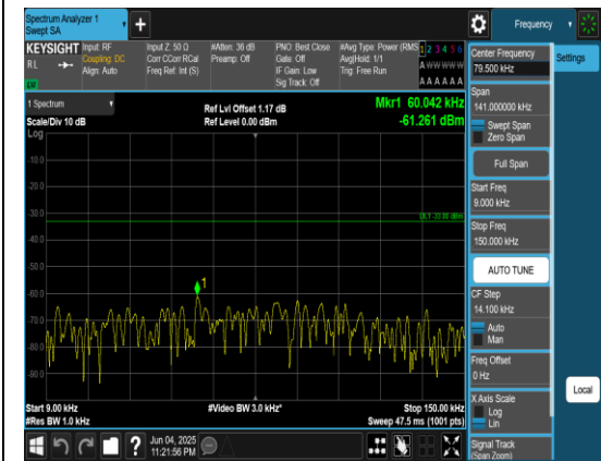
Band12_1.4MHz_QPSK_23095_1RB#0_0.009~0.15_0.009~0.15
