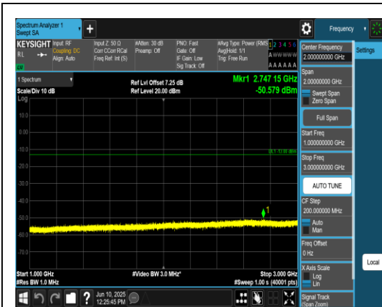
Band5_10MHz_QPSK_20600_1RB#0_1000~3000_1000~3000
