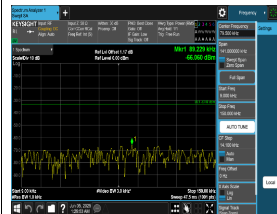
Band12_10MHz_QPSK_23130_1RB#0_0.009~0.15_0.009~0.15
