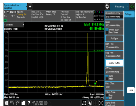
Band5_10MHz_QPSK_20525_1RB#0_30~1000_30~1000
