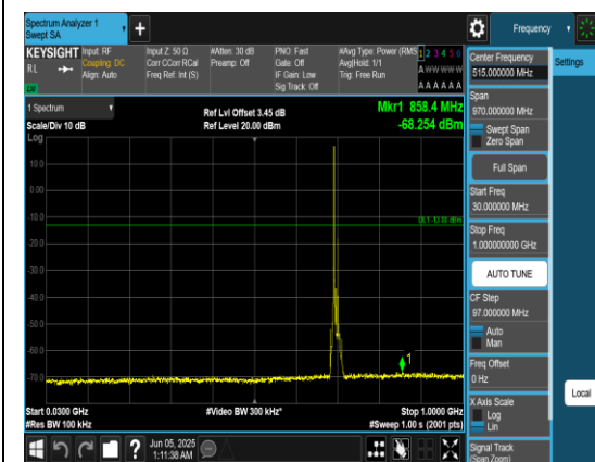
Band12_10MHz_QPSK_23060_1RB#0_30-1000_30-1000
