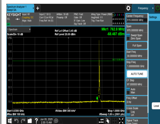
Band13_5MHz_QPSK_23230_1RB#0_30~1000_30~1000
