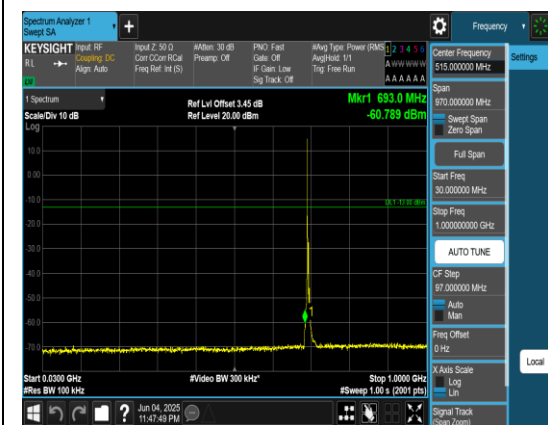
Band12_3MHz_QPSK_23025_1RB#0_30~1000_30~1000
