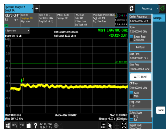
Band5_10MHz_QPSK_20525_1RB#0_3000~10000_3000~10000
