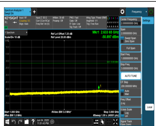
Band12_3MHz_QPSK_23165_1RB#0_1000~3000_0_1000~3000
