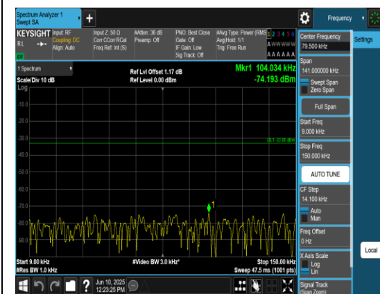
Band5_10MHz_QPSK_20525_1RB#0_0.009~0.1_0.009~0.15
