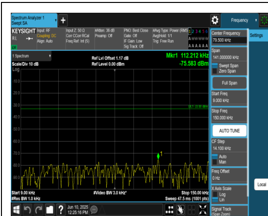
Band5_10MHz_QPSK_20600_1RB#0_0.009~0.15_0.009~0.15
