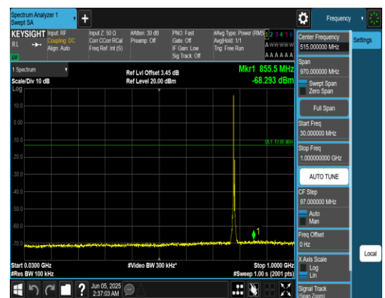
Band13_5MHz_QPSK_23255_1RB#0_30~1000_ 30~1000
