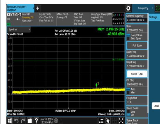
Band5_10MHz_QPSK_20525_1RB#0_1000~3000_1000~3000
