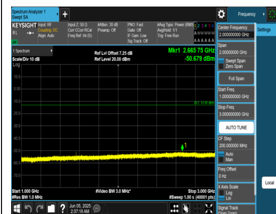
Band13_5MHz_QPSK_23255_1RB#0_1000~300 0_1000~3000
