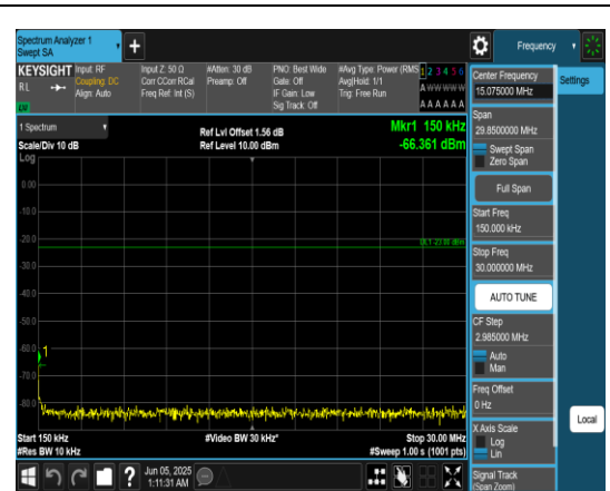
Band12_10MHz_QPSK_23060_1RB#0_0.15-30_0.15-30
