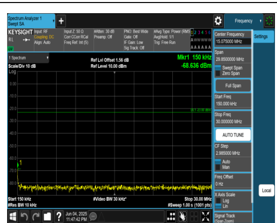
Band12_3MHz_QPSK_23025_1RB#0_0.15~30_0.15~30
