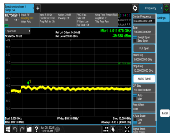
Band12_10MHz_QPSK_23095_1RB#0_3000~10_000_3000~10000
