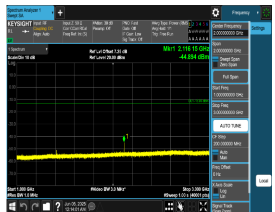
Band12_5MHz_QPSK_23095_1RB#0_1000~3000_1000~3000
