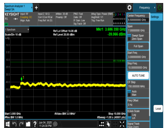
Band12_1.4MHz_QPSK_23173_1RB#0_3000~10000_00_3000~10000
