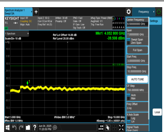
Band12_1.4MHz_QPSK_23017_1RB#0_3000~10000_3000~10000
