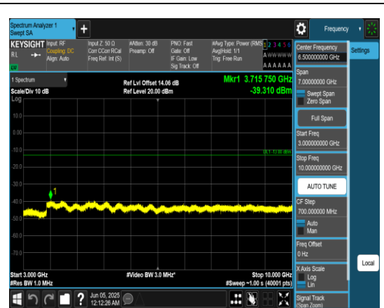
Band12_5MHz_QPSK_23035_1RB#0_3000~10000_3000~10000
