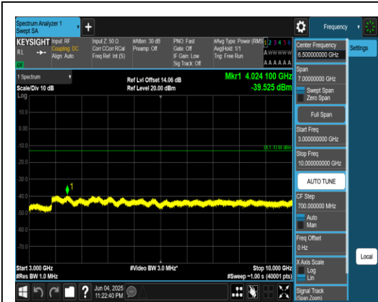
Band12_1.4MHz_QPSK_23095_1RB#0_3000~10000_3000~10000
