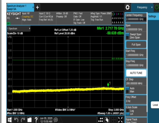
Band12_5MHz_QPSK_23155_1RB#0_1000~300 0_1000~3000
