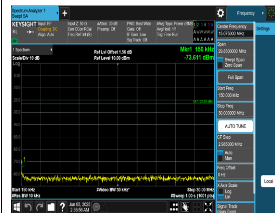
Band13_5MHz_QPSK_23255_1RB#0_0.15~30_0 .15~30
