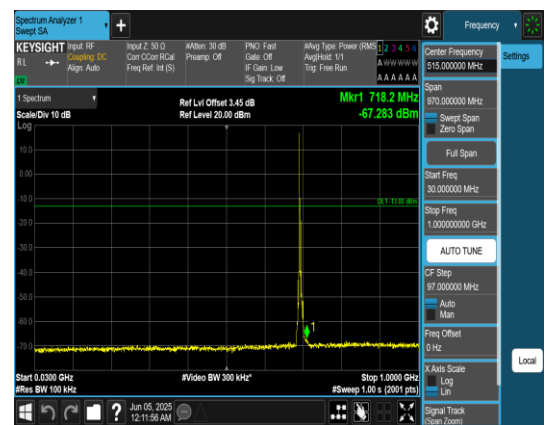
Band12_5MHz_QPSK_23035_1RB#0_30~1000_30~1000
