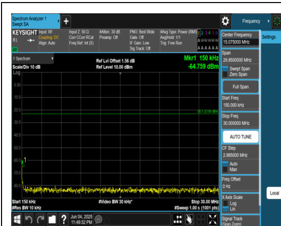
Band12_3MHz_QPSK_23095_1RB#0_0.15~30_0 .15~30
