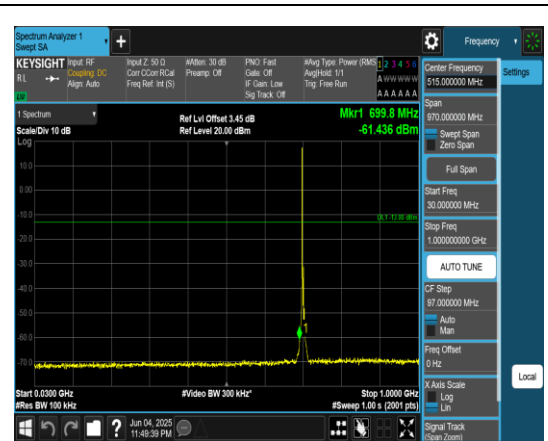
Band12_3MHz_QPSK_23095_1RB#0_30~1000_30~1000
