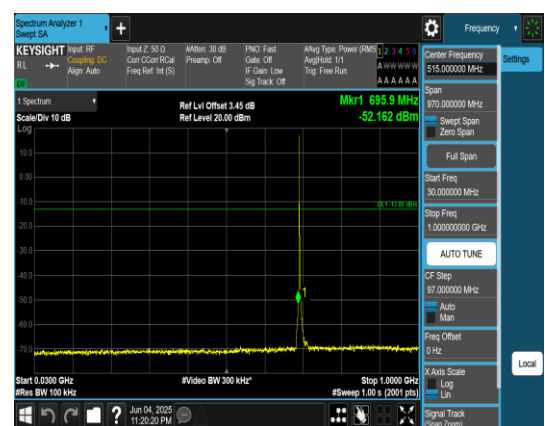
Band12_1.4MHz_QPSK_23017_1RB#0_30~1000_30~1000
