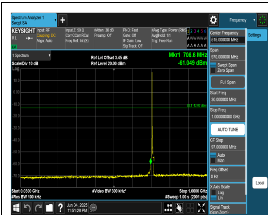
Band12_3MHz_QPSK_23165_1RB#0_30~1000_30~1000
