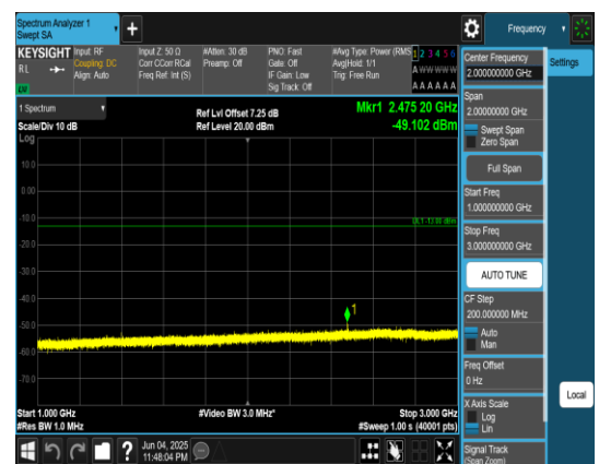
Band12_3MHz_QPSK_23025_1RB#0_1000~3000_1000~3000
