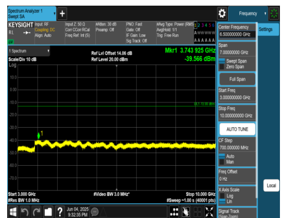
Band5_5MHz_QPSK_20525_1RB#0_3000~1000 0_3000~10000
