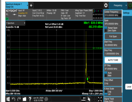
Band5_5MHz_QPSK_20425_1RB#0_30~1000_3 0~1000
