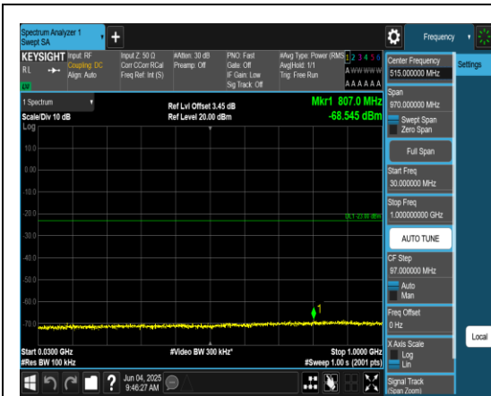
Band4_5MHz_QPSK_20375_1RB#0_30~1000_30~1000
