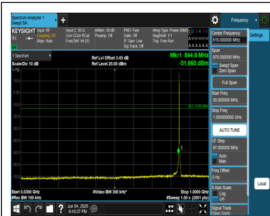
Band5_1.4MHz_QPSK_20643_1RB#0_30~1000_30~1000
