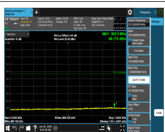
Band4_5MHz_QPSK_20175_1RB#0_30~1000_3 0~1000
