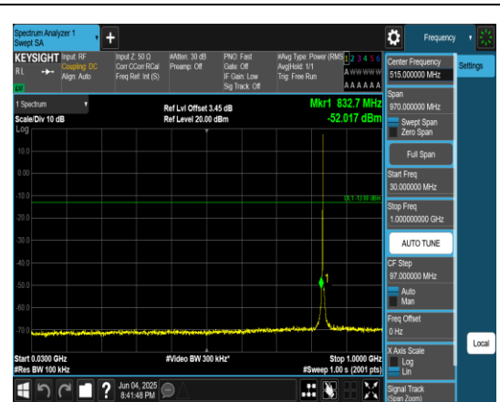
Band5_1.4MHz_QPSK_20525_1RB#0_30~1000_30~1000
