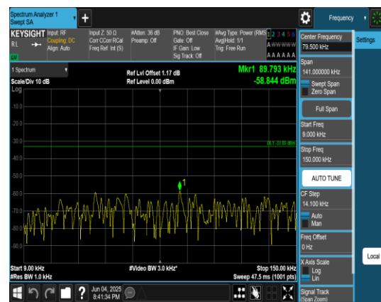
Band5_1.4MHz_QPSK_20525_1RB#0_0.009~0.15_5_0.009~0.15
