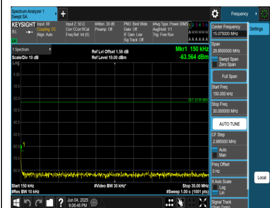
Band5_3MHz_QPSK_20415_1RB#0_0.15~30_0.15~30
