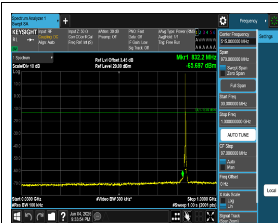
Band5_5MHz_QPSK_20625_1RB#0_30~1000_30~1000
