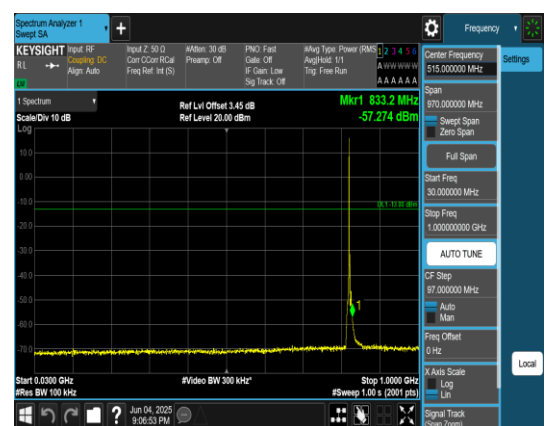
Band5_3MHz_QPSK_20415_1RB#0_30~1000_30~1000
