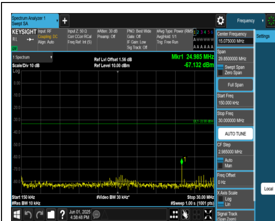
Band4_10MHz_QPSK_20175_1RB#0_0.15~30_0.15~30
