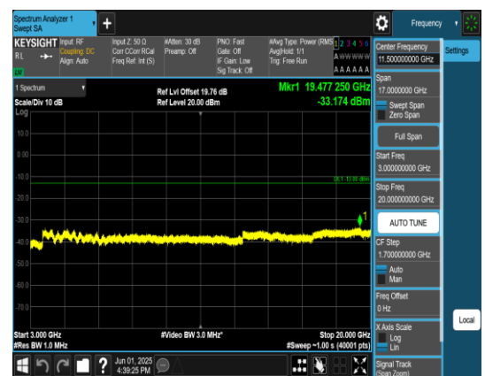
Band4_10MHz_QPSK_20175_1RB#0_3000~200_00_3000~20000
