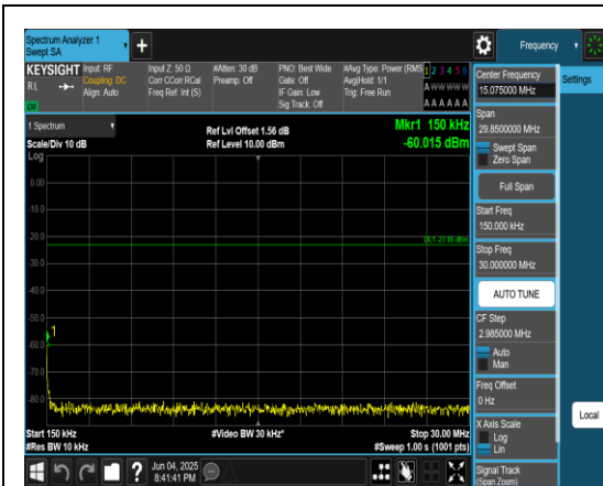
Band5_1.4MHz_QPSK_20525_1RB#0_0.15~30_0.15~30
