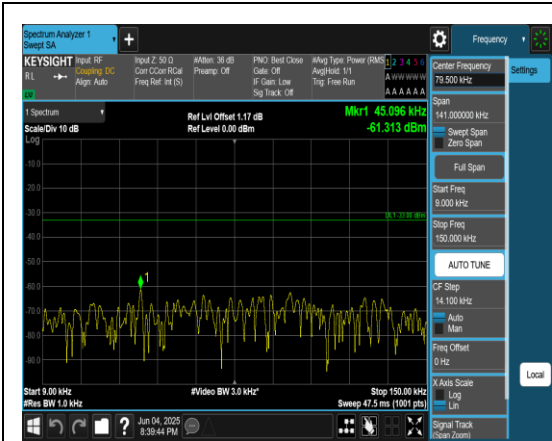
Band5_1.4MHz_QPSK_20407_1RB#0_0.009~0.15_0.009~0.15
