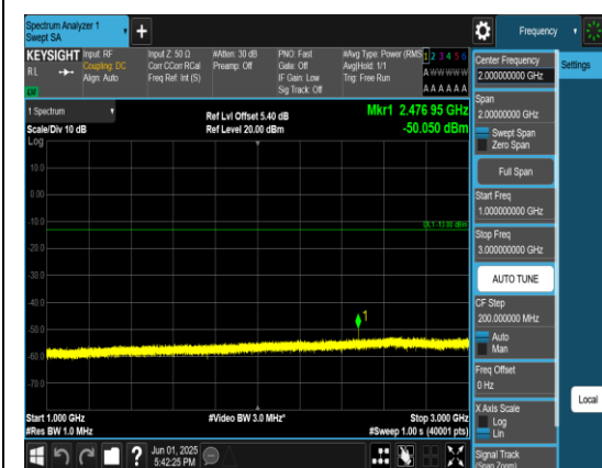
Band4_15MHz_QPSK_20325_1RB#0_1000~3000_0_1000~3000
