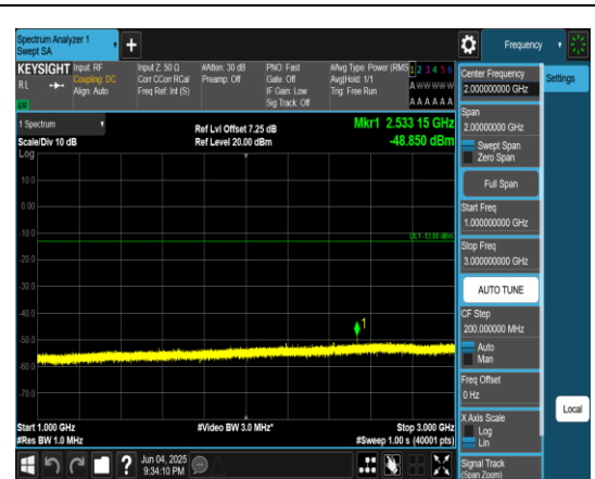
Band5_5MHz_QPSK_20625_1RB#0_1000~3000_1000~3000
