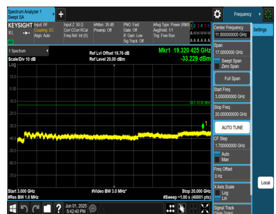
Band4_15MHz_QPSK_20325_1RB#0_3000~20000_00_3000~20000
