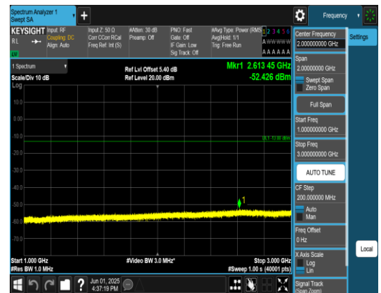
Band4_10MHz_QPSK_20000_1RB#0_1000~300_0_1000~3000
