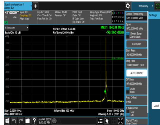
Band5_3MHz_QPSK_20635_1RB#0_30~1000_3 0~1000
