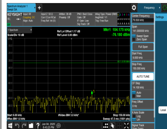
Band5_1.4MHz_QPSK_20643_1RB#0_0.009~0.15_0.009~0.15
