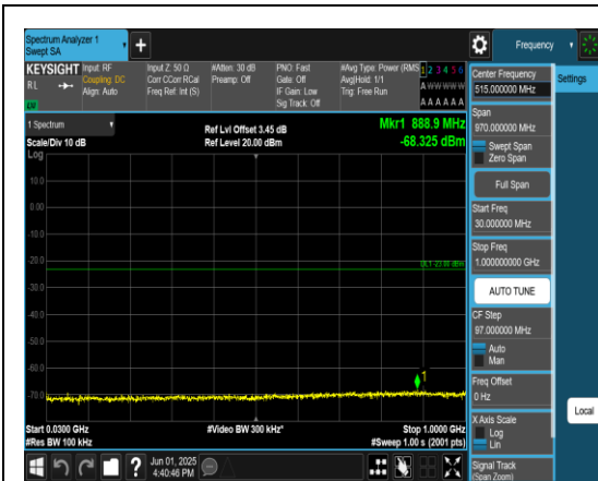
Band4_10MHz_QPSK_20350_1RB#0_30~1000_30~1000
