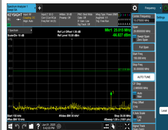
Band4_15MHz_QPSK_20325_1RB#0_0.15~30_0.15~30
