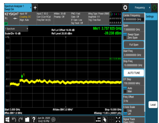
Band5_1.4MHz_QPSK_20525_1RB#0_3000~10000_00_3000~10000
