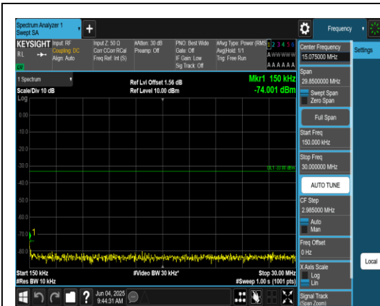
Band4_5MHz_QPSK_20175_1RB#0_0.15~30_0. 15~30
