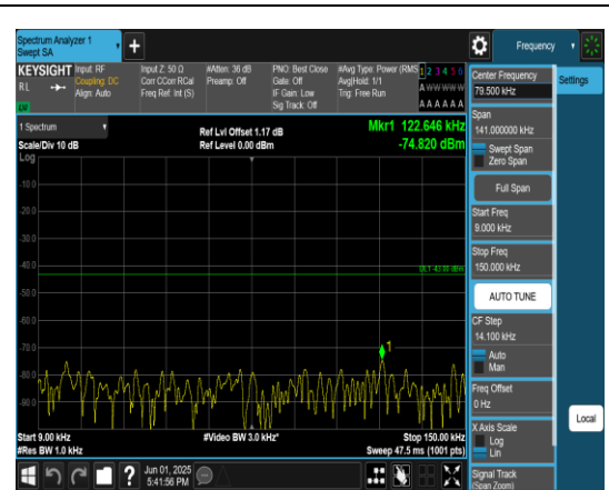
Band4_15MHz_QPSK_20325_1RB#0_0.009~0.15_0.009~0.15
