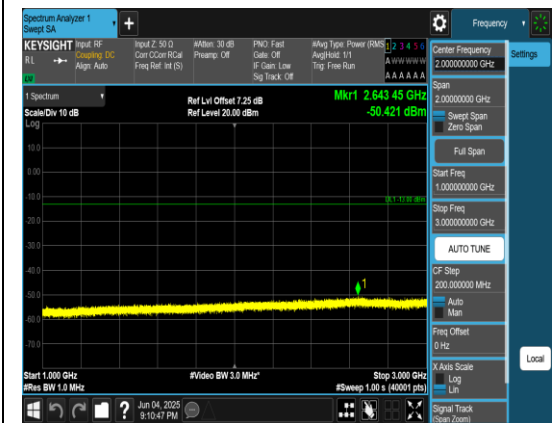
Band5_3MHz_QPSK_20635_1RB#0_1000~3000 _1000~3000
