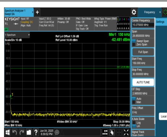
Band5_1.4MHz_QPSK_20407_1RB#0_0.15~30_0.15~30
