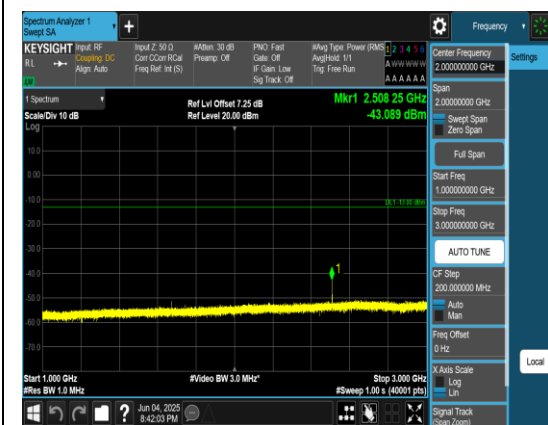
Band5_1.4MHz_QPSK_20525_1RB#0_1000~3000_0_1000~3000
