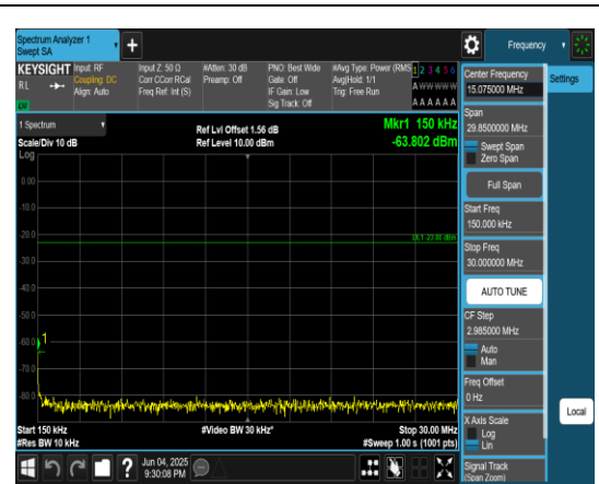
Band5_5MHz_QPSK_20425_1RB#0_0.15~30_0. 15~30
