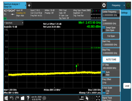
Band5_5MHz_QPSK_20425_1RB#0_1000~3000 _1000~3000
