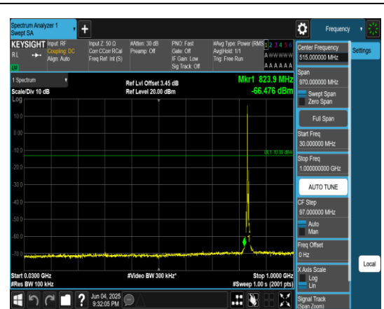
Band5_5MHz_QPSK_20525_1RB#0_30~1000_3 0~1000
