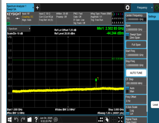
Band5_5MHz_QPSK_20525_1RB#0_1000~3000 _1000~3000
