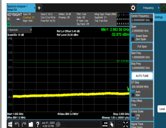
Band4_10MHz_QPSK_20175_1RB#0_1000~300_0_1000~3000
