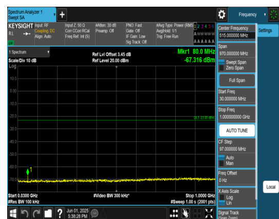
Band4_15MHz_QPSK_20025_1RB#0_30~1000_30~1000
