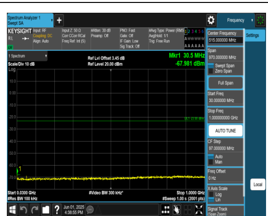
Band4_10MHz_QPSK_20175_1RB#0_30~1000_30~1000
