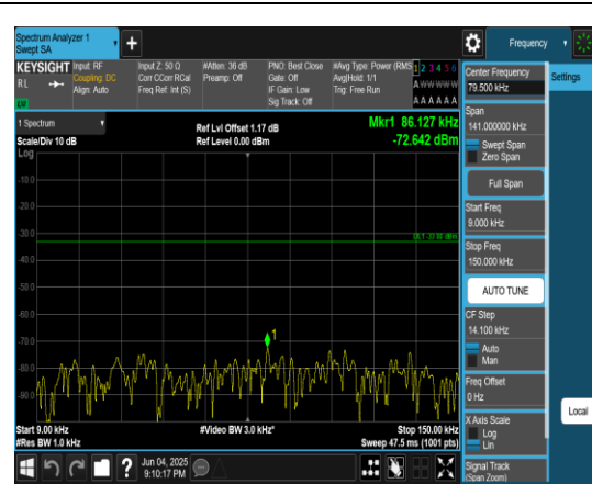
Band5_3MHz_QPSK_20635_1RB#0_0.009~0.15 _0.009~0.15
