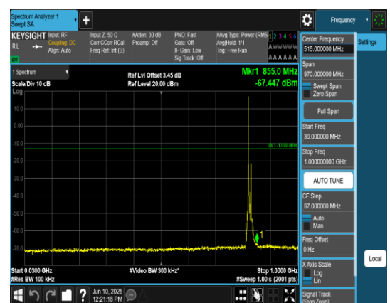
Band5_10MHz_QPSK_20450_1RB#0_30~1000_30~1000
