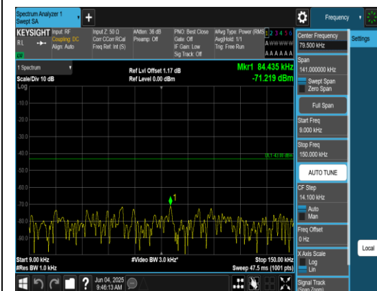
Band4_5MHz_QPSK_20375_1RB#0_0.009~0.15 _0.009~0.15
