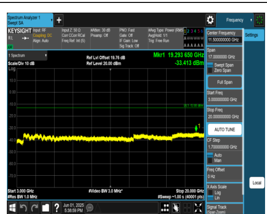
Band4_15MHz_QPSK_20025_1RB#0_3000~20000_3000~20000
