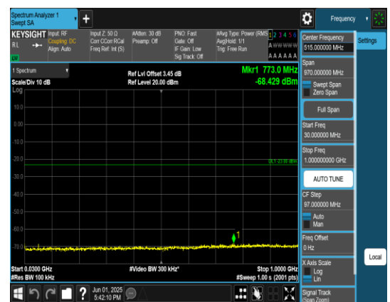
Band4_15MHz_QPSK_20325_1RB#0_30~1000_30~1000
