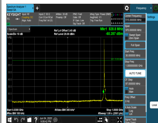
Band5_3MHz_QPSK_20525_1RB#0_30~1000_3 0~1000
