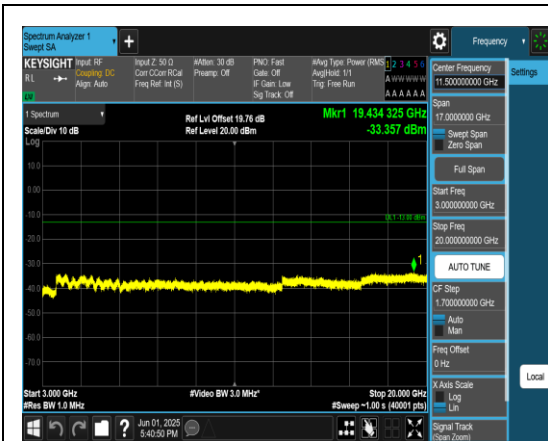
Band4_15MHz_QPSK_20175_1RB#0_3000~20000_3000~20000
