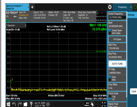
Band5_10MHz_QPSK_20450_1RB#0_0.15~30_0.15~30
