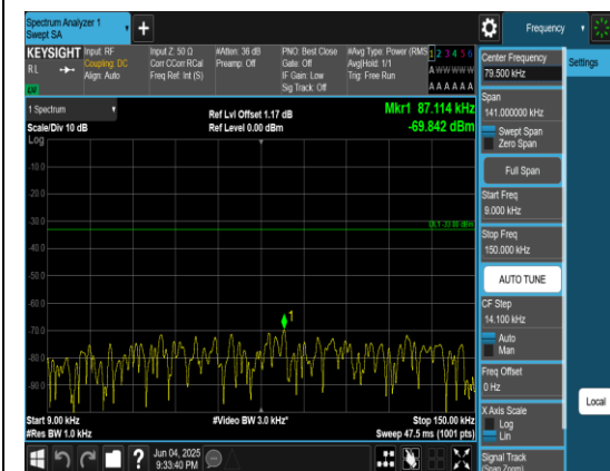
Band5_5MHz_QPSK_20625_1RB#0_0.009~0.15 _0.009~0.15
