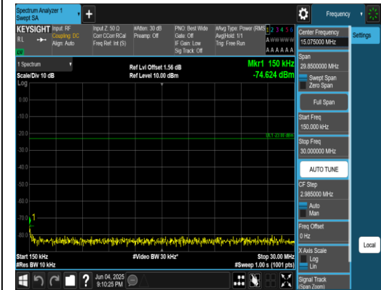
Band5_3MHz_QPSK_20635_1RB#0_0.15~30_0. 15~30
