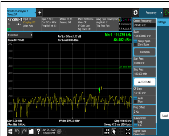
Band5_5MHz_QPSK_20425_1RB#0_0.009~0.15 _0.009~0.15
