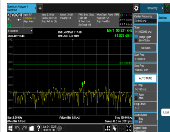
Band5_3MHz_QPSK_20525_1RB#0_0.009~0.15 _0.009~0.15
