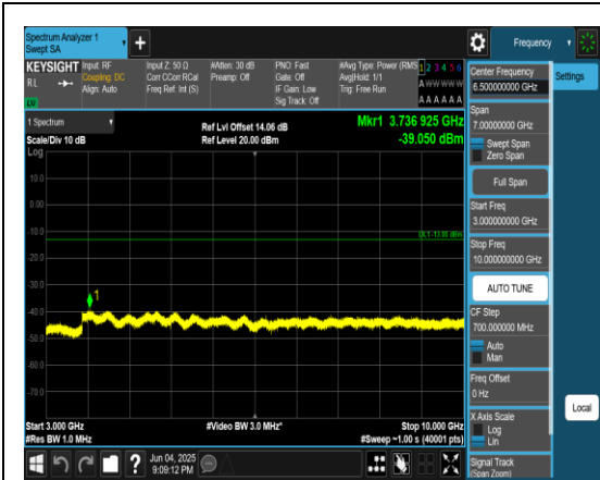
Band5_3MHz_QPSK_20525_1RB#0_3000~1000 0_3000~10000
