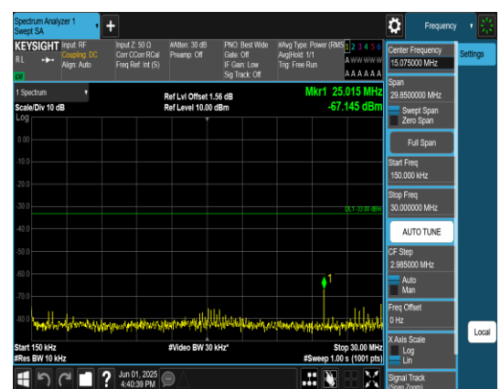
Band4_10MHz_QPSK_20350_1RB#0_0.15~30_0.15~30
