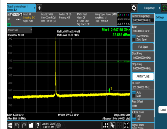
Band4_5MHz_QPSK_20175_1RB#0_1000~3000 _1000~3000
