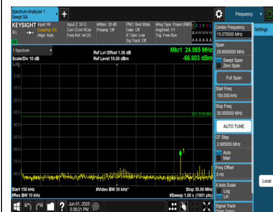
Band4_15MHz_QPSK_20025_1RB#0_0.15~30_0.15~30
