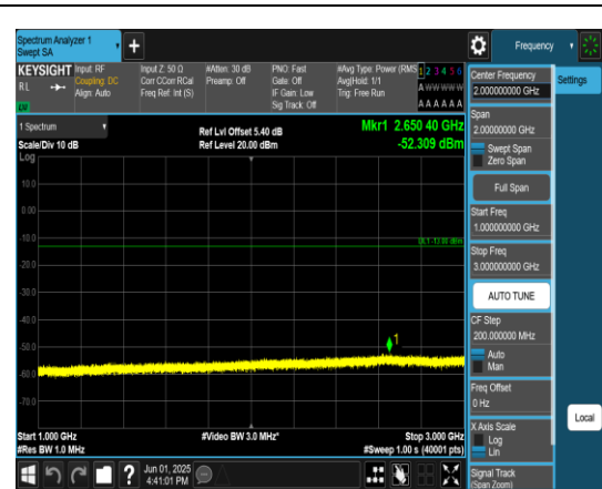
Band4_10MHz_QPSK_20350_1RB#0_1000~3000_0_1000~3000
