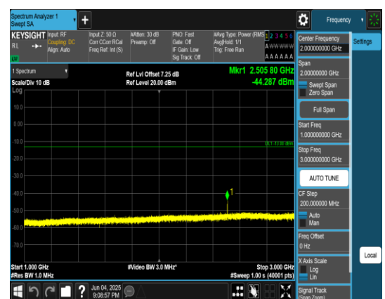
Band5_3MHz_QPSK_20525_1RB#0_1000~3000 _1000~3000
