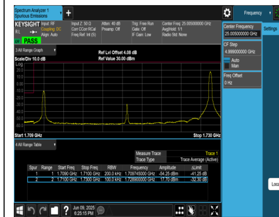
Band4_20MHz_QPSK_20050_1RB#99
