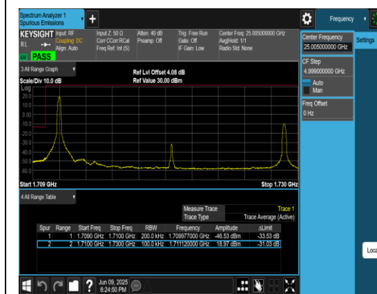
Band4_20MHz_QPSK_20050_1RB#0
