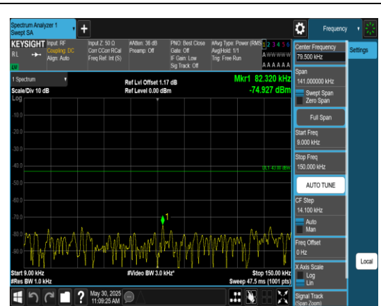
Band2_3MHz_QPSK_19185_1RB#0_0.009~0.15 _0.009~0.15
