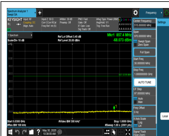
Band2_1.4MHz_QPSK_19193_1RB#0_30~1000_30~1000
