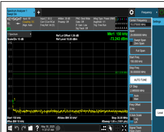
Band2_5MHz_QPSK_18900_1RB#0_0.15~30_0. 15~30
