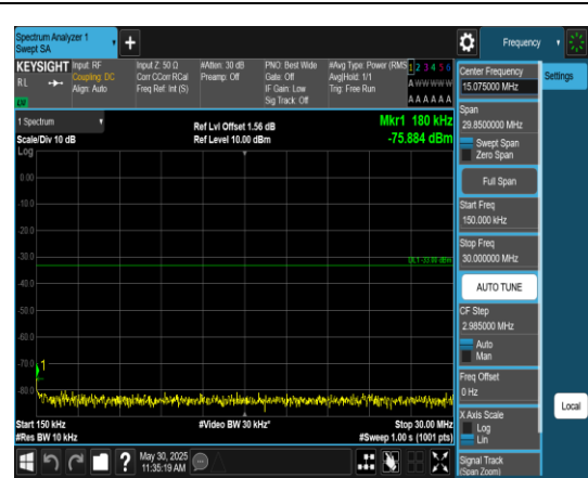
Band2_5MHz_QPSK_18625_1RB#0_0.15~30_0. 15~30
