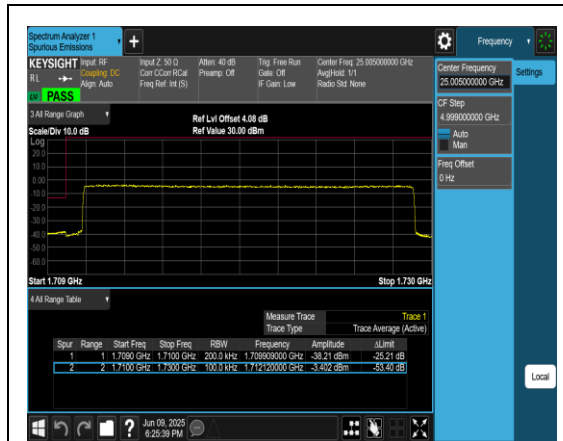
Band4_20MHz_QPSK_20050_100RB#0
