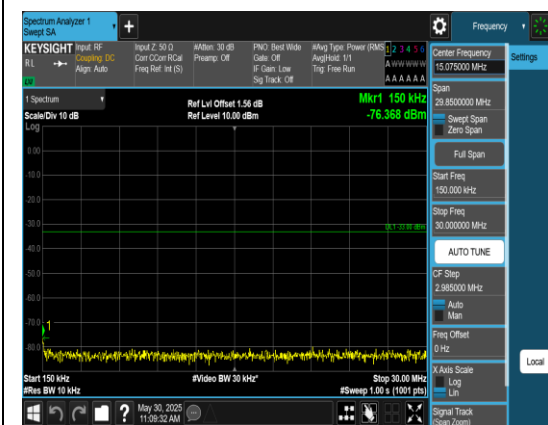
Band2_3MHz_QPSK_19185_1RB#0_0.15~30_0. 15~30
