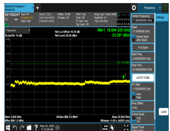
Band2_3MHz_QPSK_19185_1RB#0_3000~2000 0_3000~20000
