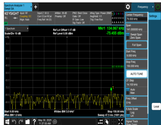
Band2_5MHz_QPSK_18900_1RB#0_0.009~0.15 _0.009~0.15
