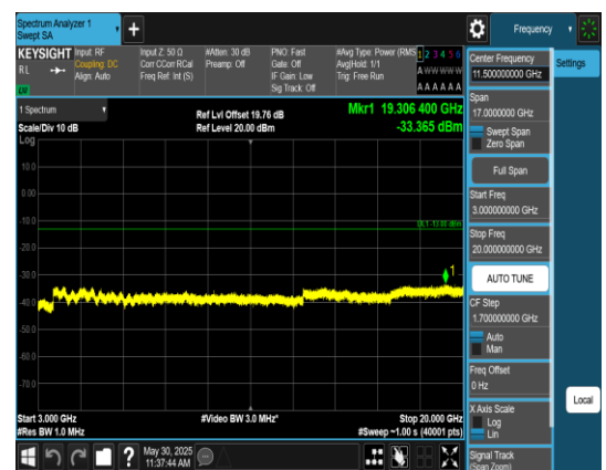
Band2_5MHz_QPSK_18900_1RB#0_3000~2000 0_3000~20000
