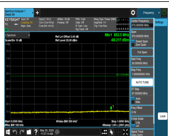
Band2_5MHz_QPSK_18900_1RB#0_30~1000_3 0~1000
