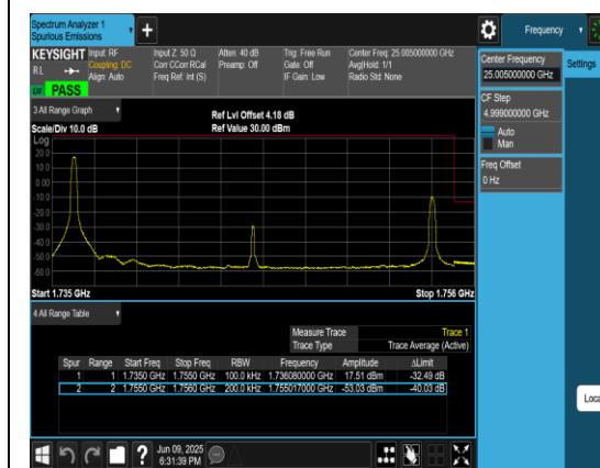
Band4_20MHz_QPSK_20300_1RB#0
