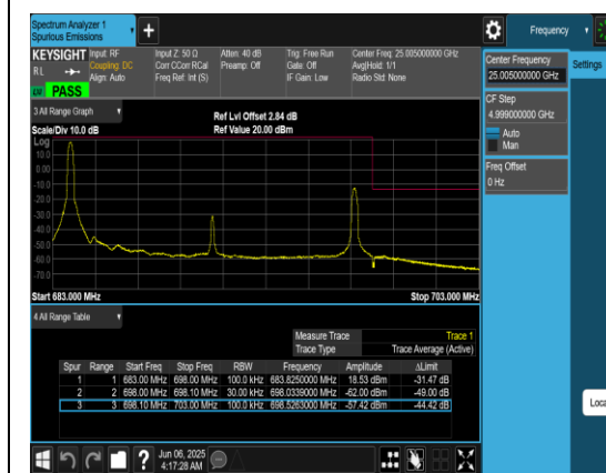
Band71_15MHz_QPSK_133397_1RB#0
