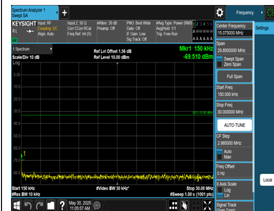
Band2_3MHz_QPSK_18615_1RB#0_0.15~30_0.15~30
