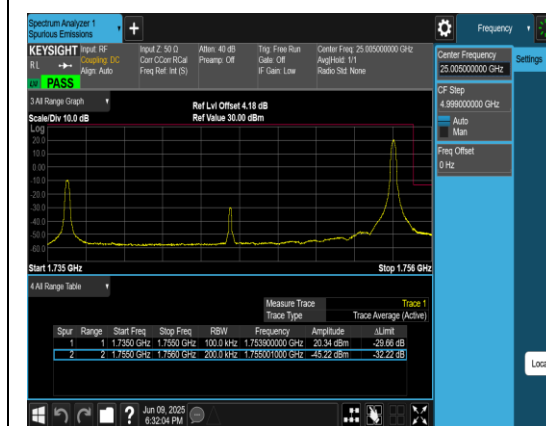
Band4_20MHz_QPSK_20300_1RB#99
