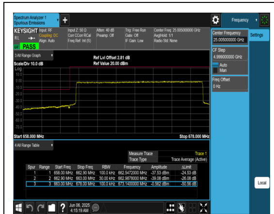
Band71_15MHz_QPSK_133197_75RB#0
