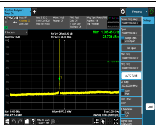
Band2_1.4MHz_QPSK_19193_1RB#0_1000~3000_0_1000~3000
