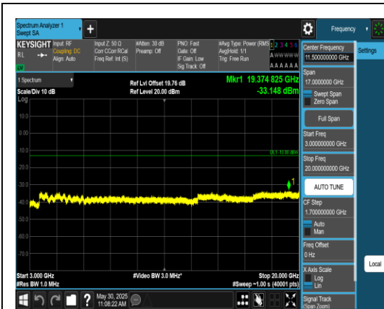
Band2_3MHz_QPSK_18900_1RB#0_3000~2000 0_3000~20000
