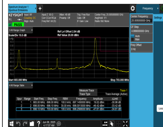
Band71_15MHz_QPSK_133397_1RB#74
