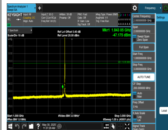
Band2_5MHz_QPSK_18900_1RB#0_1000~3000 _1000~3000
