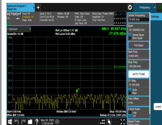
Band2_5MHz_QPSK_19175_1RB#0_0.009~0.15 _0.009~0.15
