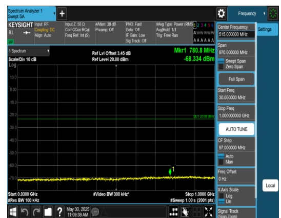
Band2_3MHz_QPSK_19185_1RB#0_30~1000_3 0~1000
