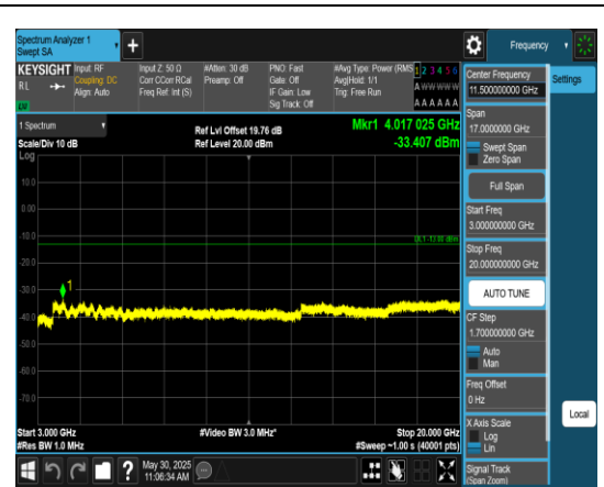
Band2_3MHz_QPSK_18615_1RB#0_3000~20000_0_3000~20000
