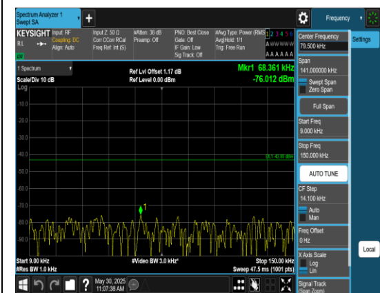
Band2_3MHz_QPSK_18900_1RB#0_0.009~0.15_0.009~0.15
