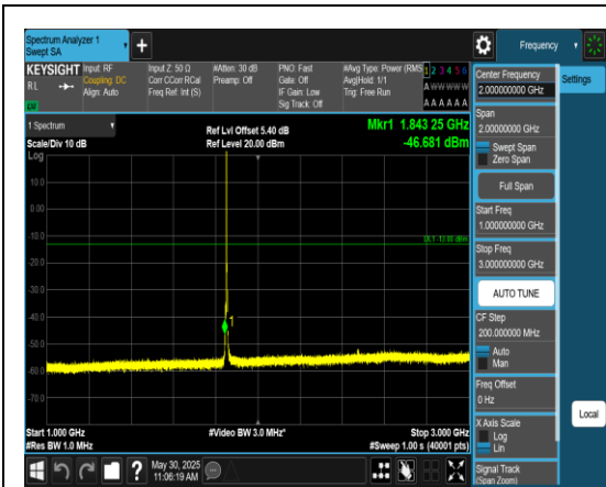
Band2_3MHz_QPSK_18615_1RB#0_1000~3000_1000~3000
