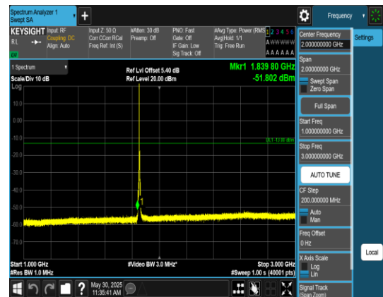
Band2_5MHz_QPSK_18625_1RB#0_1000~3000 _1000~3000
