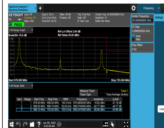
Band71_20MHz_QPSK_133372_1RB#0
