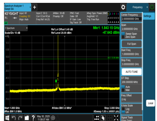
Band2_3MHz_QPSK_18900_1RB#0_1000~3000_1000~3000
