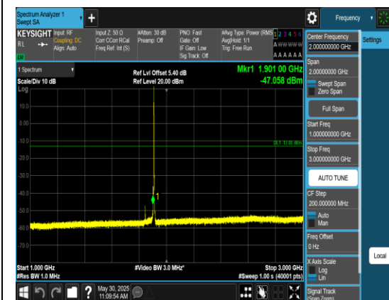
Band2_3MHz_QPSK_19185_1RB#0_1000~3000 _1000~3000
