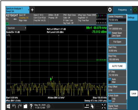
Band2_5MHz_QPSK_18625_1RB#0_0.009~0.15 _0.009~0.15
