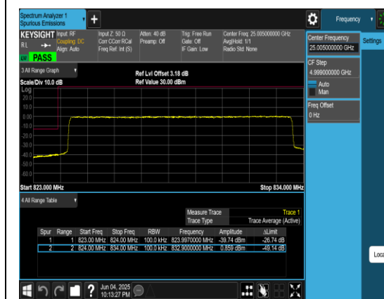
Band5_10MHz_QPSK_20450_50RB#0
