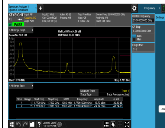
Band66_10MHz_QPSK_132622_1RB#0
