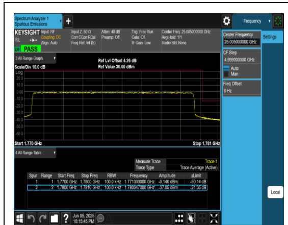
Band66_10MHz_QPSK_132622_50RB#0
