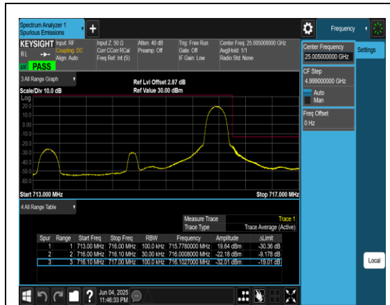
Band12_3MHz_QPSK_23165_1RB#14
