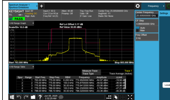
Band13_5MHz_QPSK_23255_25RB#0
