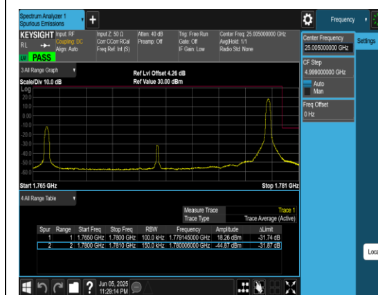
Band66_15MHz_QPSK_132597_1RB#74
