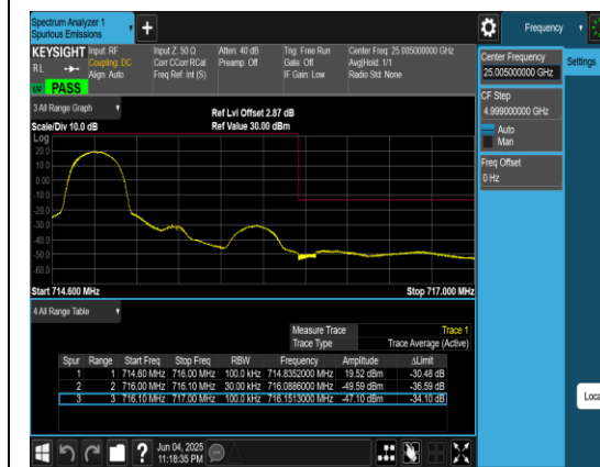
Band12_1.4MHz_QPSK_23173_1RB#0
