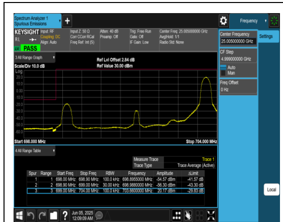
Band12_5MHz_QPSK_23035_1RB#24
