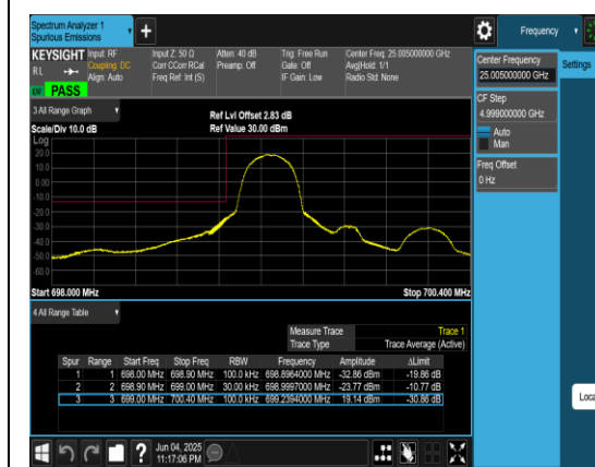
Band12_1.4MHz_QPSK_23017_1RB#0
