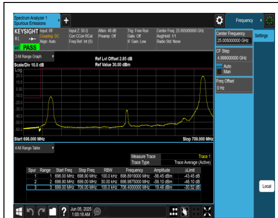
Band12_10MHz_QPSK_23060_1RB#49
