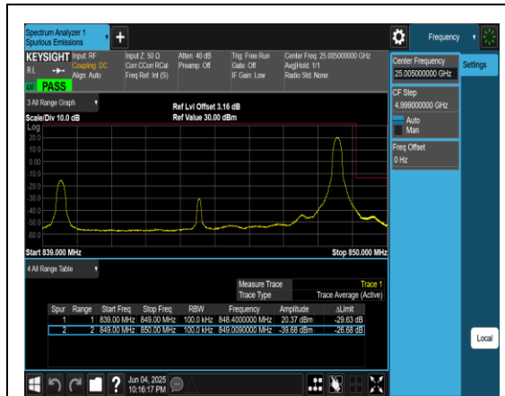
Band5_10MHz_QPSK_20600_1RB#49
