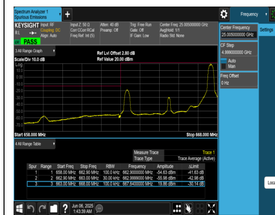
Band71_5MHz_QPSK_133147_1RB#24
