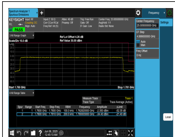
Band66_20MHz_QPSK_132572_100RB#0
