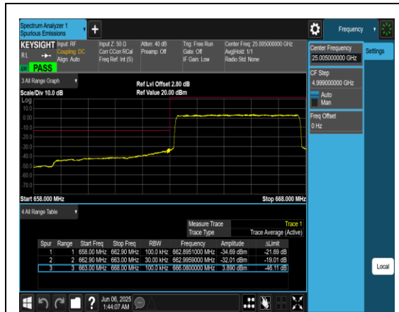
Band71_5MHz_QPSK_133147_25RB#0
