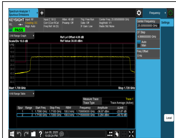
Band66_10MHz_QPSK_132022_50RB#0
