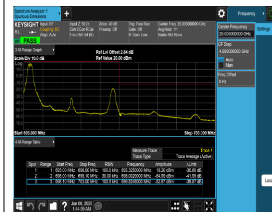
Band71_5MHz_QPSK_133447_1RB#0
