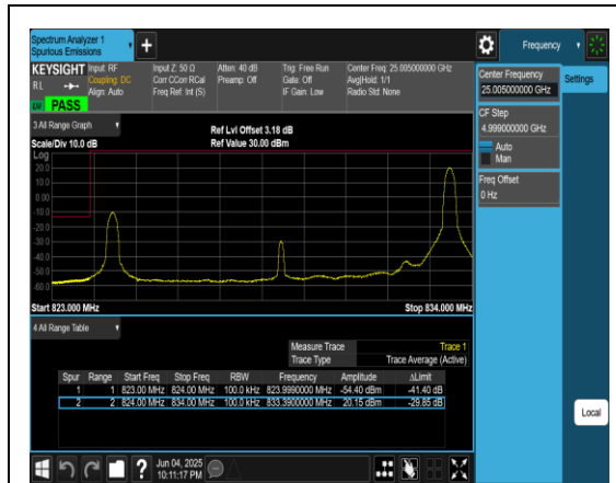
Band5_10MHz_QPSK_20450_1RB#49
