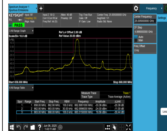
Band71_5MHz_QPSK_133147_1RB#0
