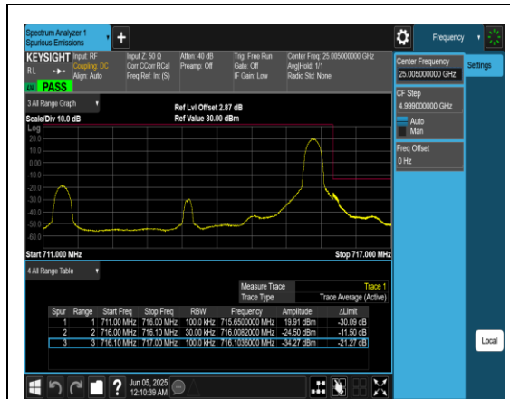
Band12_5MHz_QPSK_23155_1RB#24
