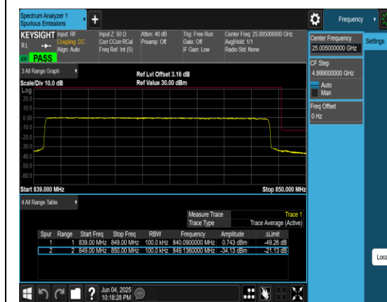
Band5_10MHz_QPSK_20600_50RB#0
