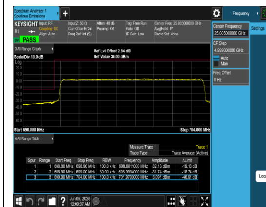
Band12_5MHz_QPSK_23035_25RB#0
