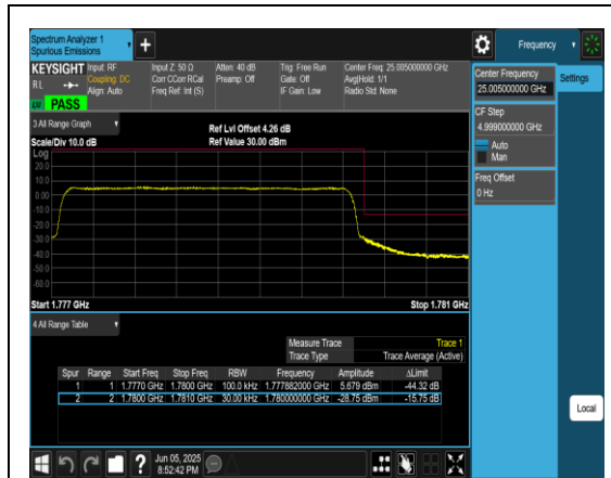
Band66_3MHz_QPSK_132657_15RB#0
