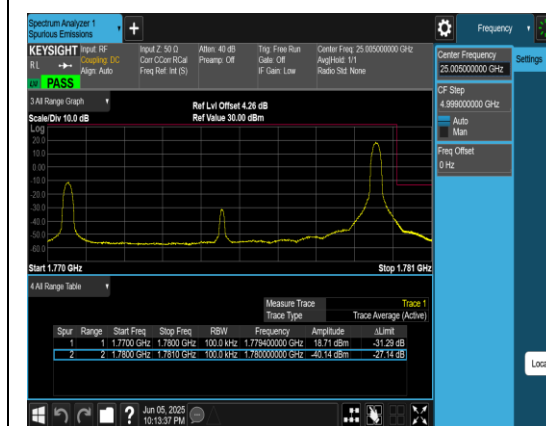
Band66_10MHz_QPSK_132622_1RB#49
