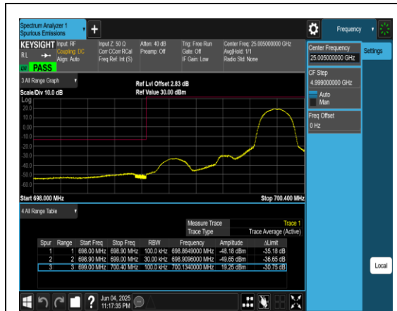
Band12_1.4MHz_QPSK_23017_1RB#5
