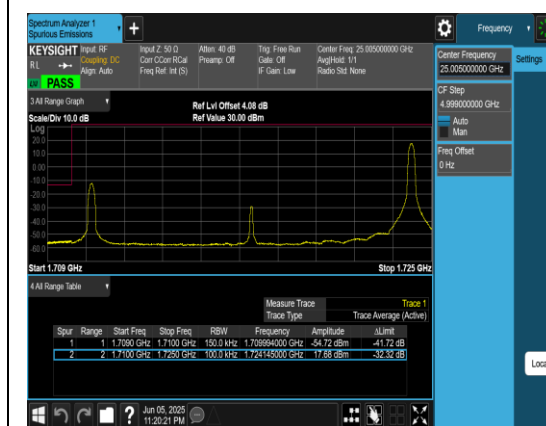
Band66_15MHz_QPSK_132047_1RB#74
