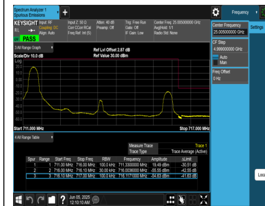
Band12_5MHz_QPSK_23155_1RB#0
