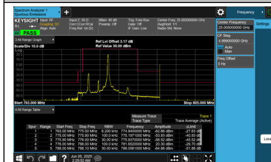
Band13_5MHz_QPSK_23205_1RB#24
