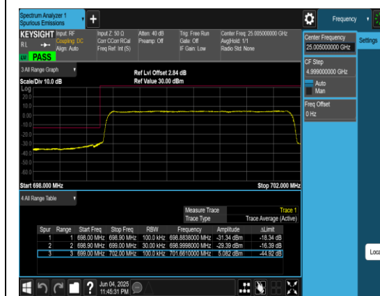
Band12_3MHz_QPSK_23025_15RB#0
