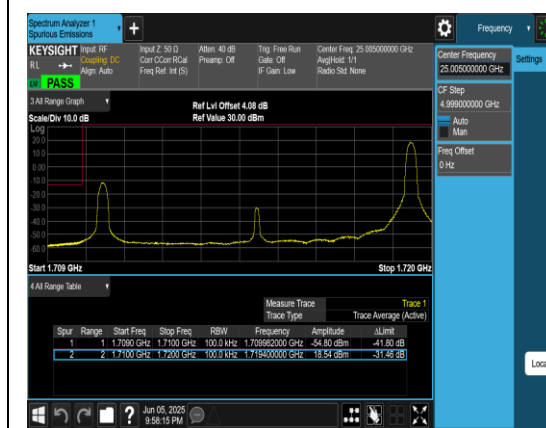
Band66_10MHz_QPSK_132022_1RB#49
