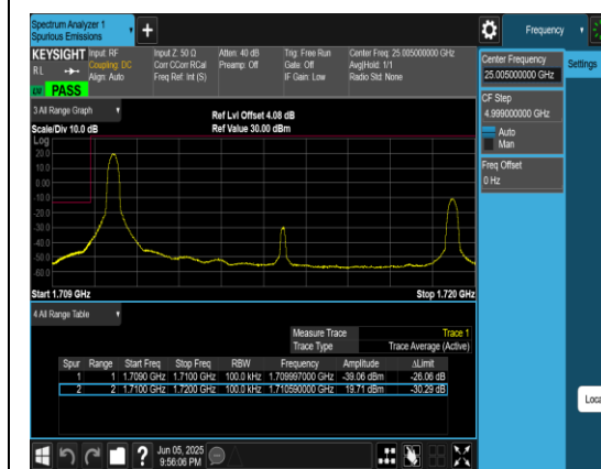
Band66_10MHz_QPSK_132022_1RB#0
