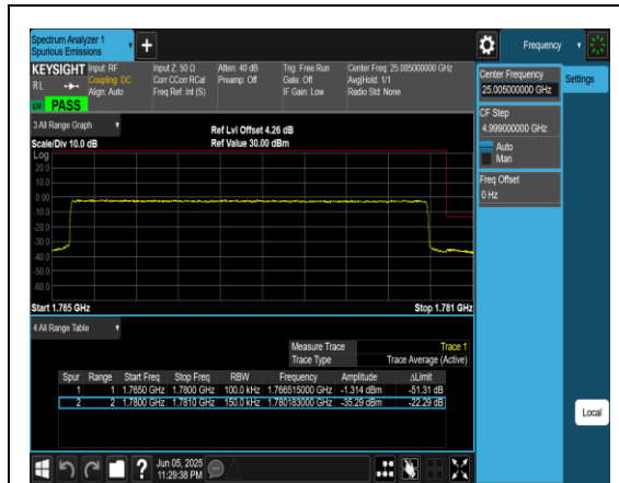
Band66_15MHz_QPSK_132597_75RB#0
