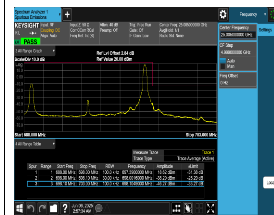
Band71_10MHz_QPSK_133422_1RB#49
