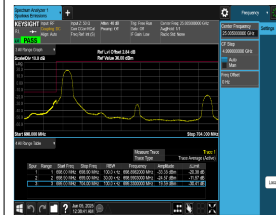
Band12_5MHz_QPSK_23035_1RB#0
