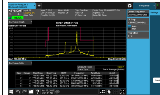
Band13_5MHz_QPSK_23255_1RB#24
