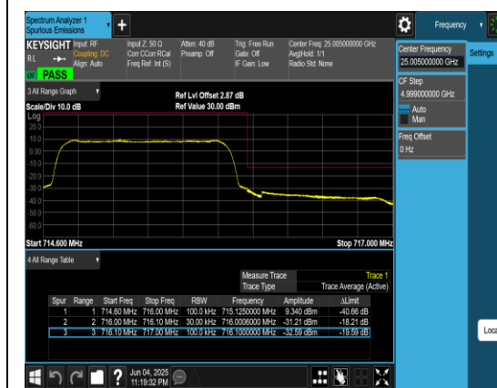
Band12_1.4MHz_QPSK_23173_6RB#0
