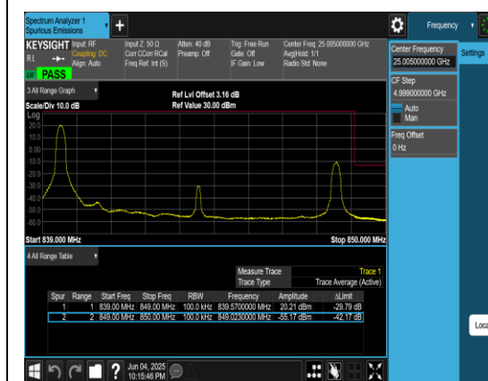
Band5_10MHz_QPSK_20600_1RB#0
