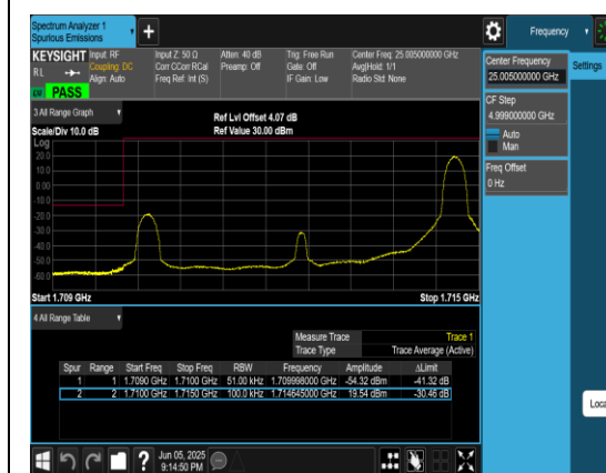
Band66_5MHz_QPSK_131997_1RB#24
