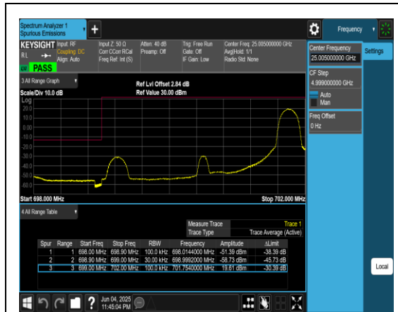
Band12_3MHz_QPSK_23025_1RB#14
