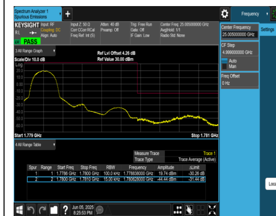
Band66_1.4MHz_QPSK_132665_1RB#0
