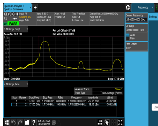
Band66_3MHz_QPSK_131987_1RB#0
