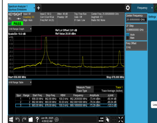
Band71_15MHz_QPSK_133197_1RB#0
