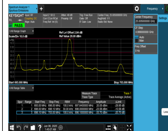
Band71_5MHz_QPSK_133447_1RB#24
