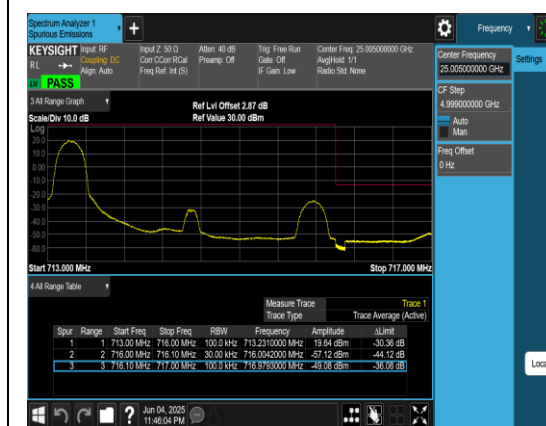
Band12_3MHz_QPSK_23165_1RB#0
