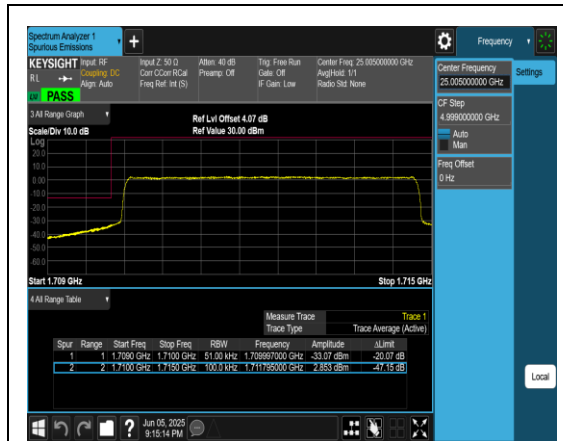
Band66_5MHz_QPSK_131997_25RB#0
