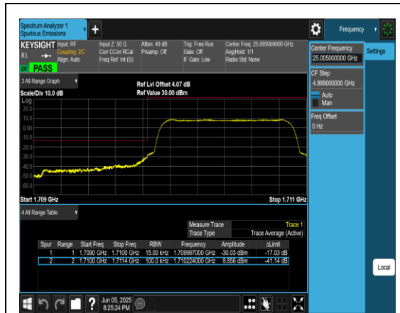
Band66_1.4MHz_QPSK_131979_6RB#0
