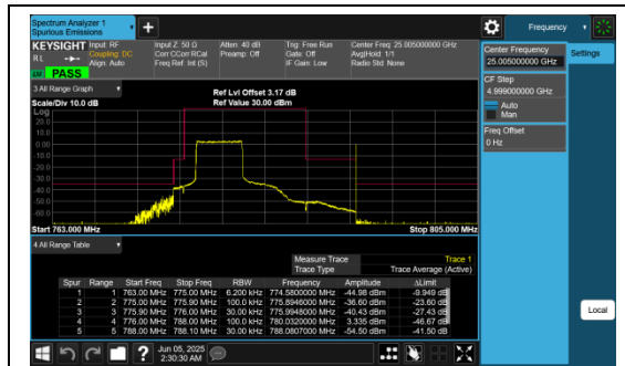
Band13_5MHz_QPSK_23205_25RB#0
