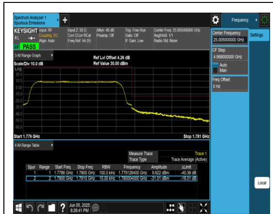
Band66_1.4MHz_QPSK_132665_6RB#0
