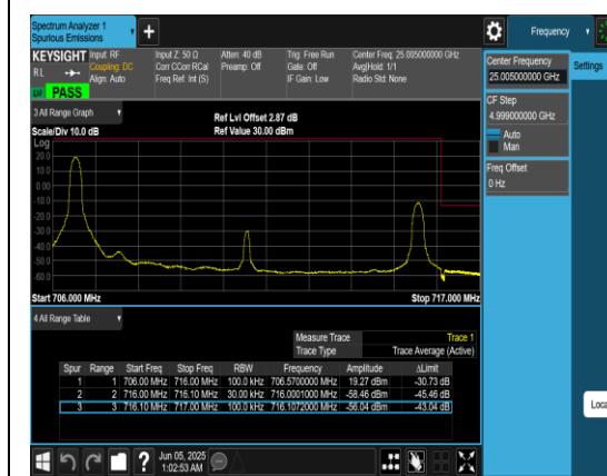
Band12_10MHz_QPSK_23130_1RB#0
