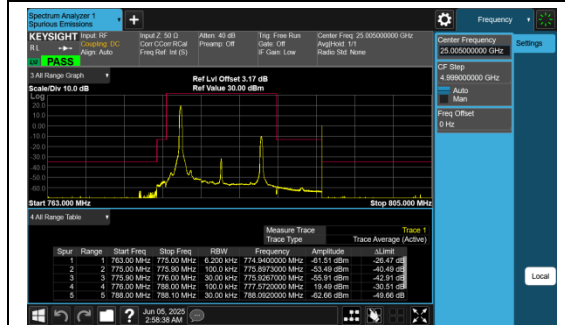
Band13_5MHz_QPSK_23255_25RB#0
