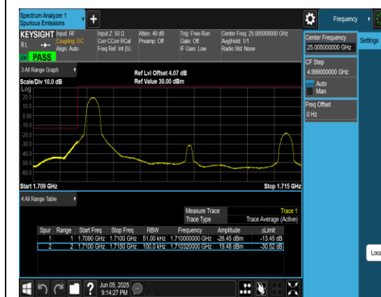
Band66_5MHz_QPSK_131997_1RB#0
