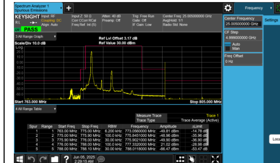
Band13_5MHz_QPSK_23205_1RB#0
