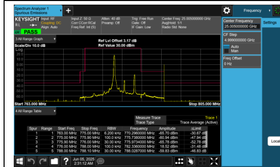
Band13_5MHz_QPSK_23255_1RB#0
