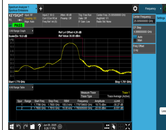
Band66_1.4MHz_QPSK_132665_1RB#5
