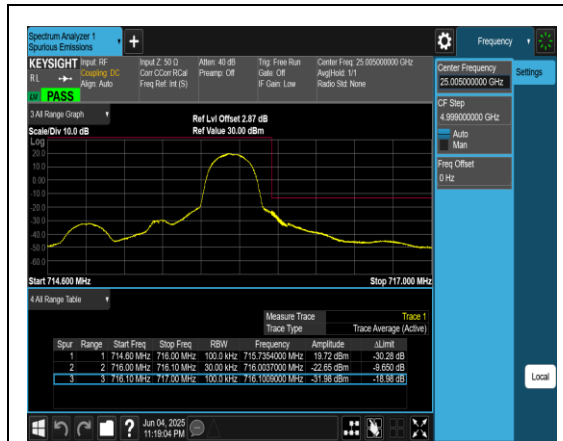
Band12_1.4MHz_QPSK_23173_1RB#5
