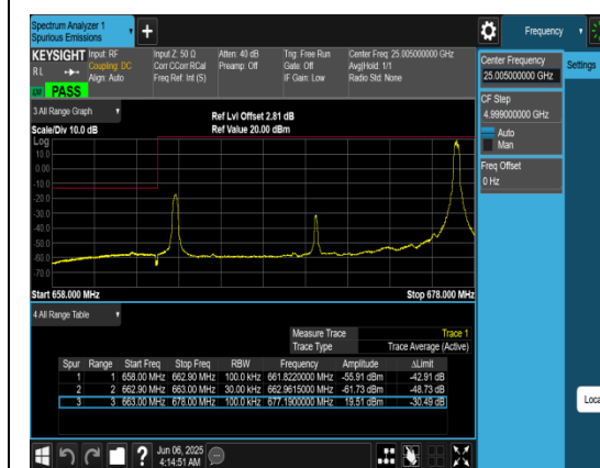
Band71_15MHz_QPSK_133197_1RB#74
