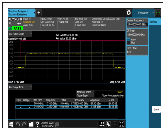
Band66_15MHz_QPSK_132047_75RB#0
