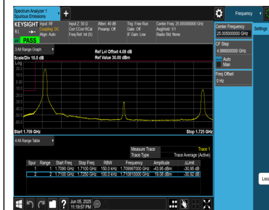
Band66_15MHz_QPSK_132047_1RB#0
