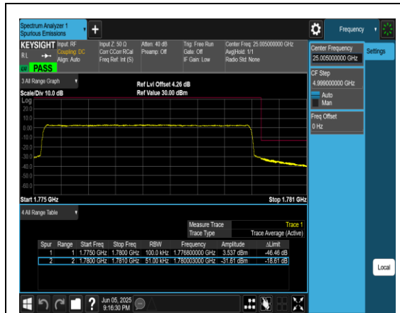
Band66_5MHz_QPSK_132647_25RB#0
