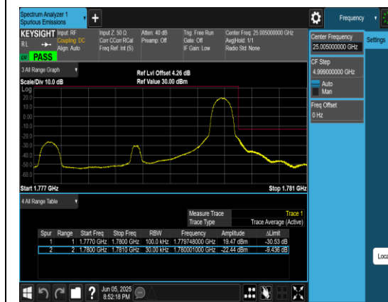
Band66_3MHz_QPSK_132657_1RB#14
