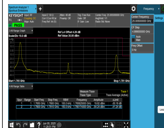
Band66_15MHz_QPSK_132597_1RB#0
