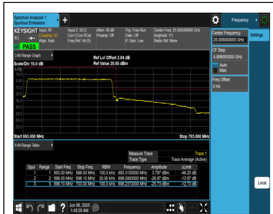
Band71_5MHz_QPSK_133447_25RB#0
