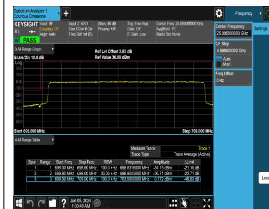
Band12_10MHz_QPSK_23060_50RB#0
