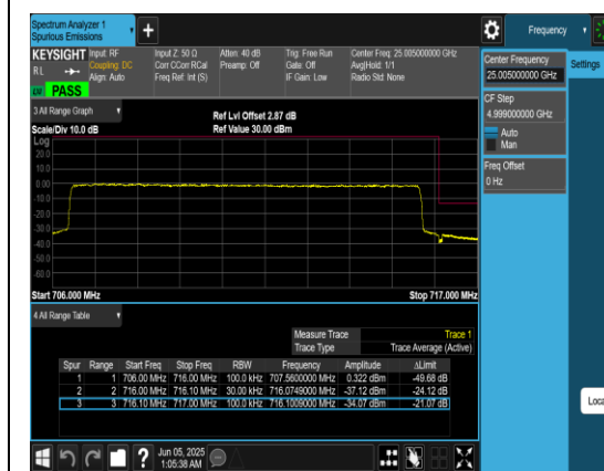
Band12_10MHz_QPSK_23130_50RB#0
