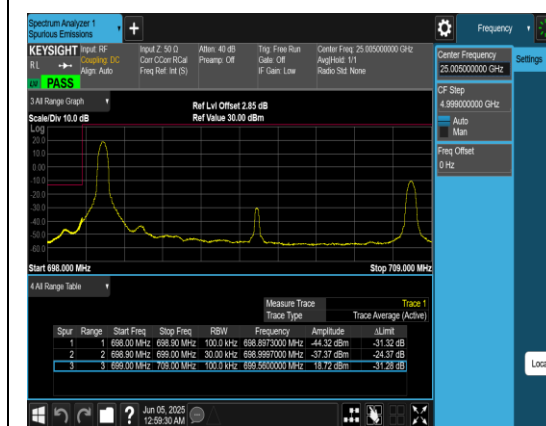
Band12_10MHz_QPSK_23060_1RB#0
