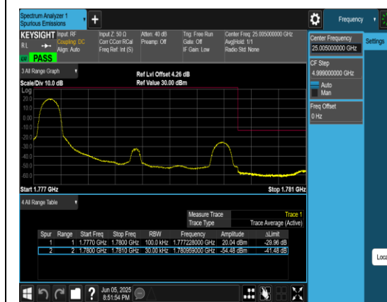
Band66_3MHz_QPSK_132657_1RB#0
