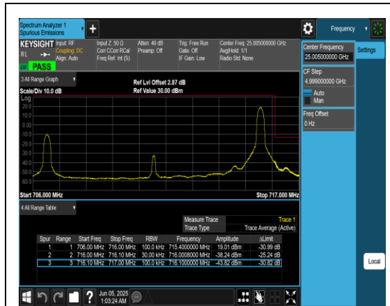
Band12_10MHz_QPSK_23130_1RB#49
