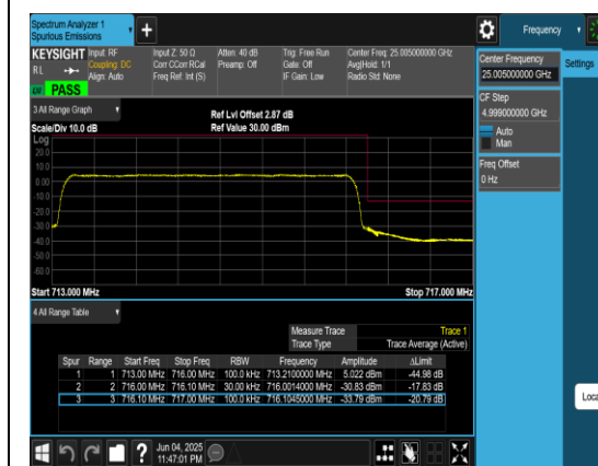
Band12_3MHz_QPSK_23165_15RB#0
