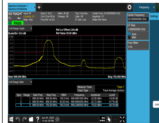
Band12_3MHz_QPSK_23025_1RB#0
