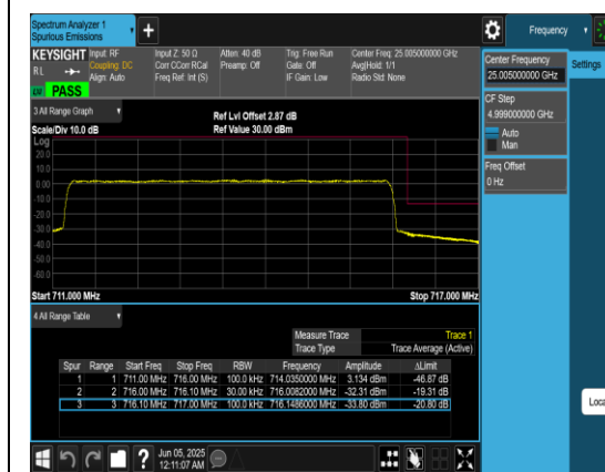
Band12_5MHz_QPSK_23155_25RB#0
