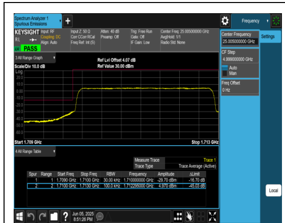
Band66_3MHz_QPSK_131987_15RB#0
