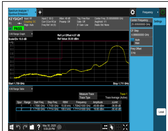
Band4_1.4MHz_QPSK_19957_1RB#5
