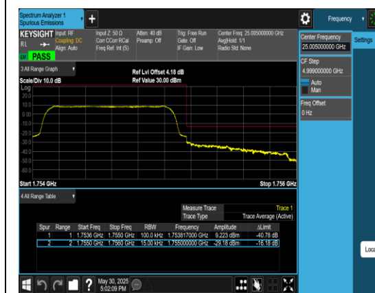
Band4_1.4MHz_QPSK_20393_6RB#0
