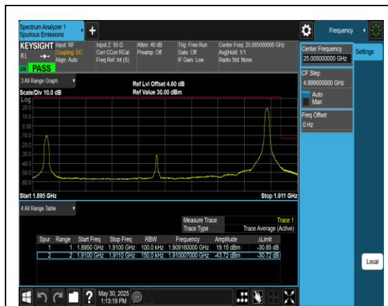
Band2_15MHz_QPSK_19125_1RB#74
