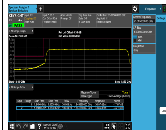
Band2_3MHz_QPSK_18615_15RB#0
