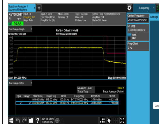
Band5_5MHz_QPSK_20625_25RB#0
