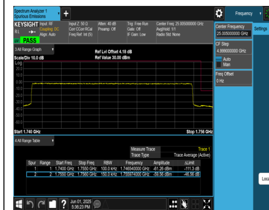
Band4_15MHz_QPSK_20325_75RB#0
