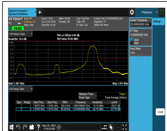
Band2_3MHz_QPSK_19185_1RB#14
