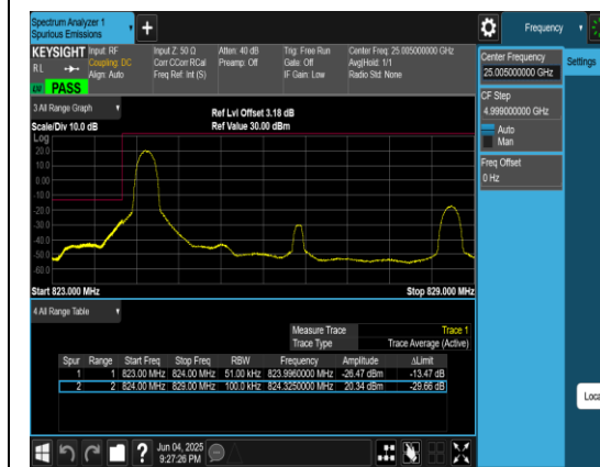
Band5_5MHz_QPSK_20425_1RB#0
