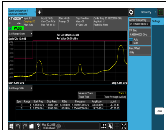
Band2_5MHz_QPSK_18625_1RB#24
