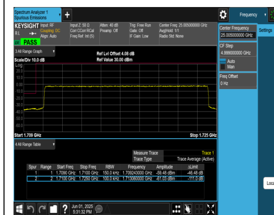
Band4_15MHz_QPSK_20025_75RB#0
