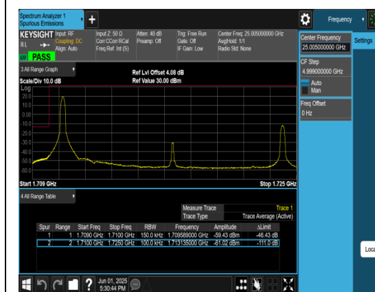
Band4_15MHz_QPSK_20025_1RB#0
