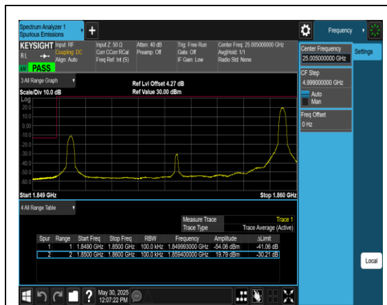
Band2_10MHz_QPSK_18650_1RB#49
