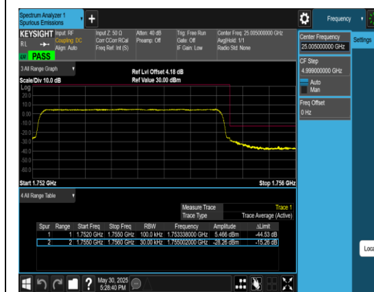
Band4_3MHz_QPSK_20385_15RB#0
