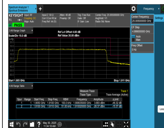
Band2_5MHz_QPSK_19175_25RB#0
