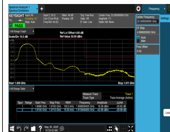
Band2_1.4MHz_QPSK_19193_1RB#0
