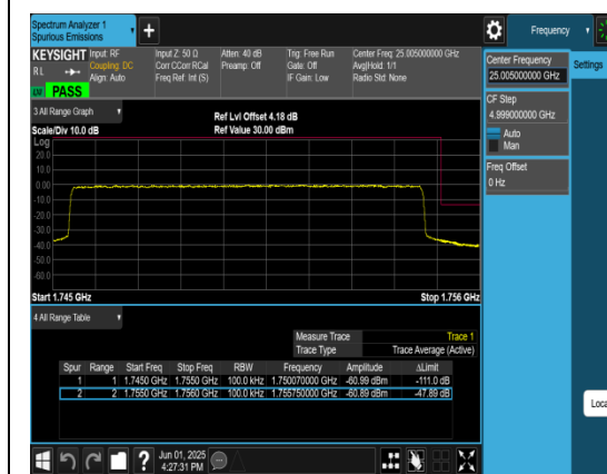
Band4_10MHz_QPSK_20350_50RB#0
