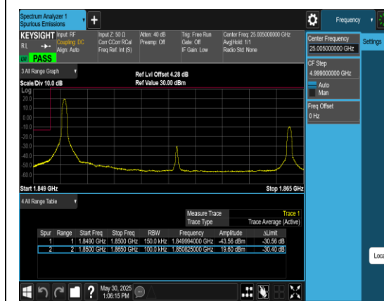
Band2_15MHz_QPSK_18675_1RB#0
