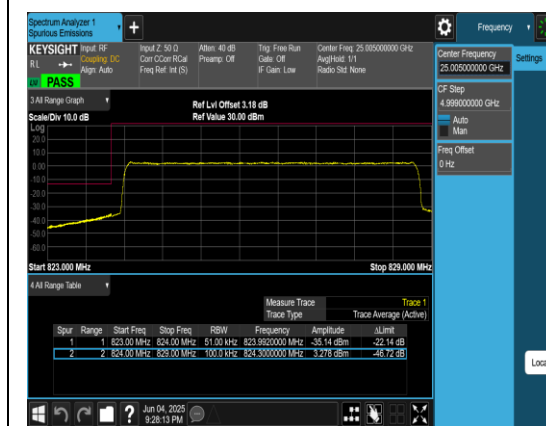
Band5_5MHz_QPSK_20425_25RB#0
