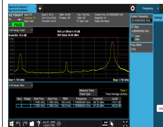
Band4_10MHz_QPSK_20350_1RB#0
