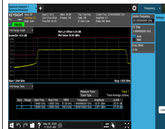
Band2_5MHz_QPSK_18625_25RB#0
