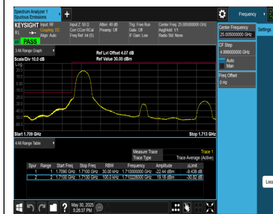
Band4_3MHz_QPSK_19965_1RB#0
