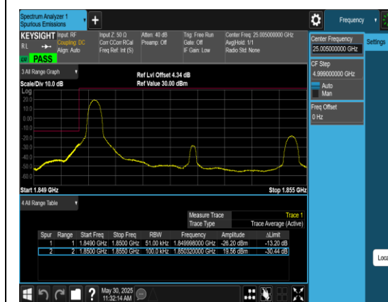
Band2_5MHz_QPSK_18625_1RB#0
