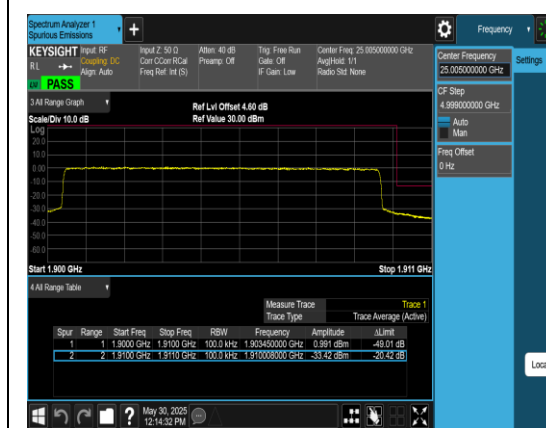
Band2_10MHz_QPSK_19150_50RB#0
