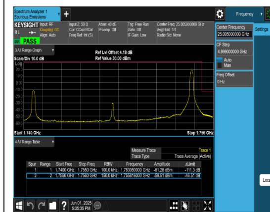
Band4_15MHz_QPSK_20325_1RB#0
