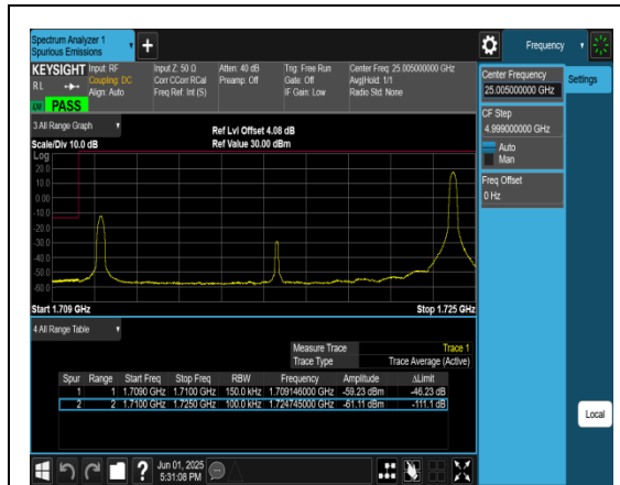
Band4_15MHz_QPSK_20025_1RB#74
