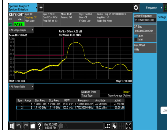
Band4_1.4MHz_QPSK_19957_1RB#0
