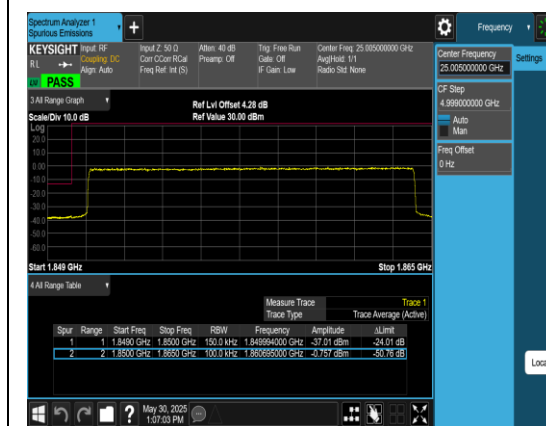
Band2_15MHz_QPSK_18675_75RB#0
