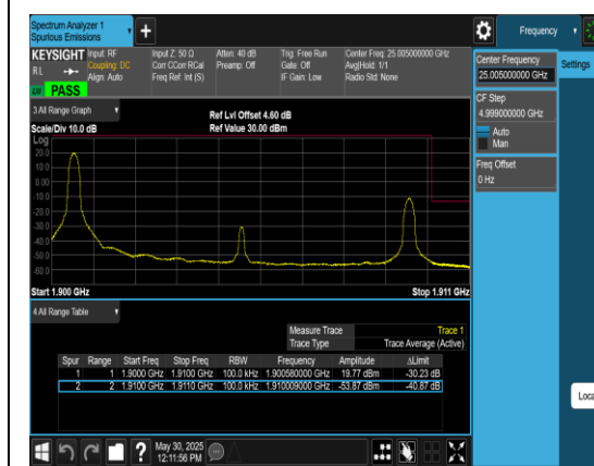
Band2_10MHz_QPSK_19150_1RB#0
