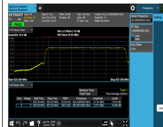
Band5_3MHz_QPSK_20415_15RB#0
