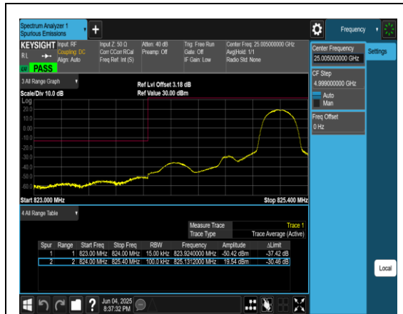
Band5_1.4MHz_QPSK_20407_1RB#5
