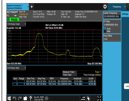
Band5_3MHz_QPSK_20415_1RB#0
