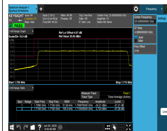
Band4_5MHz_QPSK_19975_25RB#0
