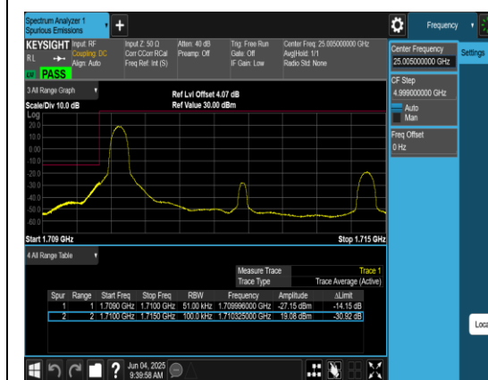
Band4_5MHz_QPSK_19975_1RB#0
