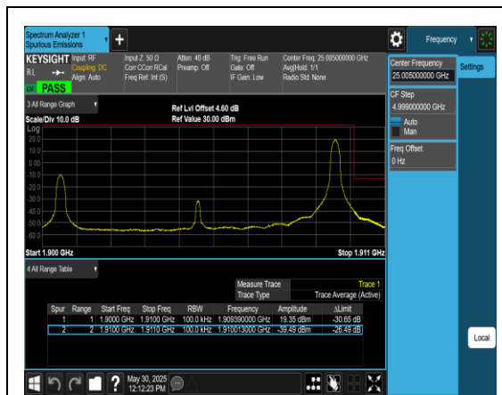
Band2_10MHz_QPSK_19150_1RB#49
