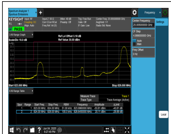
Band5_5MHz_QPSK_20425_1RB#24
