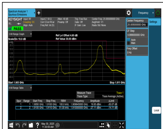
Band2_5MHz_QPSK_19175_1RB#24
