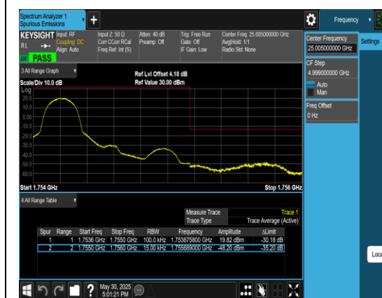
Band4_1.4MHz_QPSK_20393_1RB#0
