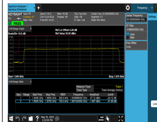
Band2_20MHz_QPSK_18700_100RB#0
