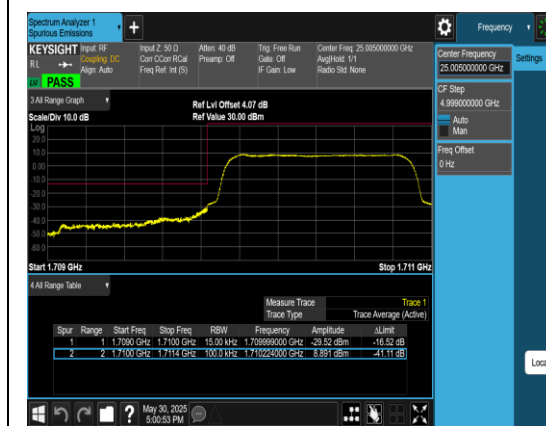
Band4_1.4MHz_QPSK_19957_6RB#0
