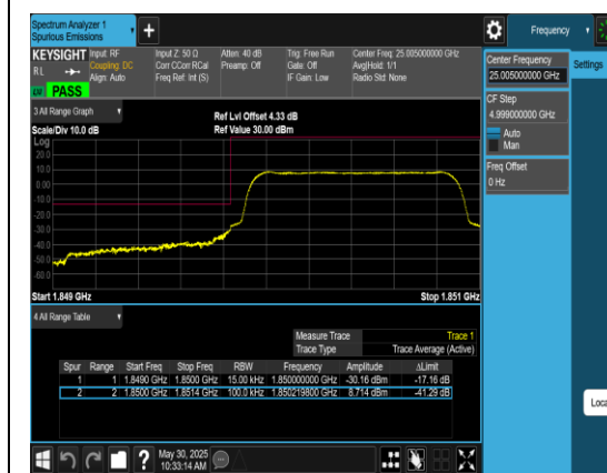
Band2_1.4MHz_QPSK_18607_6RB#0
