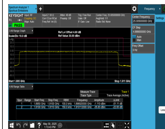
Band2_15MHz_QPSK_19125_75RB#0
