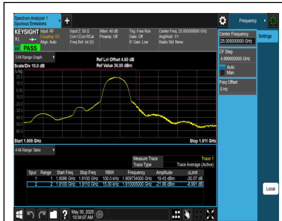
Band2_1.4MHz_QPSK_19193_1RB#5
