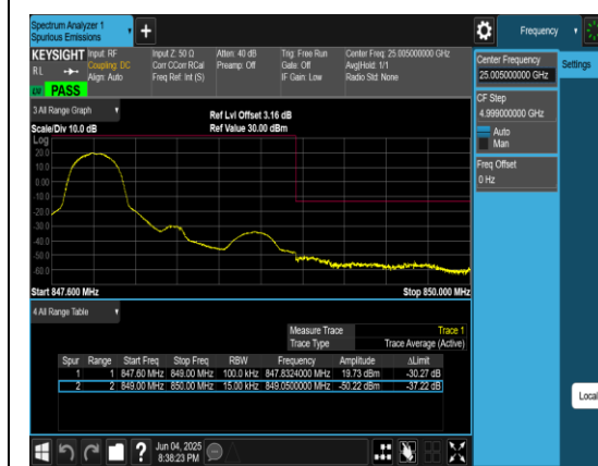
Band5_1.4MHz_QPSK_20643_1RB#0
