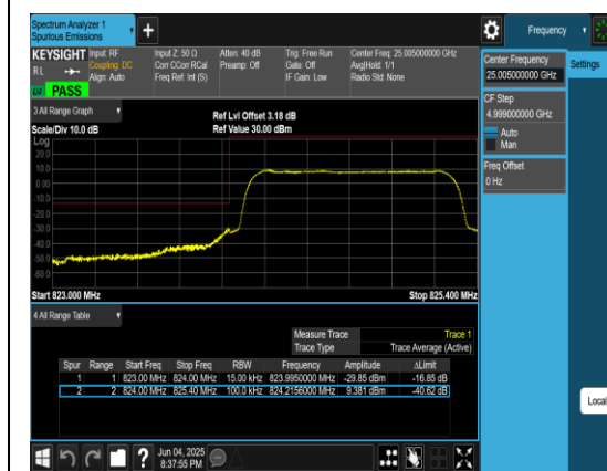
Band5_1.4MHz_QPSK_20407_6RB#0
