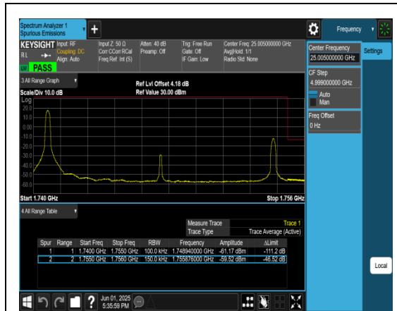
Band4_15MHz_QPSK_20325_1RB#74
