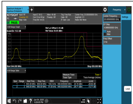
Band5_5MHz_QPSK_20625_1RB#24
