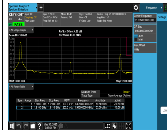
Band2_20MHz_QPSK_19100_1RB#0
