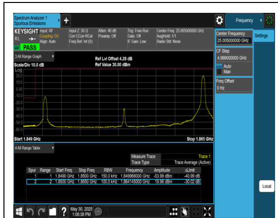
Band2_15MHz_QPSK_18675_1RB#74
