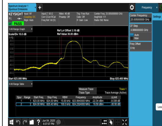
Band5_1.4MHz_QPSK_20407_1RB#0
