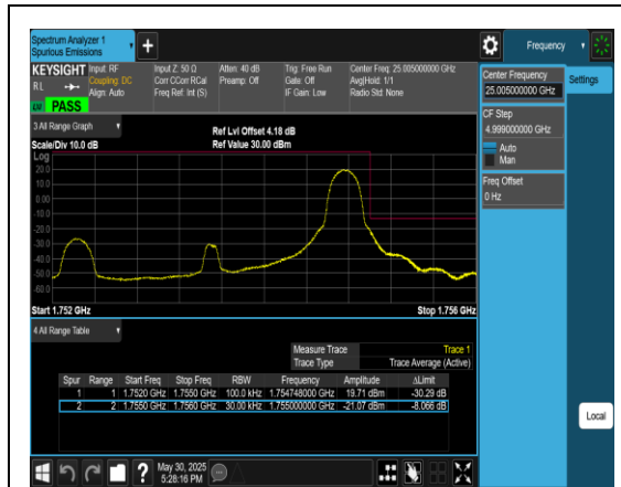
Band4_3MHz_QPSK_20385_1RB#14
