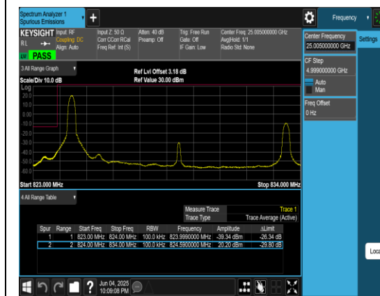
Band5_10MHz_QPSK_20450_1RB#0
