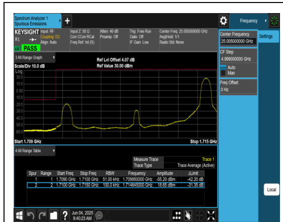
Band4_5MHz_QPSK_19975_1RB#24
