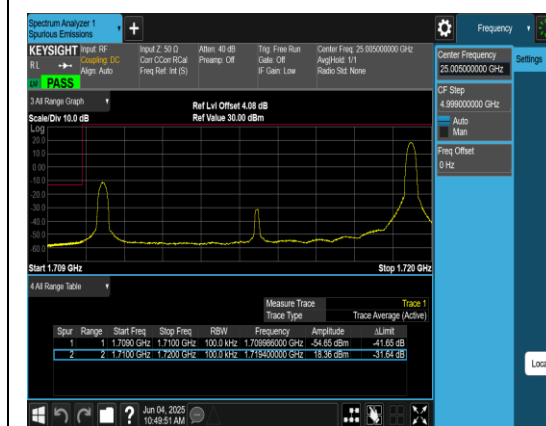
Band4_10MHz_QPSK_20000_1RB#49
