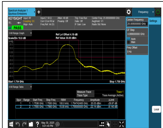
Band4_1.4MHz_QPSK_20393_1RB#5
