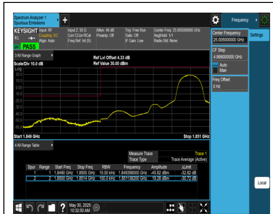
Band2_1.4MHz_QPSK_18607_1RB#5
