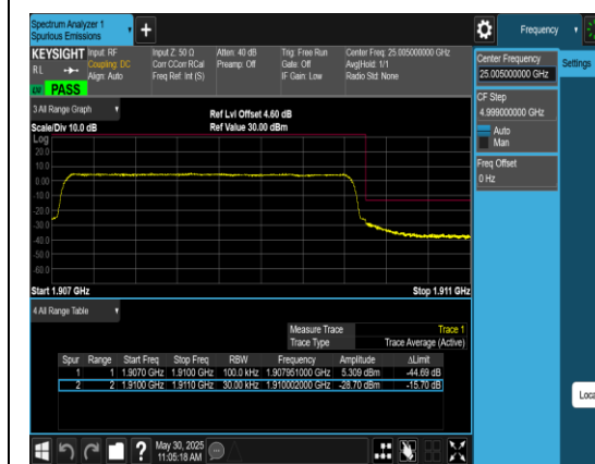
Band2_3MHz_QPSK_19185_15RB#0
