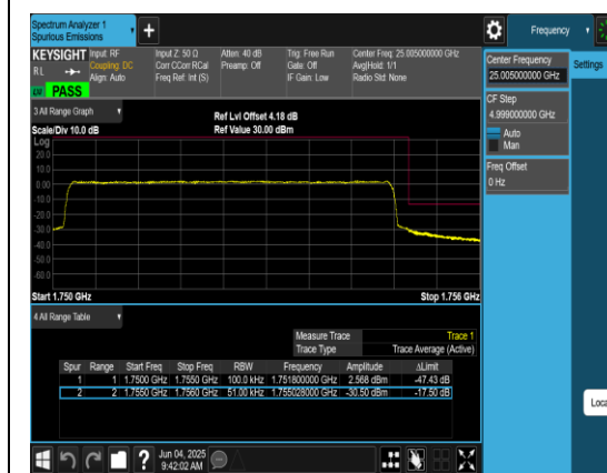
Band4_5MHz_QPSK_20375_25RB#0
