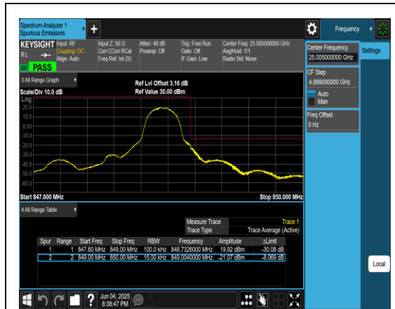
Band5_1.4MHz_QPSK_20643_1RB#5
