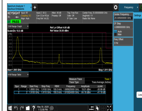
Band2_15MHz_QPSK_19125_1RB#0
