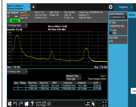
Band4_5MHz_QPSK_20375_1RB#0
