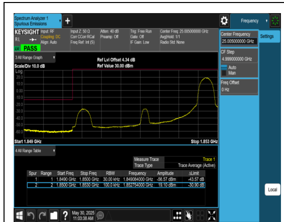
Band2_3MHz_QPSK_18615_1RB#14
