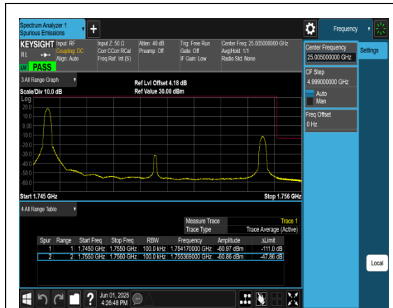
Band4_10MHz_QPSK_20350_1RB#49
