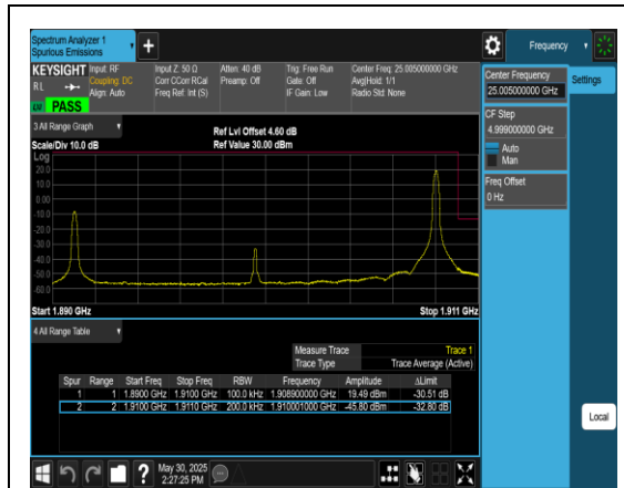
Band2_20MHz_QPSK_19100_1RB#99
