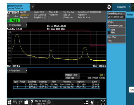
Band2_5MHz_QPSK_19175_1RB#0
