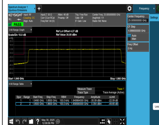
Band2_10MHz_QPSK_18650_50RB#0
