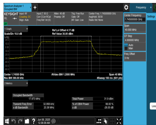
Band66-20MHz-QPSK-132322-100RB#0-PASS
