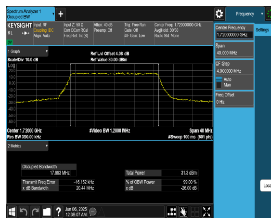
Band66-20MHz-QPSK-132072-100RB#0-PASS
