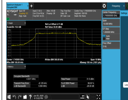
Band66-5MHz-QPSK-132322-25RB#0-PASS
