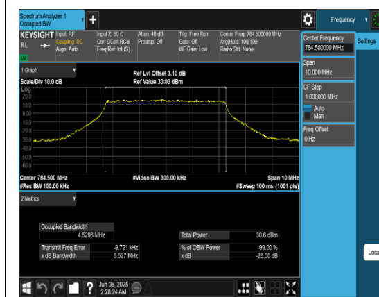
Band13-5MHz-QPSK-23255-25RB#0-PASS
