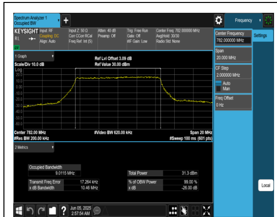
Band13-10MHz-QPSK-23230-50RB#0-PASS
