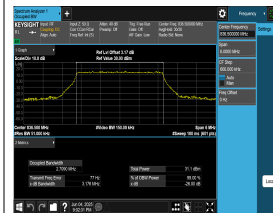
Band5-3MHz-QPSK-20525-15RB#0-PASS
