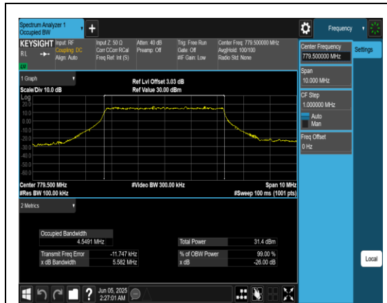
Band13-5MHz-QPSK-23205-25RB#0-PASS
