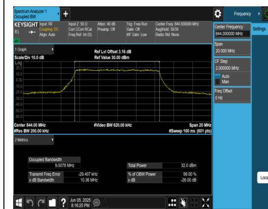
Band5-10MHz-QPSK-20600-50RB#0-PASS
