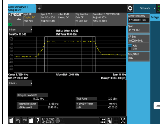
Band4-20MHz-QPSK-20175-100RB#0-PASS
