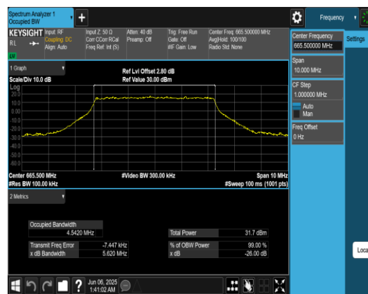
Band71-5MHz-QPSK-133147-25RB#0-PASS
