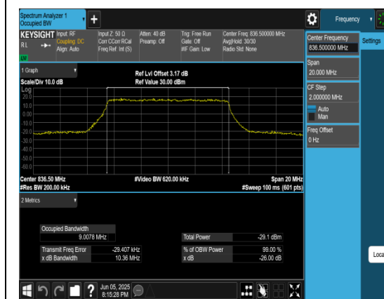
Band5-10MHz-QPSK-20525-50RB#0-PASS
