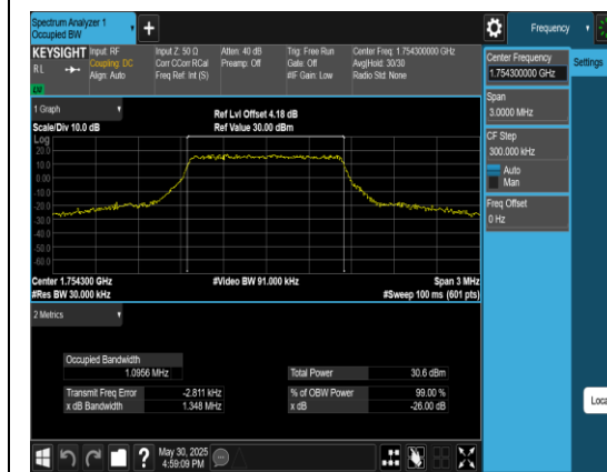
Band4-1.4MHz-QPSK-20393-6RB#0-PASS
