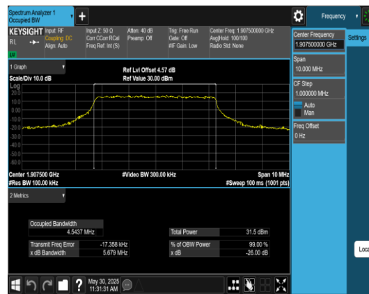
Band2-5MHz-QPSK-19175-25RB#0-PASS
