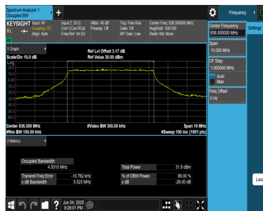
Band5-5MHz-QPSK-20525-25RB#0-PASS
