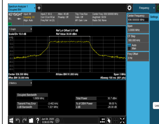
Band5-1.4MHz-QPSK-20525-6RB#0-PASS
