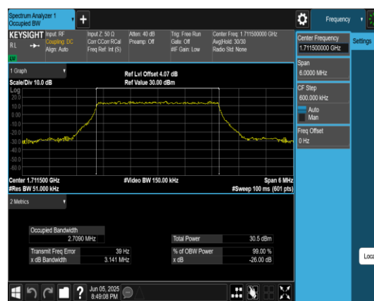
Band66-3MHz-QPSK-131987-15RB#0-PASS
