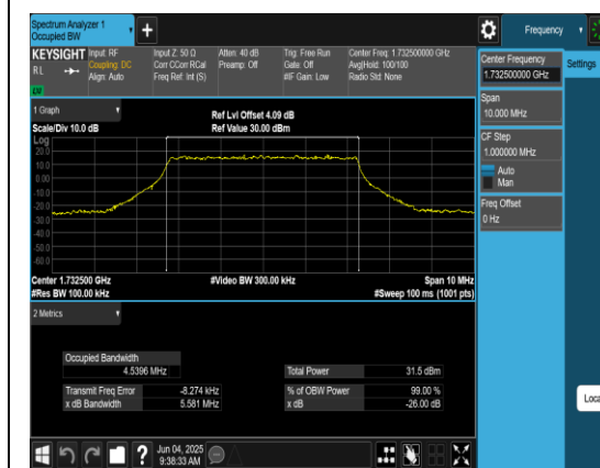
Band4-5MHz-QPSK-20175-25RB#0-PASS
