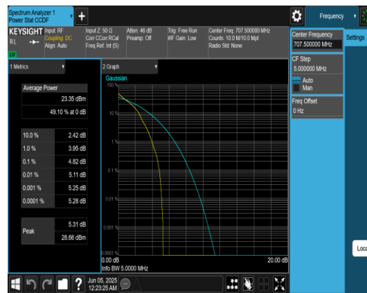
Band12-5MHz-QPSK-23095-1RB#0-PASS
