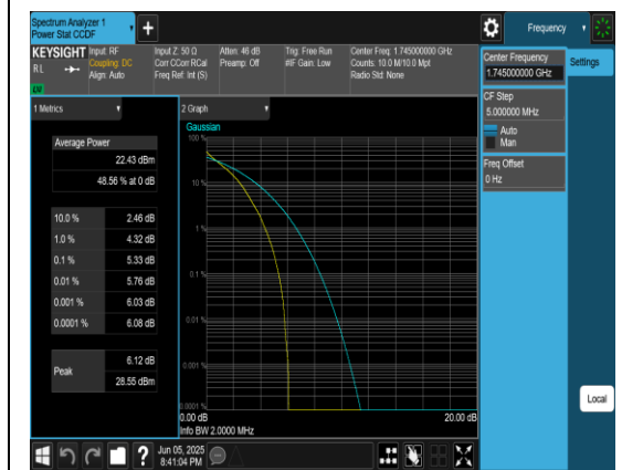
Band66-1.4MHz-QPSK-132322-6RB#0-PASS
