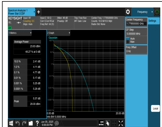
Band66-3MHz-QPSK-132657-1RB#0-PASS
