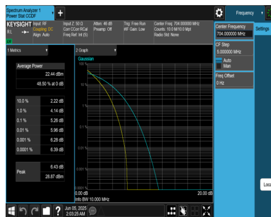
Band12-10MHz-QPSK-23060-50RB#0-PASS
