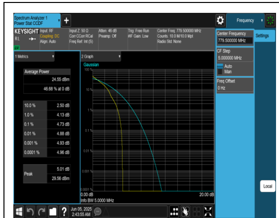
Band13-5MHz-QPSK-23205-1RB#0-PASS
