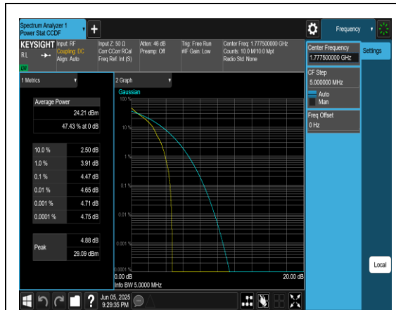
Band66-5MHz-QPSK-132647-1RB#0-PASS
