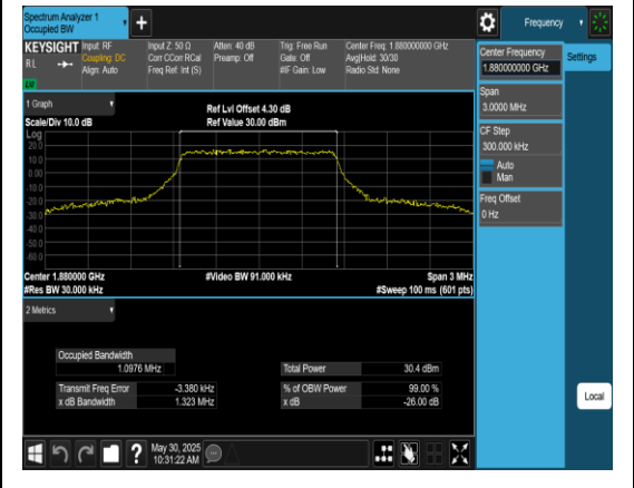
Band2-1.4MHz-QPSK-18900-6RB#0-PASS
