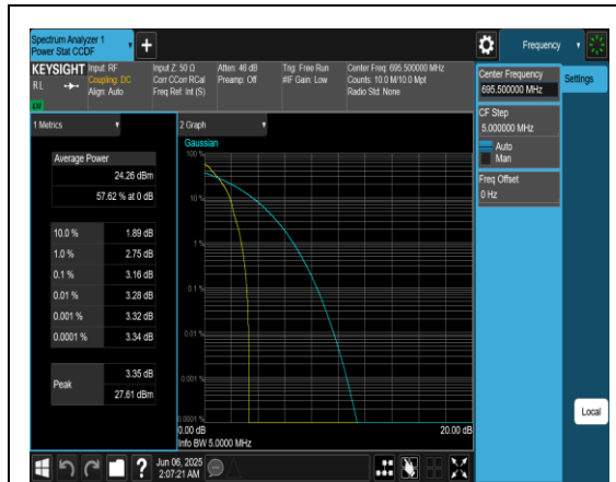
Band71-5MHz-QPSK-133447-1RB#0-PASS
