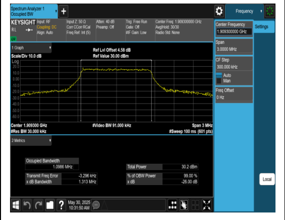
Band2-1.4MHz-QPSK-19193-6RB#0-PASS
