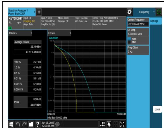
Band12-5MHz-QPSK-23095-25RB#0-PASS
