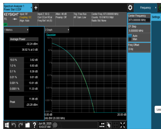
Band71-20MHz-QPSK-133222-1RB#0-PASS
