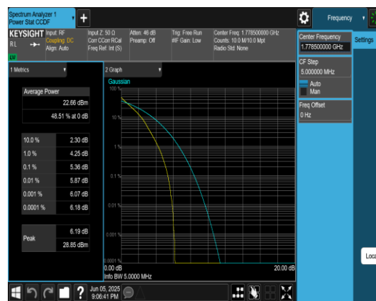
Band66-3MHz-QPSK-132657-15RB#0-PASS
