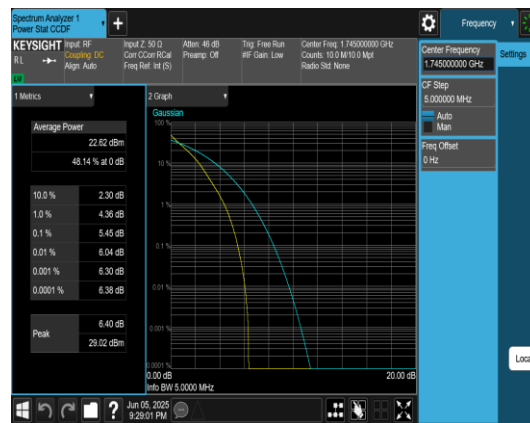
Band66-5MHz-QPSK-132322-25RB#0-PASS
