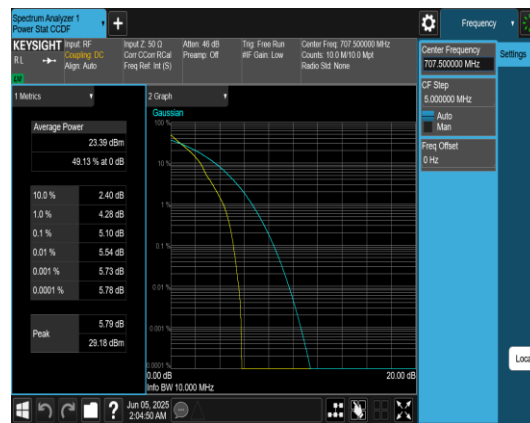
Band12-10MHz-QPSK-23095-1RB#0-PASS
