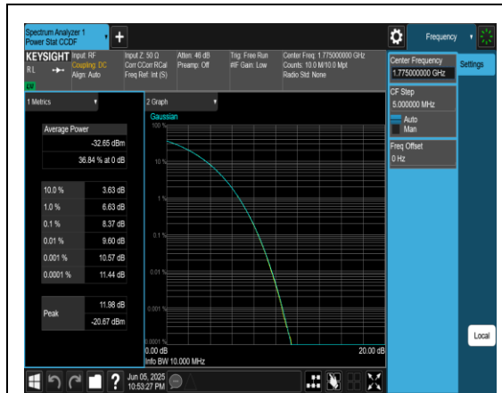
Band66-10MHz-QPSK-132622-1RB#0-PASS
