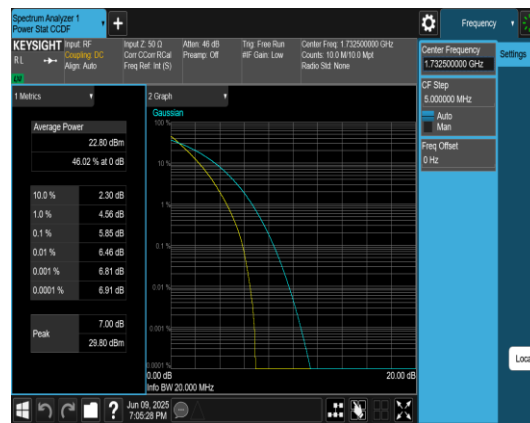
Band4-20MHz-QPSK-20175-100RB#0-PASS
