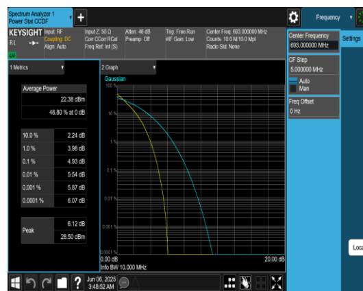
Band71-10MHz-QPSK-133422-50RB#0-PASS
