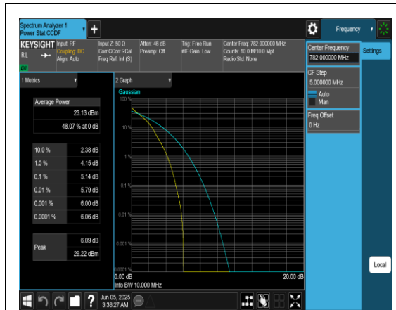
Band13-10MHz-QPSK-23230-1RB#0-PASS
