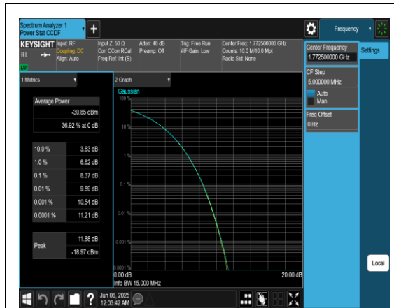
Band66-15MHz-QPSK-132597-1RB#0-PASS
