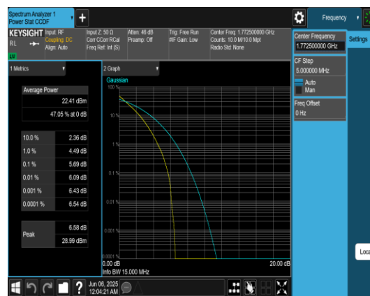
Band66-15MHz-QPSK-132597-75RB#0-PASS
