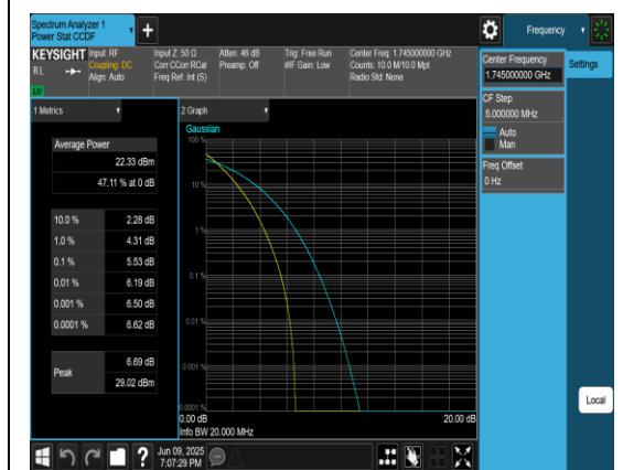
Band4-20MHz-QPSK-20300-100RB#0-PASS
