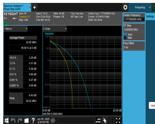
Band66-5MHz-QPSK-132647-25RB#0-PASS
