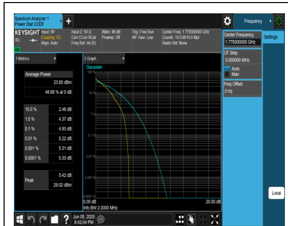
Band66-1.4MHz-QPSK-132665-1RB#0-PASS
