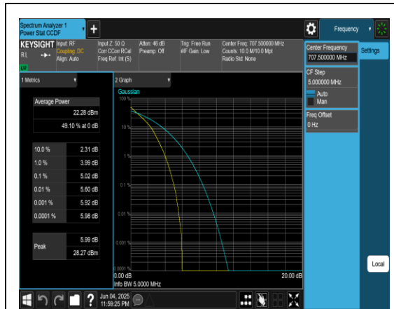
Band12-3MHz-QPSK-23095-15RB#0-PASS
