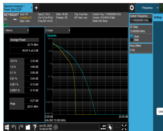
Band66-10MHz-QPSK-132322-1RB#0-PASS
