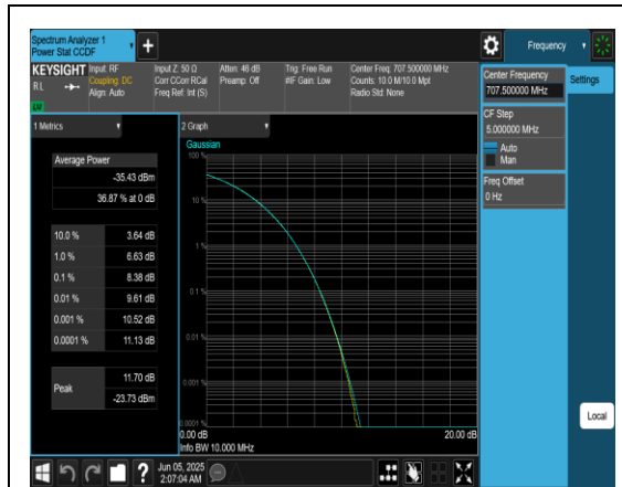
Band12-10MHz-QPSK-23095-50RB#0-PASS
