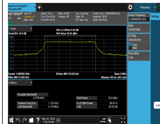
Band2-3MHz-QPSK-19185-15RB#0-PASS
