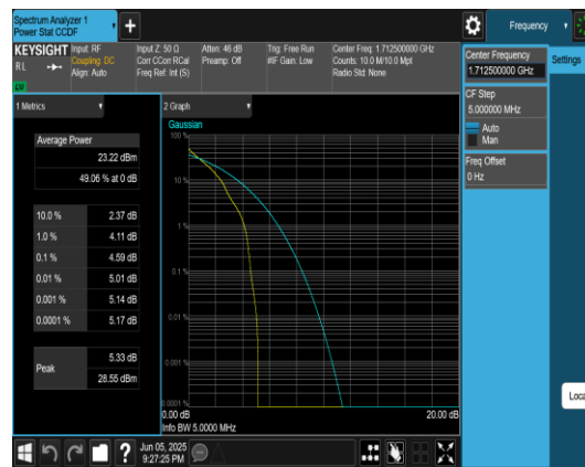
Band66-5MHz-QPSK-131997-1RB#0-PASS
