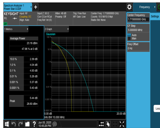
Band66-10MHz-QPSK-132022-1RB#0-PASS
