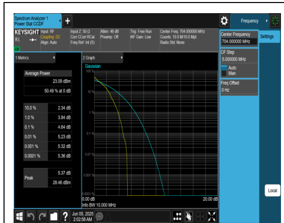
Band12-10MHz-QPSK-23060-1RB#0-PASS
