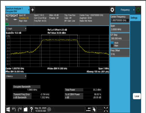
Band2-1.4MHz-QPSK-18607-6RB#0-PASS
