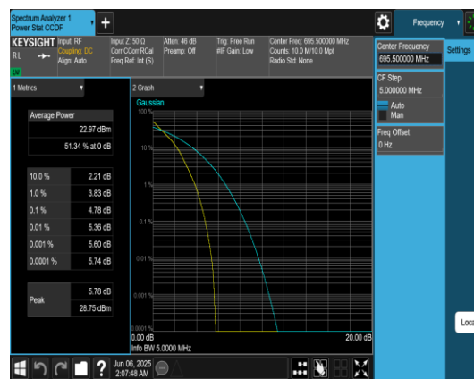
Band71-5MHz-QPSK-133447-25RB#0-PASS
