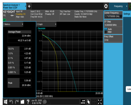
Band66-1.4MHz-QPSK-131979-1RB#0-PASS
