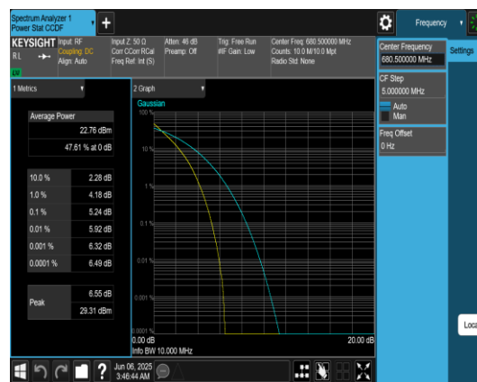
Band71-10MHz-QPSK-133297-50RB#0-PASS
