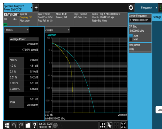
Band66-3MHz-QPSK-132322-1RB#0-PASS
