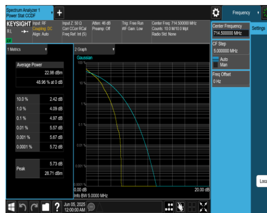
Band12-3MHz-QPSK-23165-1RB#0-PASS
