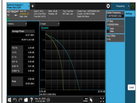
Band2-5MHz-QPSK-19175-25RB#0-PASS
