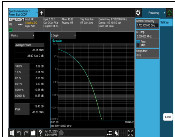
Band4-15MHz-QPSK-20175-75RB#0-PASS
