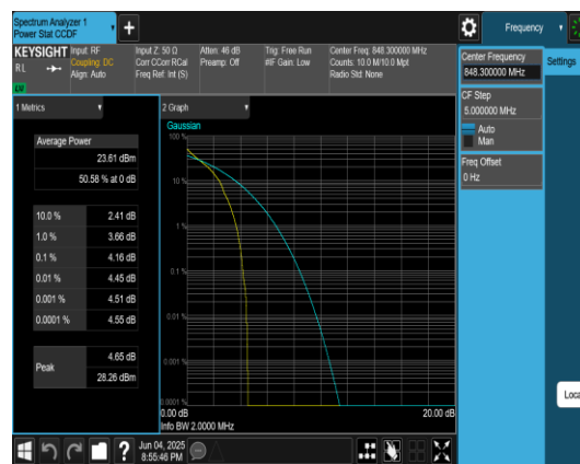
Band5-1.4MHz-QPSK-20643-1RB#0-PASS
