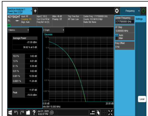
Band4-15MHz-QPSK-20025-1RB#0-PASS
