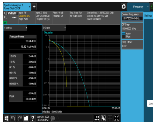
Band2-15MHz-QPSK-18675-1RB#0-PASS
