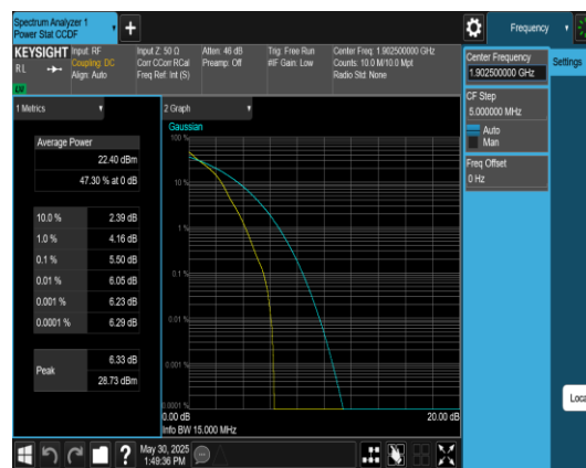
Band2-15MHz-QPSK-19125-1RB#0-PASS
