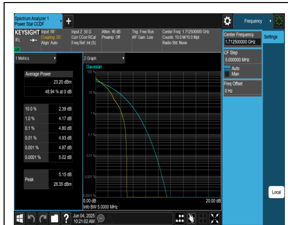
Band4-5MHz-QPSK-19975-1RB#0-PASS
