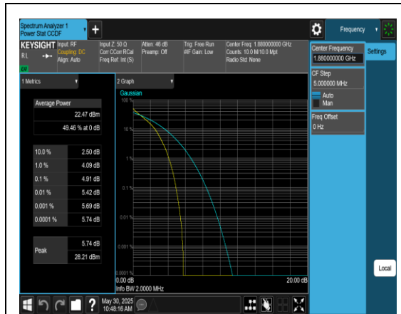
Band2-1.4MHz-QPSK-18900-6RB#0-PASS
