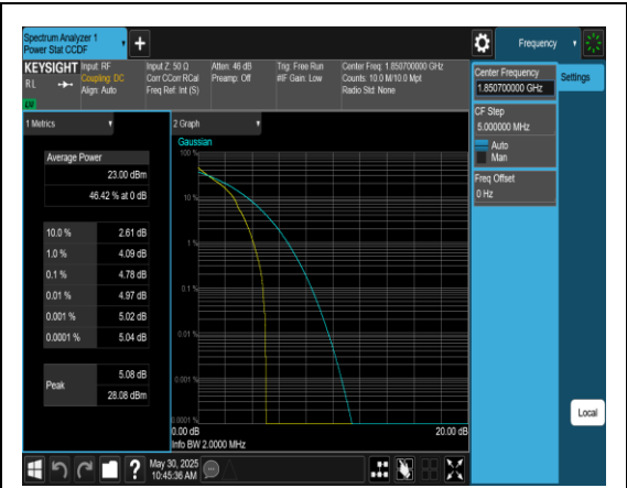
Band2-1.4MHz-QPSK-18607-1RB#0-PASS
