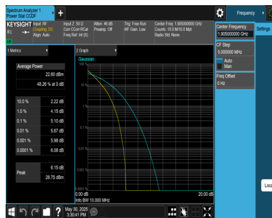
Band2-10MHz-QPSK-19150-50RB#0-PASS
