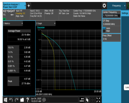
Band4-5MHz-QPSK-20375-1RB#0-PASS
