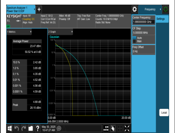
Band2-1.4MHz-QPSK-18900-1RB#0-PASS
