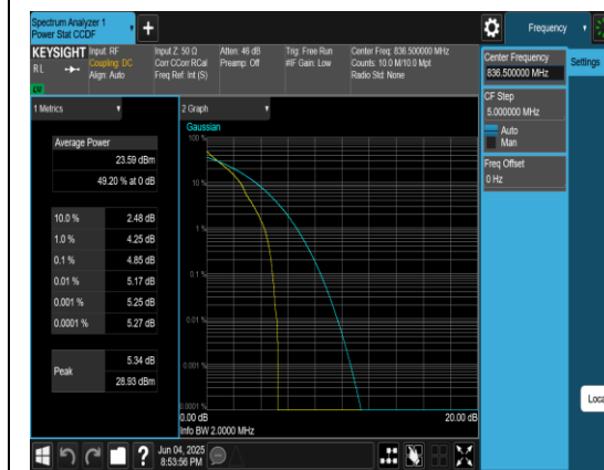
Band5-1.4MHz-QPSK-20525-1RB#0-PASS
