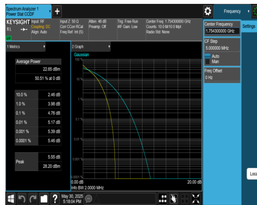
Band4-1.4MHz-QPSK-20393-6RB#0-PASS
