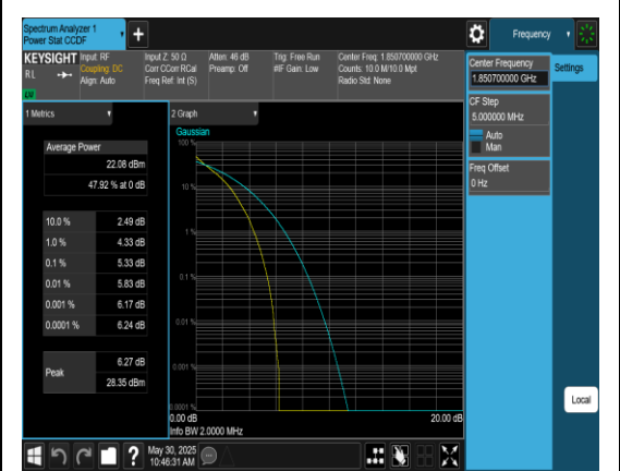
Band2-1.4MHz-QPSK-18607-6RB#0-PASS
