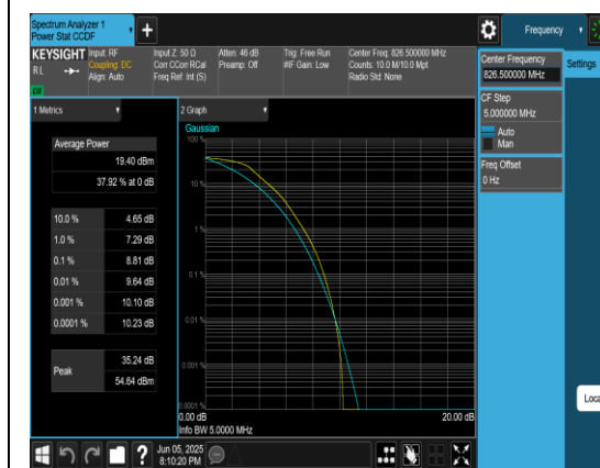
Band5-5MHz-QPSK-20425-25RB#0-PASS
