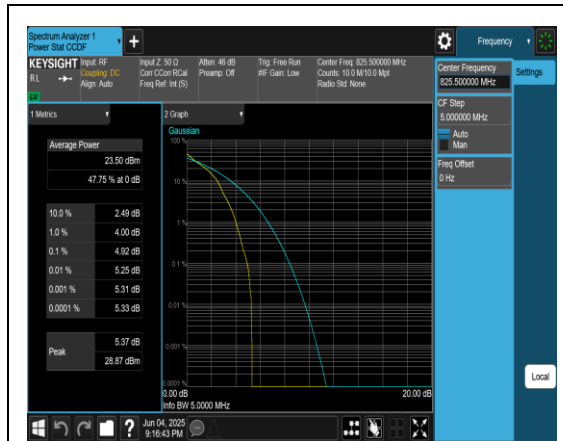
Band5-3MHz-QPSK-20415-1RB#0-PASS
