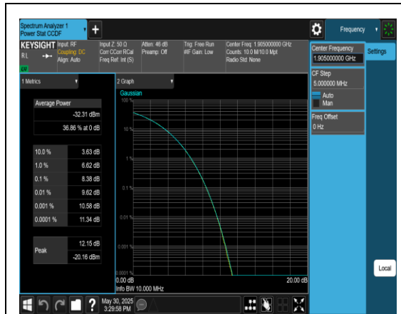
Band2-10MHz-QPSK-19150-1RB#0-PASS
