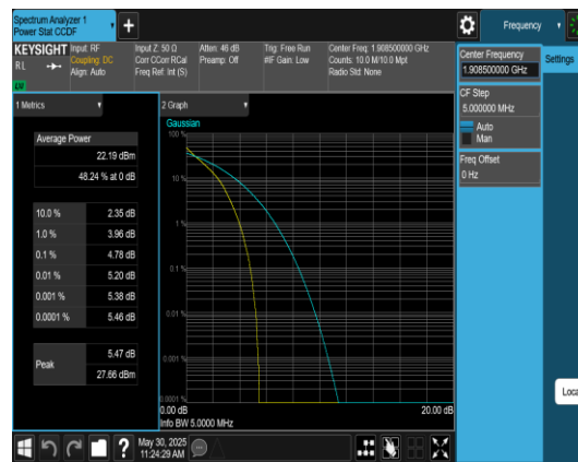
Band2-3MHz-QPSK-19185-15RB#0-PASS
