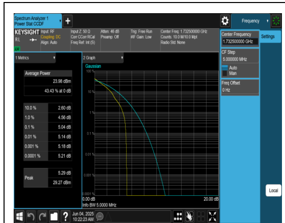
Band4-5MHz-QPSK-20175-1RB#0-PASS
