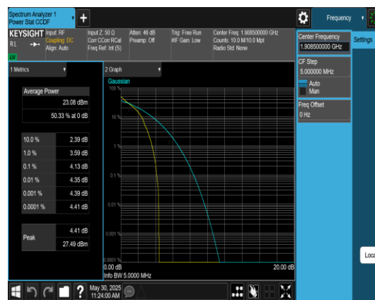
Band2-3MHz-QPSK-19185-1RB#0-PASS
