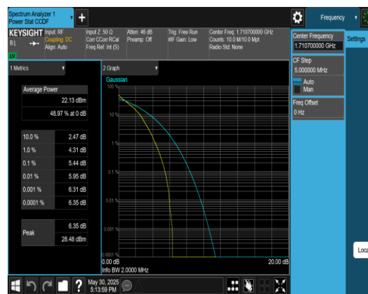
Band4-1.4MHz-QPSK-19957-6RB#0-PASS
