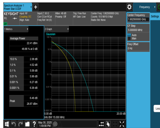
Band2-15MHz-QPSK-19125-75RB#0-PASS
