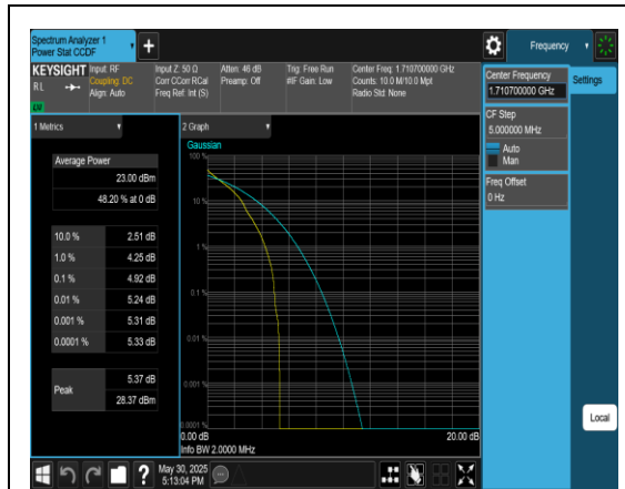
Band4-1.4MHz-QPSK-19957-1RB#0-PASS
