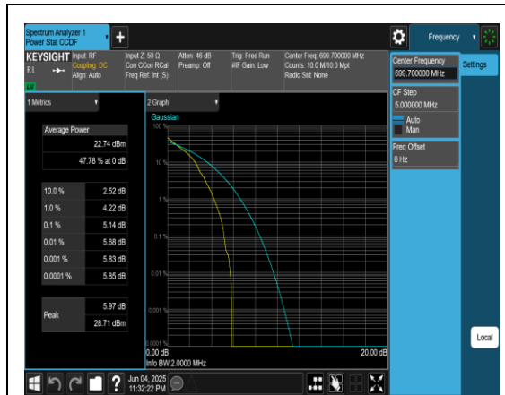
Band12-1.4MHz-QPSK-23017-1RB#0-PASS
