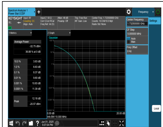
Band4-10MHz-QPSK-20175-50RB#0-PASS
