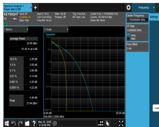
Band4-1.4MHz-QPSK-20393-1RB#0-PASS
