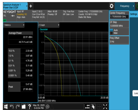
Band4-3MHz-QPSK-20385-15RB#0-PASS
