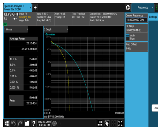
Band2-15MHz-QPSK-18900-1RB#0-PASS
