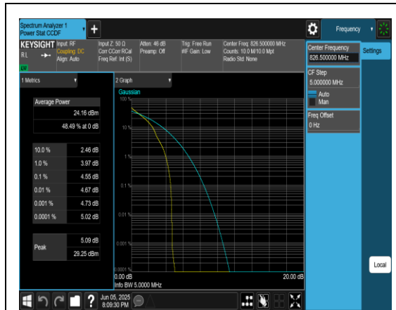
Band5-5MHz-QPSK-20425-1RB#0-PASS
