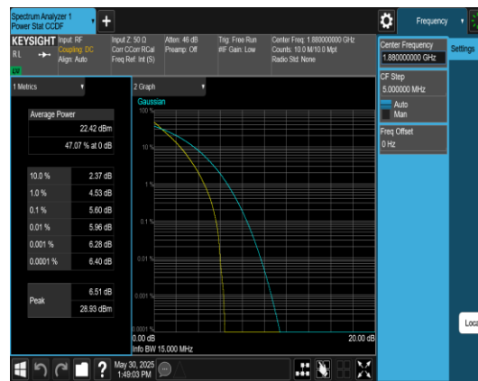
Band2-15MHz-QPSK-18900-75RB#0-PASS
