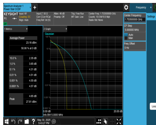
Band4-3MHz-QPSK-20385-1RB#0-PASS
