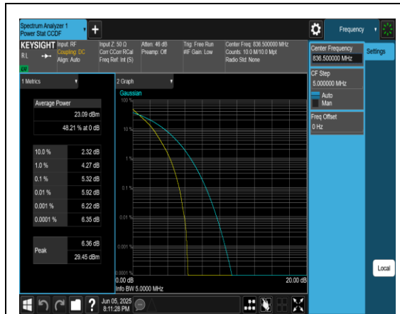
Band5-5MHz-QPSK-20525-25RB#0-PASS
