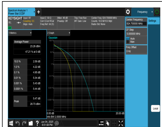
Band5-1.4MHz-QPSK-20407-1RB#0-PASS
