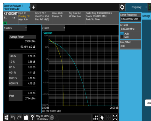
Band2-1.4MHz-QPSK-19193-1RB#0-PASS
