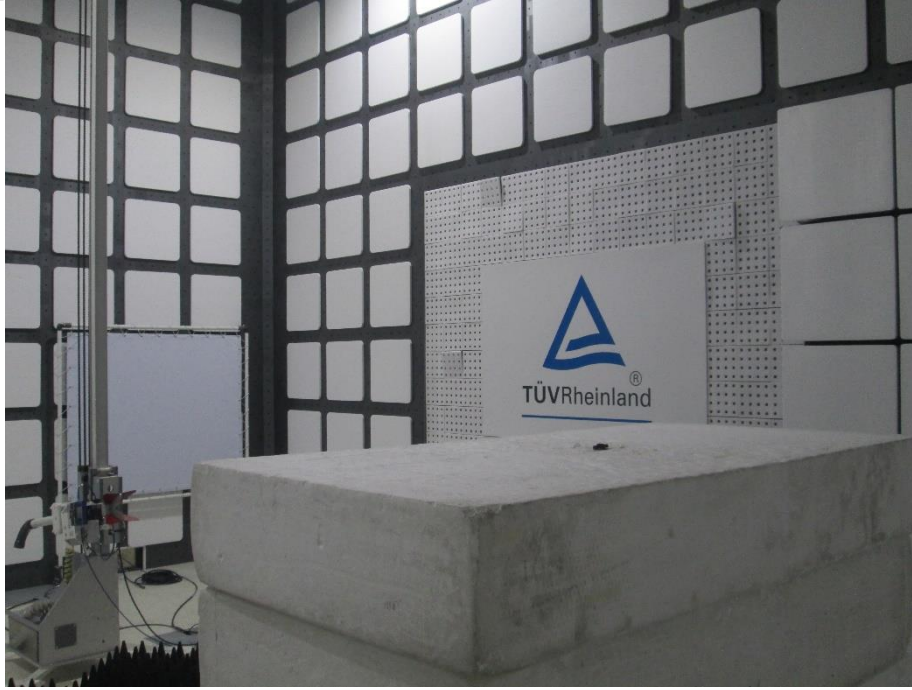
Photograph 6: Test Setup for Spurious Emissions (Front View 1, 433.92MHz)
