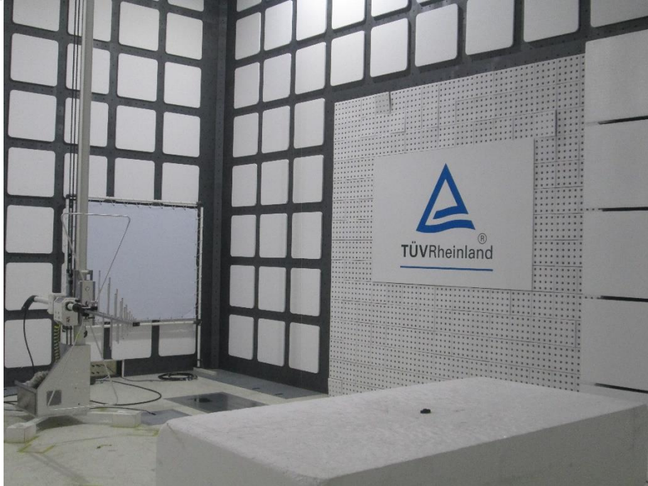
Photograph 9: Test Setup for Spurious Emissions (Back View 2, 433.92MHz)
