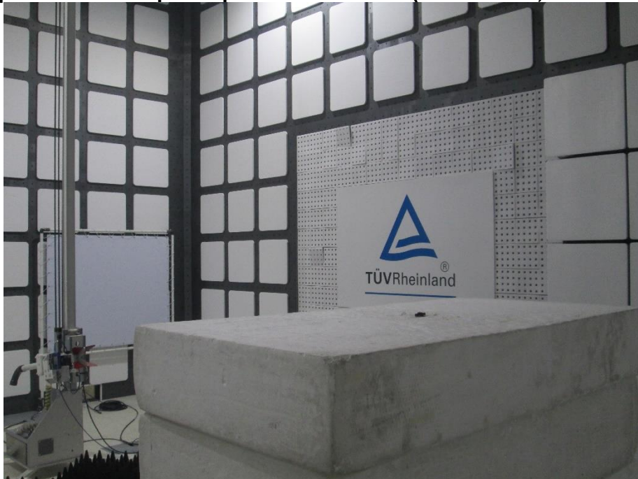
Photograph 10: Test Setup for Spurious Emissions (Back View 3, 433.92MHz)
