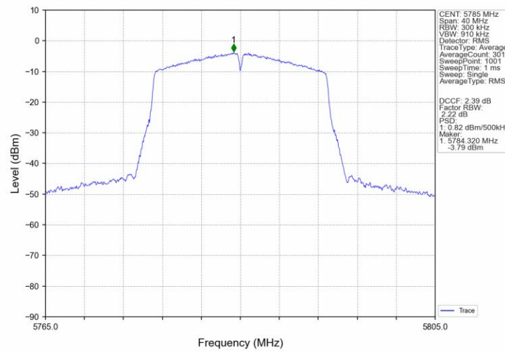
802.11ac(VHT20)_MCH_5785MHz_Ant2_NTNV
