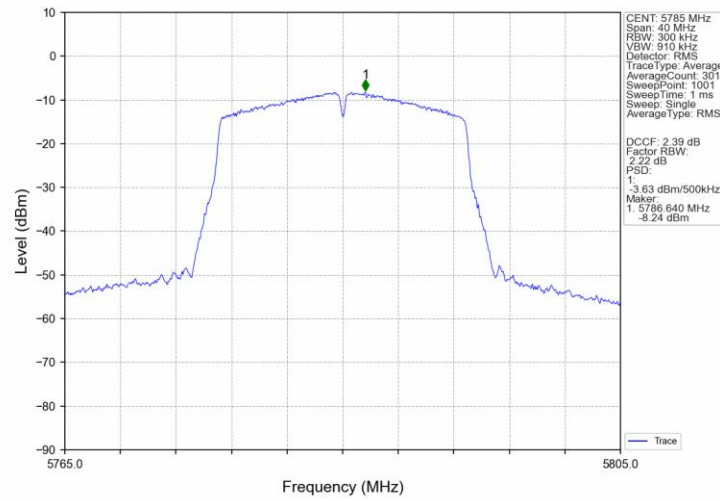
802.11ac(VHT20)_MCH_5785MHz_Ant2_NTNV
