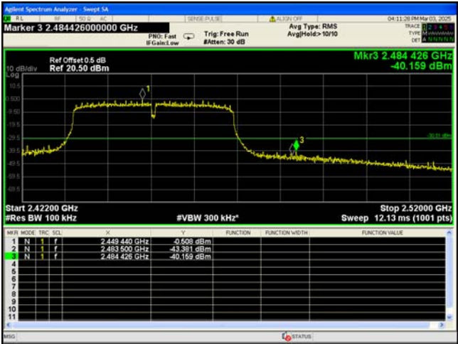
TX 11n HT40: Band edge-right side
