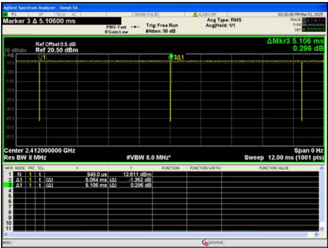
Wi-Fi 802.11n-HT20
