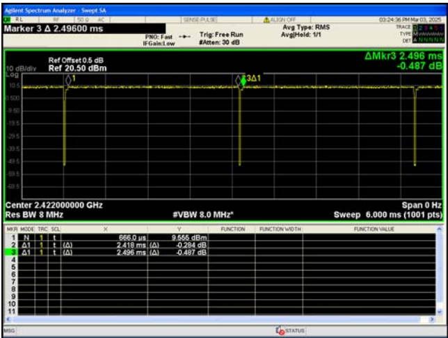
Wi-Fi 802.11n-HT40
