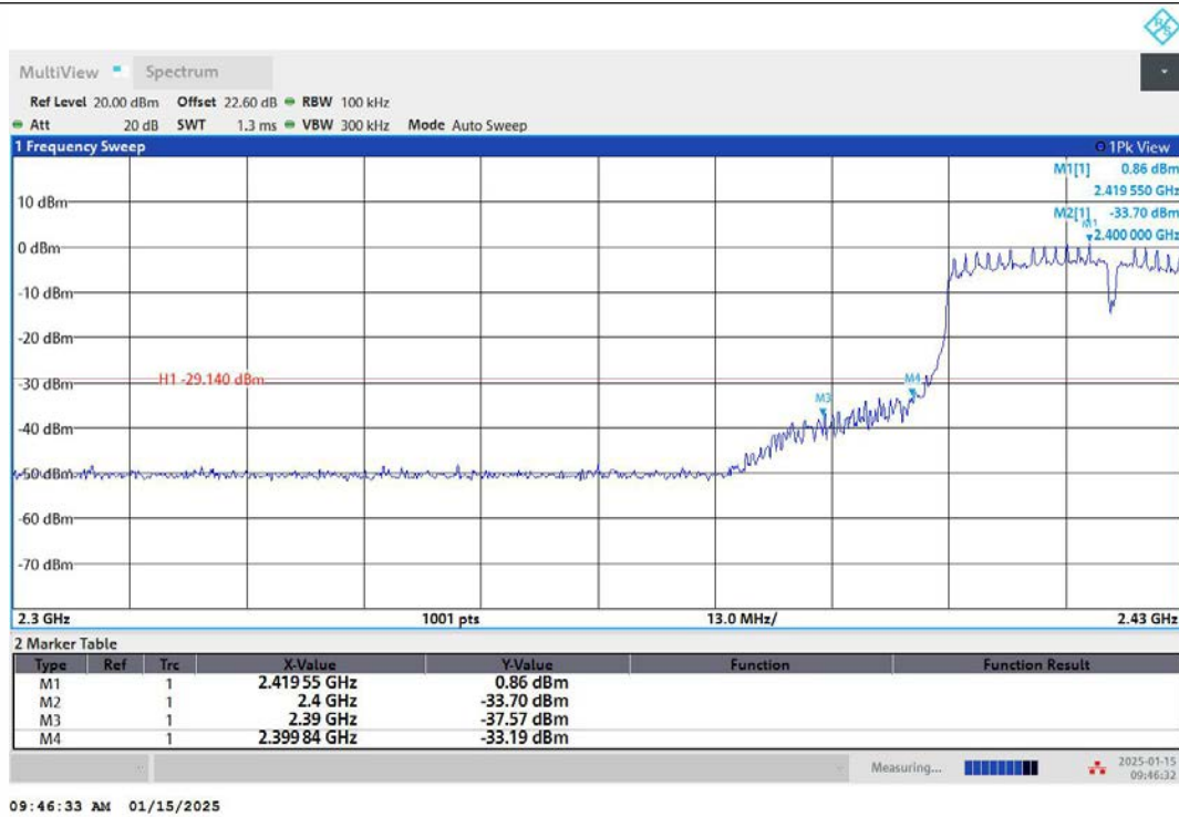
11N40SISO-Ant1-2422-PASS
