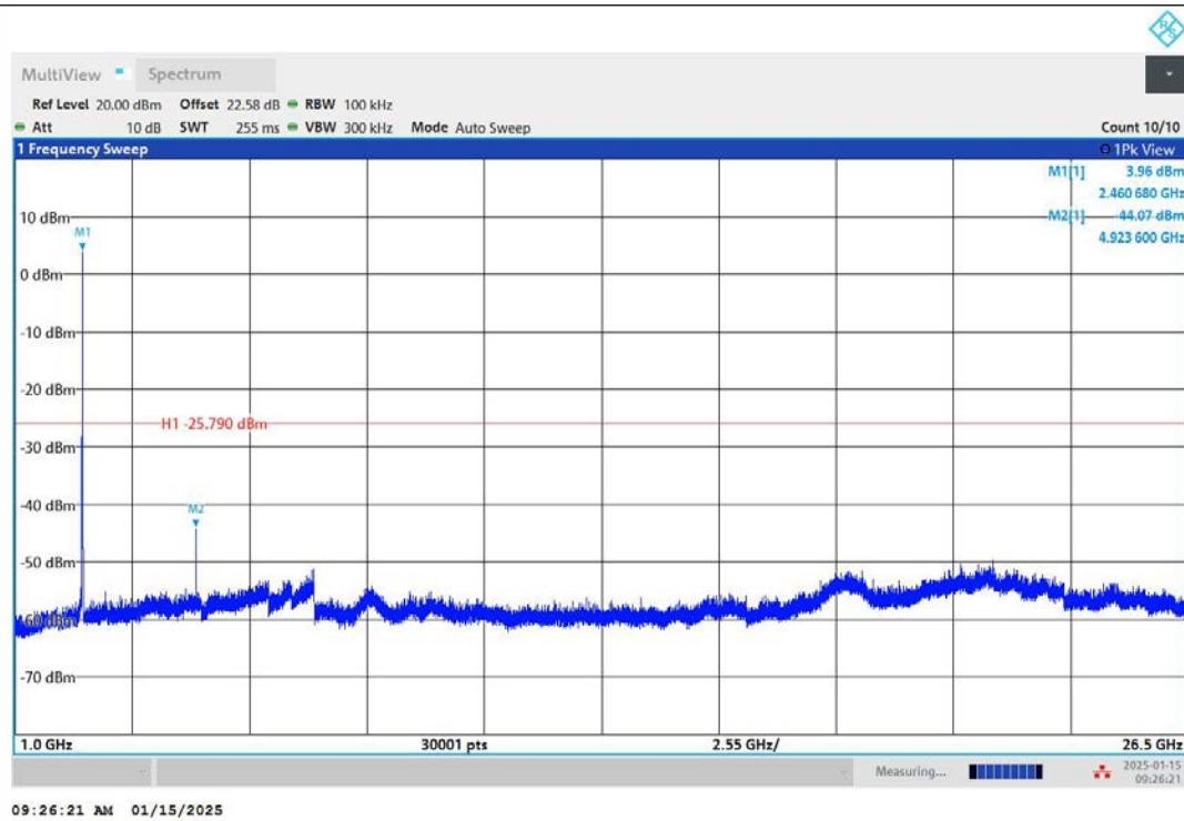
11B-Ant1-2462-1000~26500-PASS
