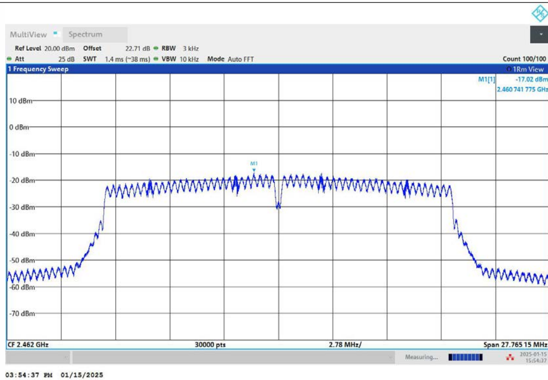
11N20SISO-Ant1-2462-PASS
