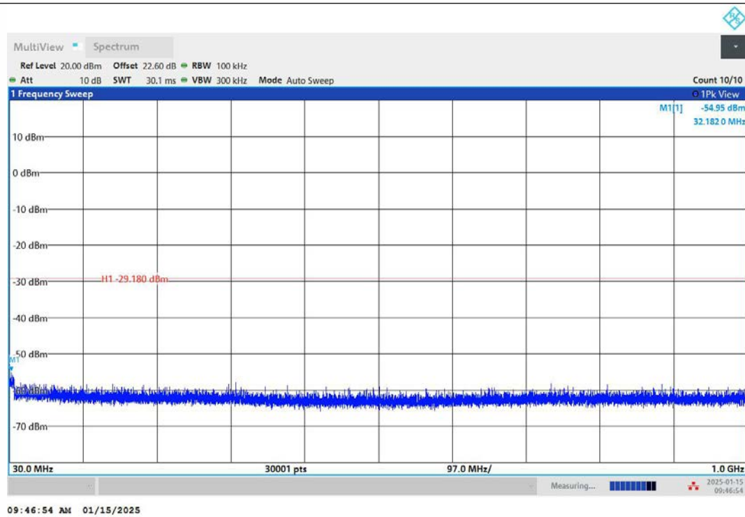
11N40SISO-Ant1-2422-30~1000-PASS
