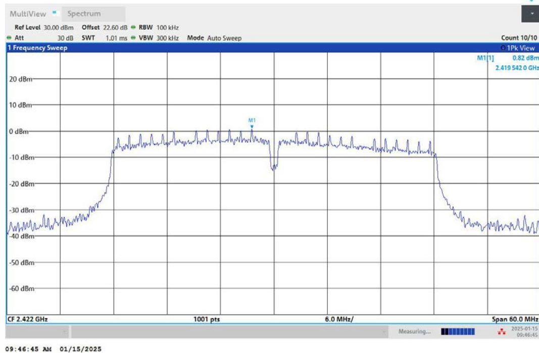
11N40SISO-Ant1-2422-0~Reference-PASS
