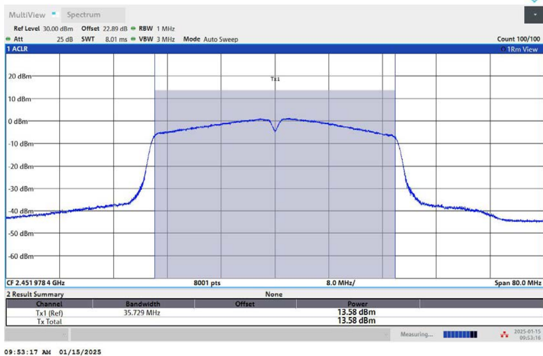
11N40SISO-Ant1-2452-PASS
