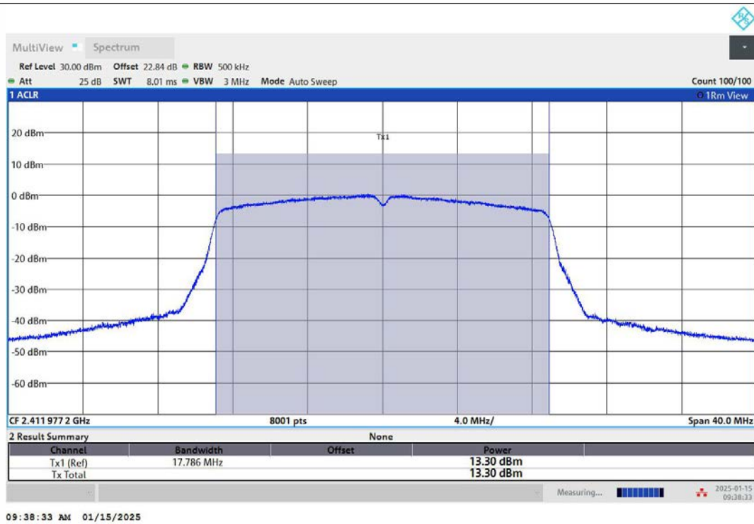
11N20SISO-Ant1-2412-PASS
