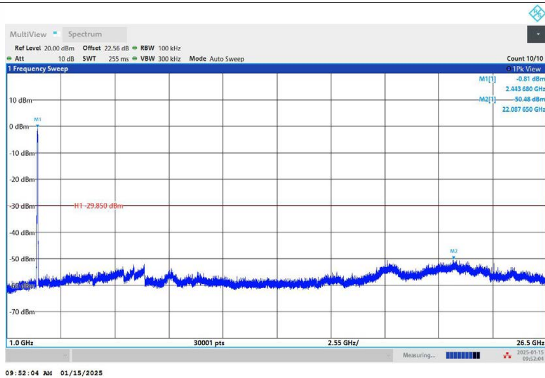
11N40SISO-Ant1-2437-1000~26500-PASS
