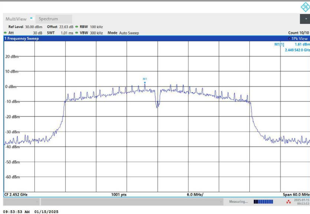
11N40SISO-Ant1-2452-0~Reference-PASS
