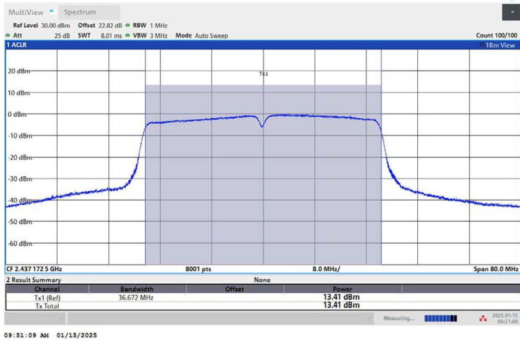
11N40SISO-Ant1-2437-PASS
