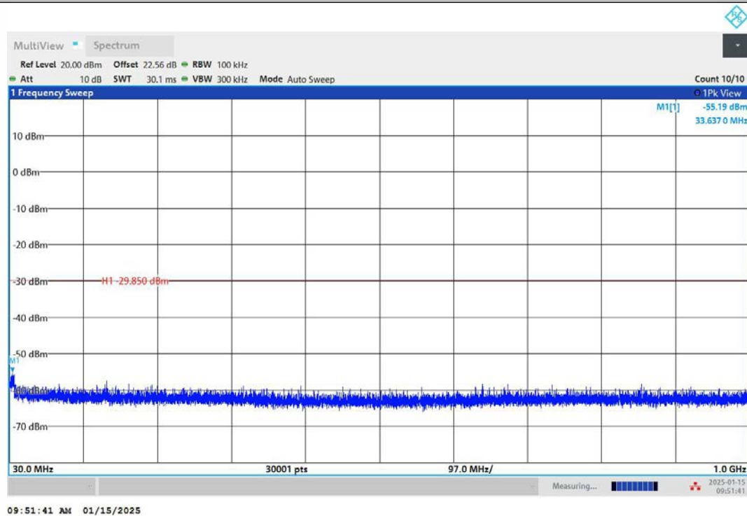
11N40SISO-Ant1-2437-30~1000-PASS
