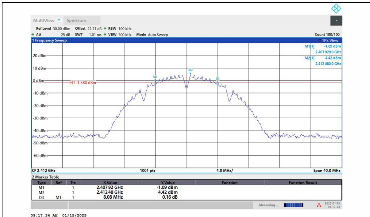
11B-Ant1-2412-PASS
