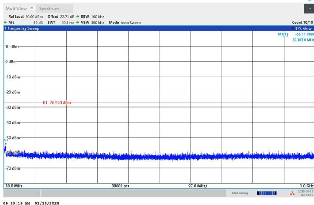
11N20SISO-Ant1-2412-30~1000-PASS
