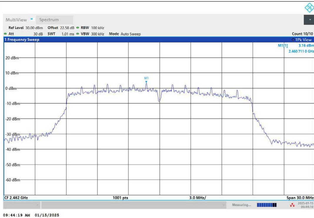
11N20SISO-Ant1-2462-0~Reference-PASS
