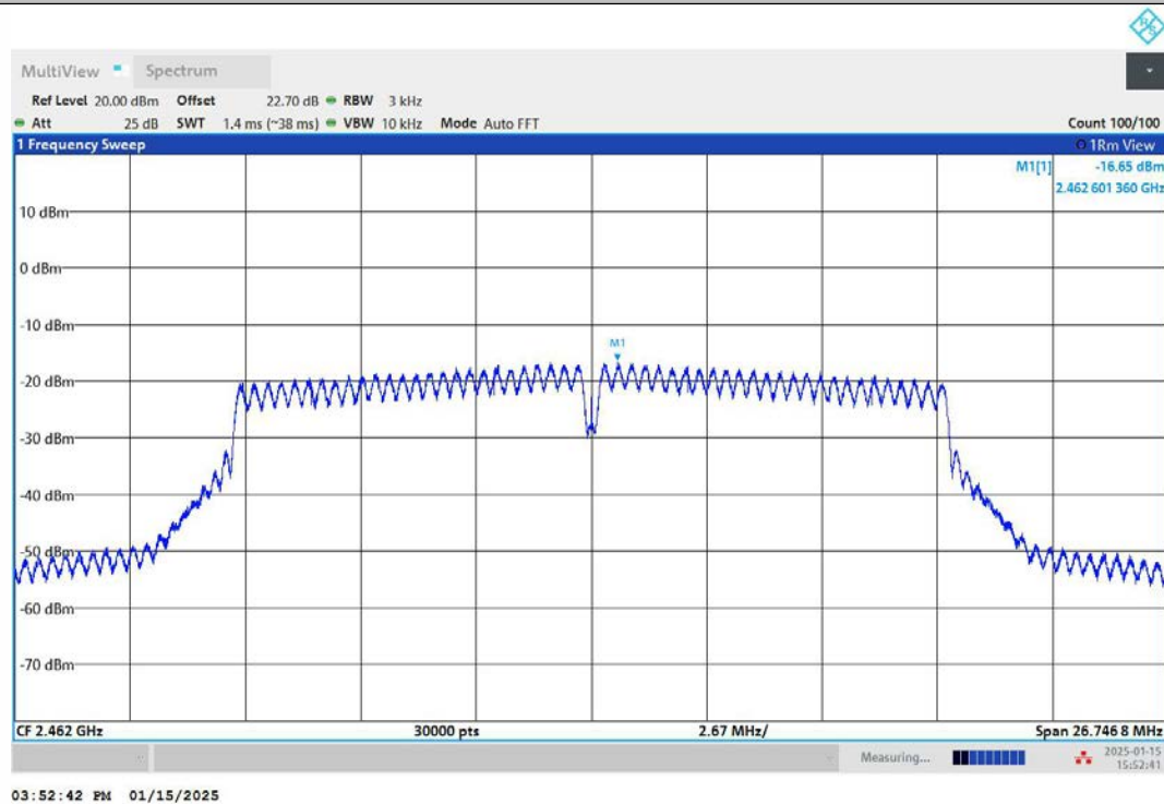
11G-Ant1-2462-PASS
