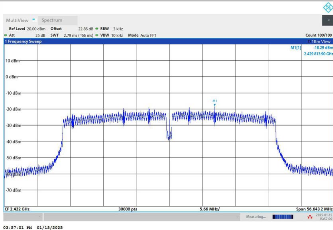
11N40SISO-Ant1-2422-PASS
