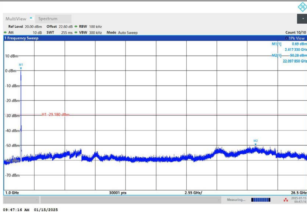
11N40SISO-Ant1-2422-1000~26500-PASS
