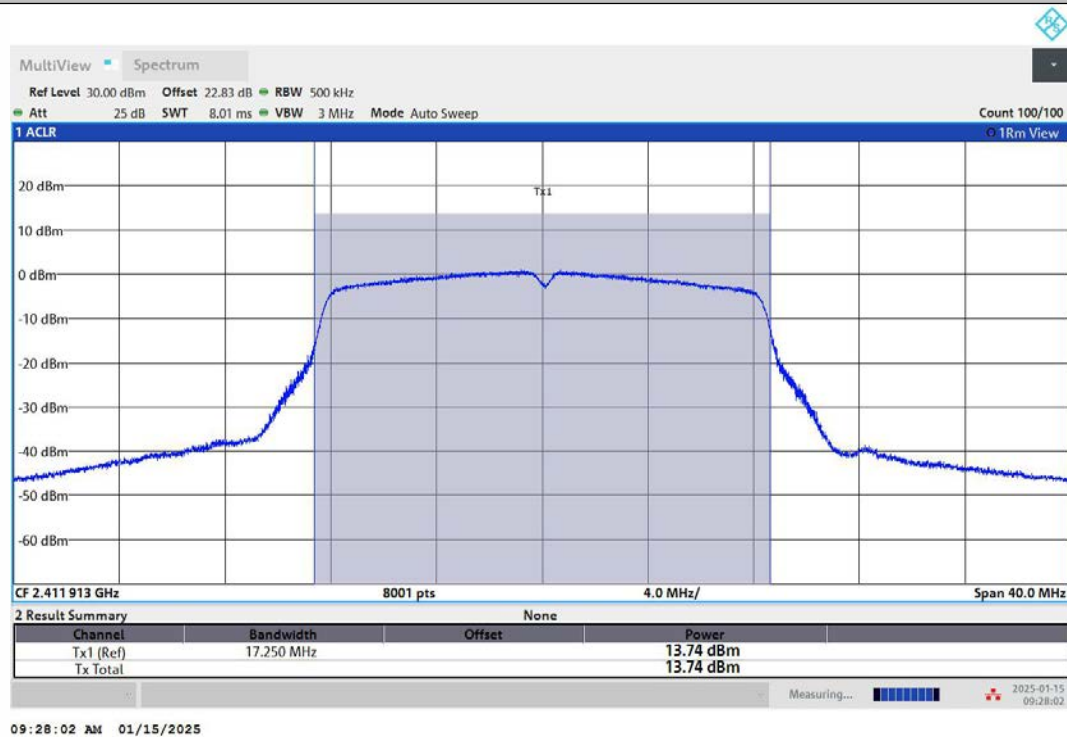
11G-Ant1-2412-PASS
