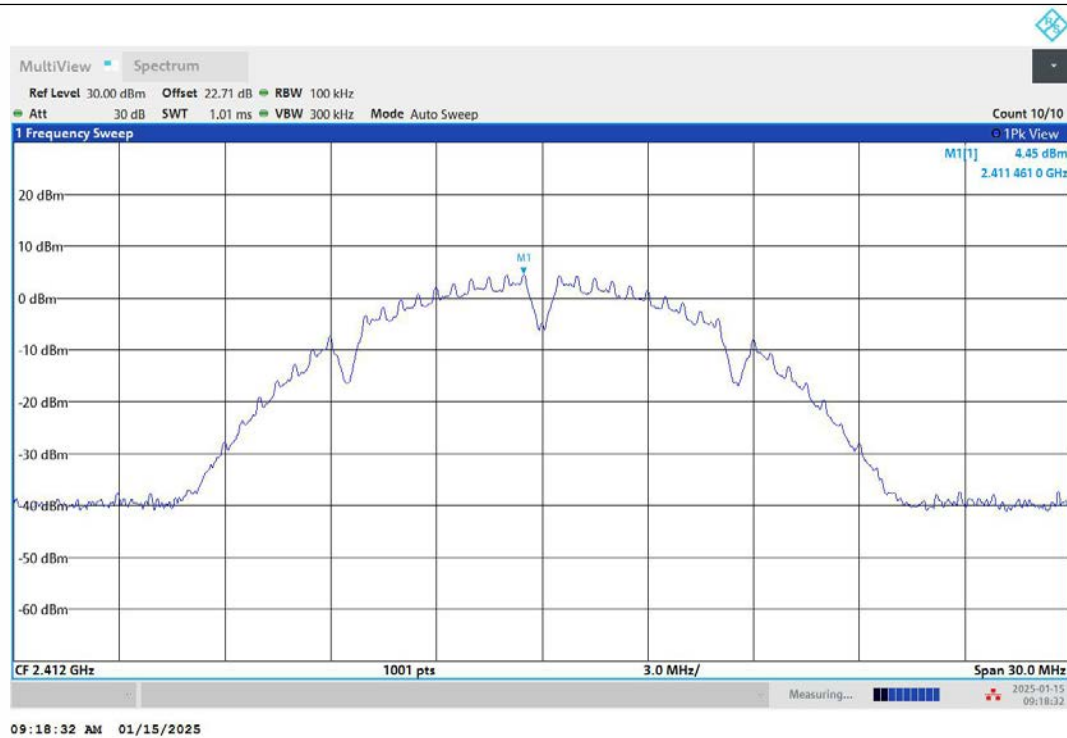
11B-Ant1-2412-0~Reference-PASS
