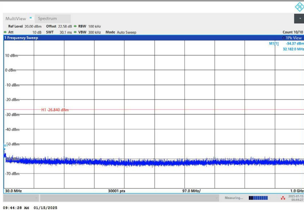
11N20SISO-Ant1-2462-30~1000-PASS
