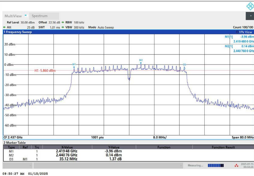
11N40SISO-Ant1-2437-PASS
