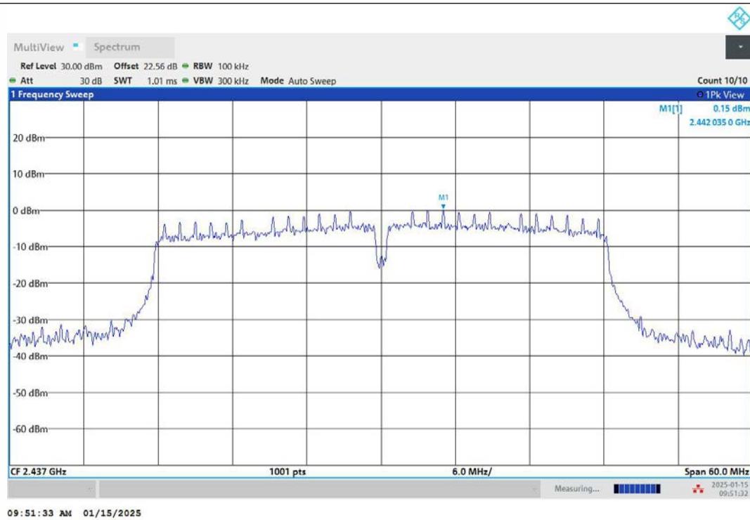
11N40SISO-Ant1-2437-0~Reference-PASS
