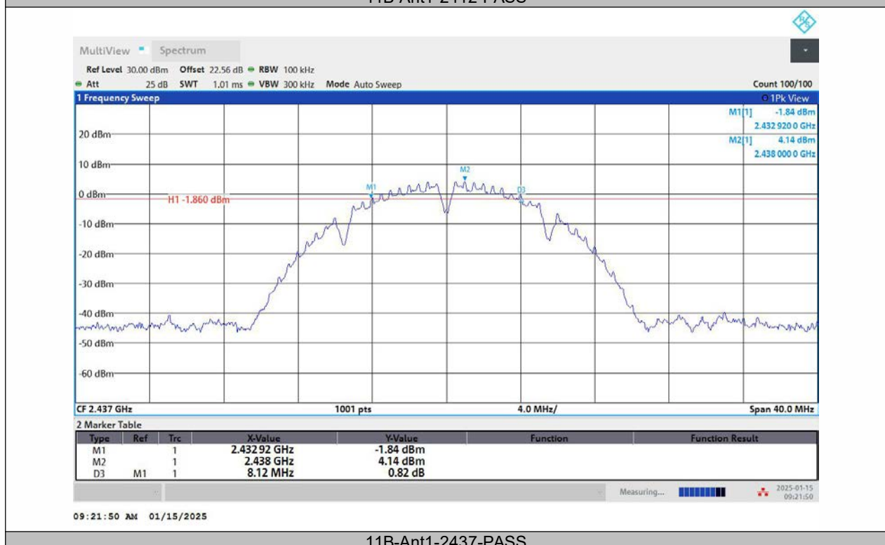
11B-Ant1-2437-PASS
