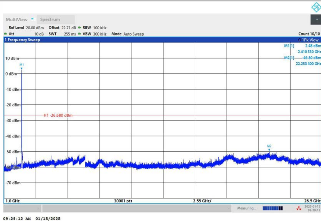
11G-Ant1-2412-1000~26500-PASS
