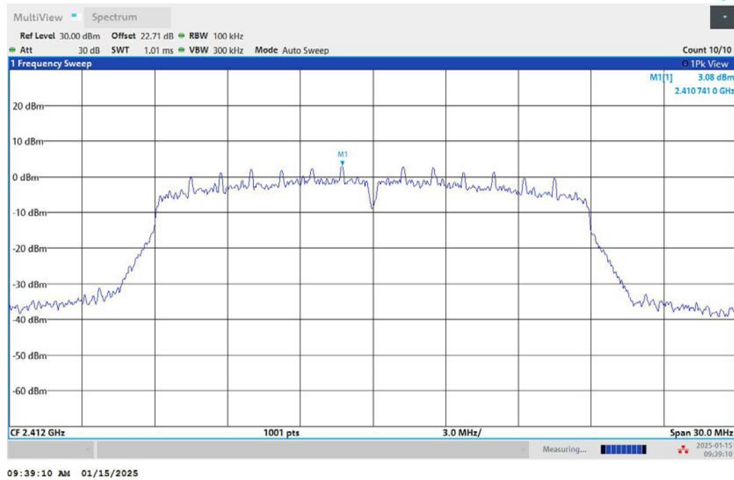
11N20SISO-Ant1-2412-0~Reference-PASS
