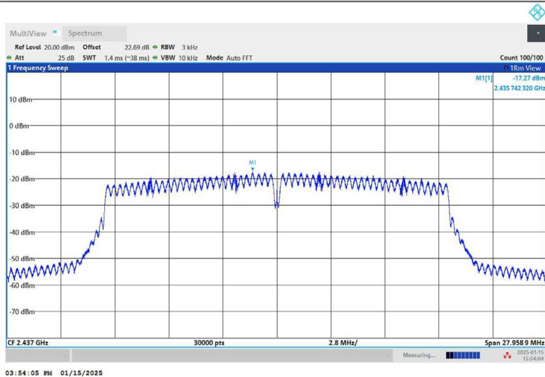
11N20SISO-Ant1-2437-PASS
