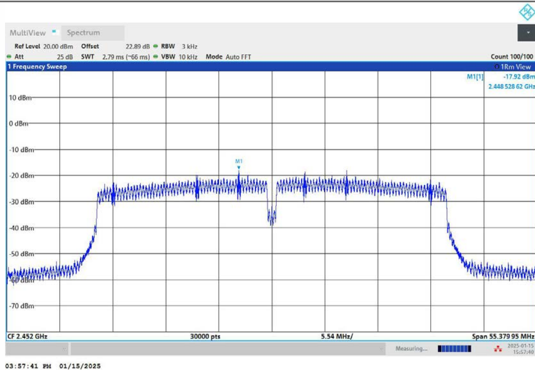
11N40SISO-Ant1-2452-PASS
