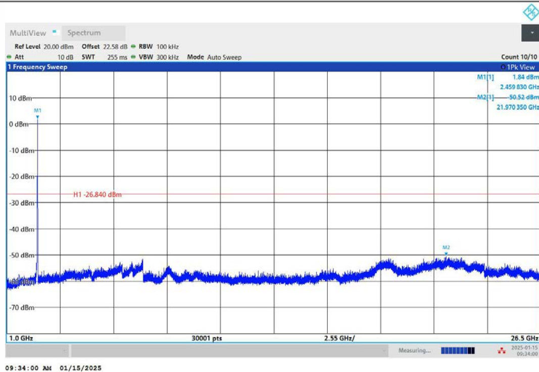
11G-Ant1-2462-1000~26500-PASS
