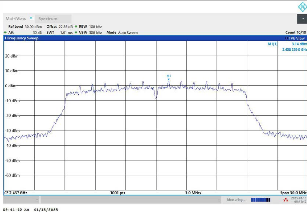
11N20SISO-Ant1-2437-0~Reference-PASS
