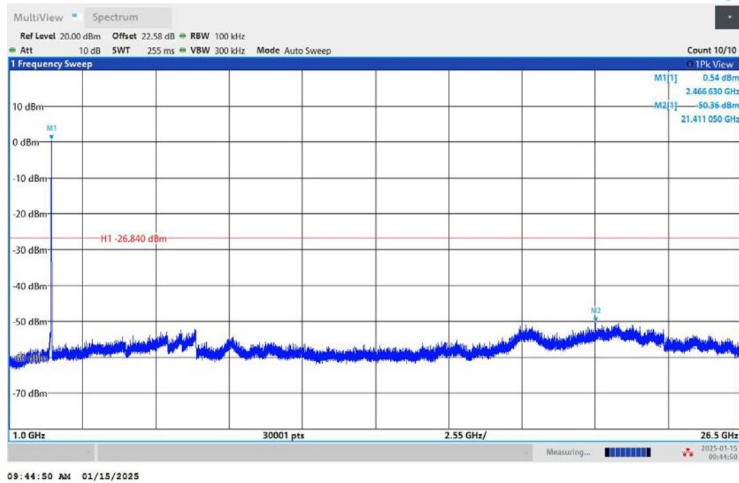
11N20SISO-Ant1-2462-1000~26500-PASS
