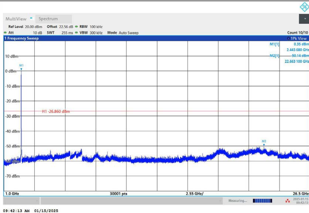
11N20SISO-Ant1-2437-1000~26500-PASS
