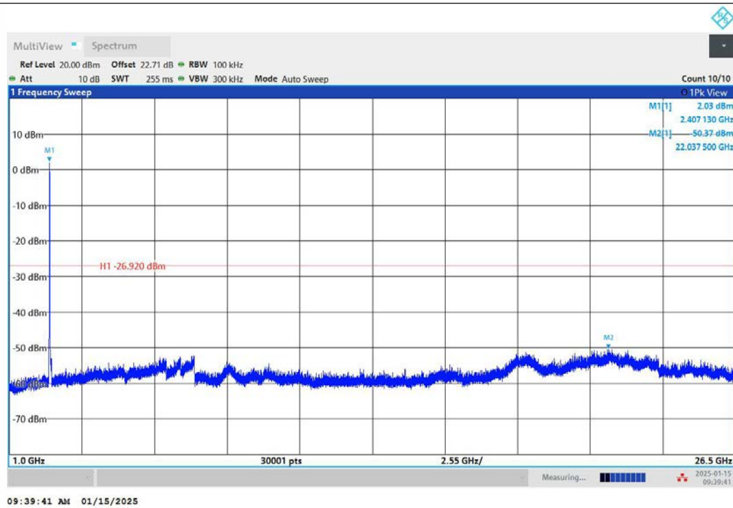
11N20SISO-Ant1-2412-1000~26500-PASS
