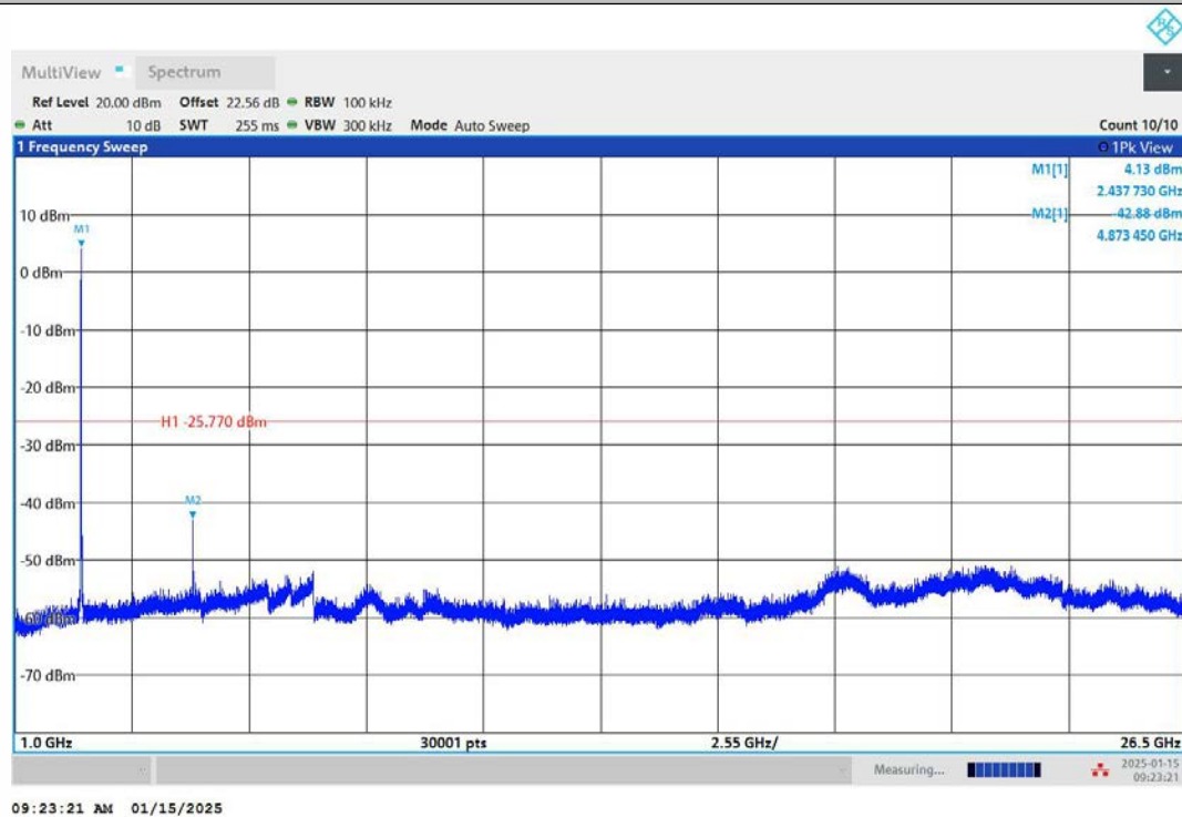
11B-Ant1-2437-1000~26500-PASS
