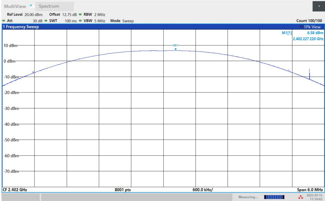
BLE_1M-Ant1-2402-PASS
