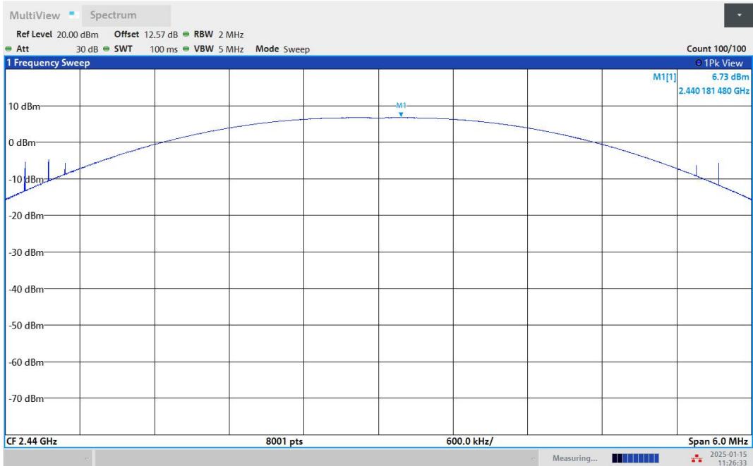
BLE_1M-Ant1-2440-PASS
