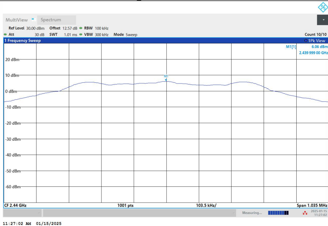
BLE_1M-Ant1-2440-PASS
