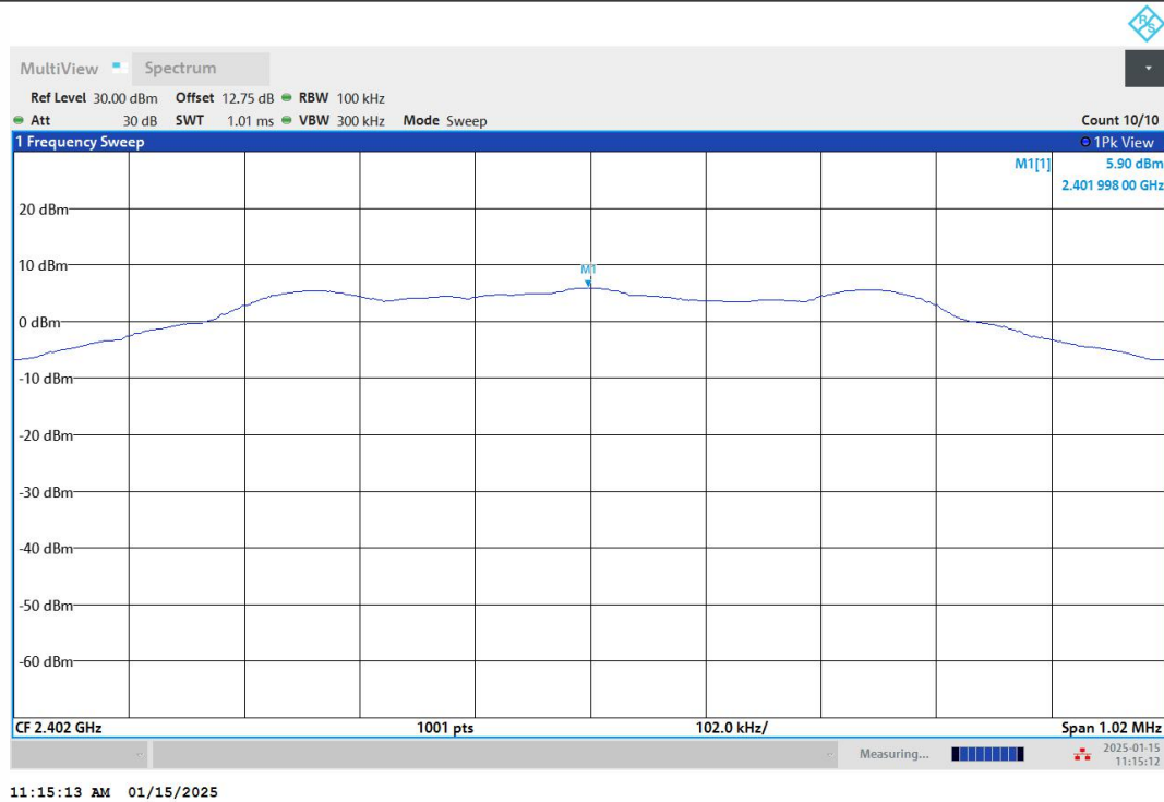
BLE_1M-Ant1-2402-PASS
