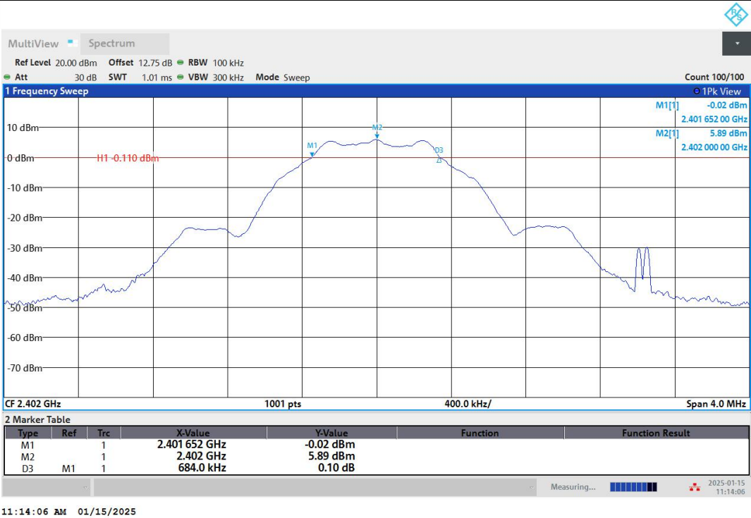
BLE_1M-Ant1-2402-PASS
