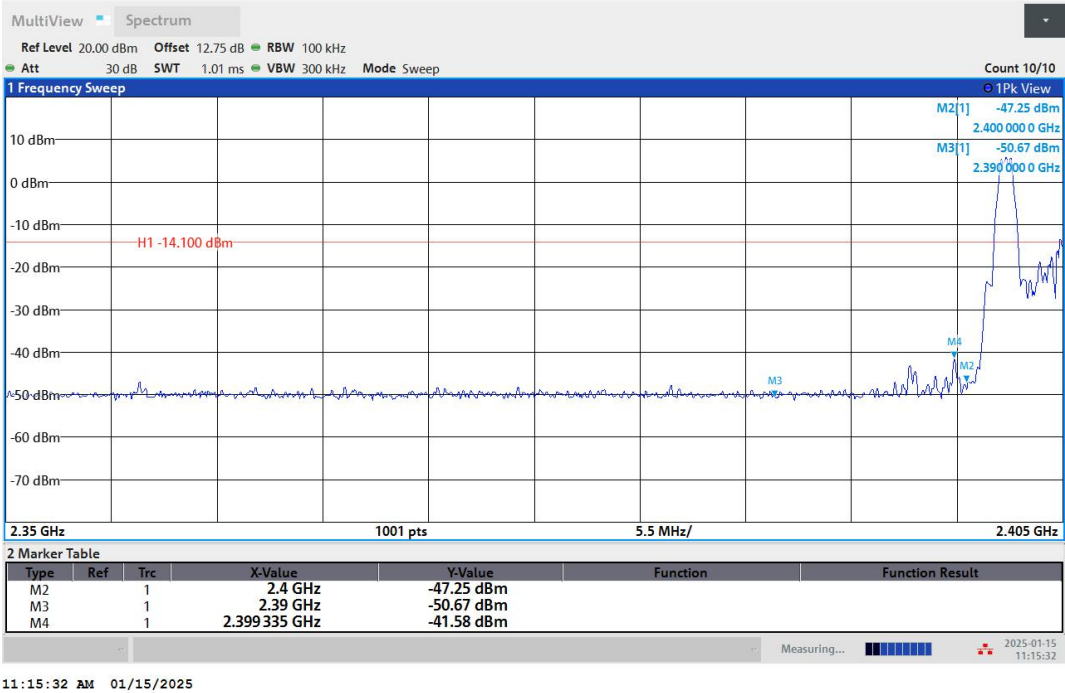
BLE_1M-Ant1-2402-PASS
