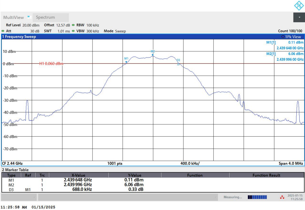
BLE_1M-Ant1-2440-PASS
