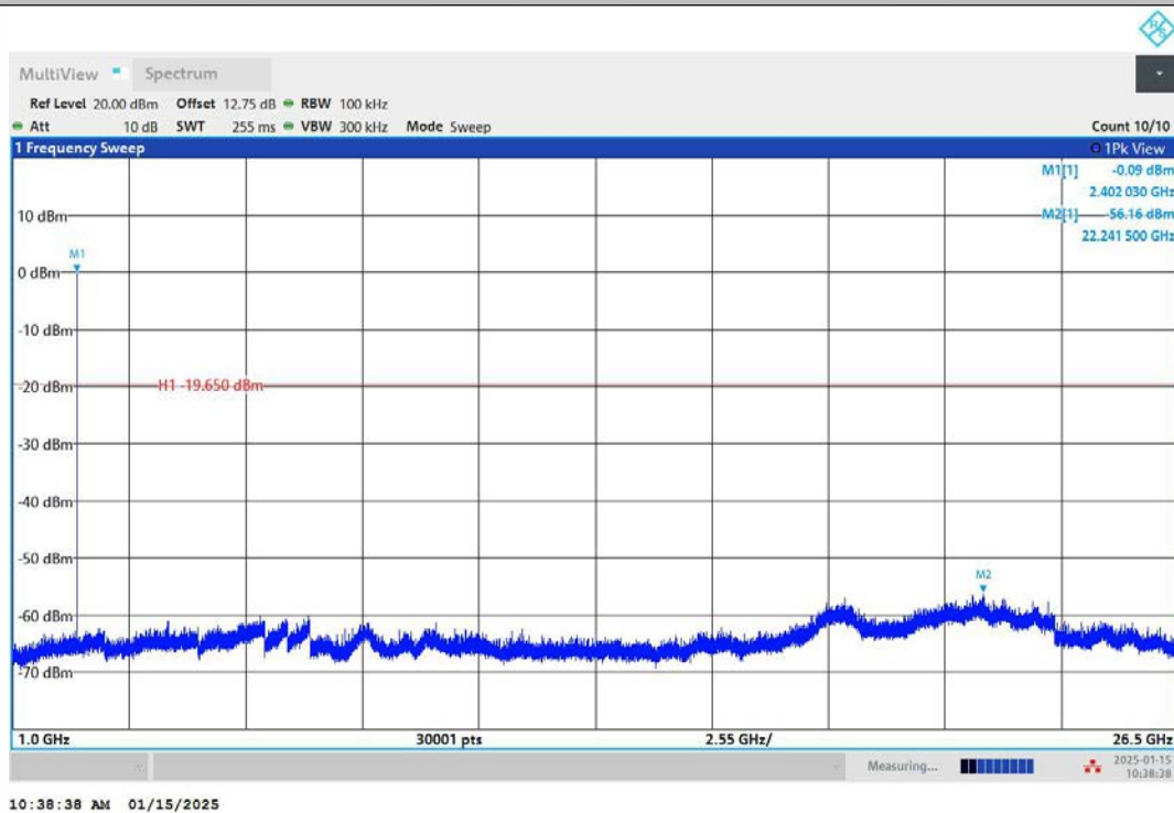
3DH5-Ant1-2402-1000~26500-PASS
