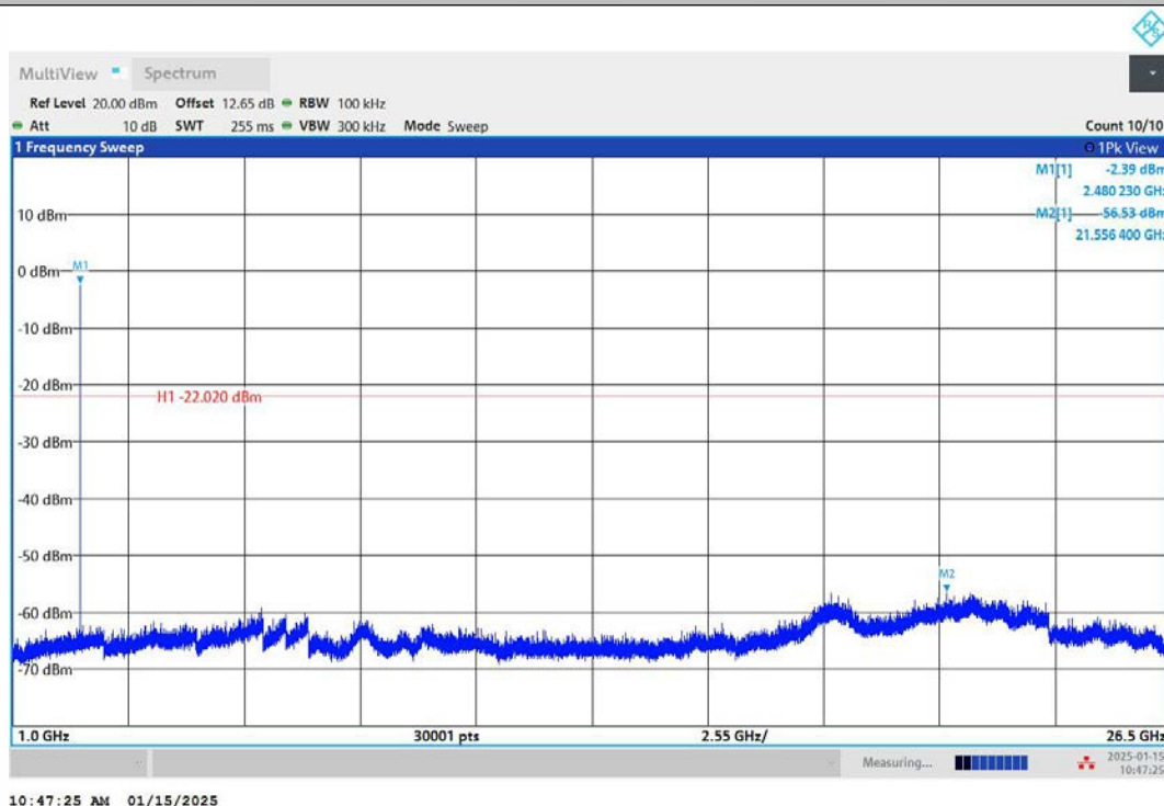
3DH5-Ant1-2480-1000~26500-PASS
