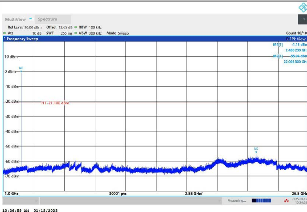
DH5-Ant1-2480-1000~26500-PASS
