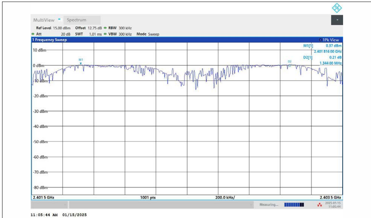
3DH5-Ant1-Hop_2402-PASS
