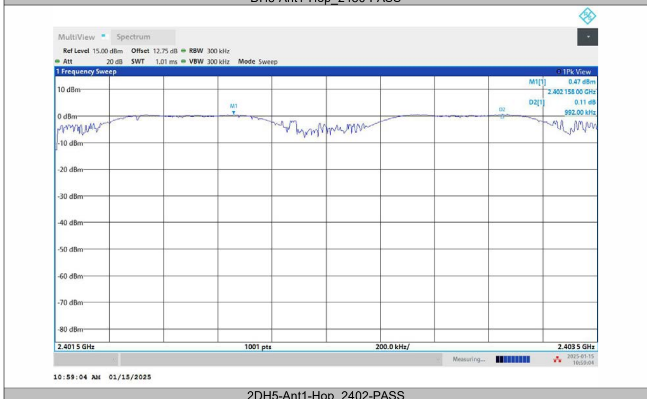
2DH5-Ant1-Hop_2402-PASS
