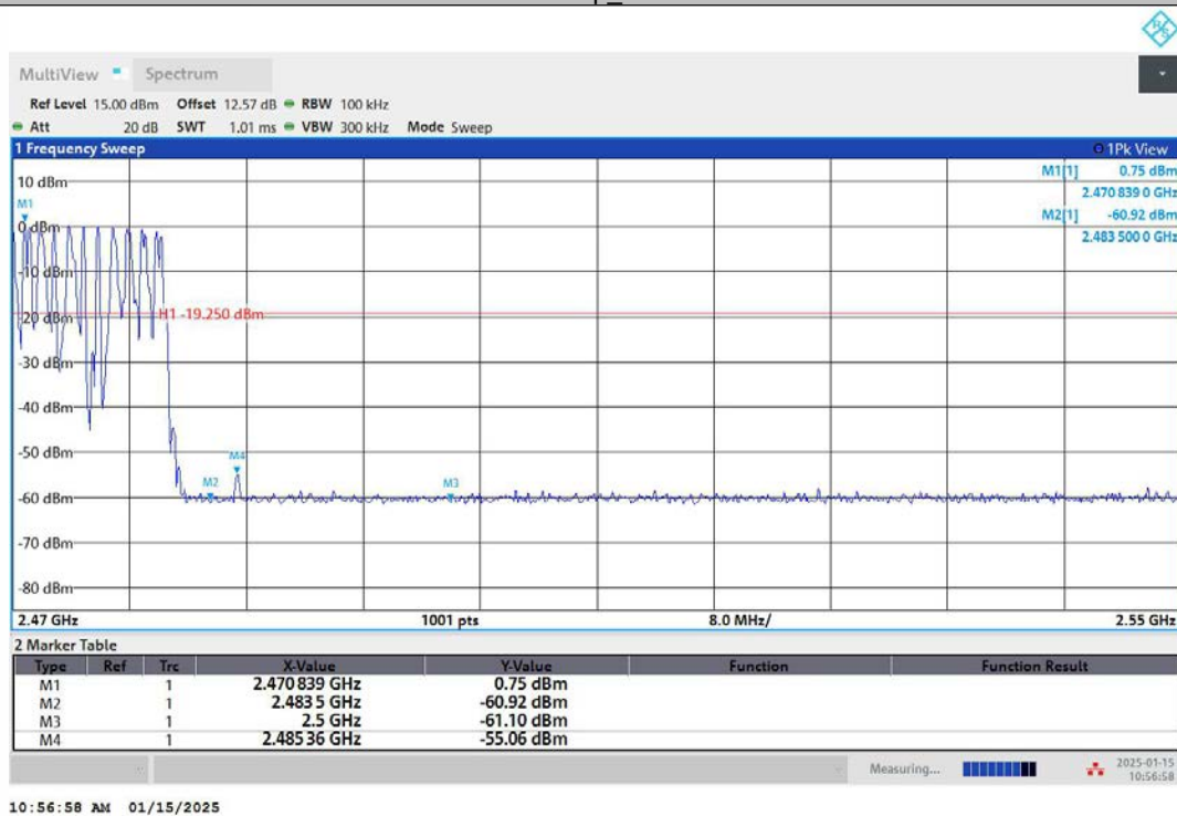
DH5-Ant1-Hop_2480-PASS
