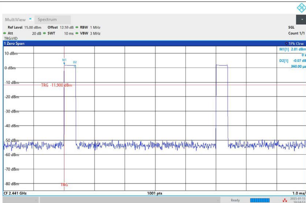
DH1-Ant1-Hop-PASS
