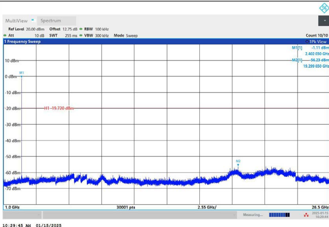
2DH5-Ant1-2402-1000~26500-PASS
