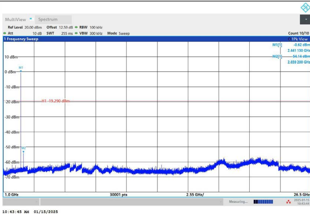
3DH5-Ant1-2441-1000~26500-PASS
