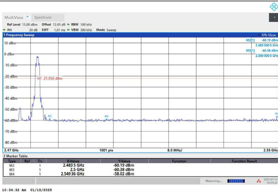
2DH5-Ant1-2480-PASS
