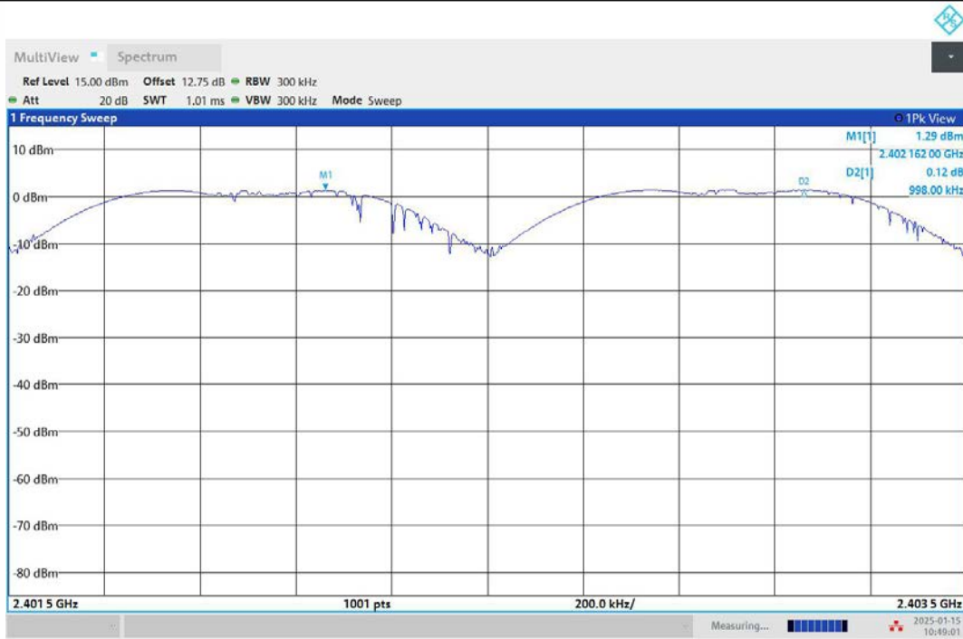
DH5-Ant1-Hop_2402-PASS
