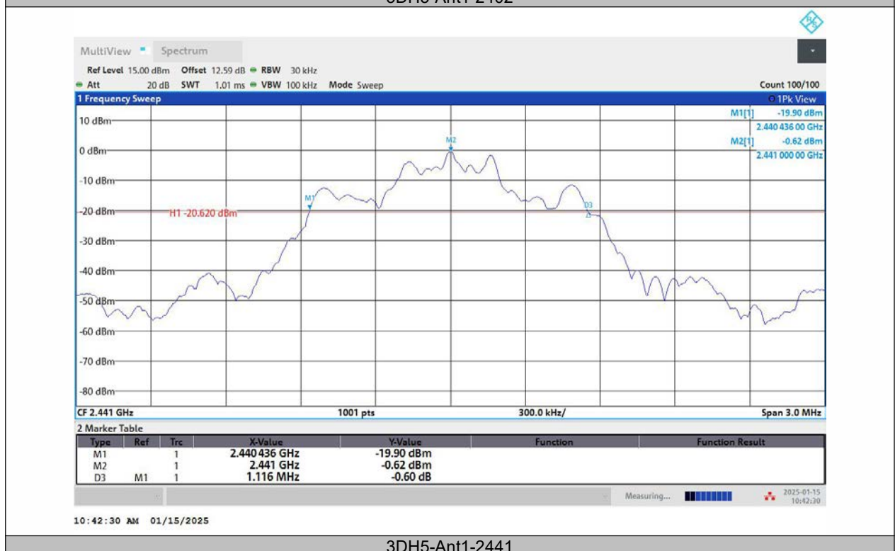
3DH5-Ant1-2441
