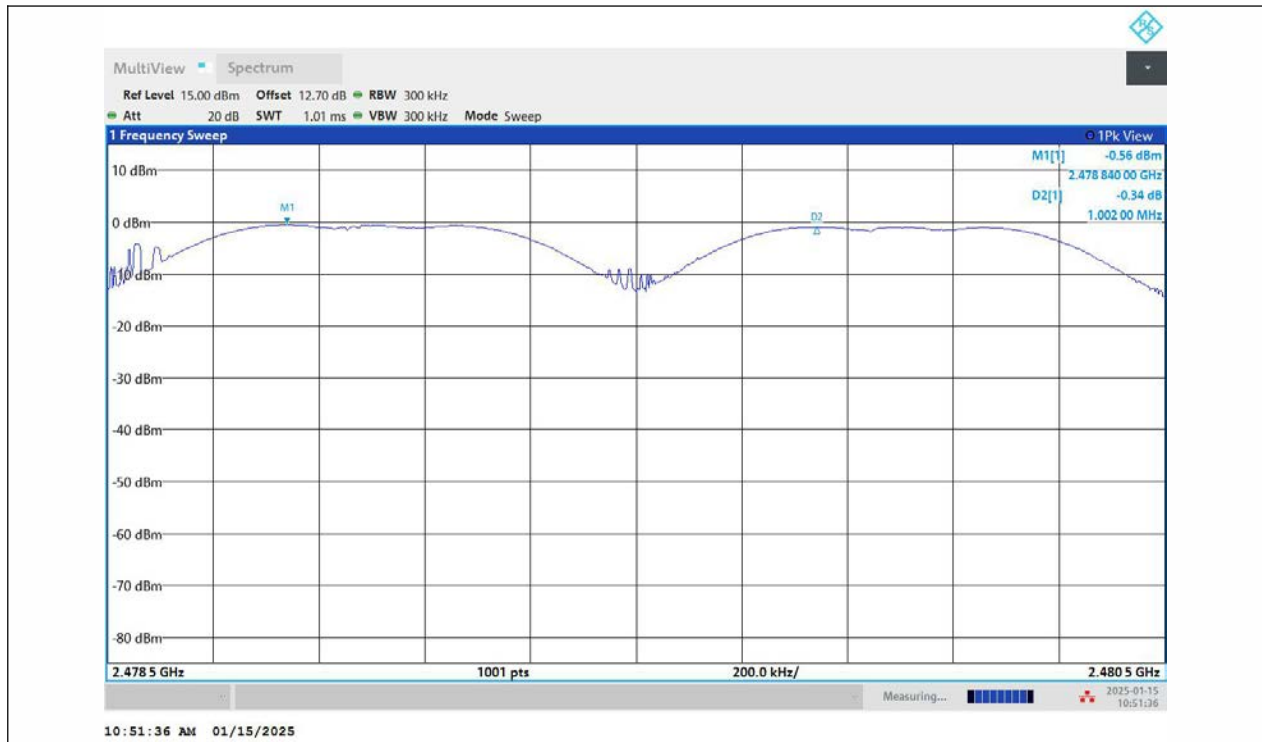
DH5-Ant1-Hop_2480-PASS
