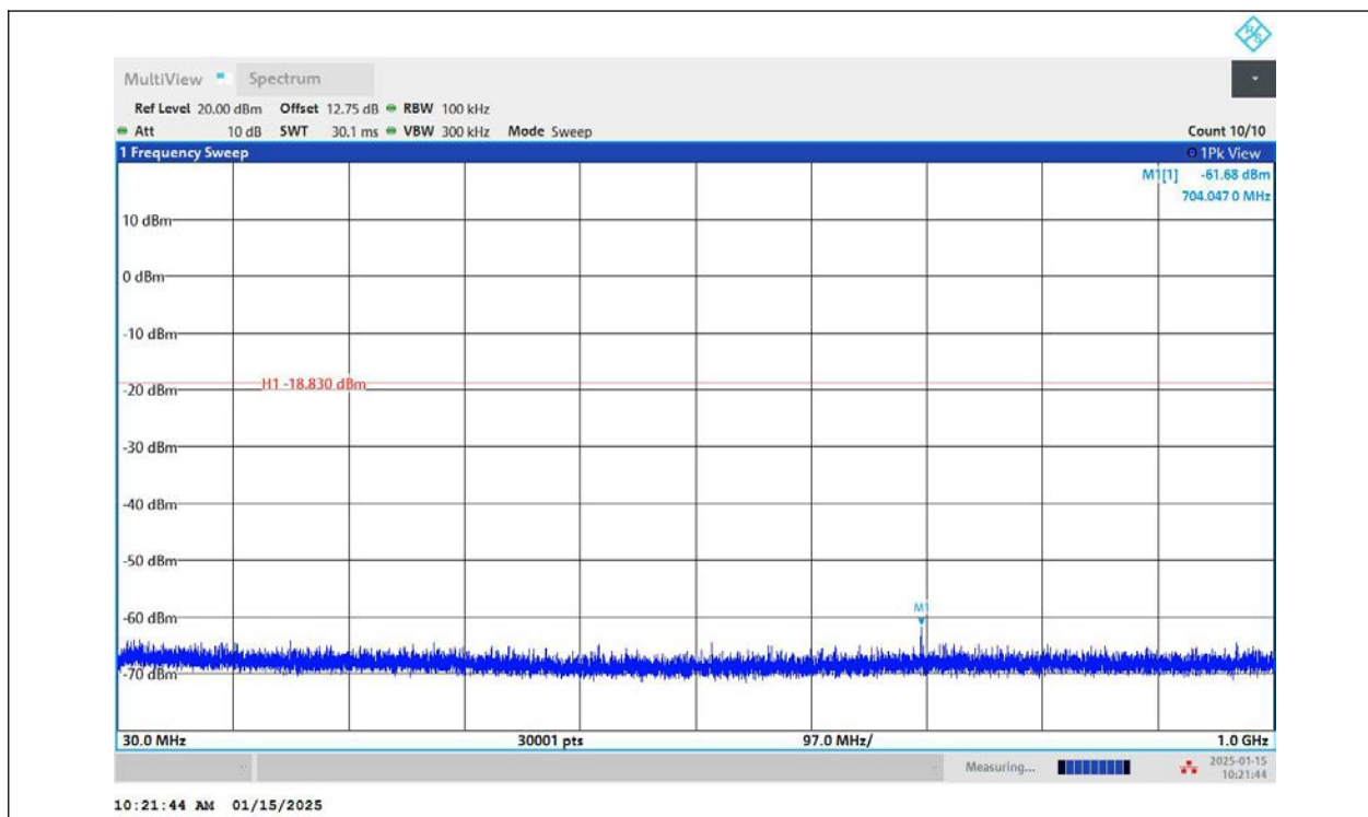
DH5-Ant1-2402-30~1000-PASS
