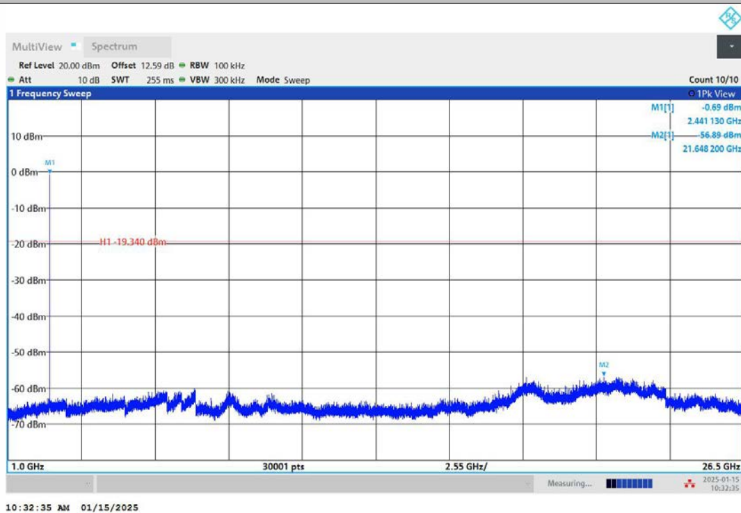
2DH5-Ant1-2441-1000~26500-PASS
