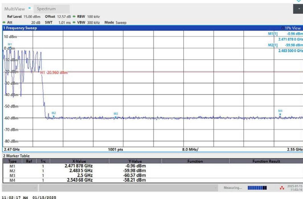
2DH5-Ant1-Hop_2480-PASS
