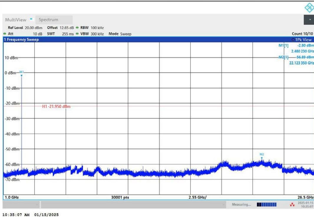
2DH5-Ant1-2480-1000~26500-PASS
