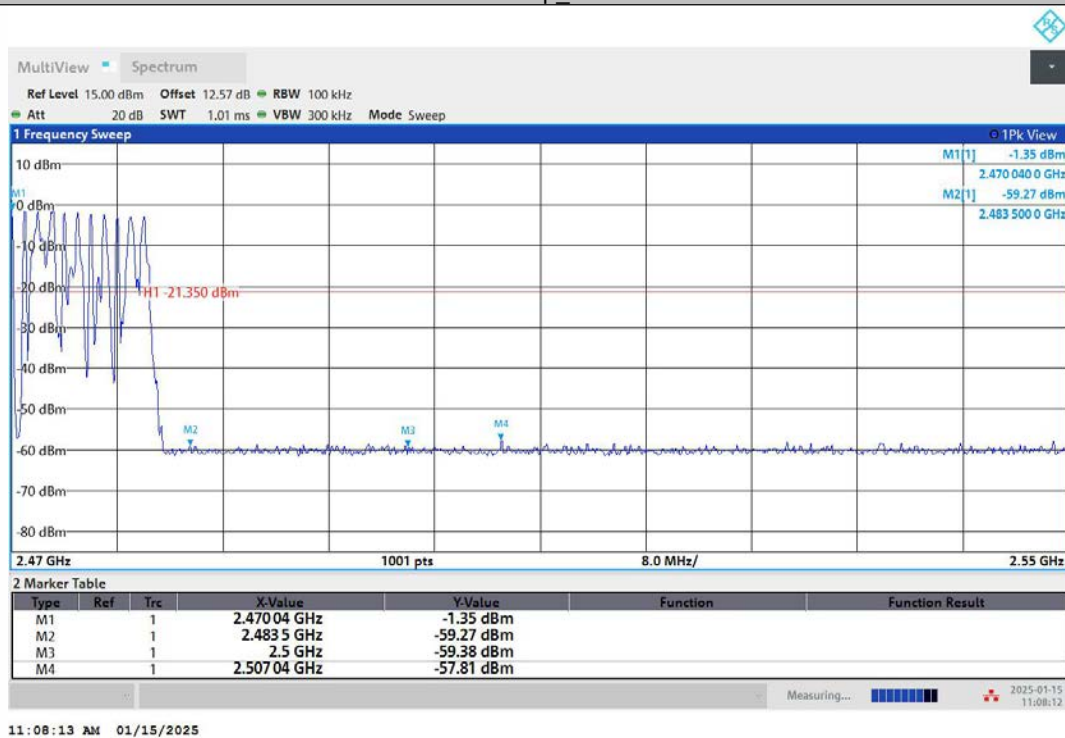
3DH5-Ant1-Hop_2480-PASS
