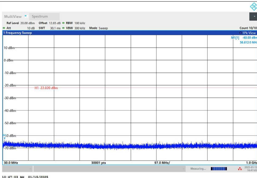
3DH5-Ant1-2480-30~1000-PASS
