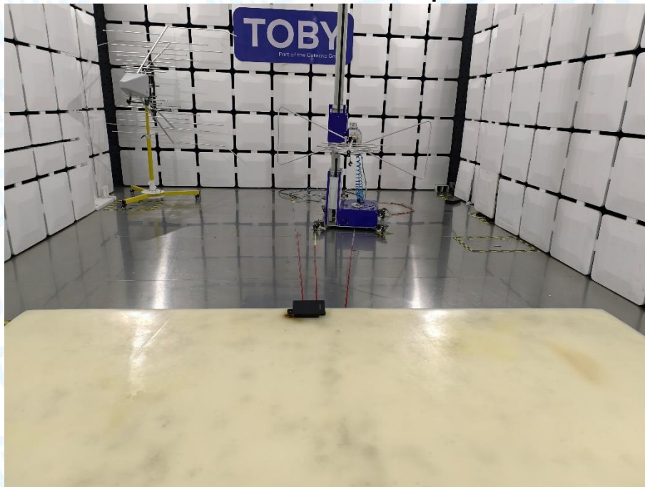
Radiated Emission Test Setup <30MHz
