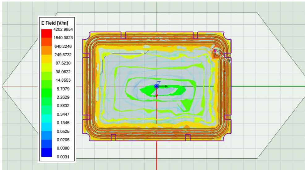
Electric Field Distribution
