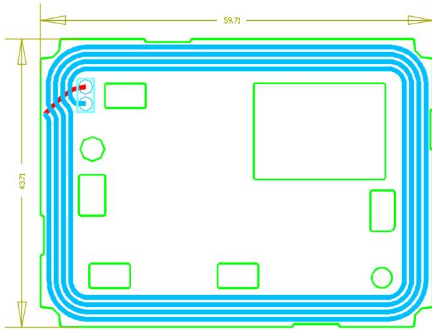
Antenna Dimension (units:mm)
