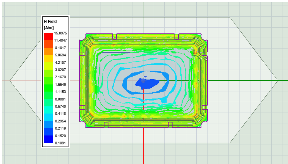
Magnetic Field Distribution
