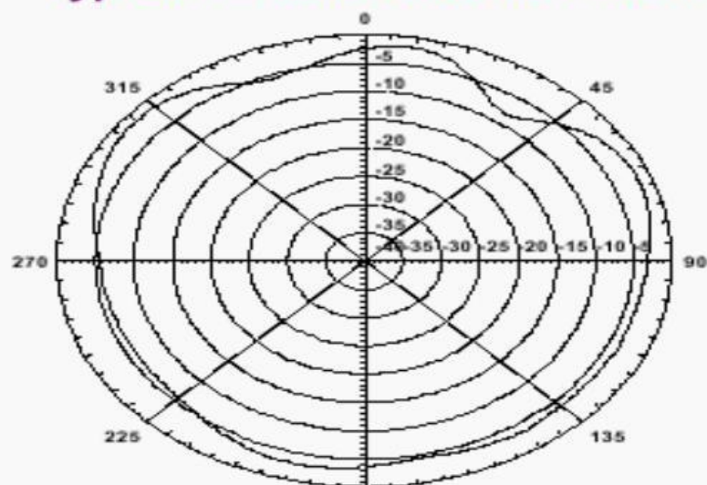
Typical H-Plane Antenna Pattern
